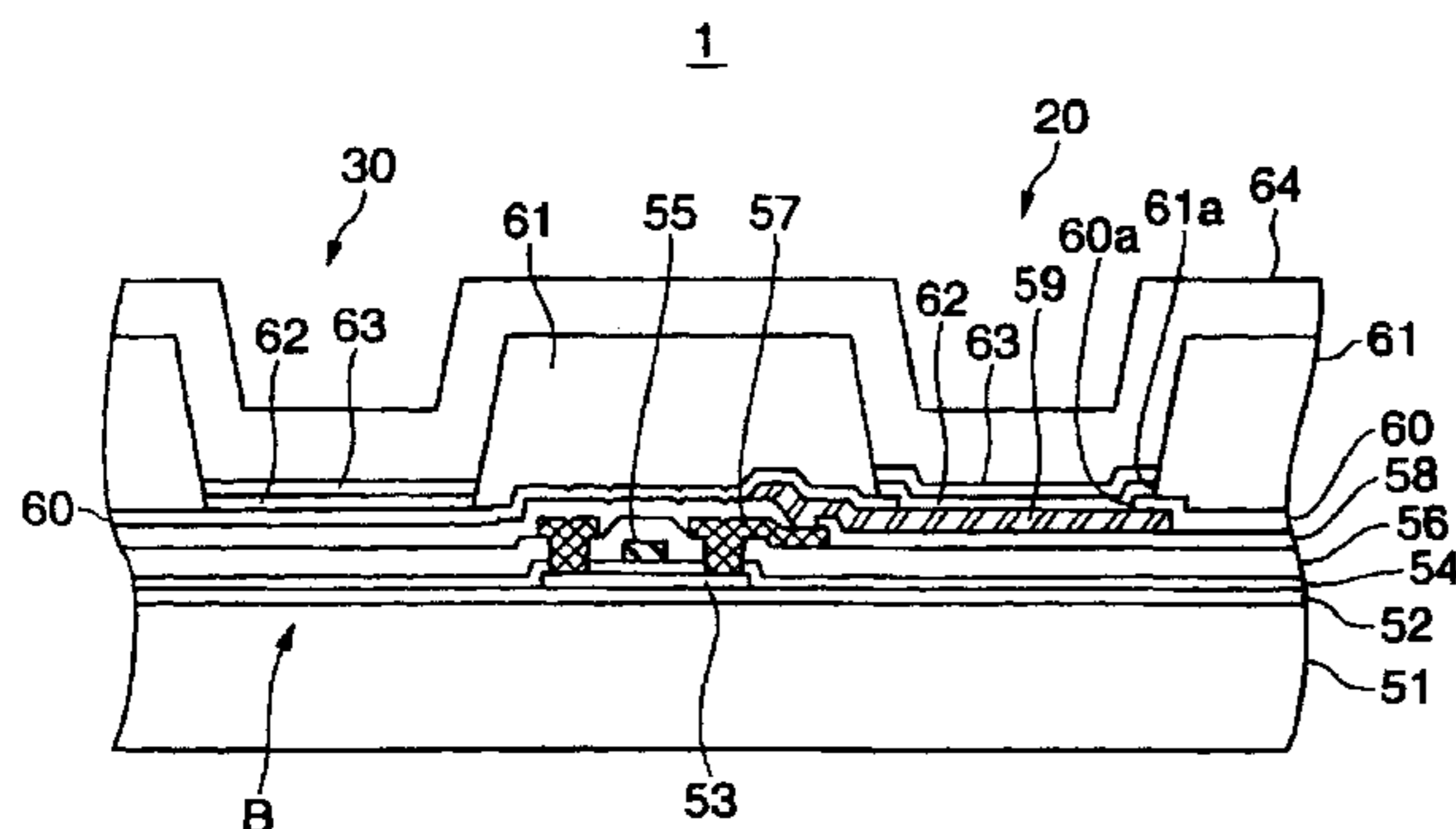
Cross sectional view along X-Y direction
