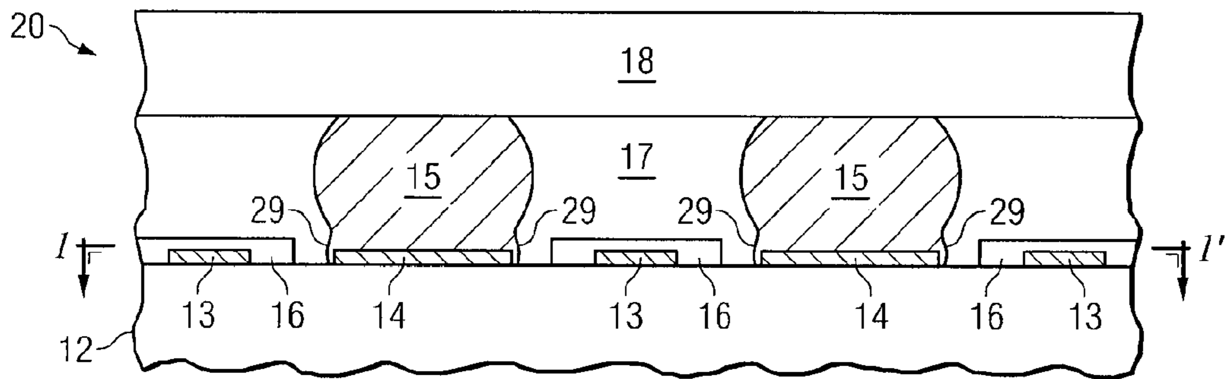
FIG. 2 (PRIOR ART)
