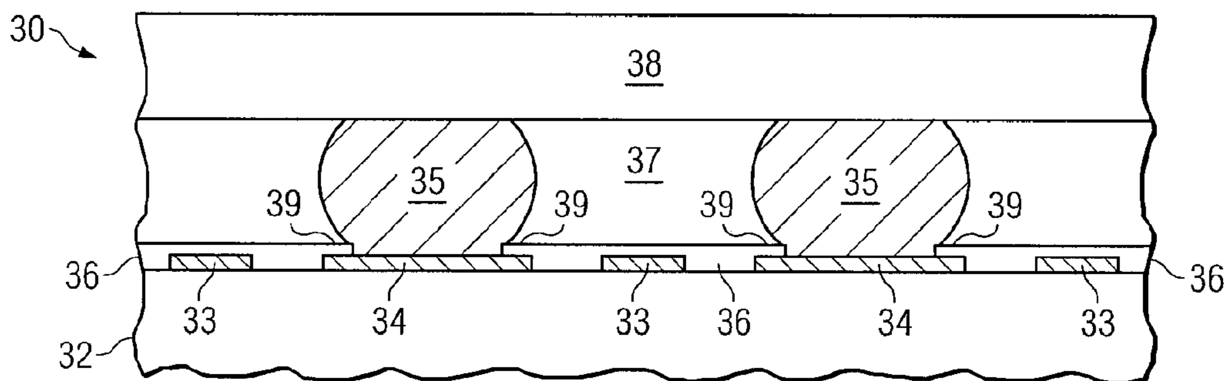
FIG. 3 (PRIOR ART)
