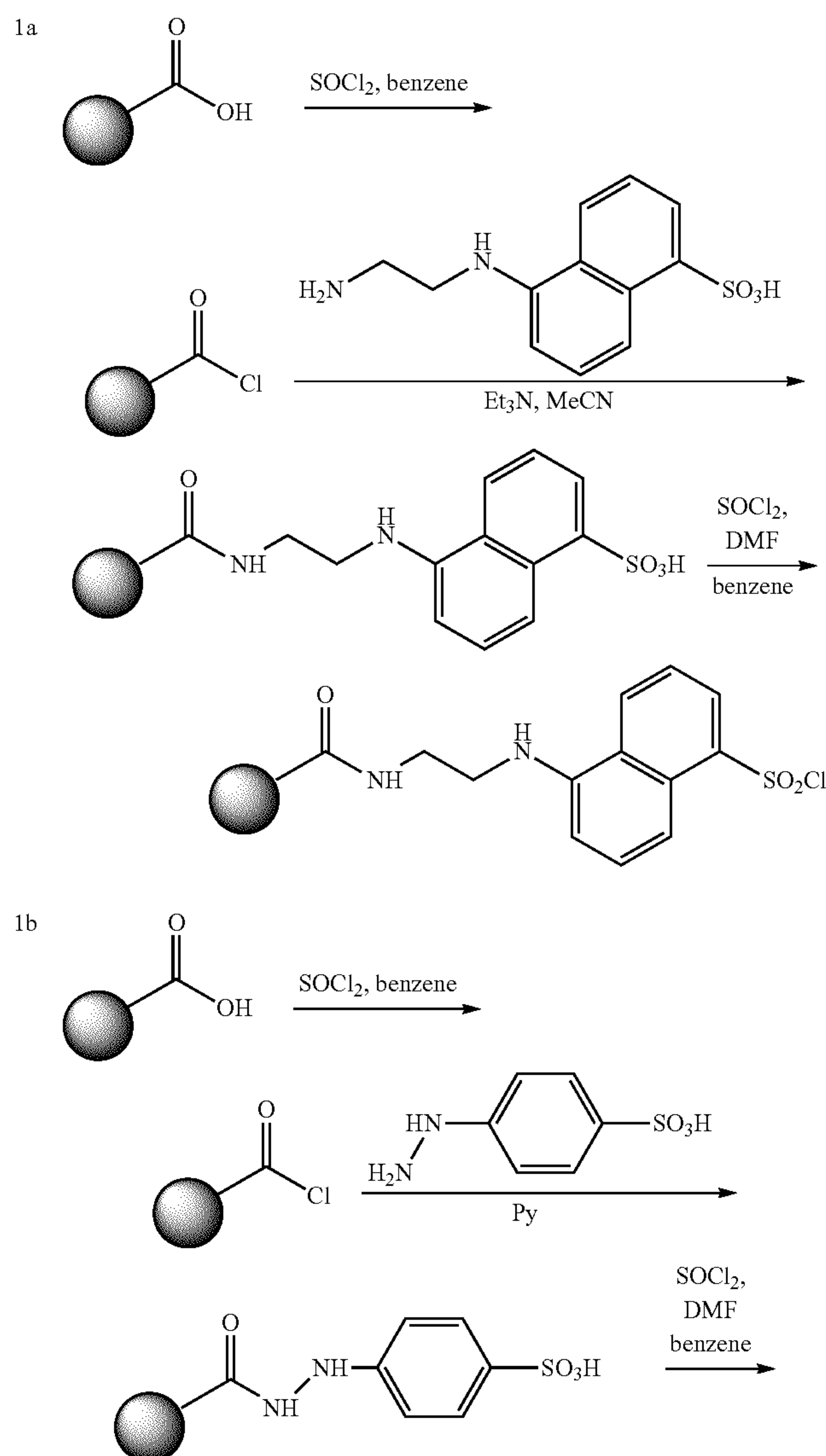
Summary of Functional Groups and Synthetic Routes to Functionalized Microspheres
