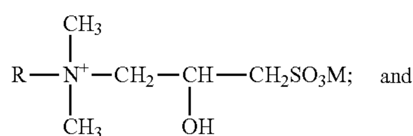
Alkyl sultaines
