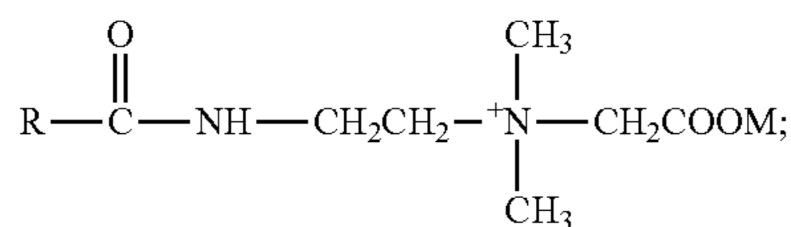
Amidopropyl betaines
