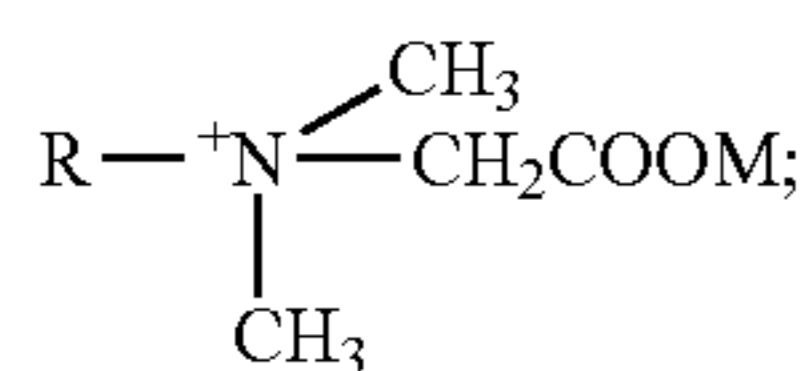
Alkyl betaines
