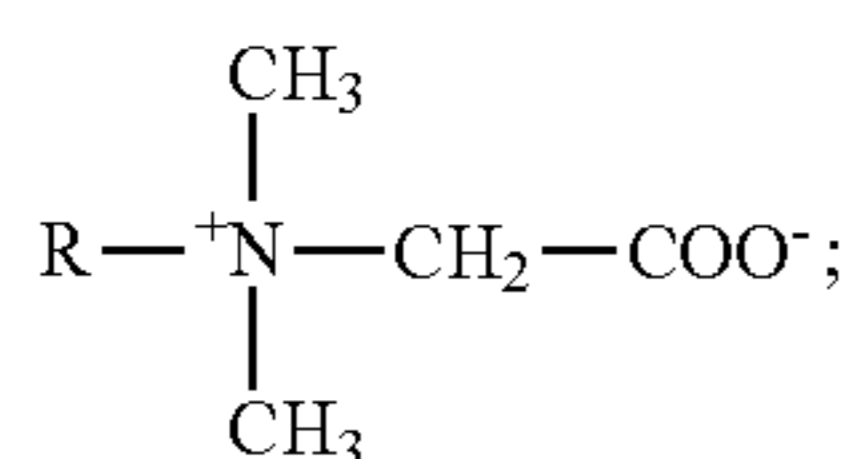
Alkyl betaines
