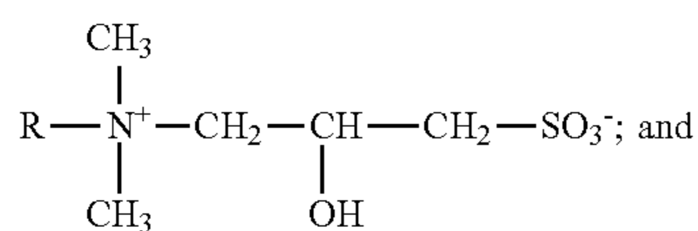
Alkyl sultaines
