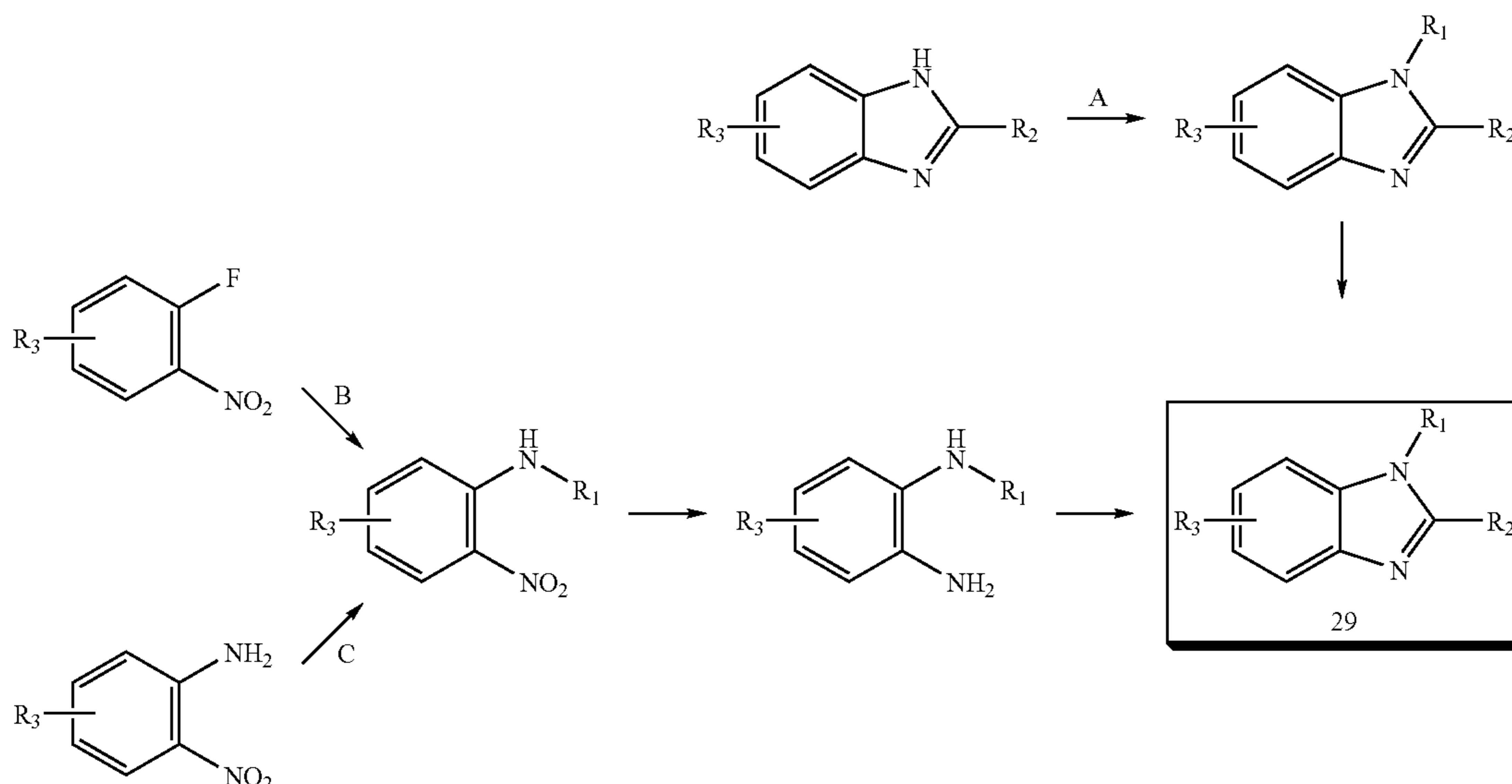
Scheme 2: Synthesis of benzimidazole analogs
