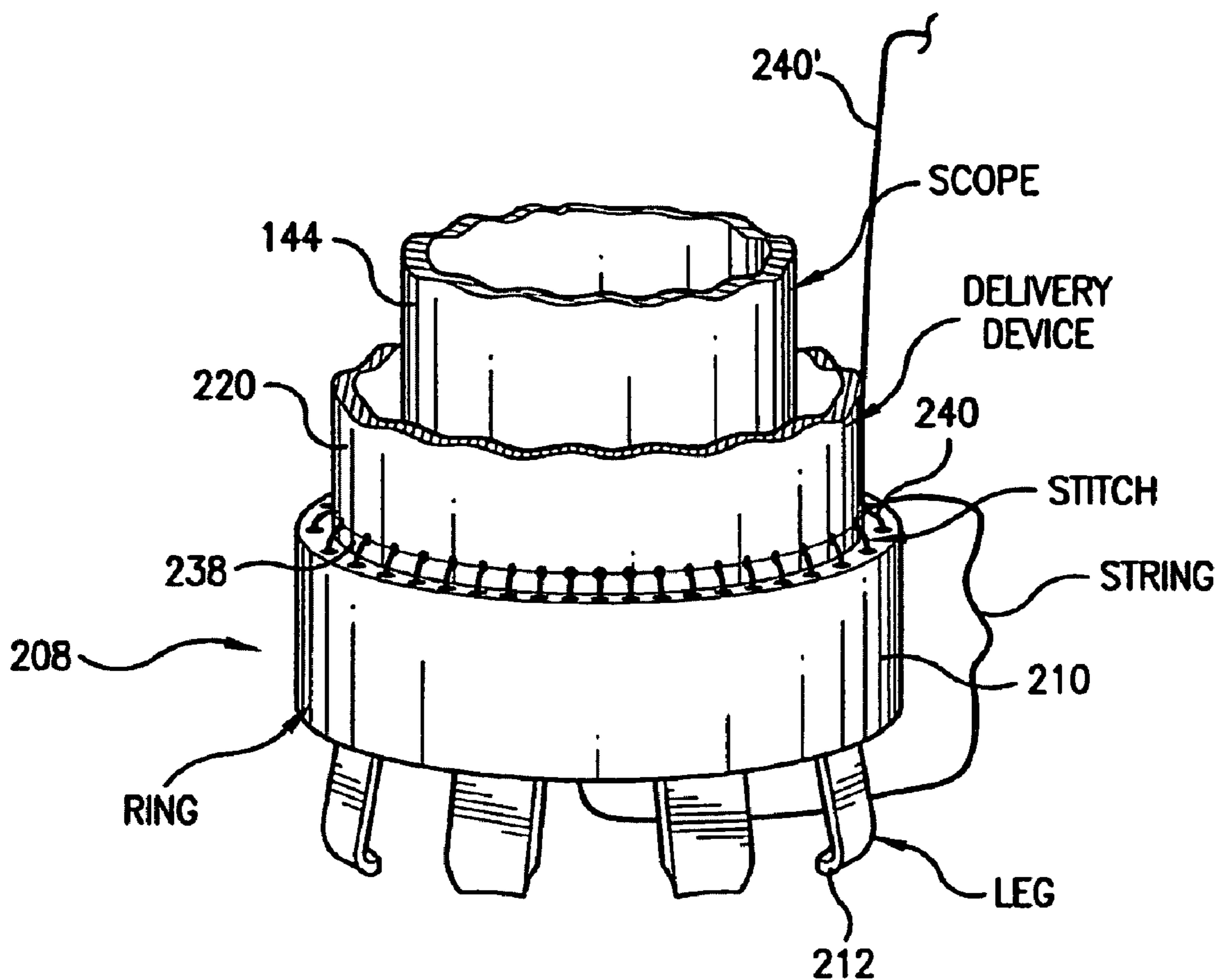
STITCH DISENGAGEMENT FIG. 60
