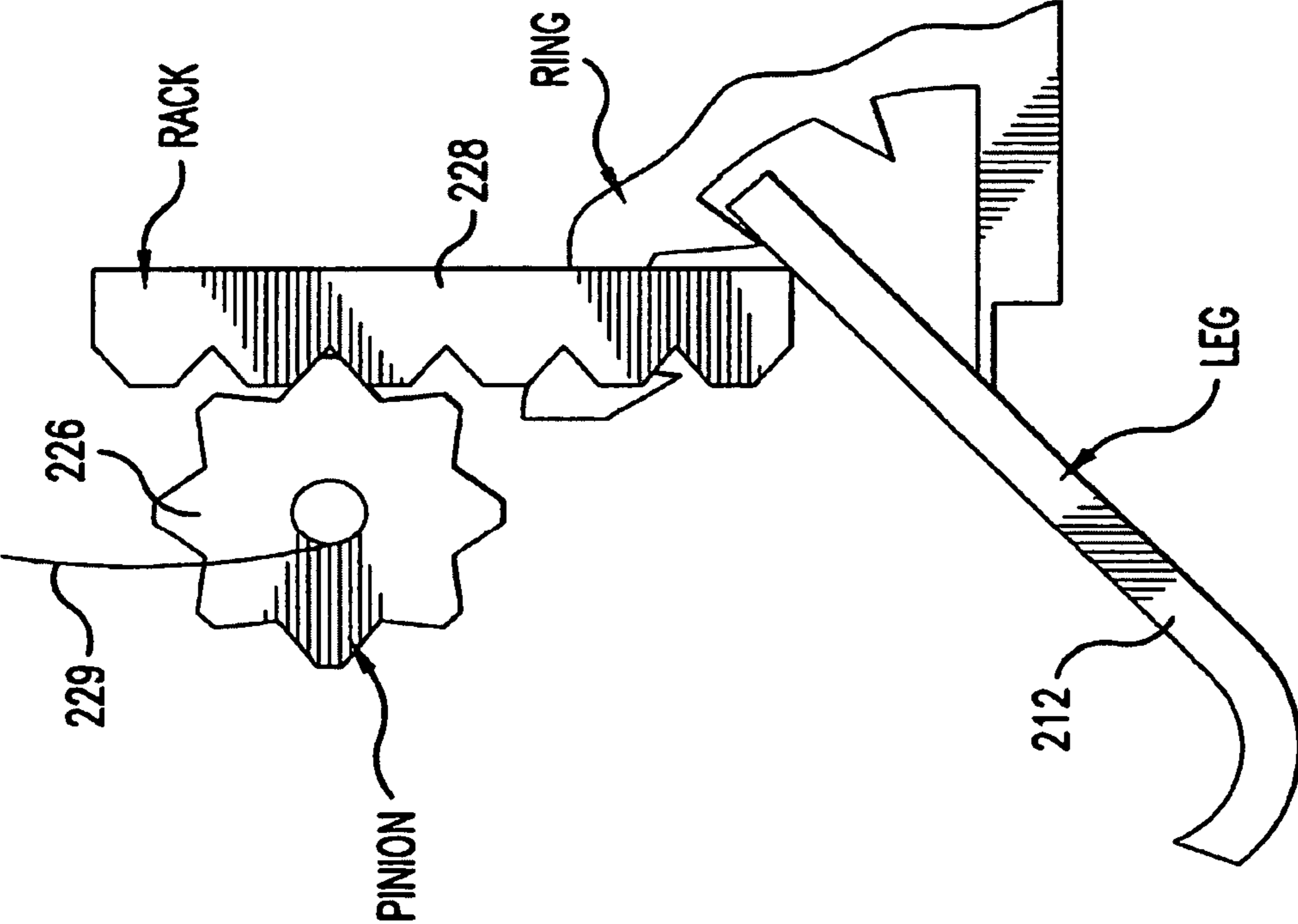
RACK & PINION DEPLOYMENT FIG. 56
