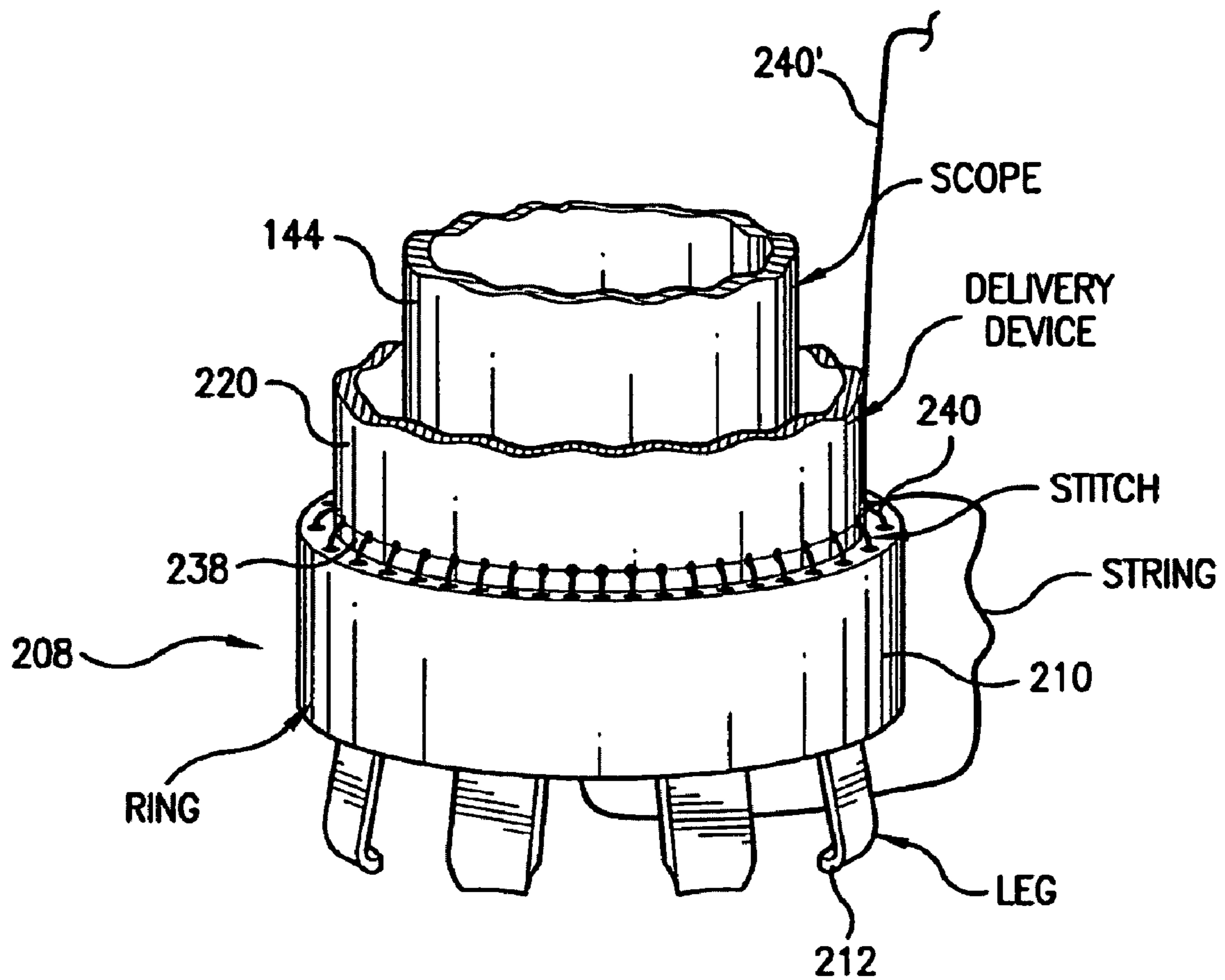
STITCH DISENGAGEMENT FIG. 60
