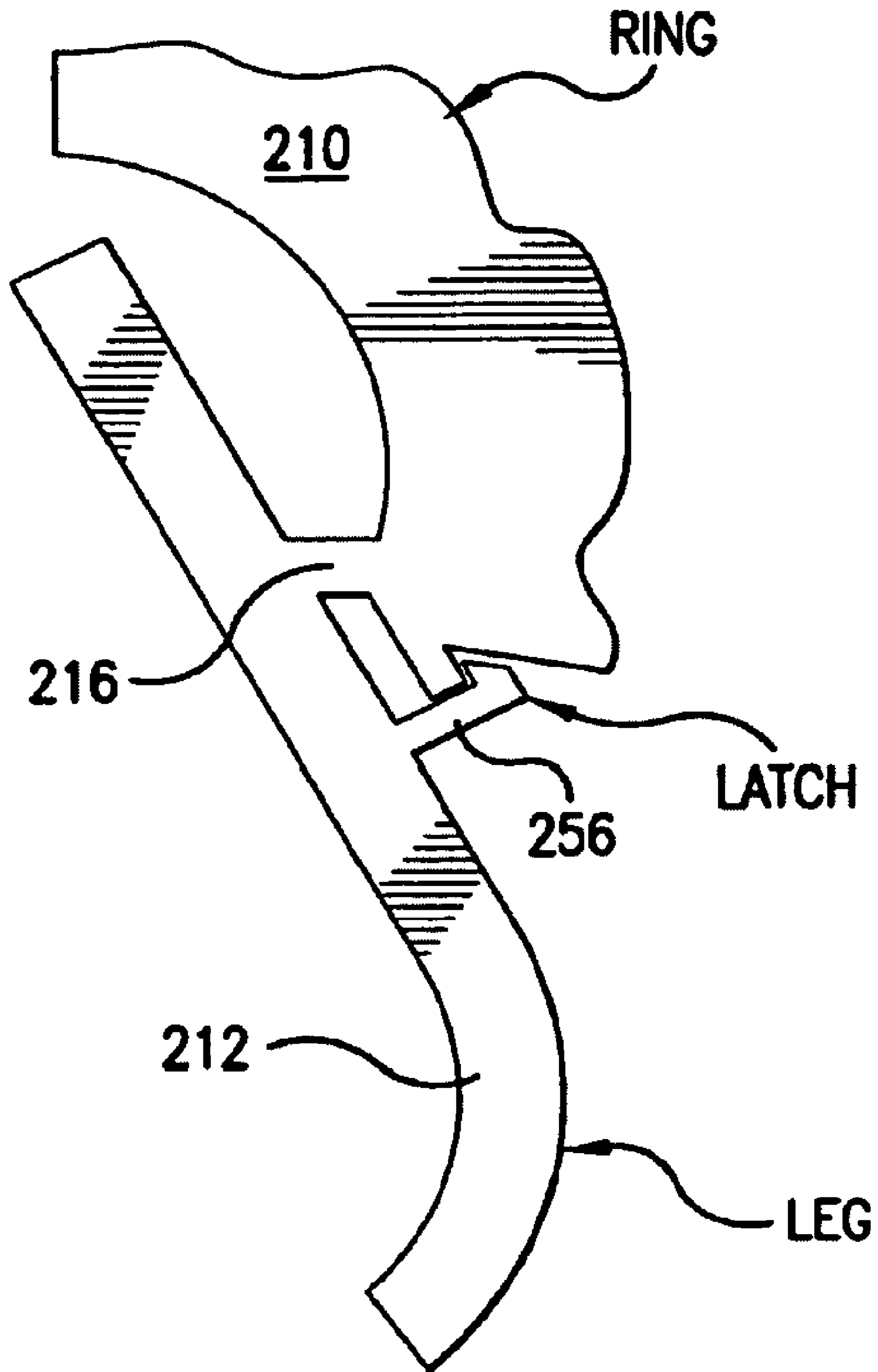
LATCH TO KEEP CLIP OPEN FIG. 68
