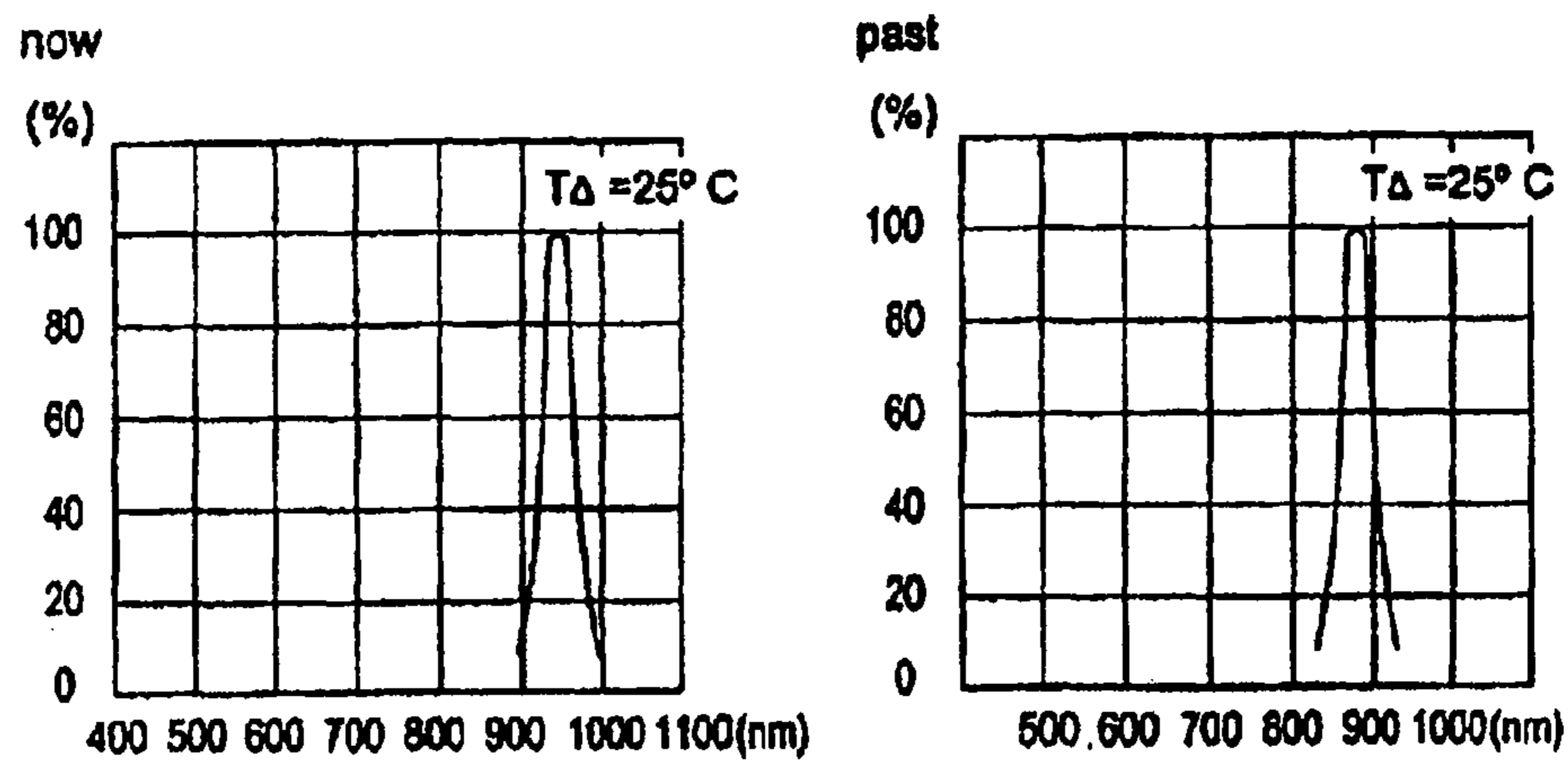
The spectral curve of the LED
