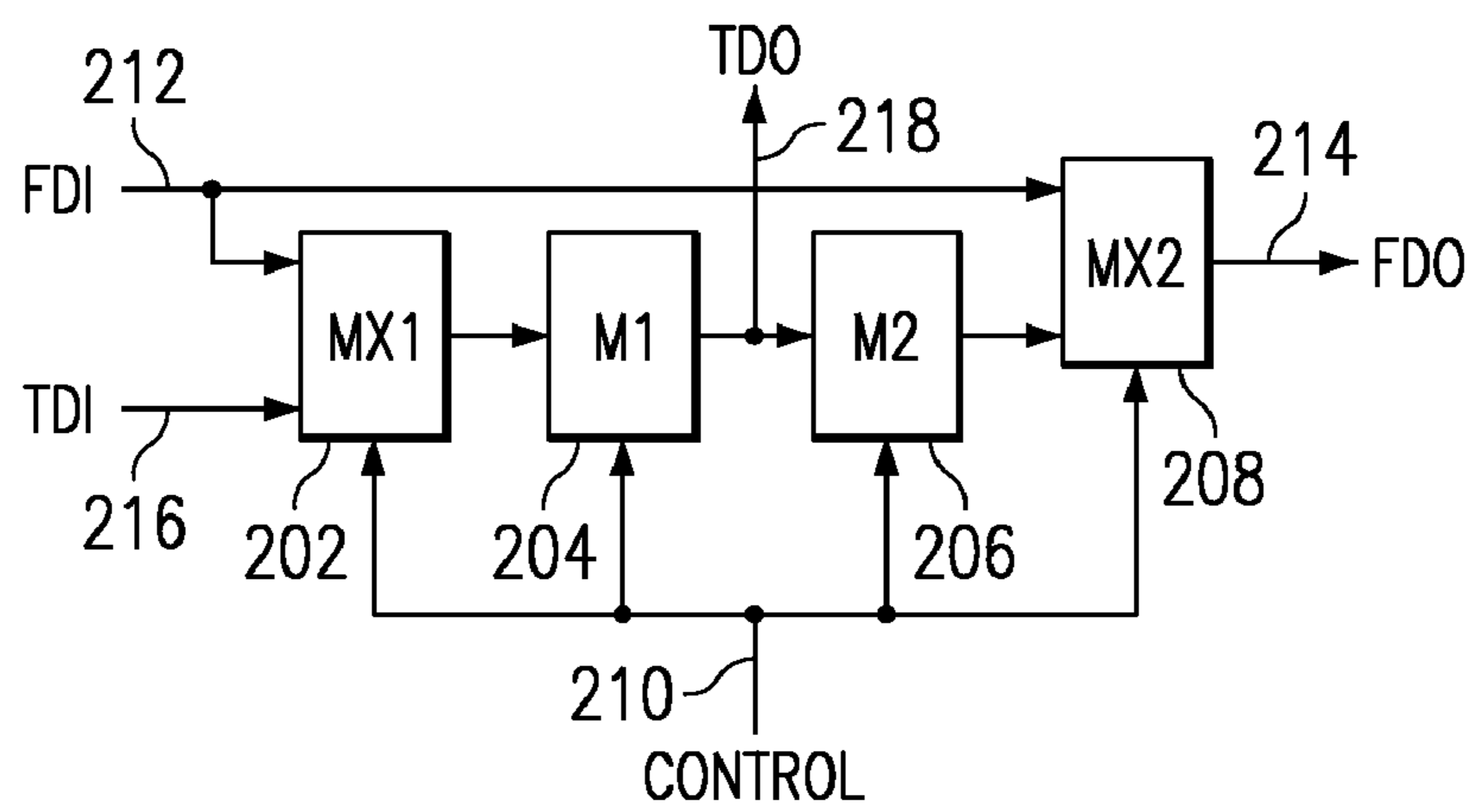
FIG. 2 (PRIOR ART)
