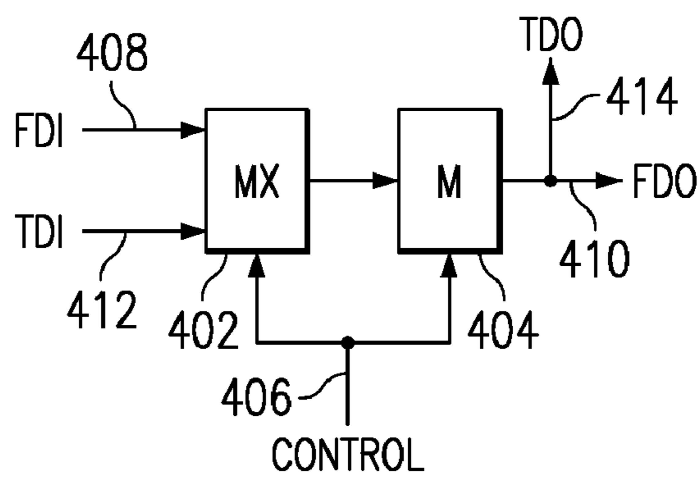
FIG. 4 (PRIOR ART)
