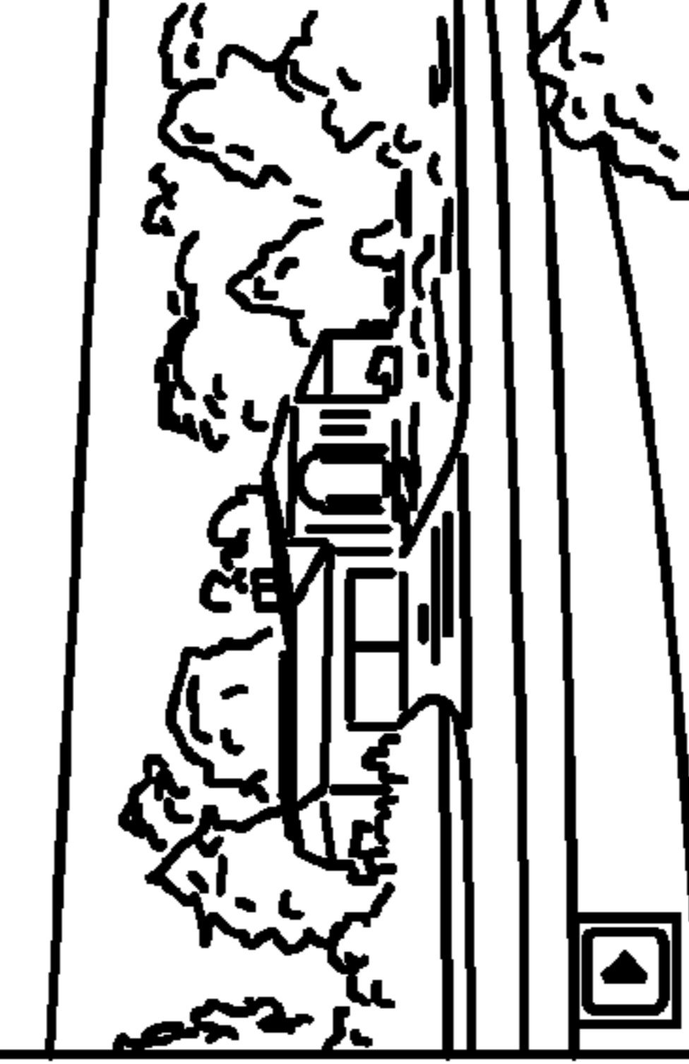
Hurricane Wilma: October 2005
