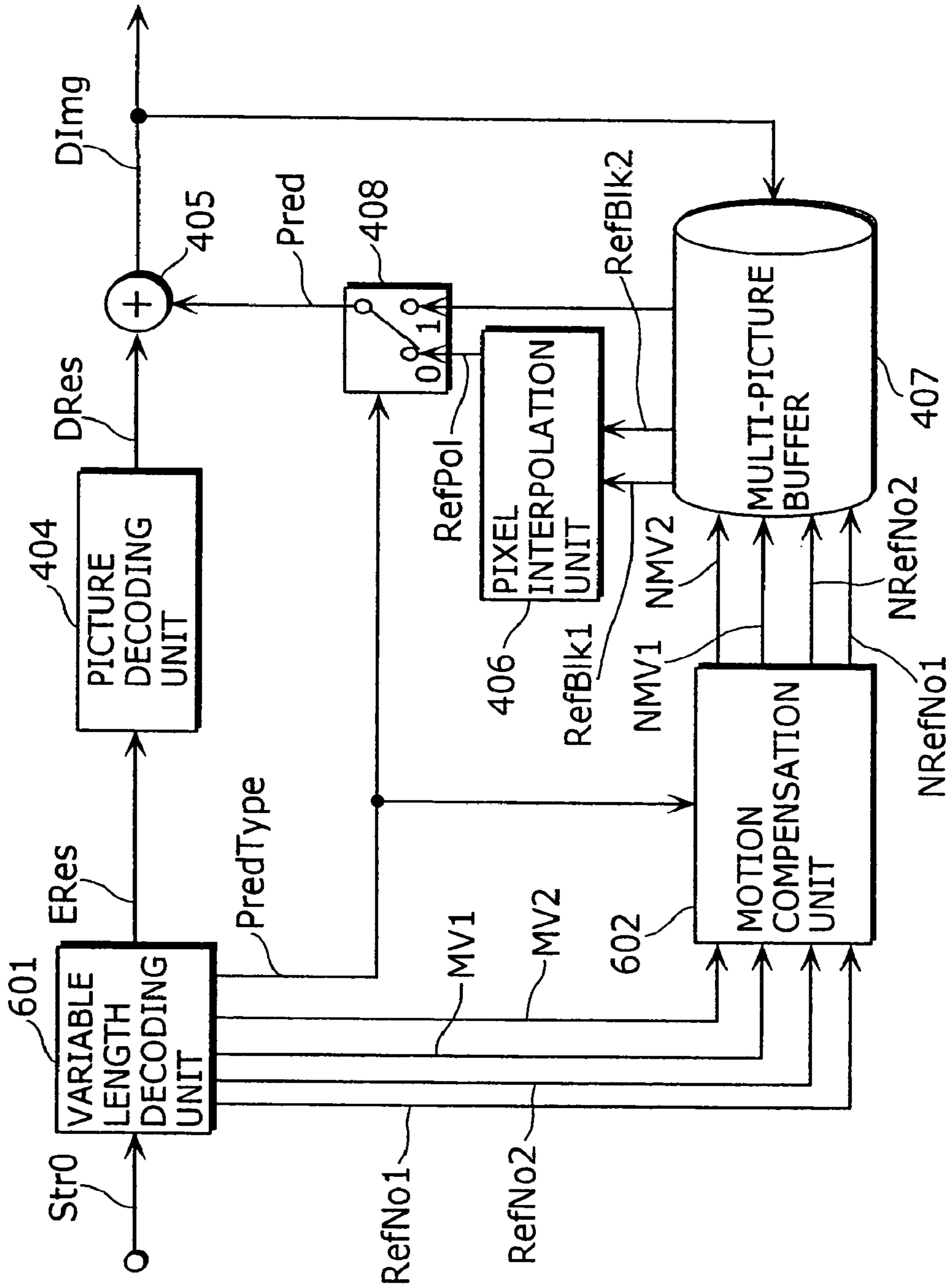
FIG. 4 PRIOR ART
