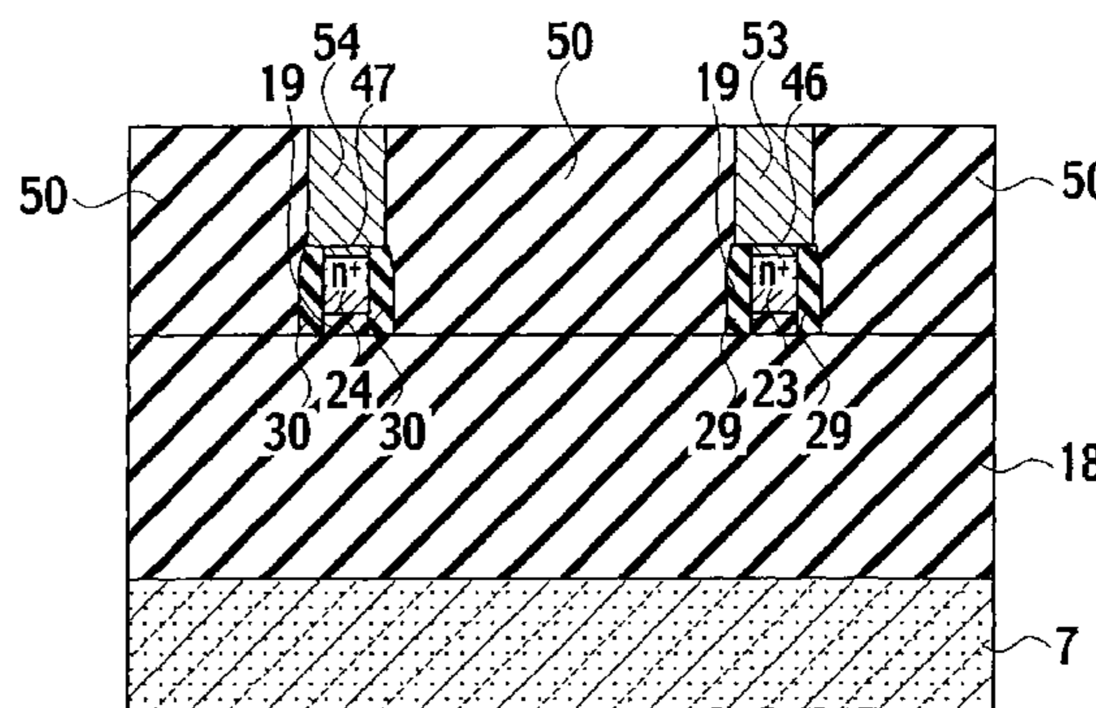
[HIGH-VOLTAGE CIRCUIT REGION]
