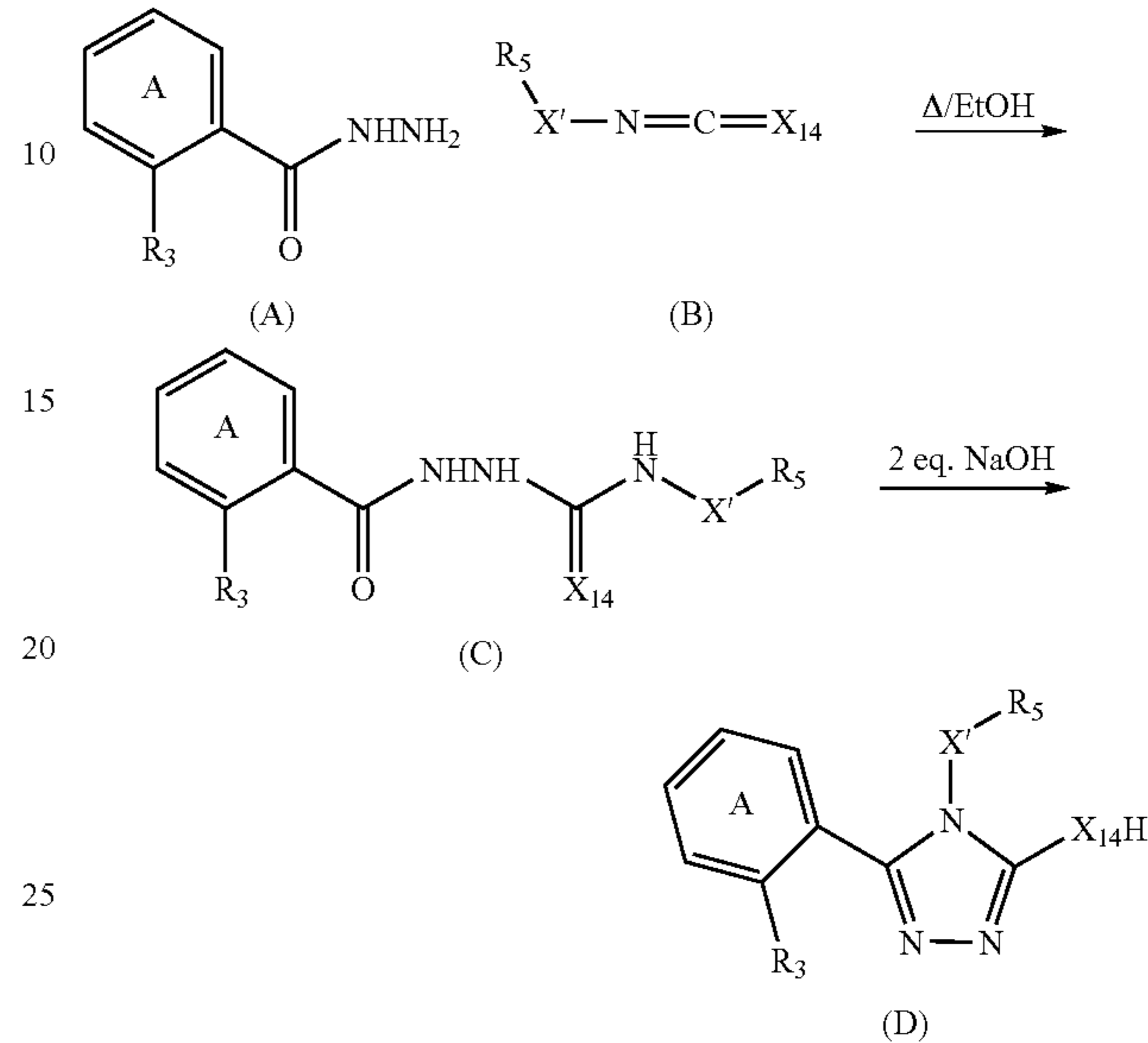
Scheme I: Synthesis of triazole compounds of the invention
