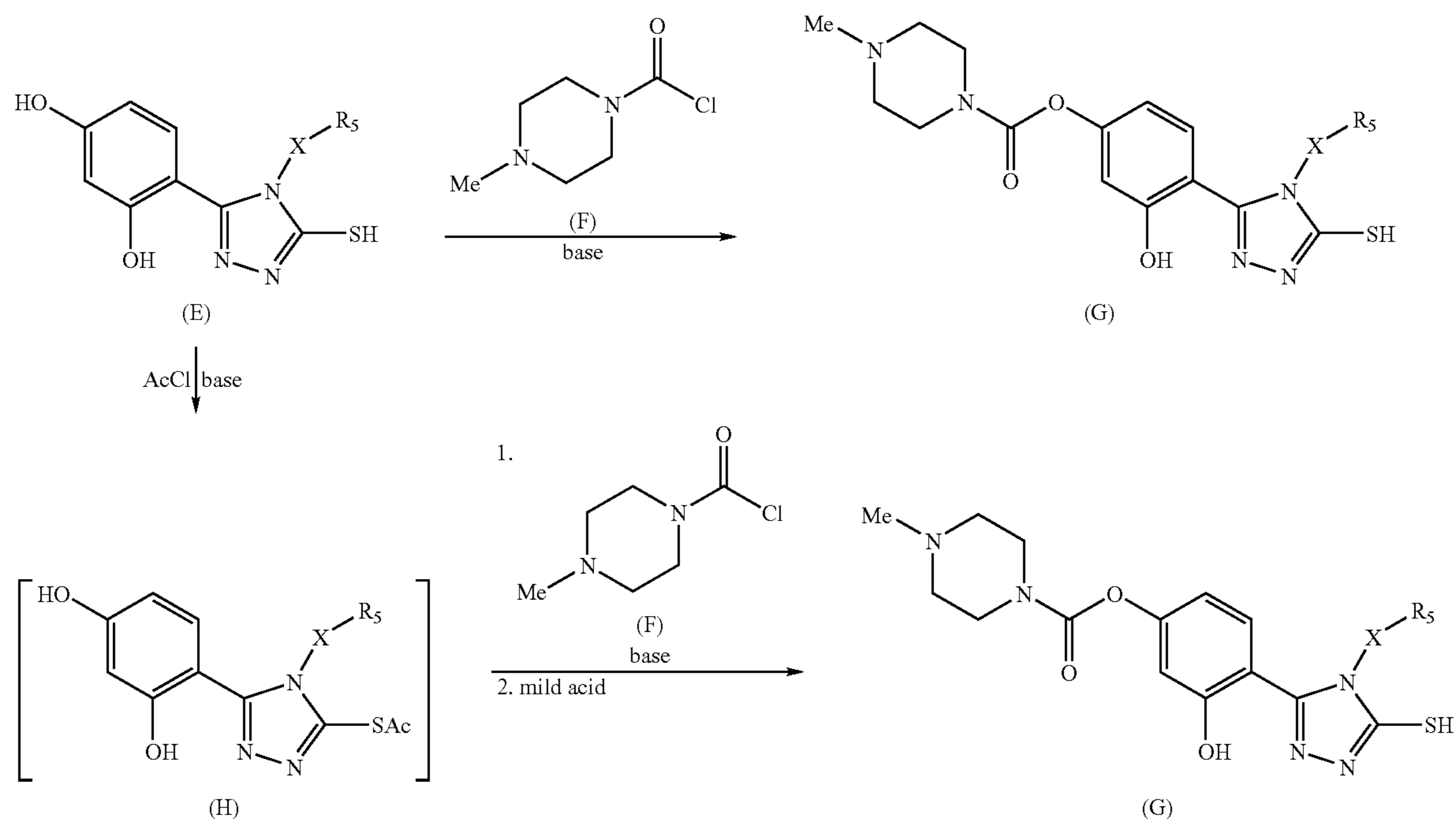
Scheme VIII: Preparation of prodrugs in which the 4-hydroxy group of compounds of the invention is protected with 4-methyl-piperazine-1-carbamoyl.
