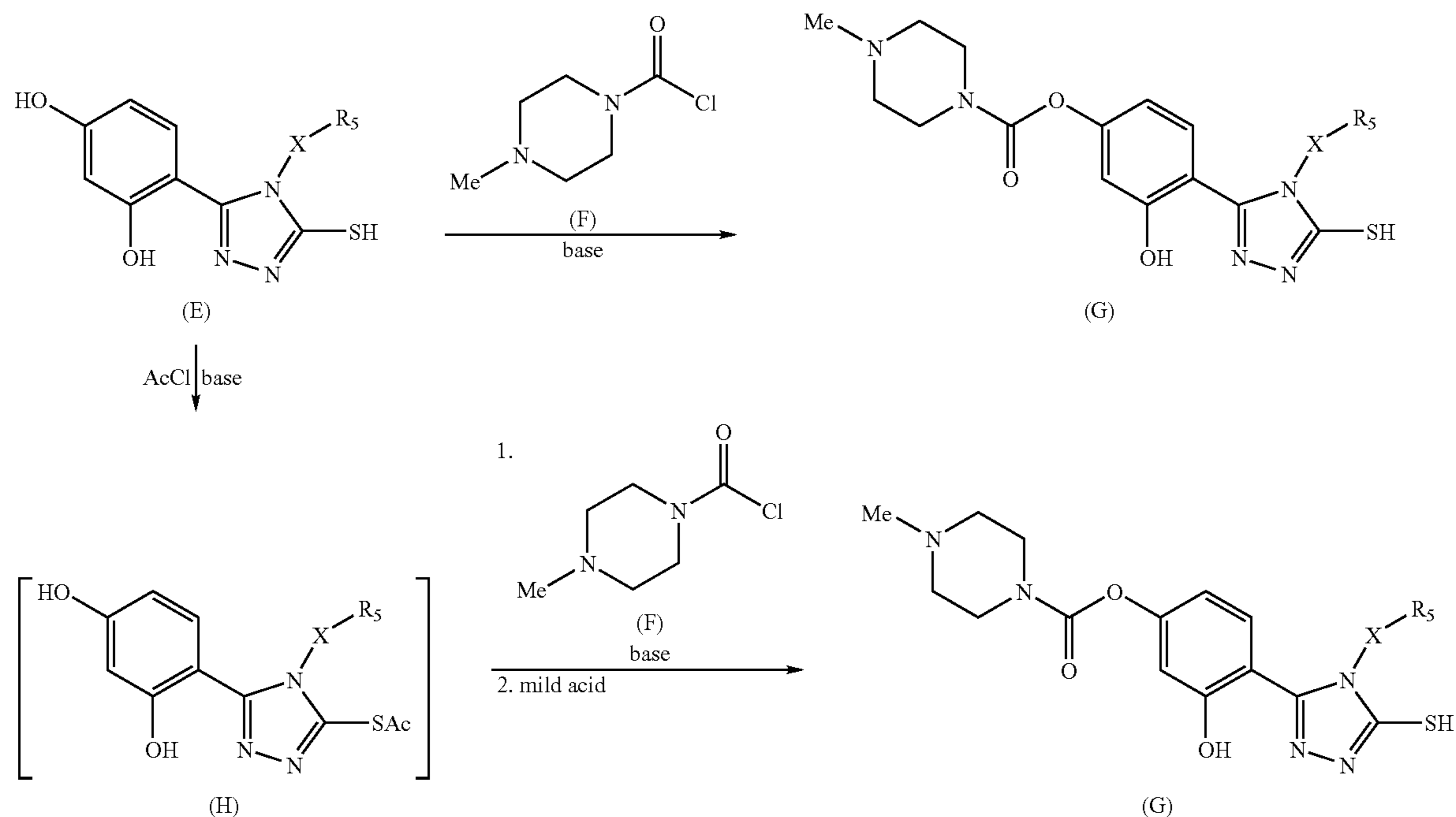
Scheme VIII: Preparation of prodrugs in which the 4-hydroxy group of compounds of the invention is protected with 4-methyl-piperazine-1-carbamoyl.
