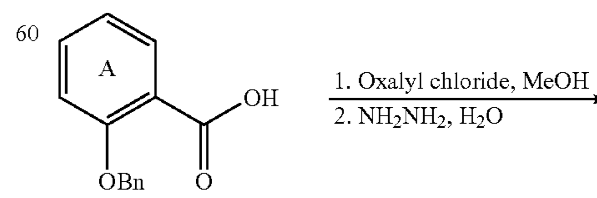
Scheme VI: Synthesis of triazole compounds of the invention wherein X is NR 7
