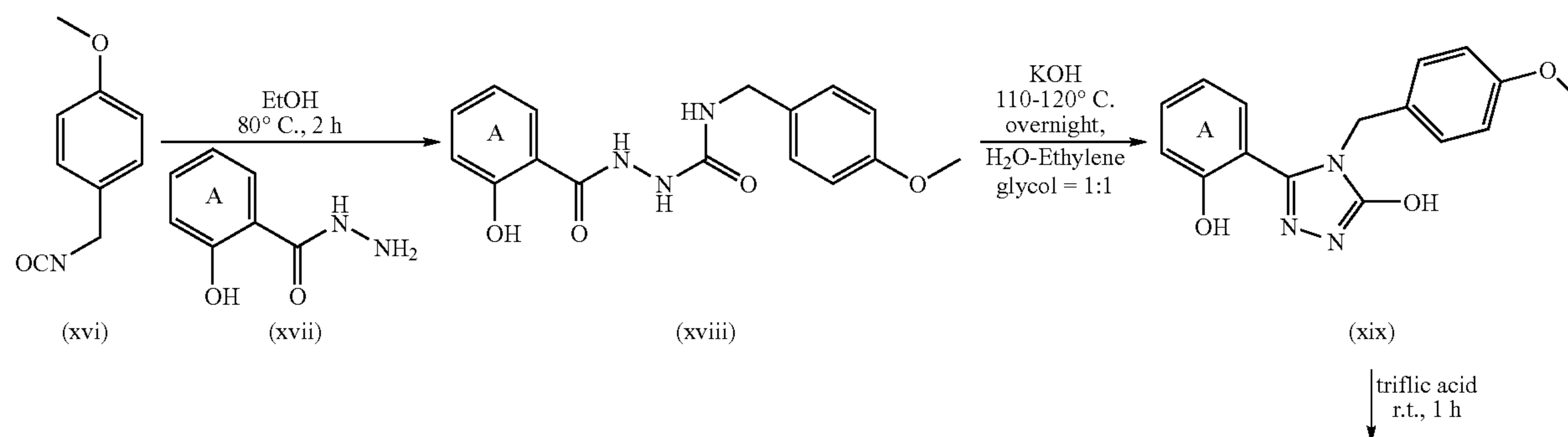
Scheme IV: Synthesis of triazole compounds of the invention wherein X is C(O)
