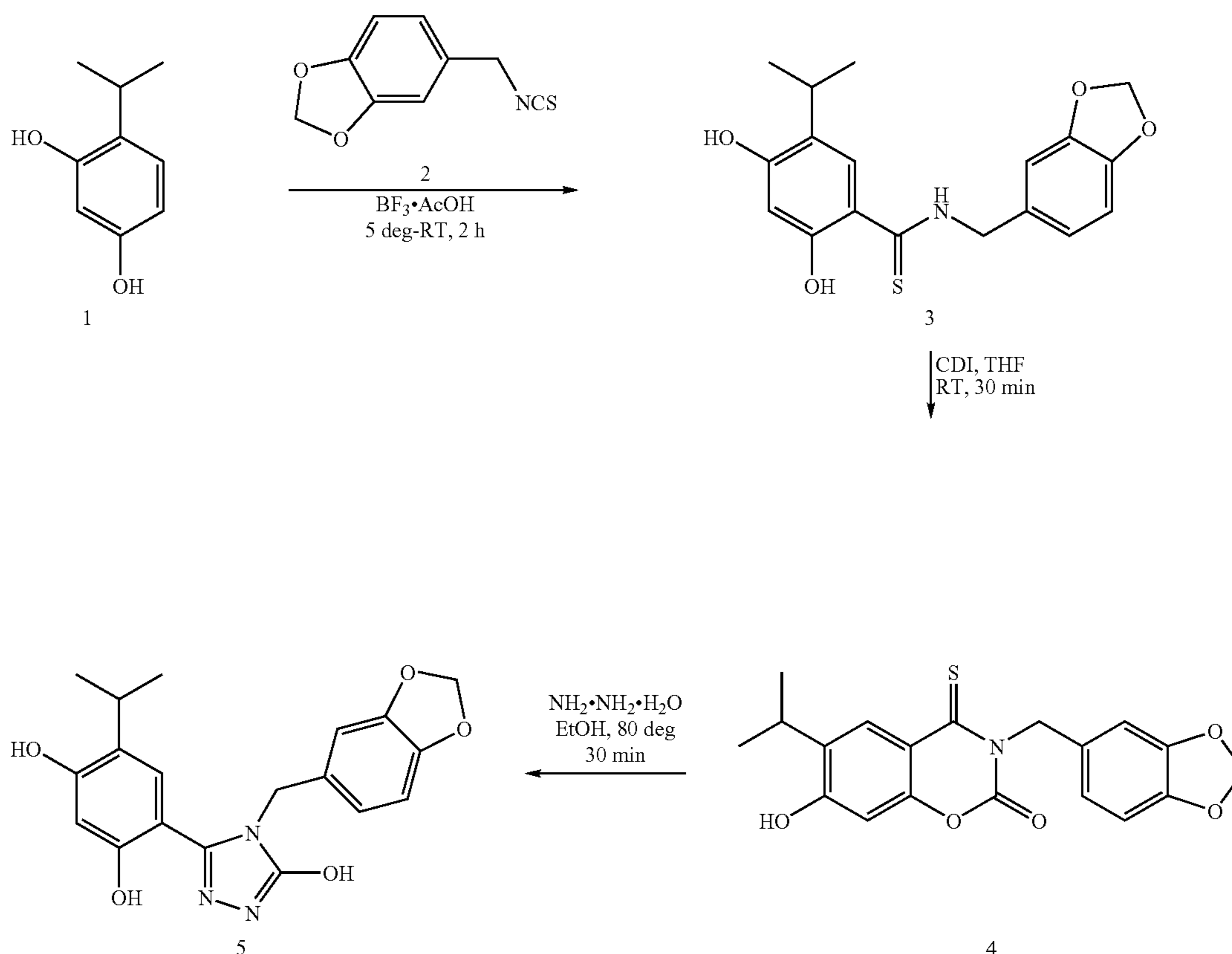
Scheme VII: Alternate Synthesis of Triazole Compounds of the Invention
