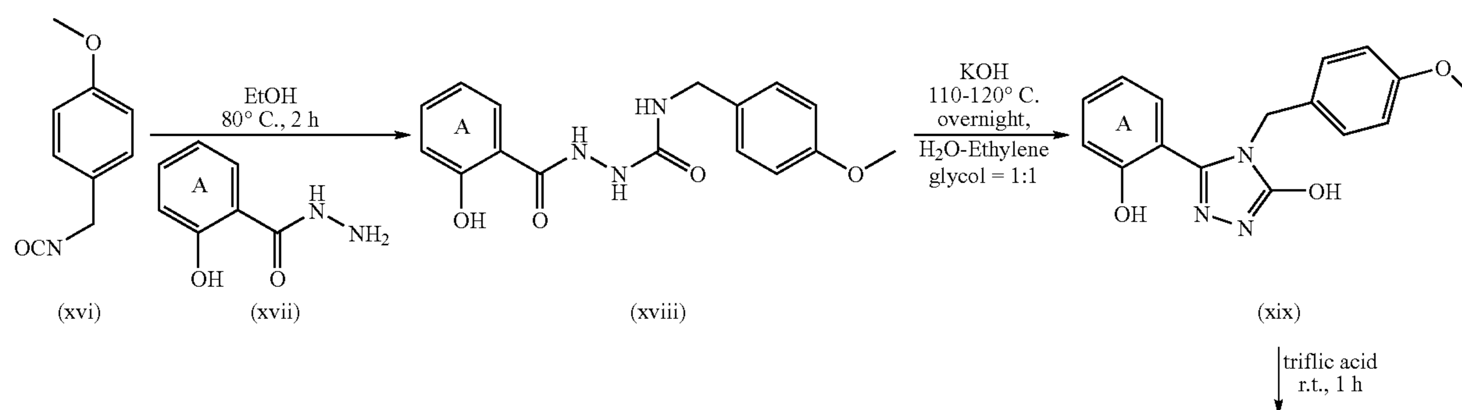
Scheme IV: Synthesis of triazole compounds of the invention wherein X is C(O)
