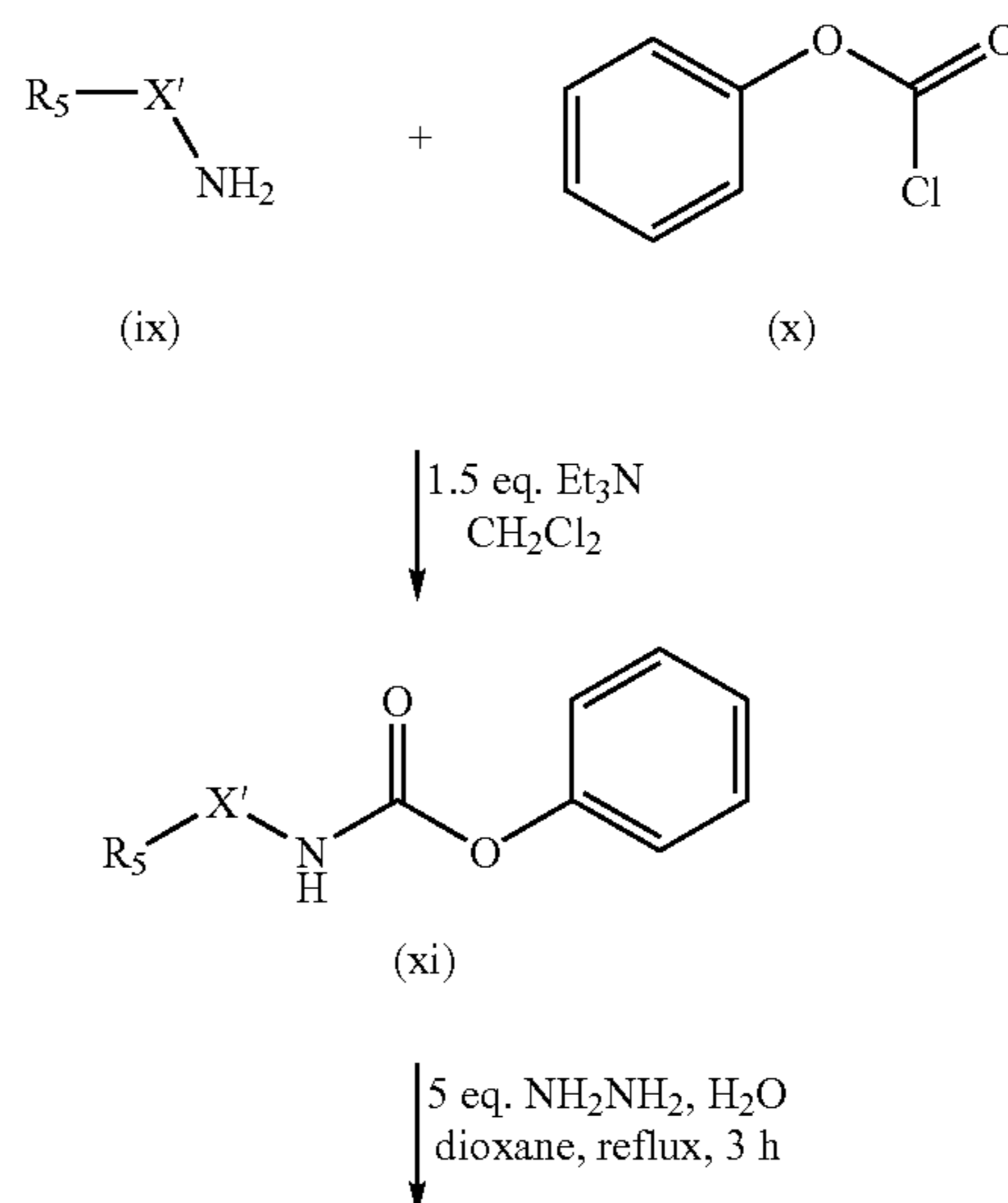
Scheme III: Alternative synthesis of triazole compounds of the invention
