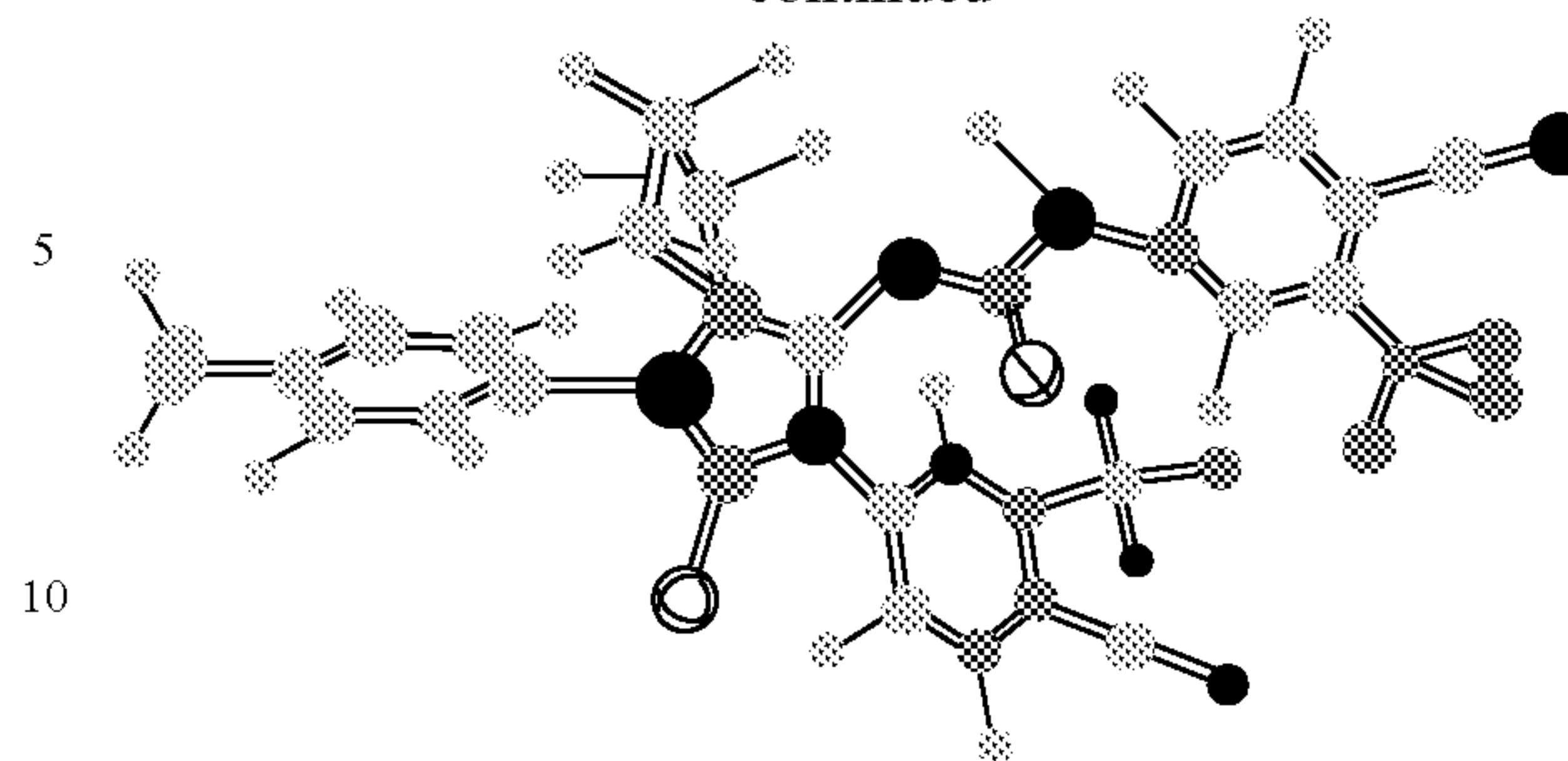
X-ray structure of 35a
