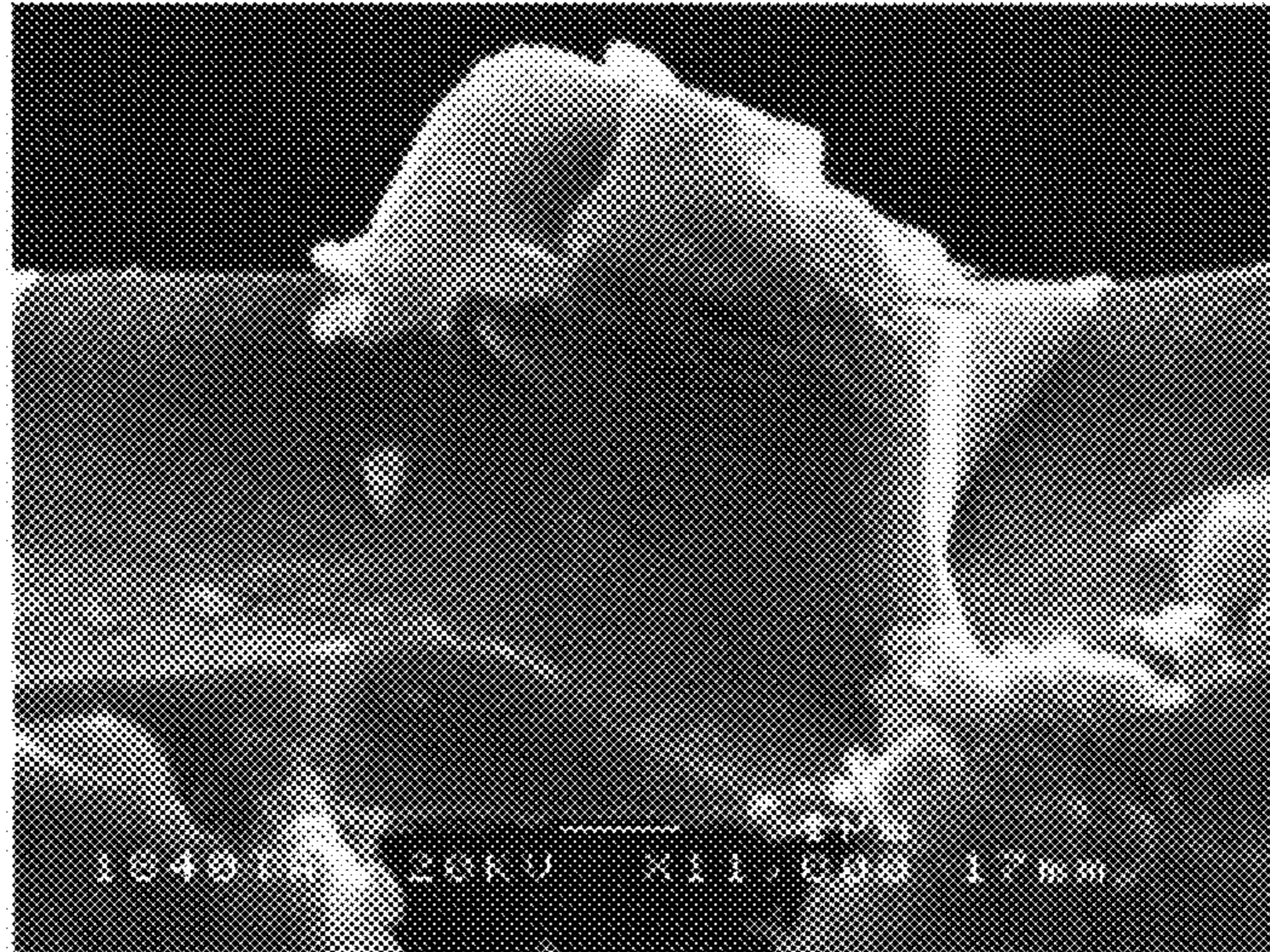
(A) SEM cross-section of void
