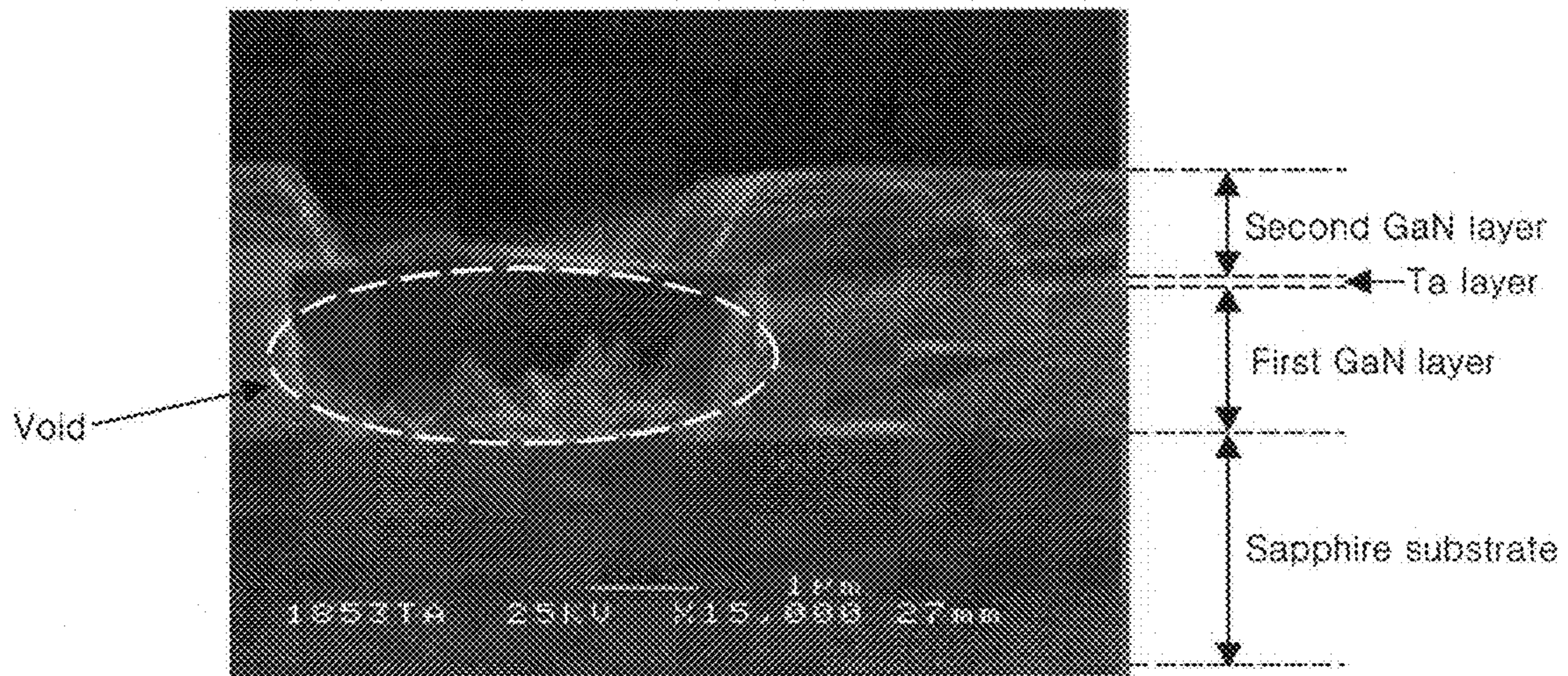
(A) SEM cross-section of substrate
