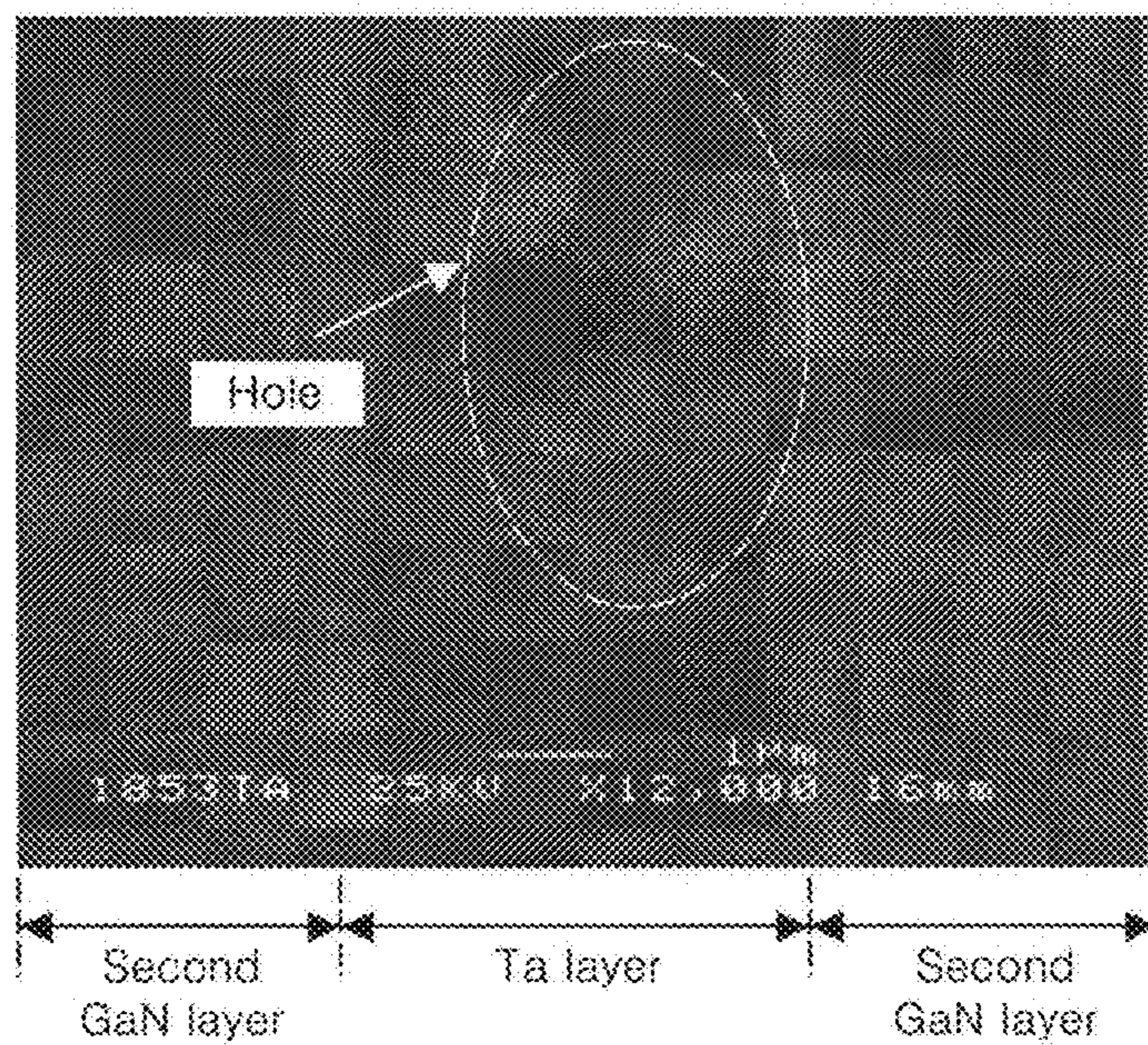
(B) SEM surface photograph of substrate
