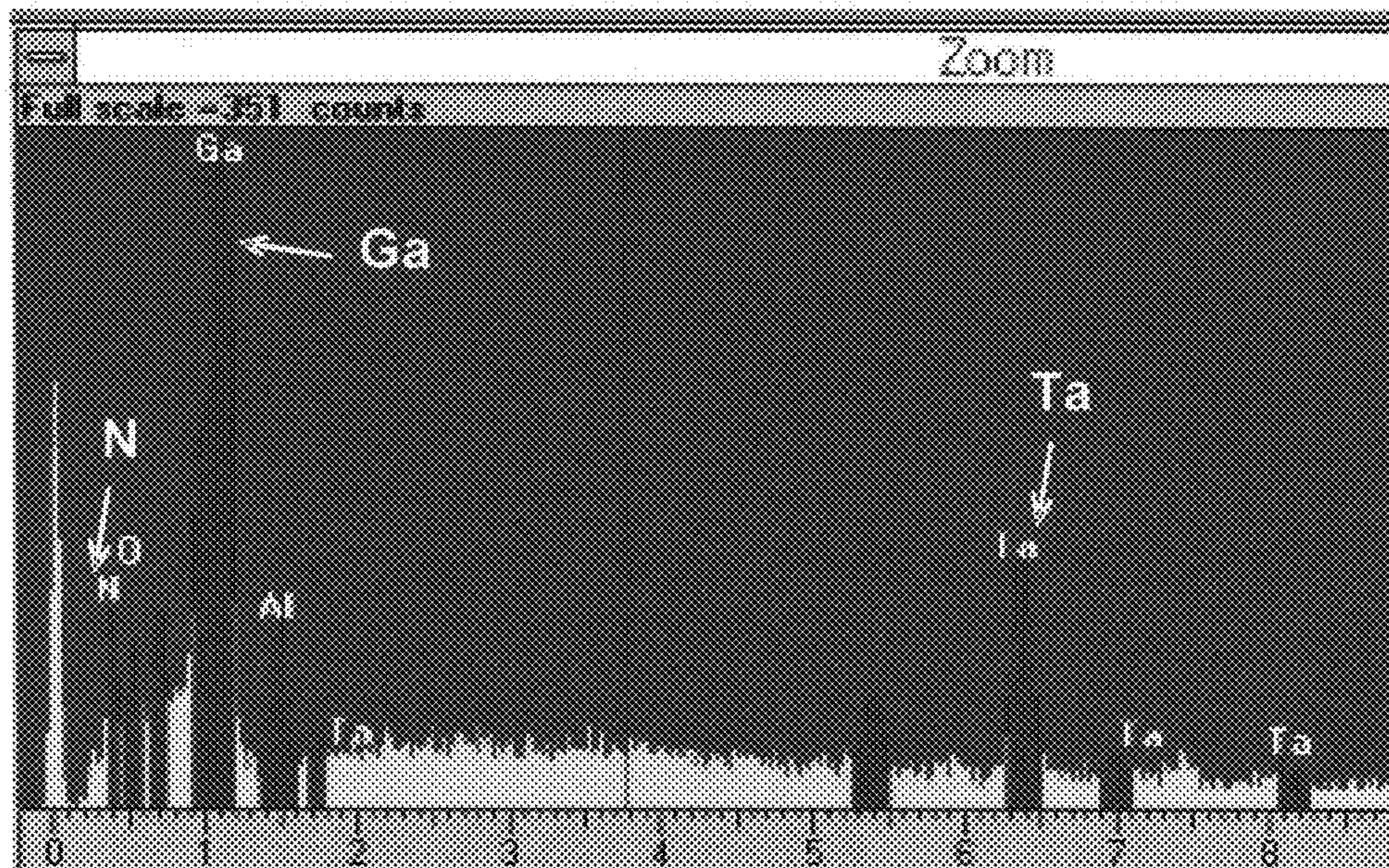
(B) EDX spectrum diagram
