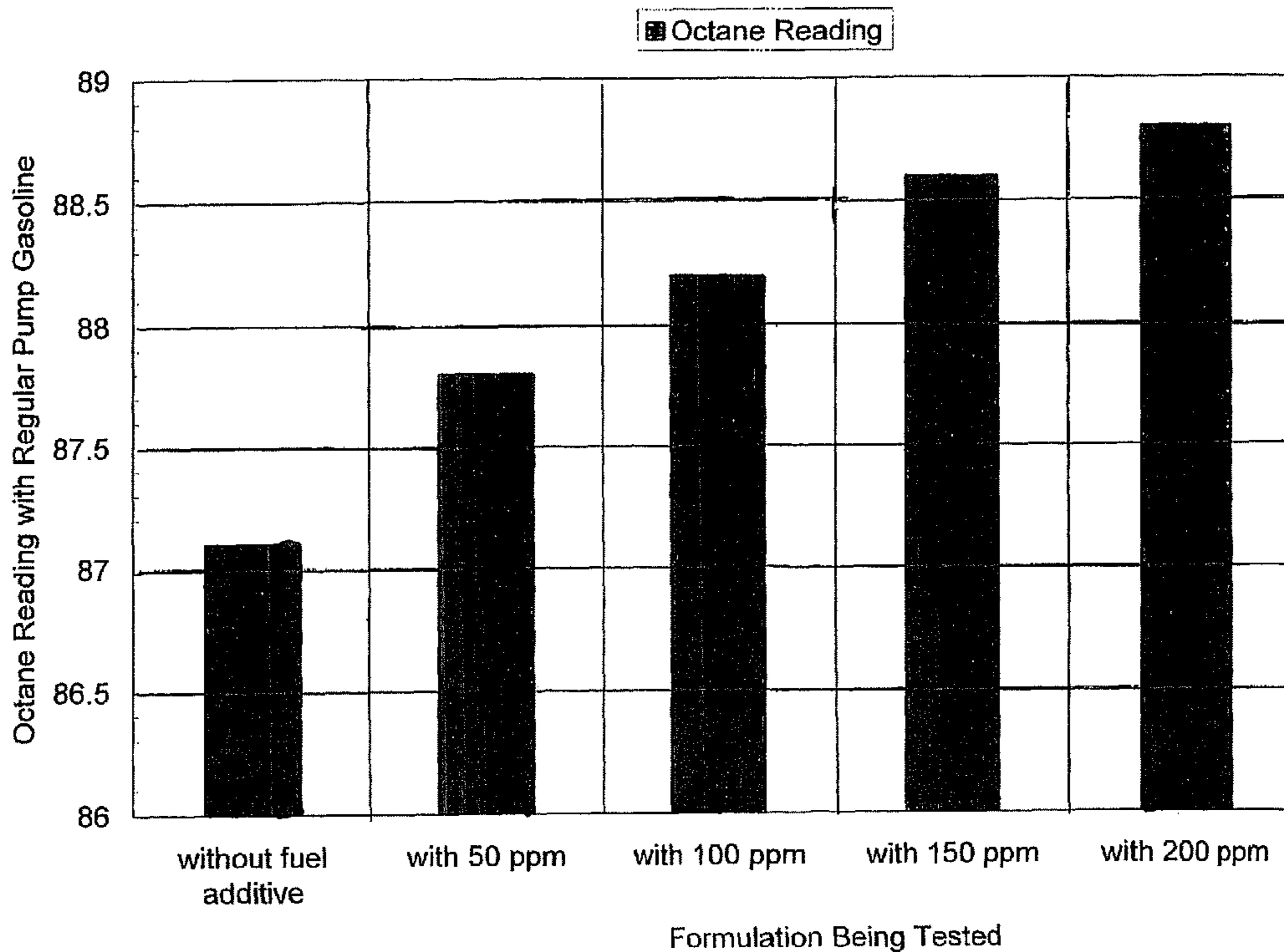
Octane Number Reading With Additive
