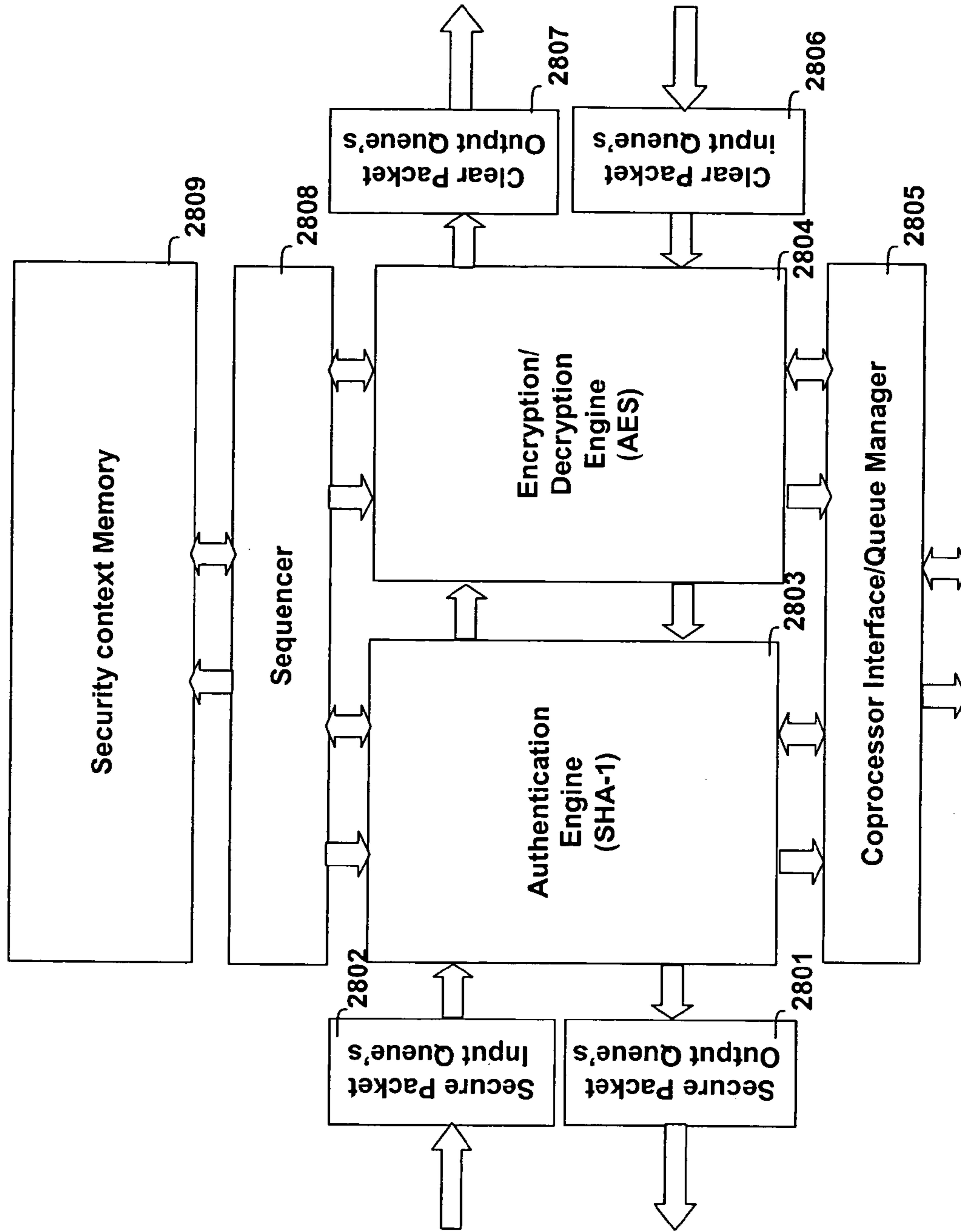
Fig. 28 Security Engine
