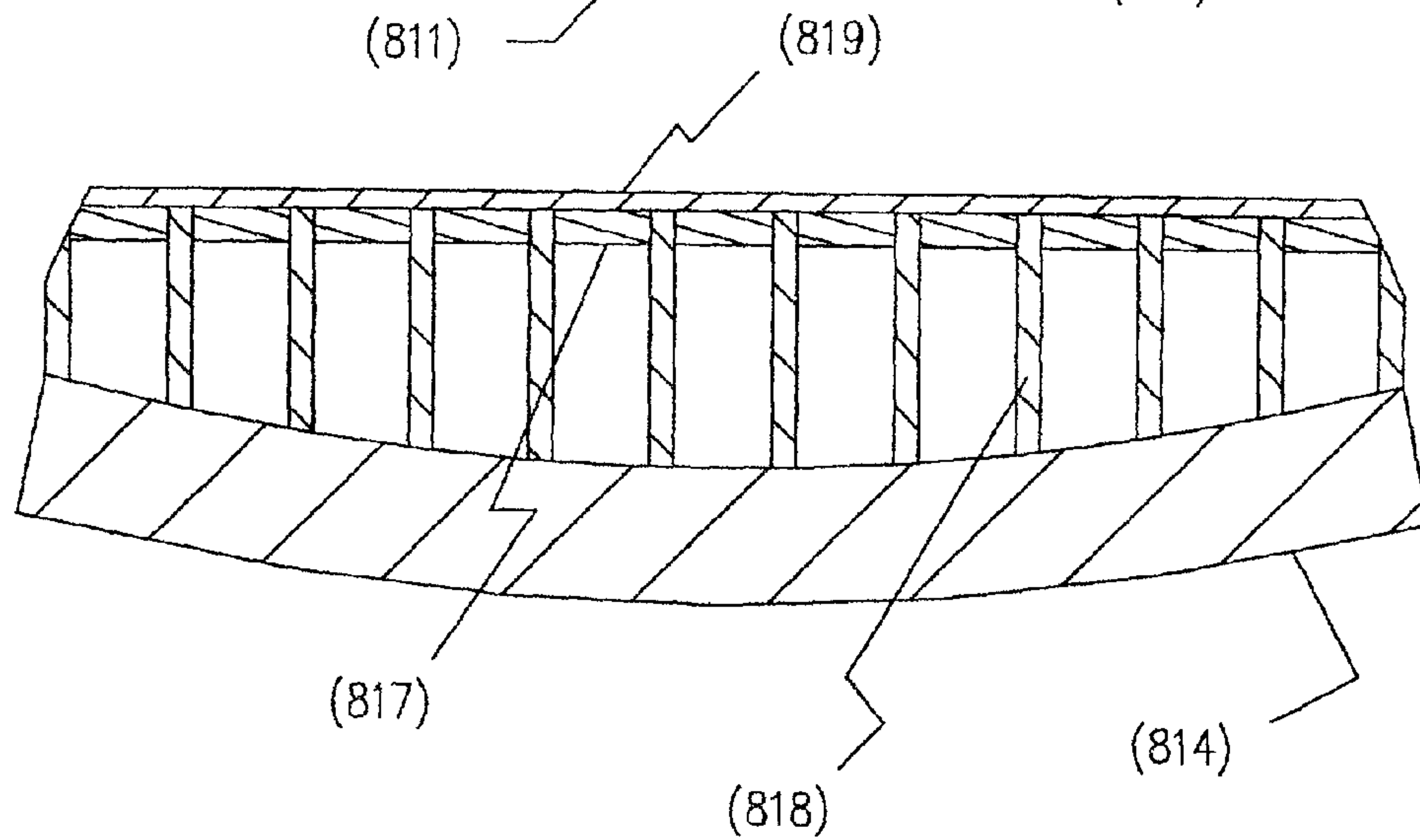
FIGURE 8b EPIRETINAL ELECTRODES - RECESSED
