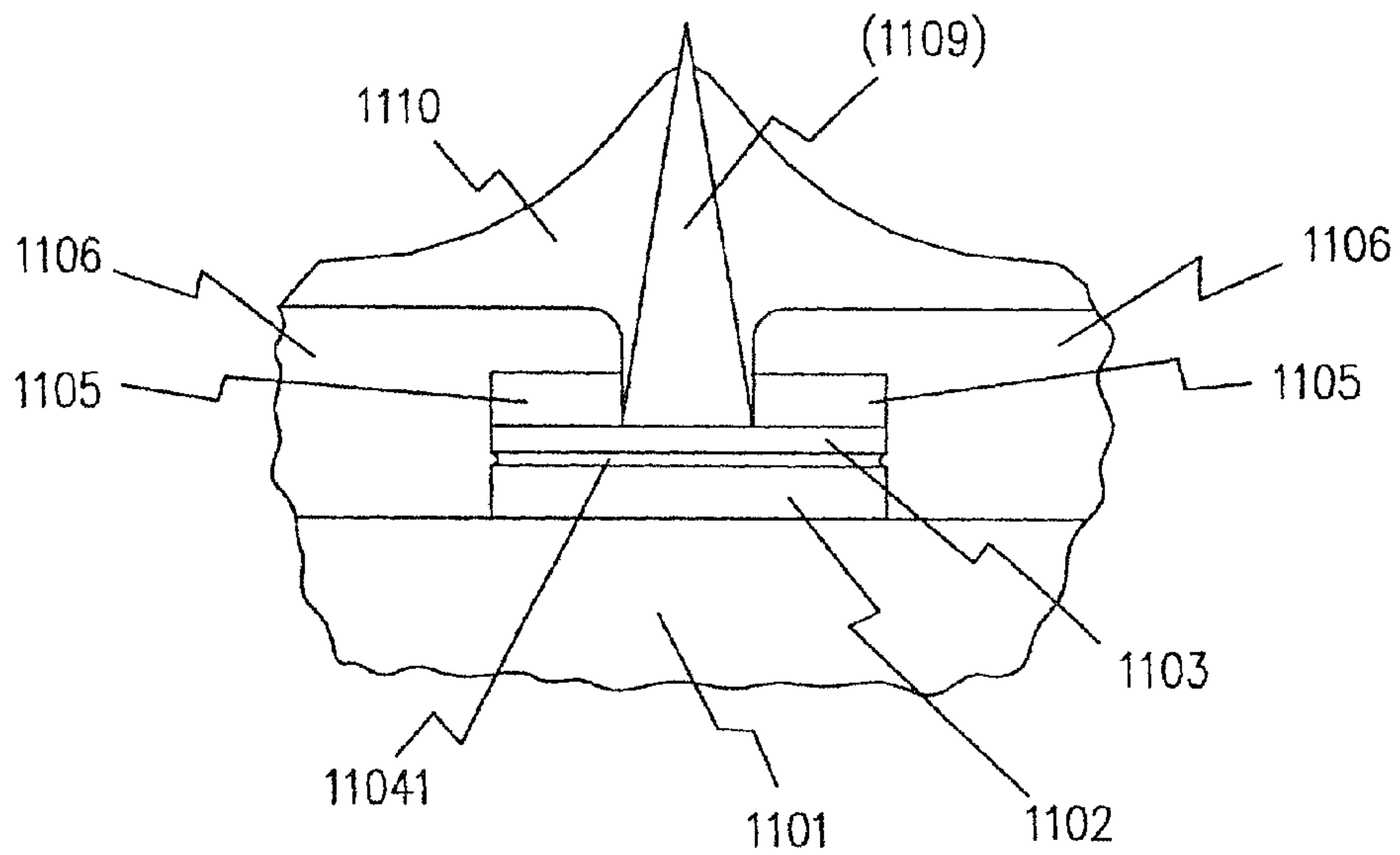
FIGURE 11b ELECTRODES
