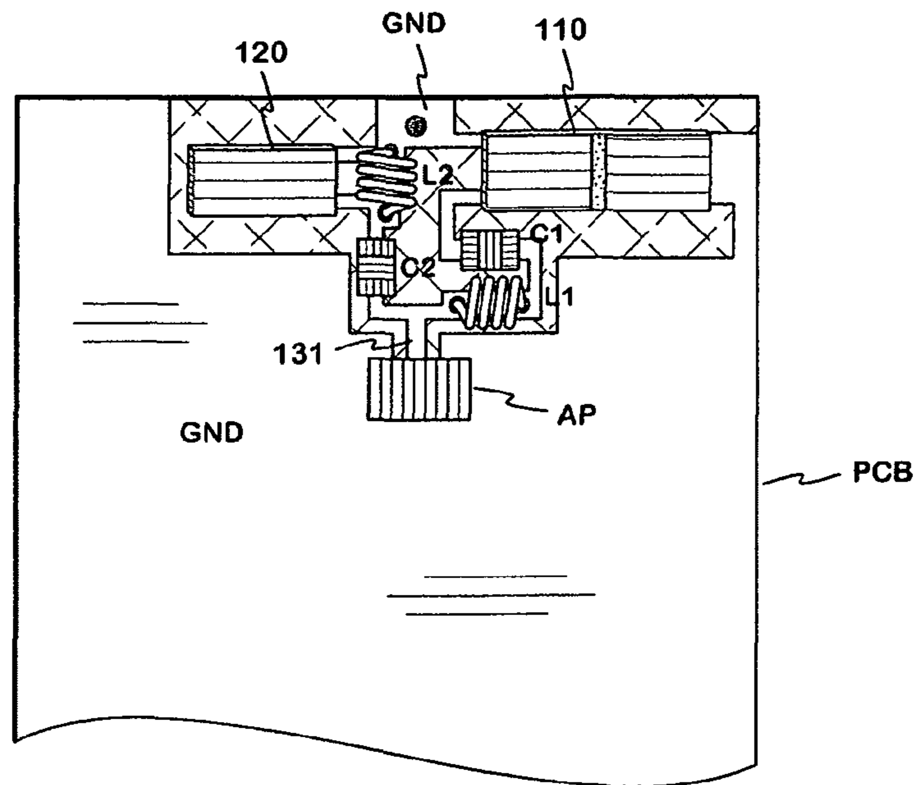
Fig. 1 PRIOR ART
