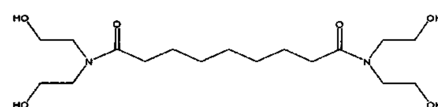
Azelaic Bis(Diethanolamide) Functionality = 4
