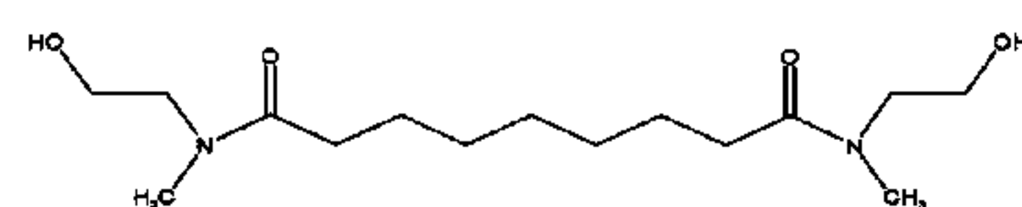
Azelaic Bis(N-Methylethanamide) Functionality = 2
