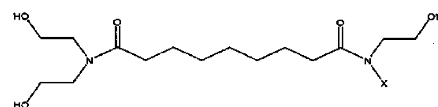
Hybrid Azelaic Diethanolamide XXX
