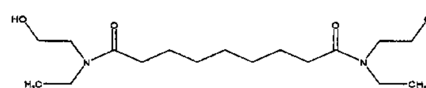
Azelaic Bis(N-Ethylethanamide) Functionality = 2
