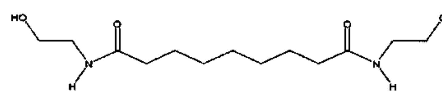
Azelaic Bis(Ethanamide) Functionality = 2
