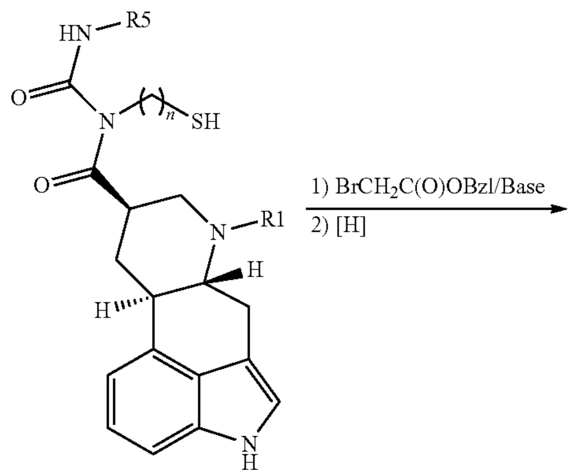
Scheme 12:
