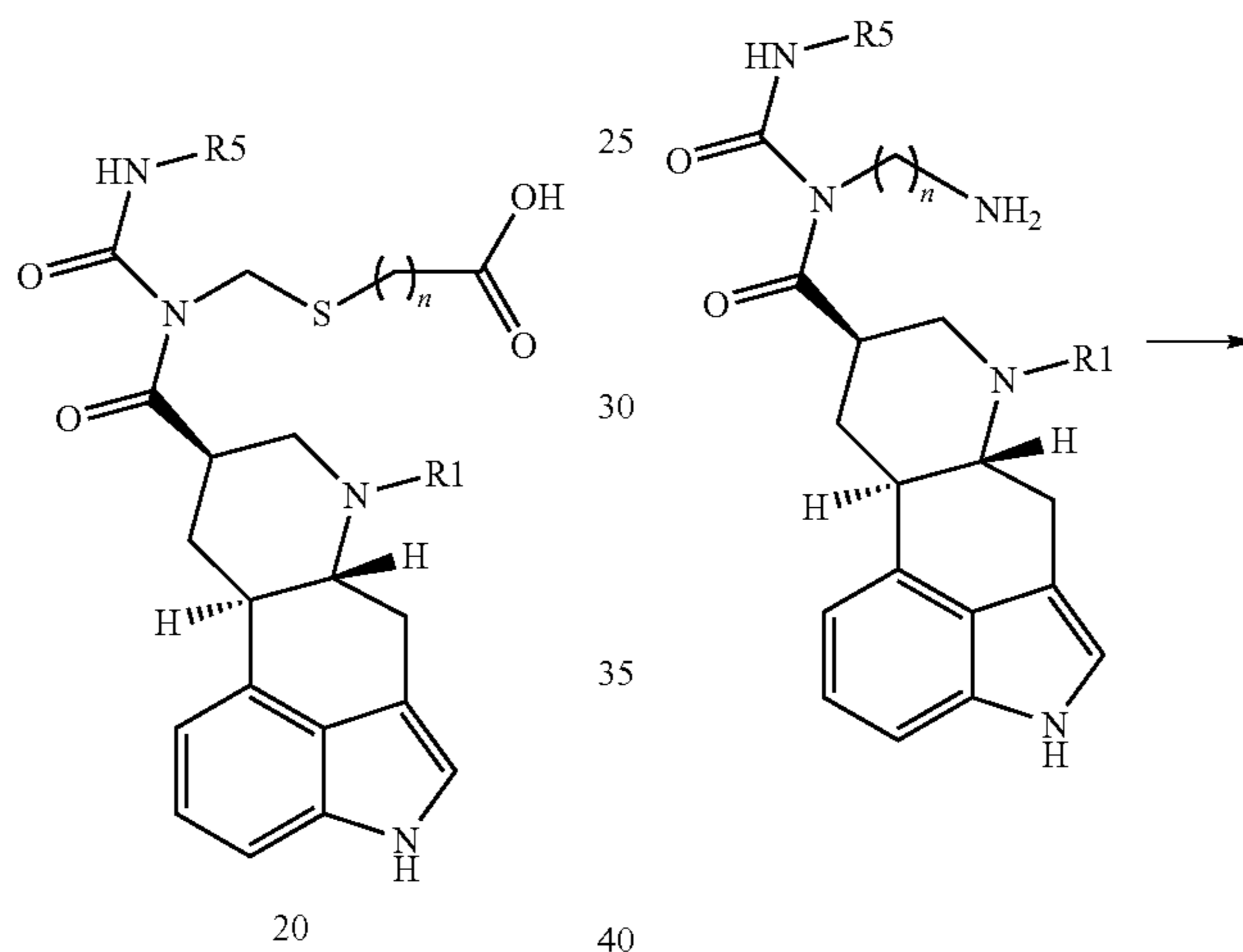
Scheme 14:
