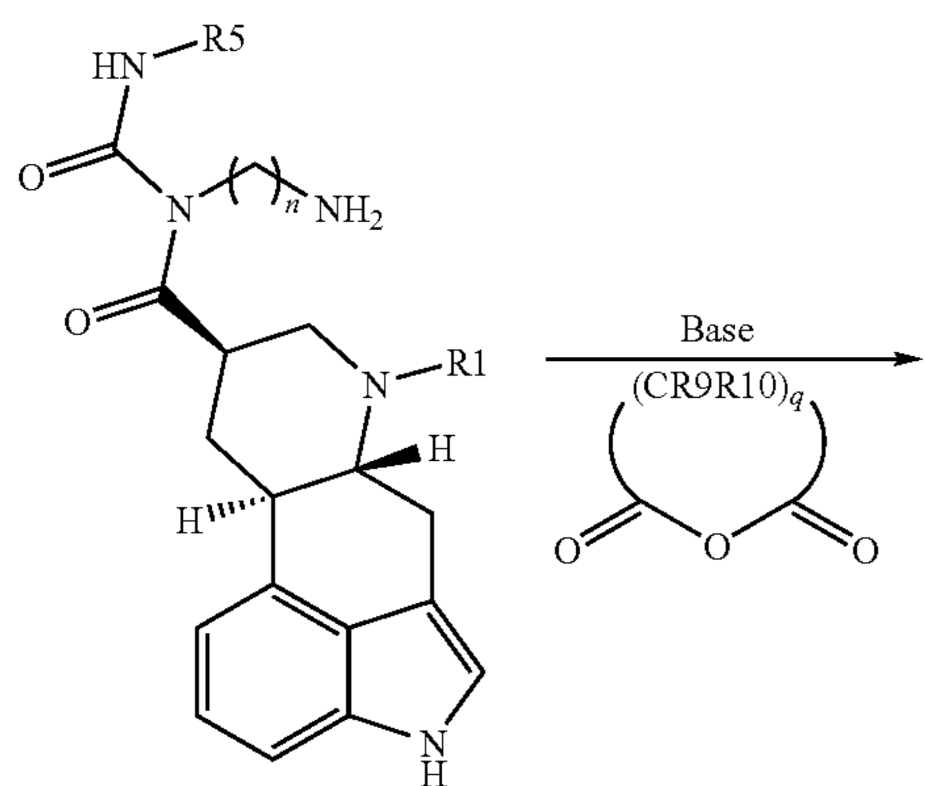
Scheme 13:
