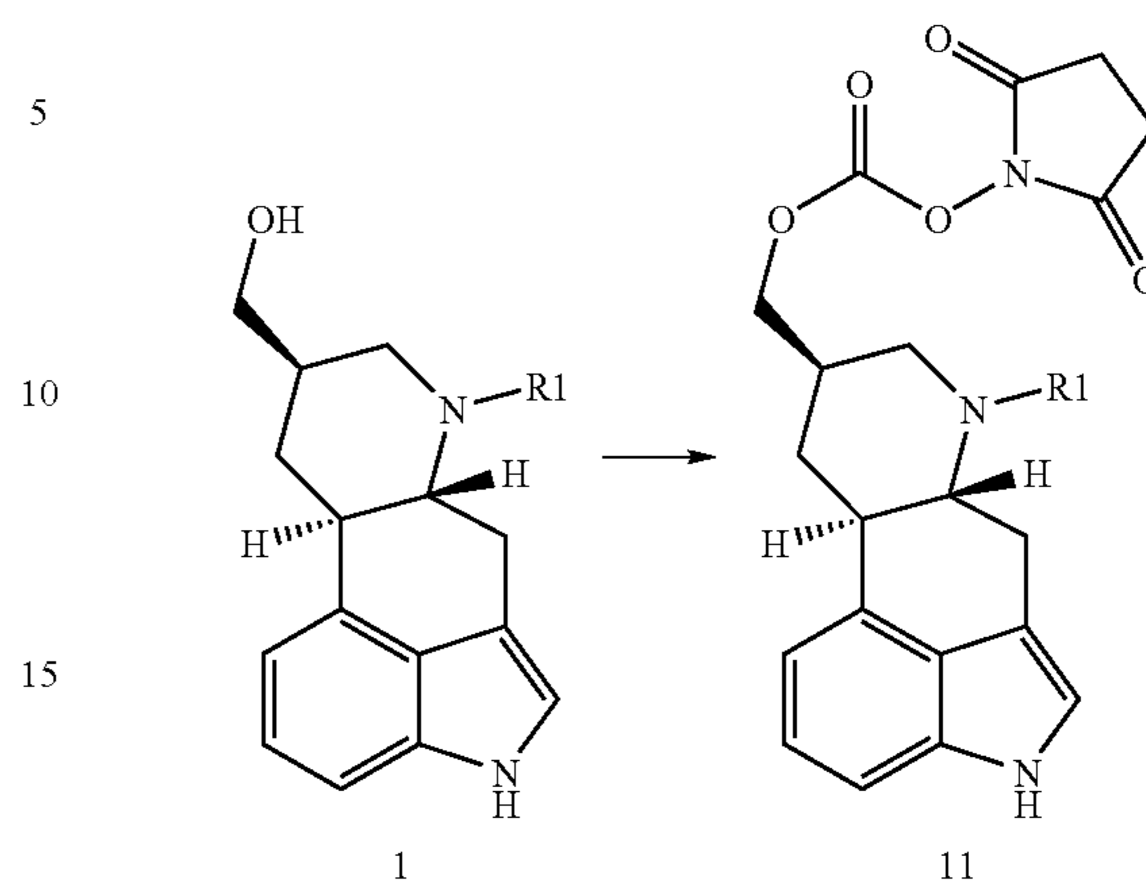
Scheme 5:
