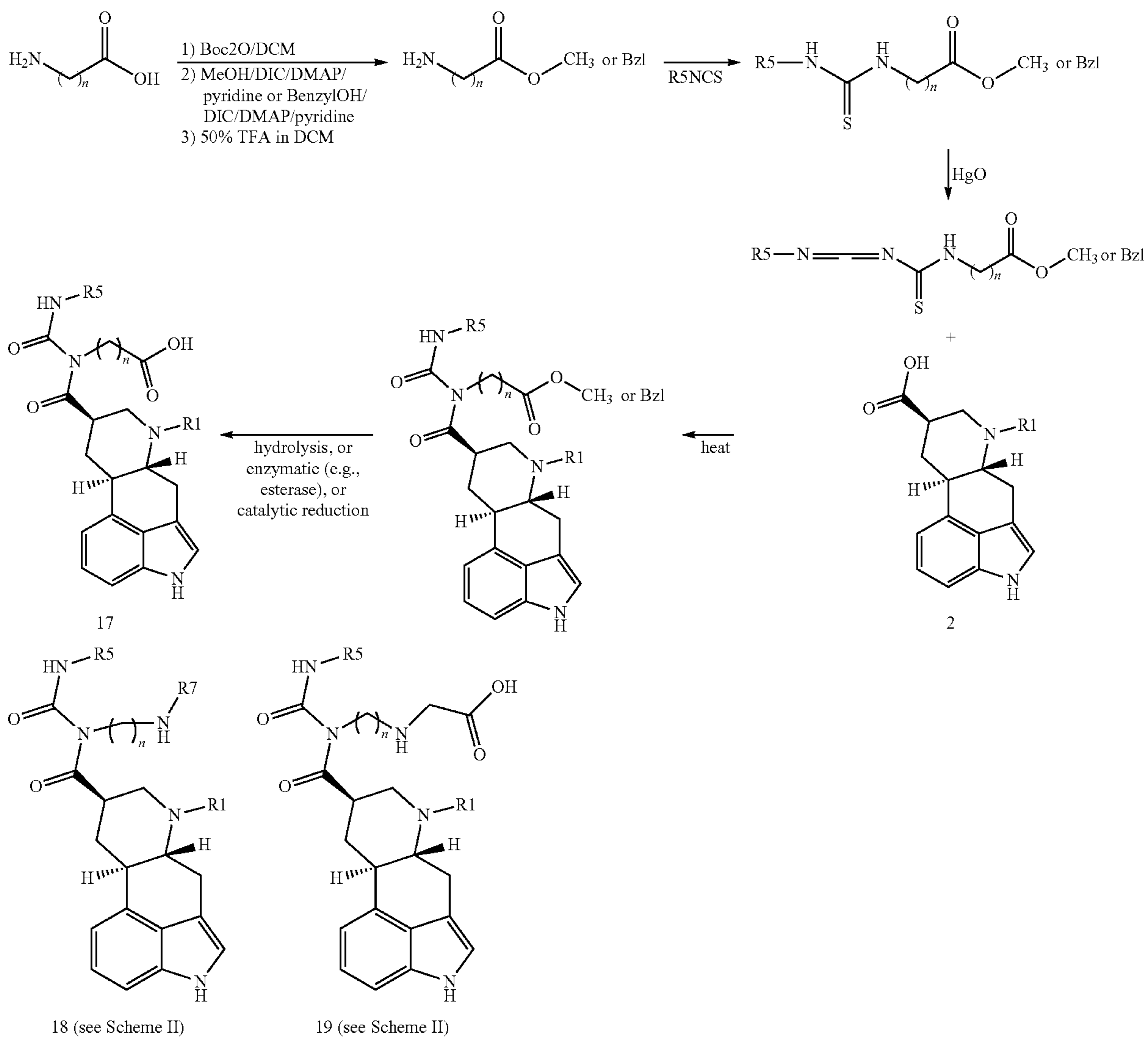
Scheme 11:
