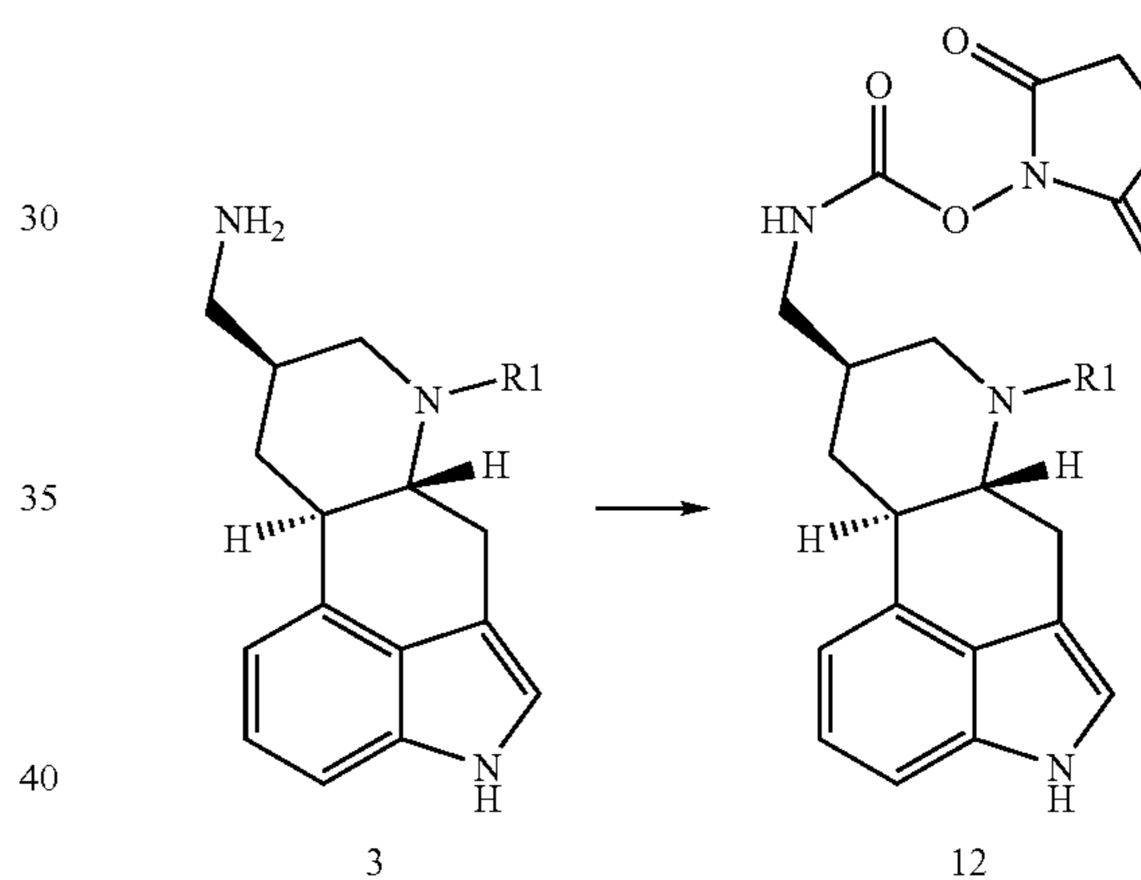
Scheme 6:
