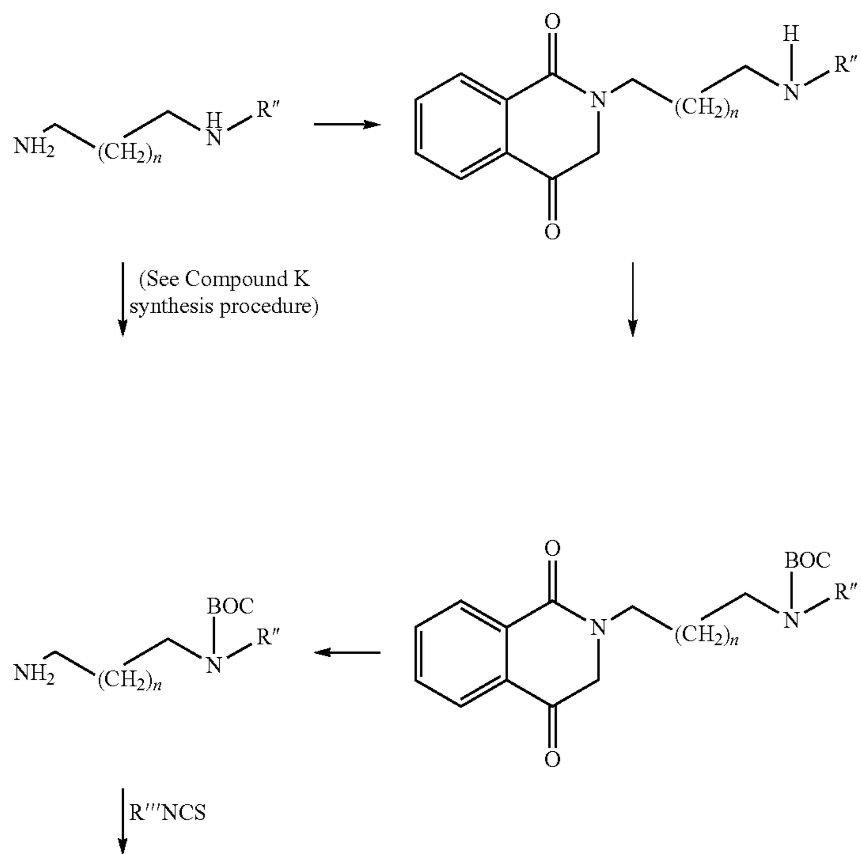
Scheme II
