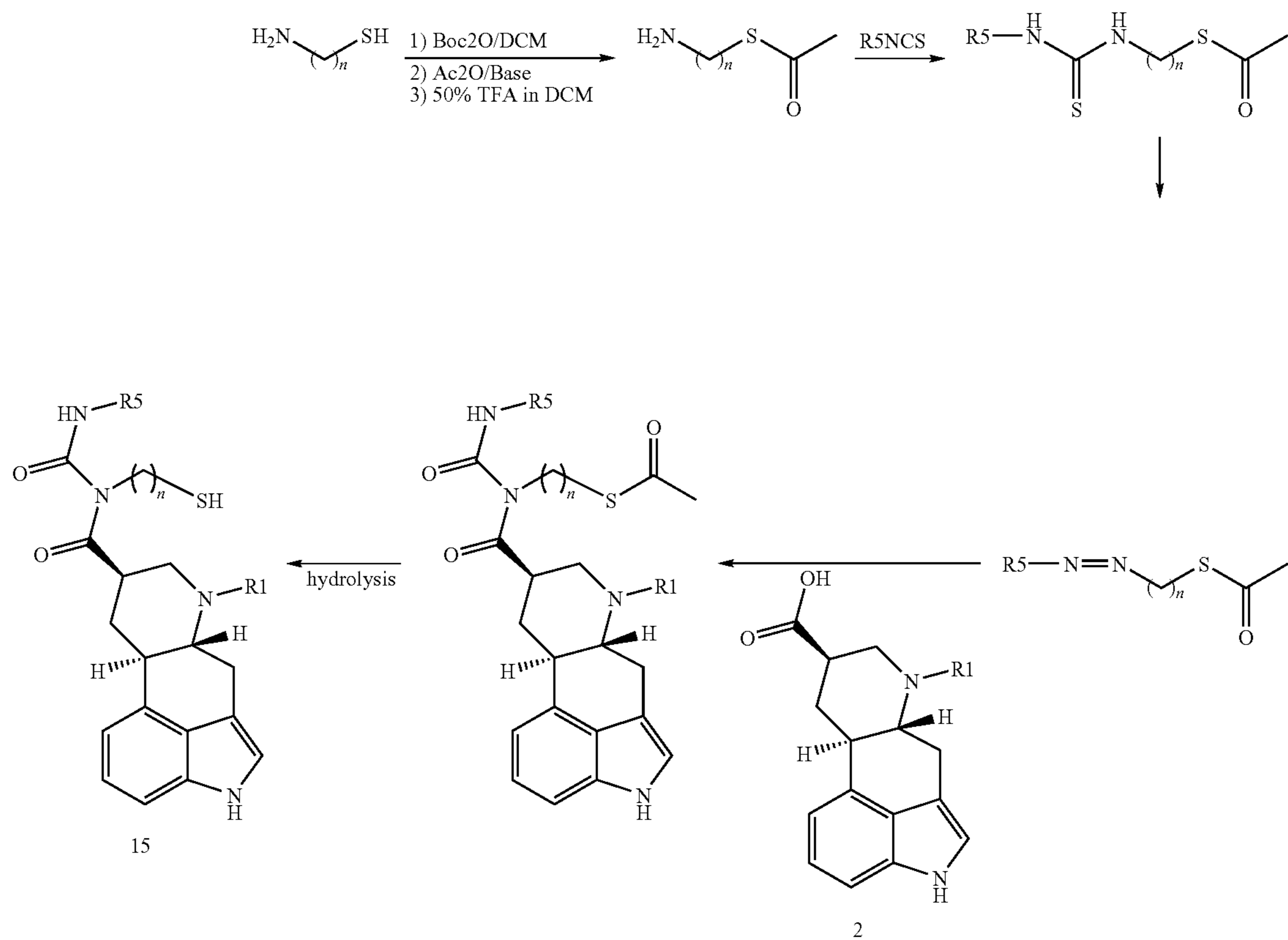
Scheme 9:
