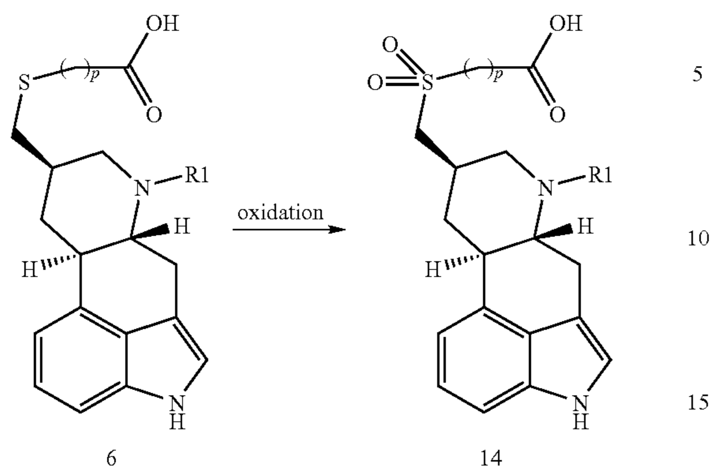
Scheme 8:
