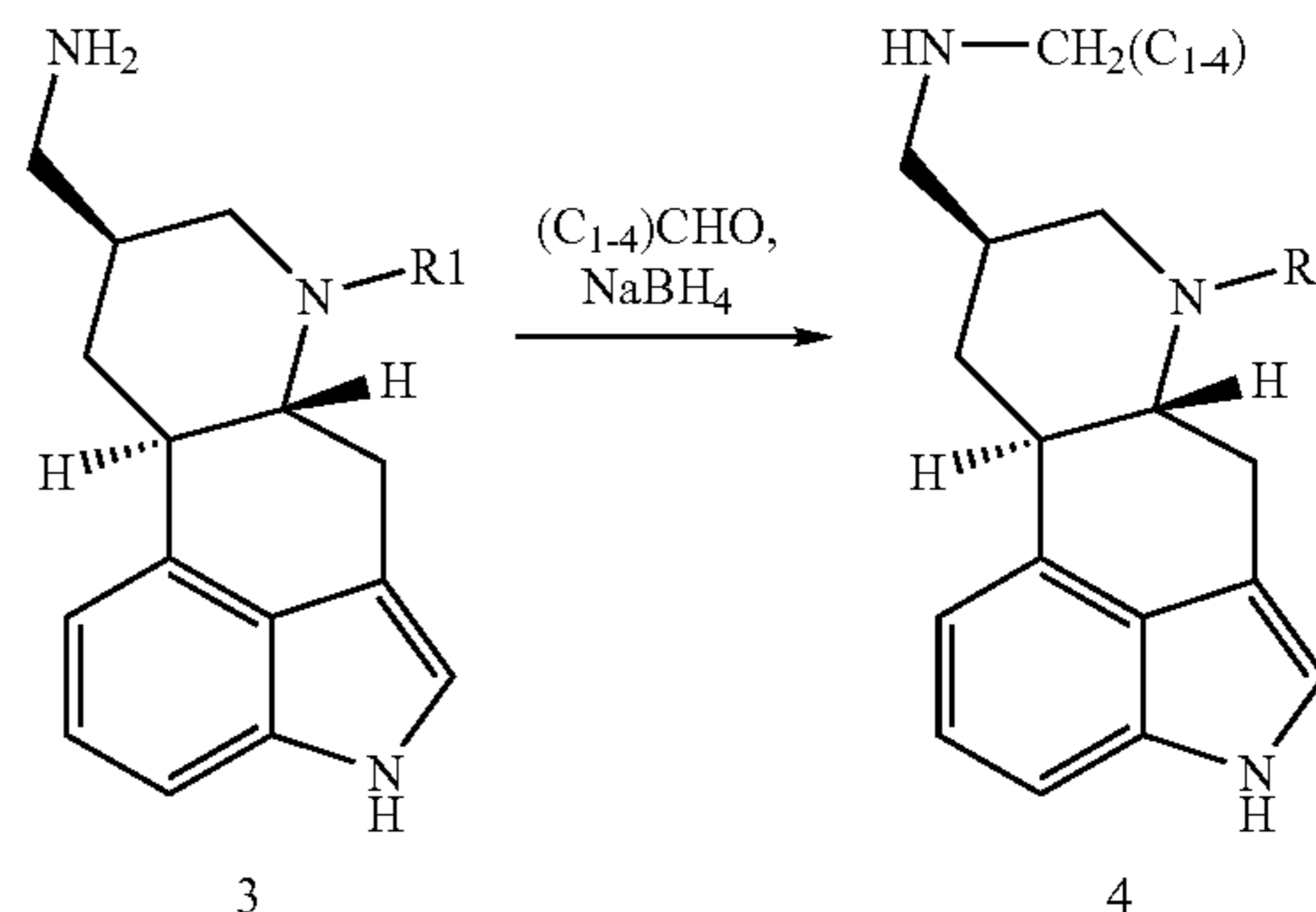
Scheme 2
