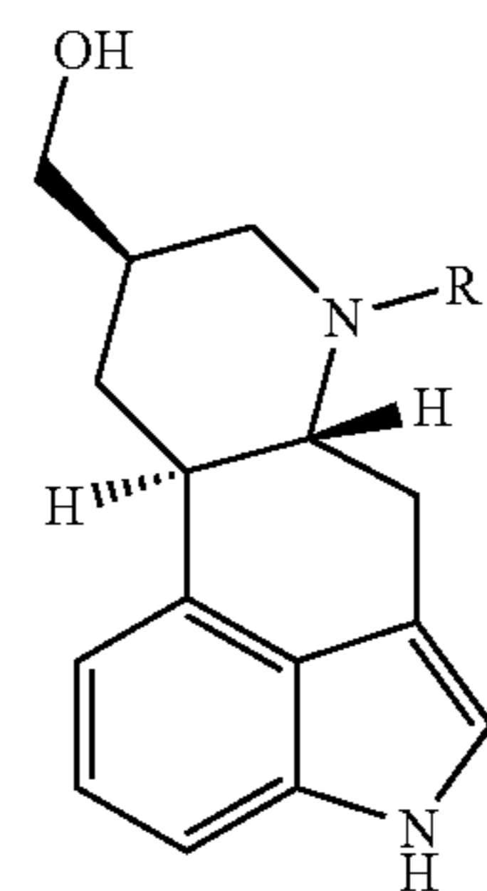
Scheme 1
