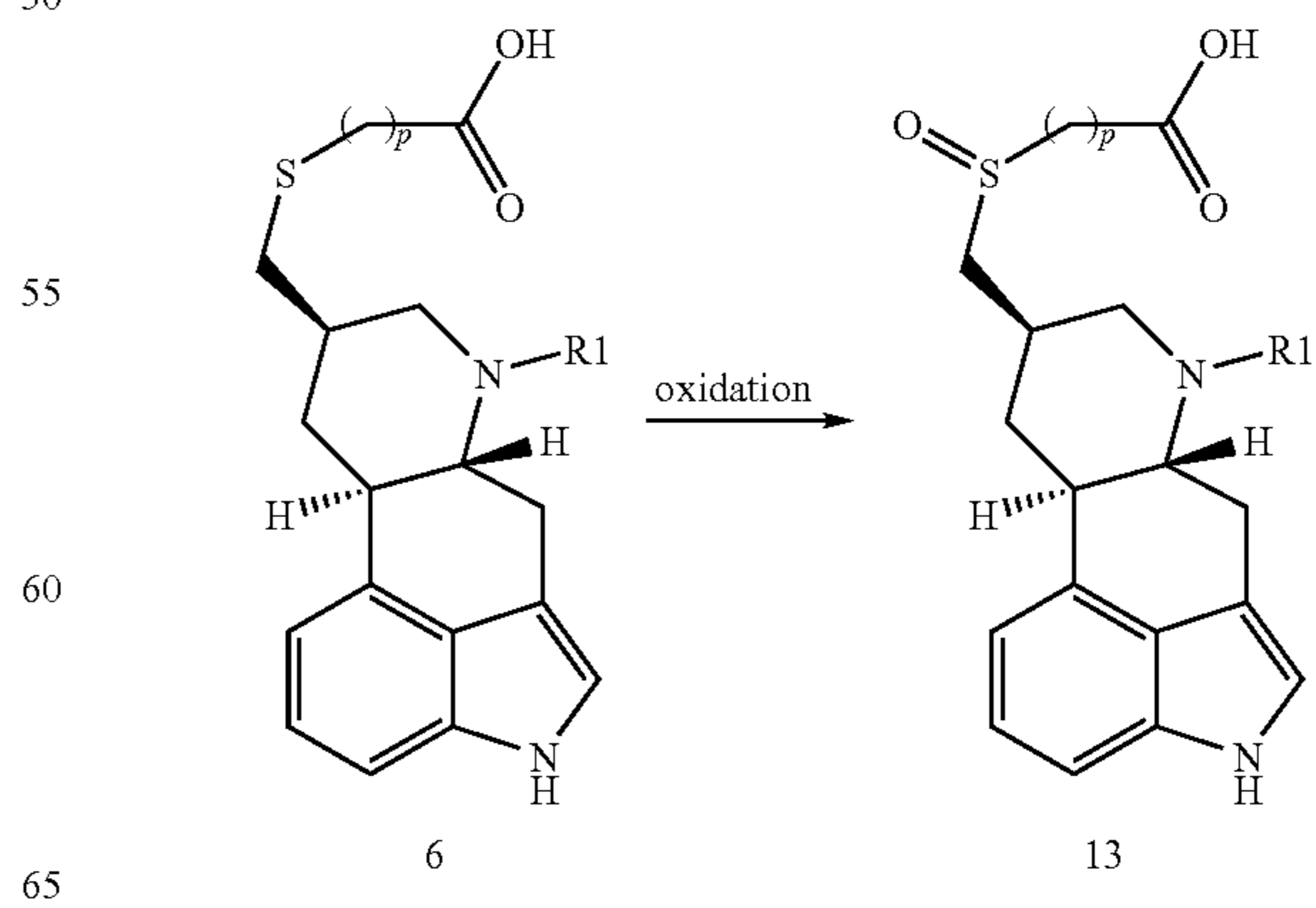
Scheme 7:
