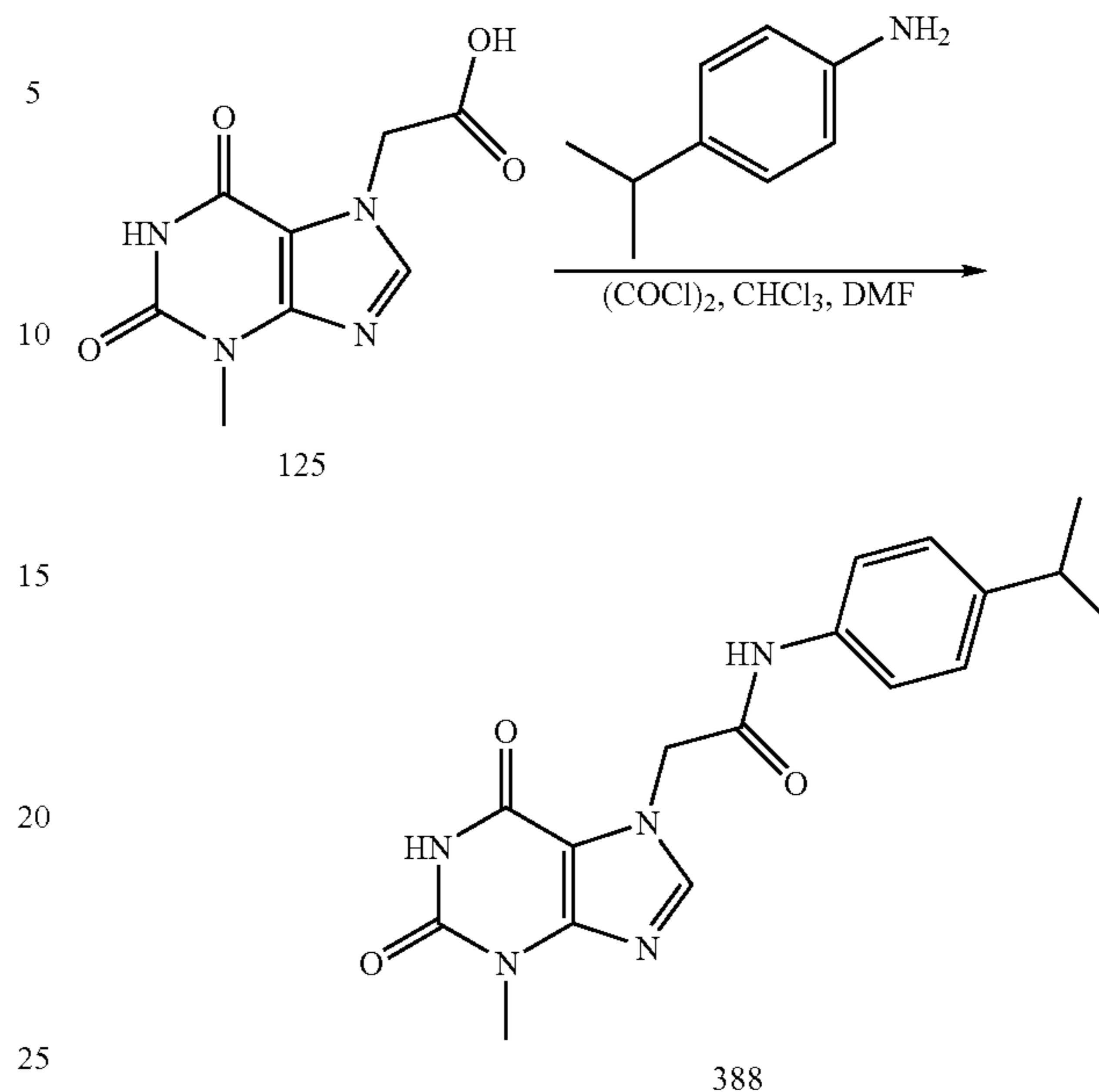
N-(4-isopropylphenyl)-2-(3-methyl-2,6-dioxo-1,2,3,6-tetrahydropurin-7-yl)acetamide (388)
