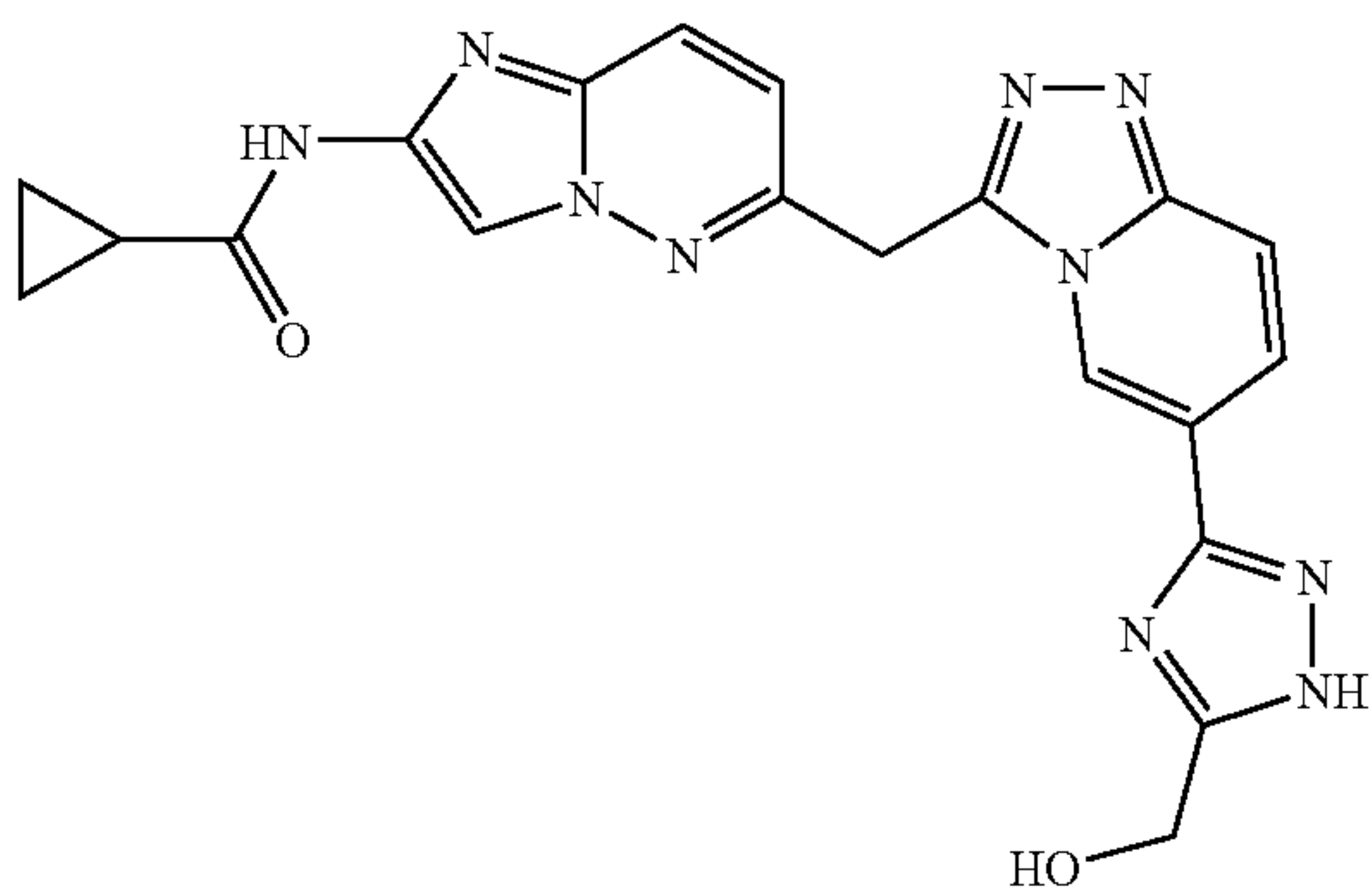
N-((6-((6-(5-(hydroxymethyl)-1H-1,2,4-triazol-3-yl)-[1,2,4]triazolo[4,3-a]pyridin-3-yl)methyl)imidazo[1,2-b]pyridazin-2-yl)cyclopropanecarboxamide
