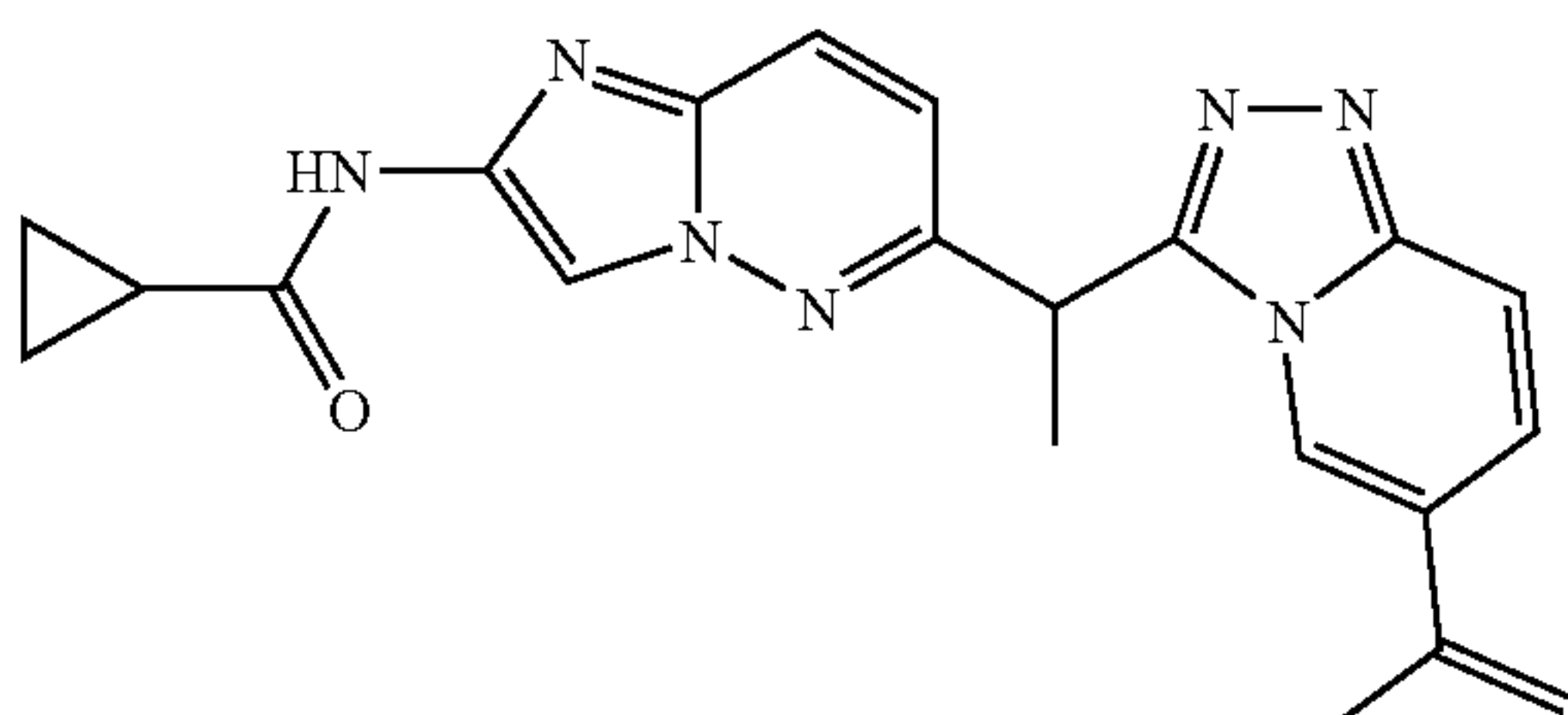
N-(6-(1-(6-(prop-1-en-2-yl)-[1,2,4]triazolo[4,3-a]pyridin-3-yl)ethyl)imidazo[1,2-b]pyridazin-2-yl)cyclopropanecarboxamide
