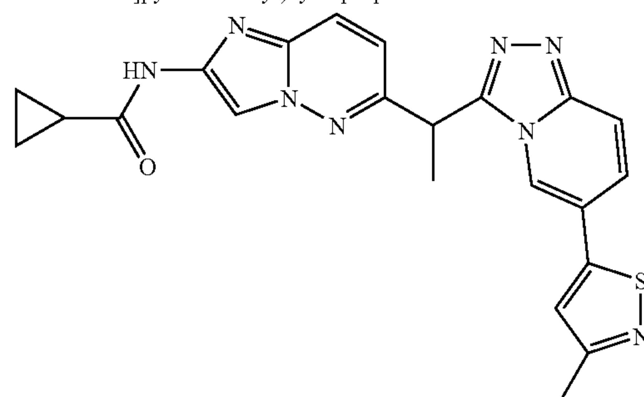
N-(6-(1-(6-(3-methylisothiazol-5-yl)-[1,2,4]triazolo[4,3-a]pyridin-3-yl)ethyl)imidazo[1,2-b]pyridazin-2-yl)cyclopropanecarboxamide
