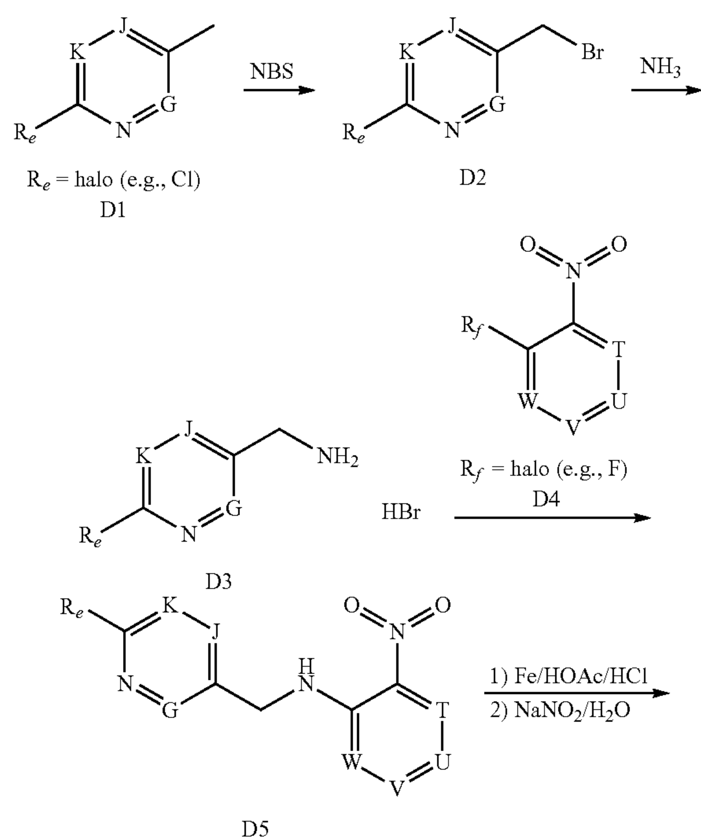
Scheme D
