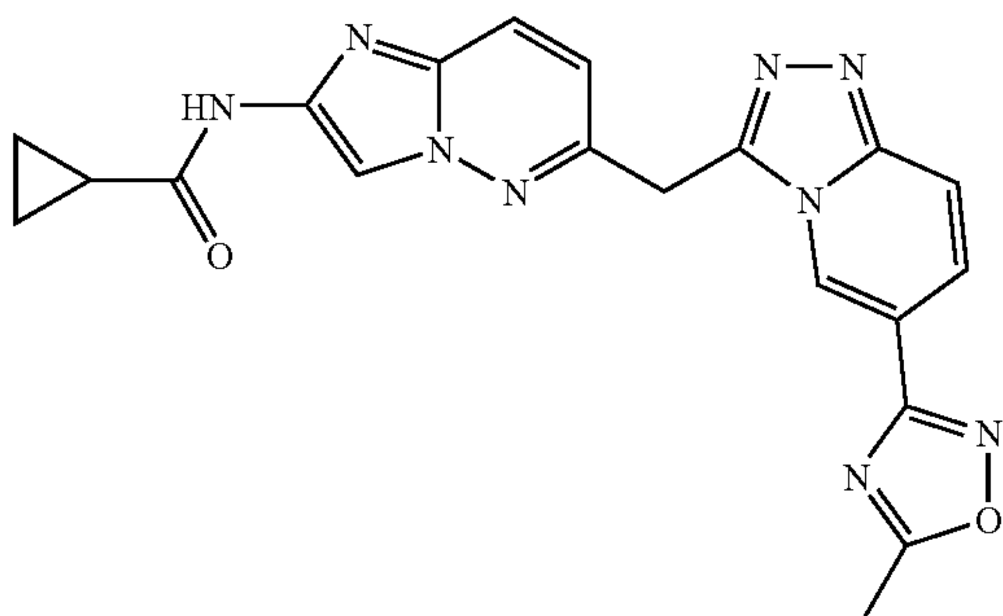
N-((6-((6-(5-methyl-1,2,4-oxadiazol-3-yl)-[1,2,4]triazolo[4,3-a]pyridin-3-yl)methyl)imidazo[1,2-b]pyridazin-2-yl)cyclopropanecarboxamide
