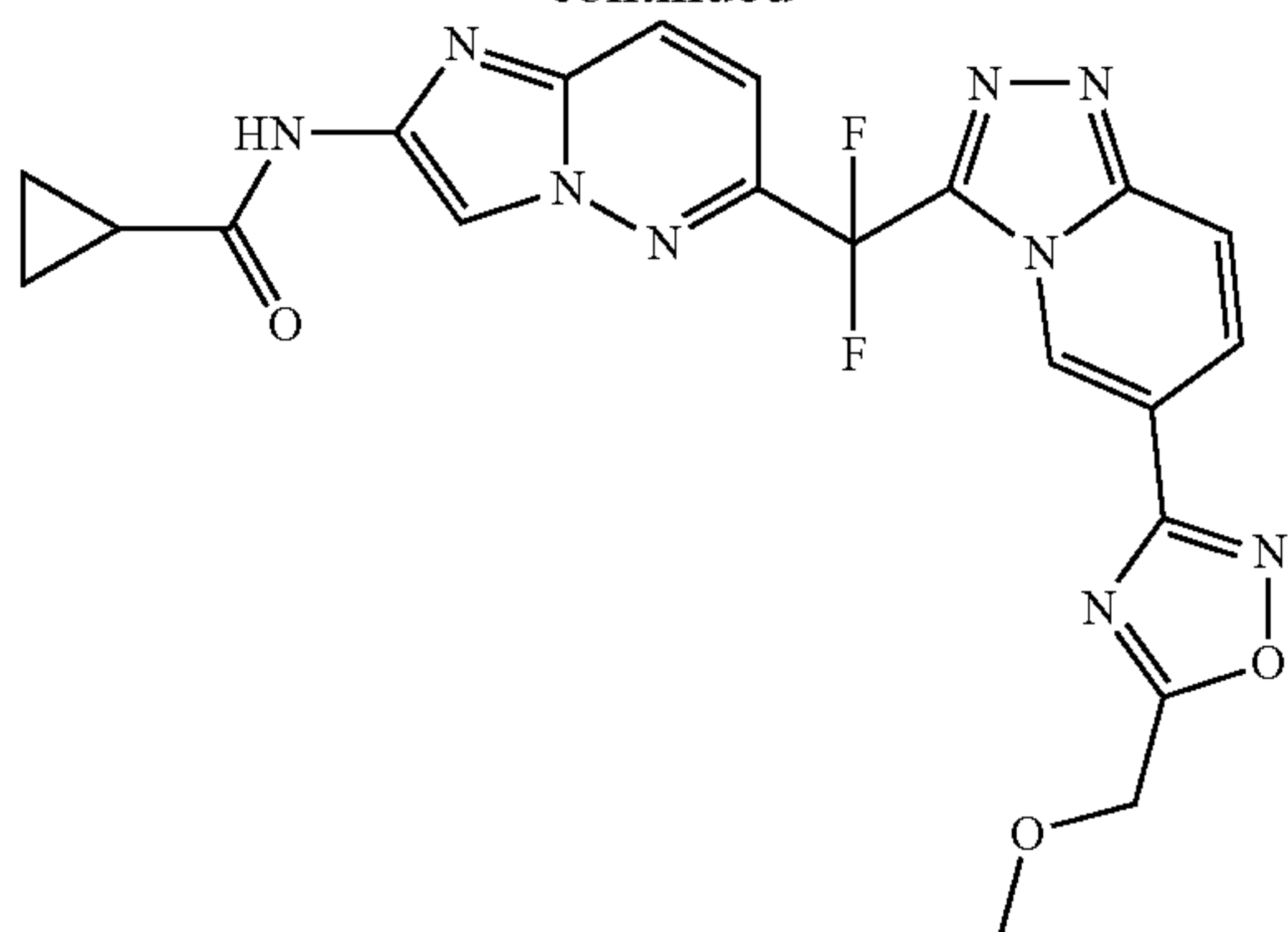
N-(6-(difluoro(6-(5-(methoxymethyl)-1,2,4-oxadiazol-3-yl)-[1,2,4]triazolo[4,3-a]pyridin-3-yl)methyl)imidazo[1,2-b]pyridazin-2-yl)cyclopropanecarboxamide
