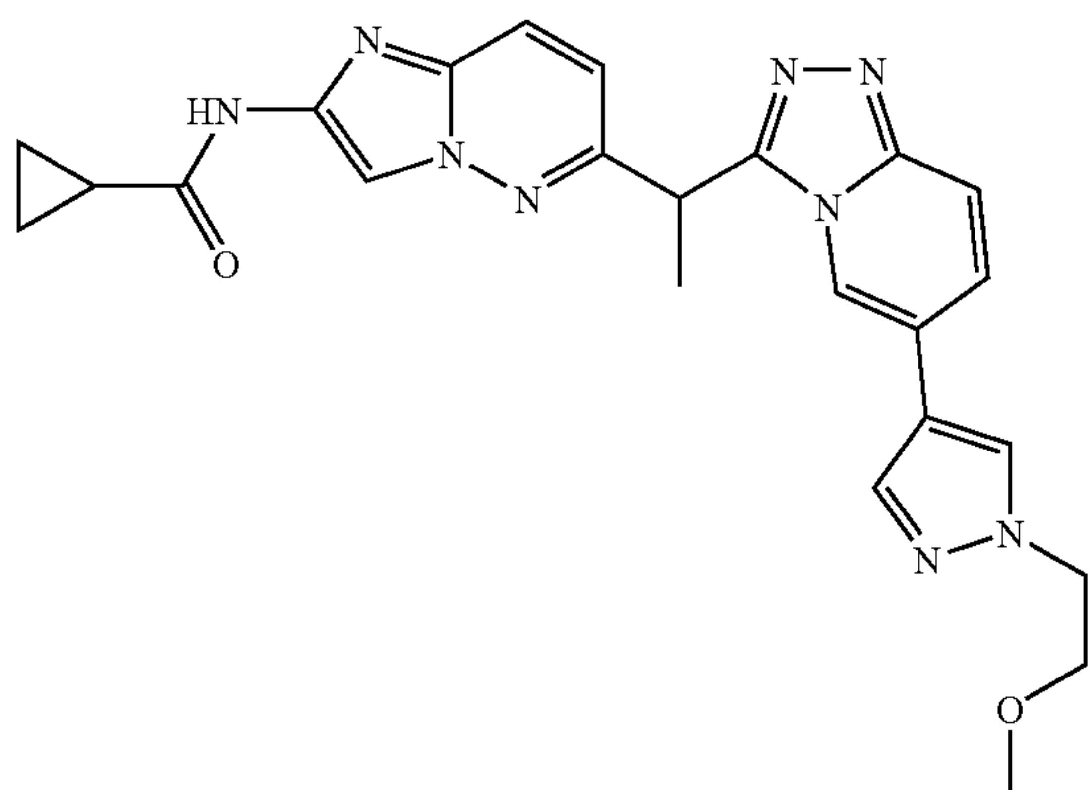
N-(6-(1-(6-(1-(2-methoxyethyl)-1H-pyrazol-4-yl)-[1,2,4]triazolo[4,3-a]pyridin-3-yl)ethyl)imidazo[1,2-b]pyridazin-2-yl)cyclopropanecarboxamide
