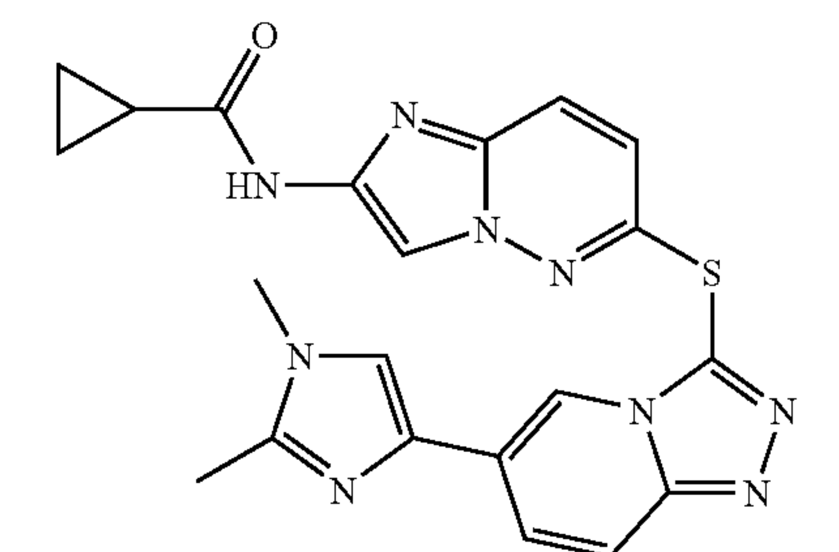
N-(6-(6-(1,2-dimethyl-1H-imidazol-4-yl)-[1,2,4]triazolo[4,3-a]pyridin-3-ylthio)imidazo[1,2-b]pyridazin-2-yl)cyclopropanecarboxamide
