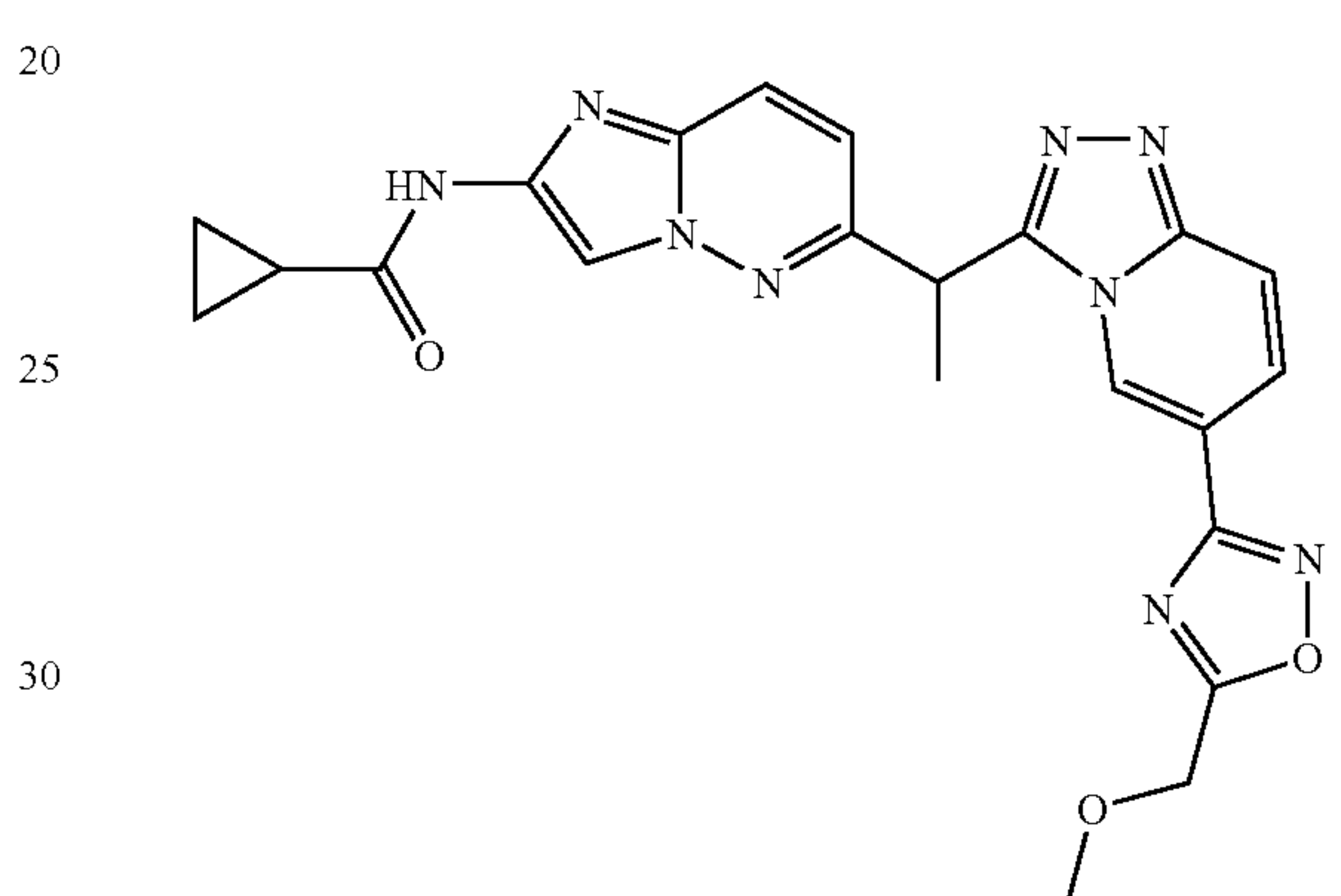
N-(6-(1-(6-(5-(methoxymethyl)-1,2,4-oxadiazol-3-yl)-[1,2,4]triazolo[4,3-a]pyridin-3-yl)ethyl)imidazo[1,2-b]pyridazin-2-yl)cyclopropanecarboxamide
