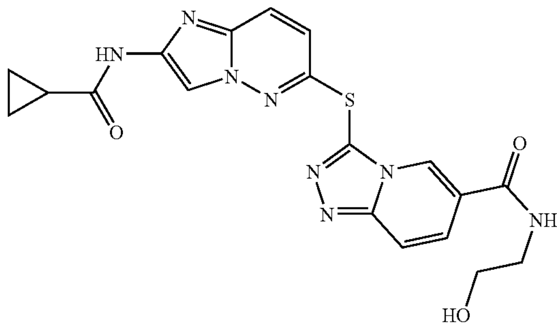
3-(2-(cyclopropanecarboxamido)imidazo[1,2-b]pyridazin-6-ylthio)-N-(2-hydroxyethyl)-[1,2,4]triazolo[4,3-a]pyridine-6-carboxamide
