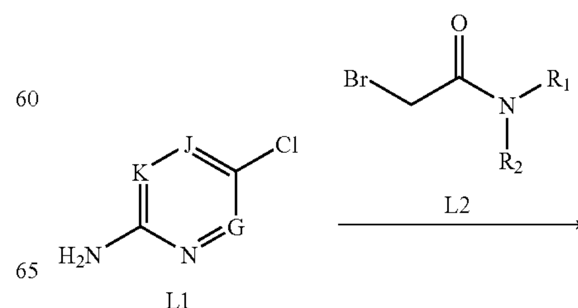
Scheme L
