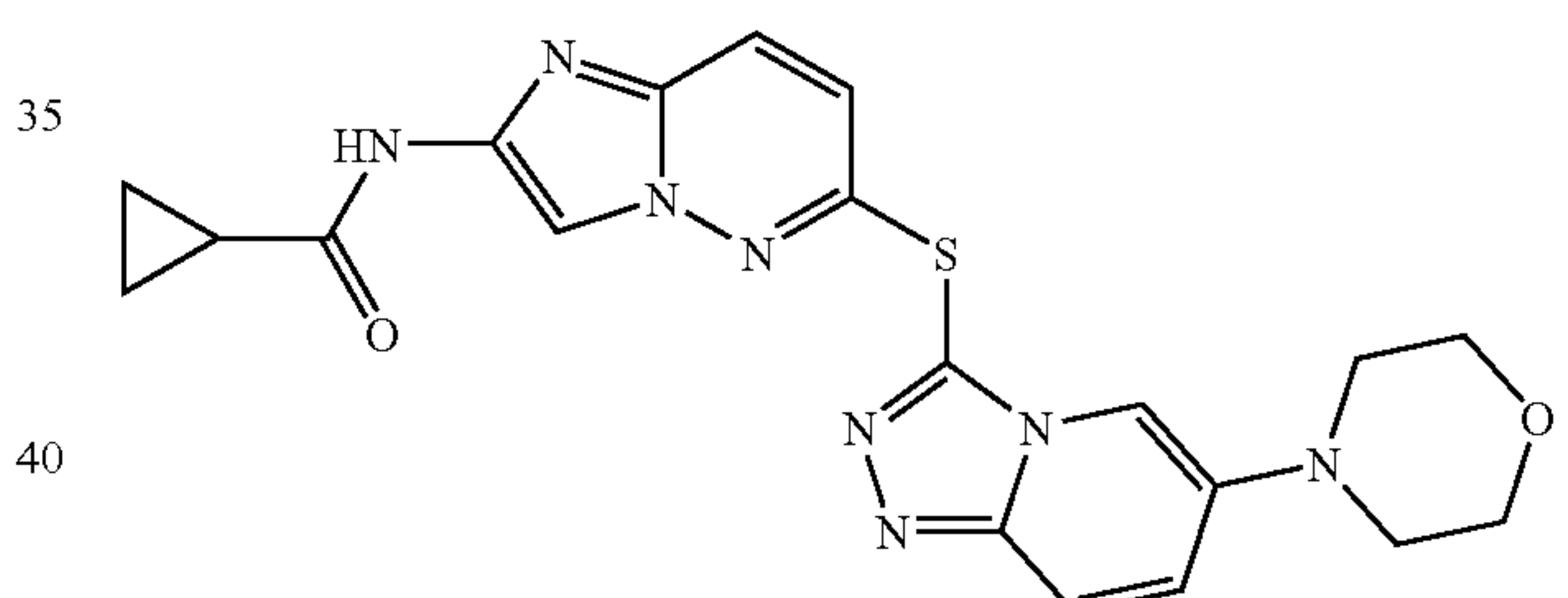
N-(6-(6-(morpholino)-[1,2,4]triazolo[4,3-a]pyridin-3-ylthio)imidazo[1,2-b]pyridazin-2-yl)cyclopropanecarboxamide
