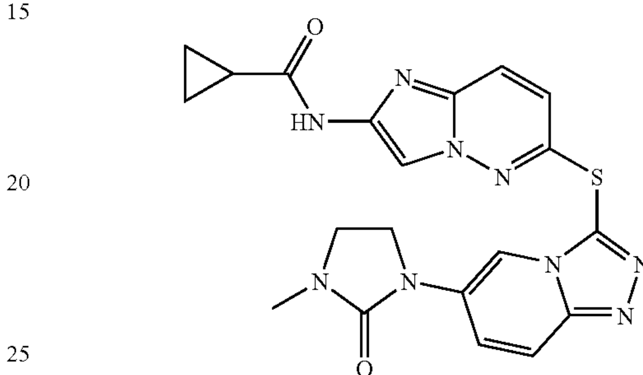
N-(6-(6-(3-methyl-2-oximidazolidin-1-yl)-[1,2,4]triazolo[4,3-a]pyridin-3-ylthio)imidazo[1,2-b]pyridazin-2-yl)cyclopropanecarboxamide
