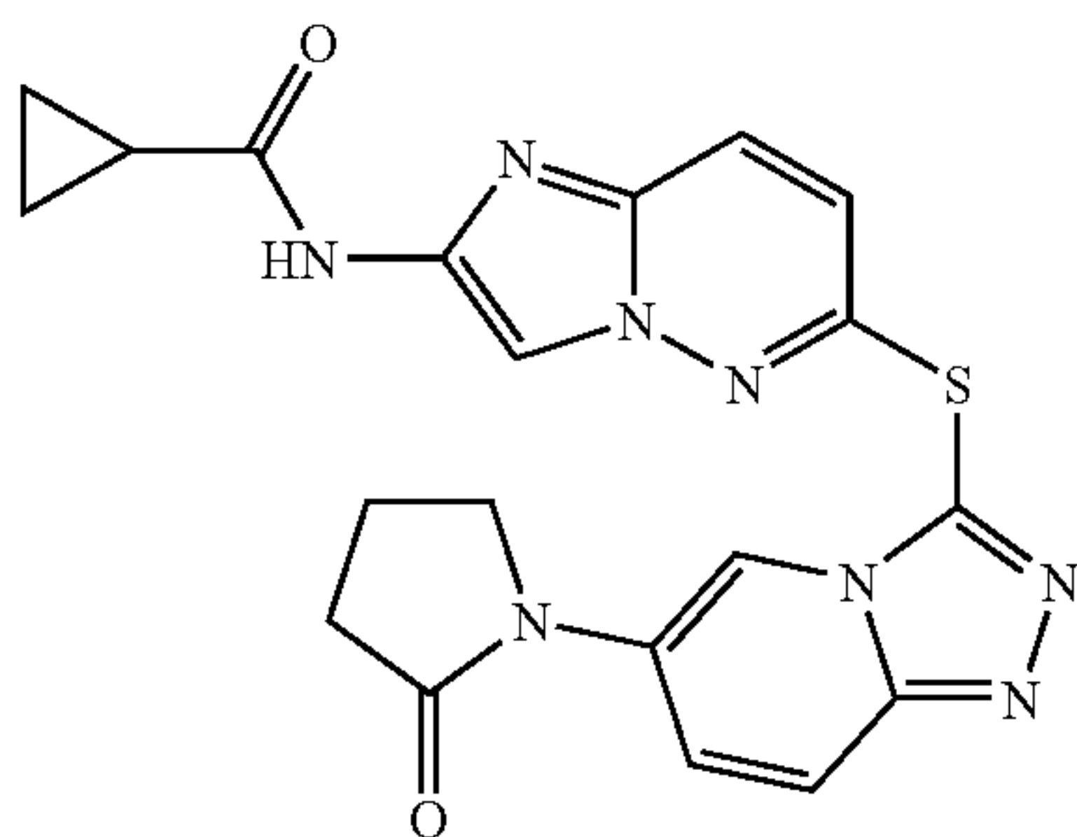
N-(6-(6-(2-oxopyrrolidin-1-yl)-[1,2,4]triazolo[4,3-a]pyridin-3-ylthio)imidazo[1,2-b]pyridazin-2-yl)cyclopropanecarboxamide
