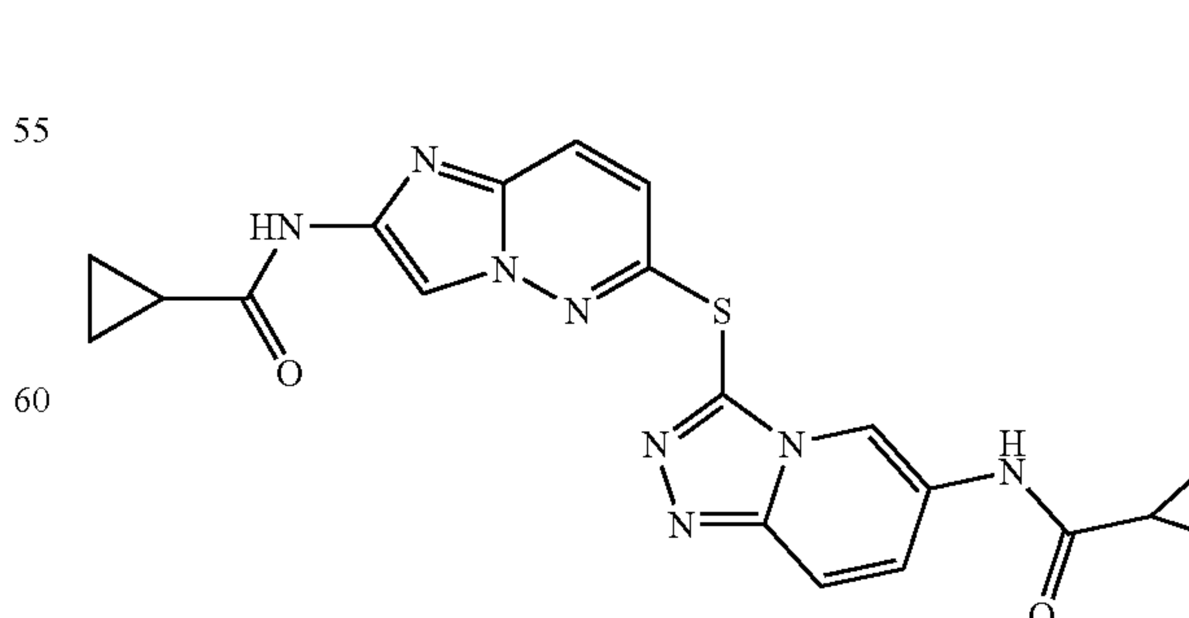
N-(6-(6-(cyclopropanecarboxamido)-[1,2,4]triazolo[4,3-a]pyridin-3-ylthio)imidazo[1,2-b]pyridazin-2-yl)cyclopropanecarboxamide
