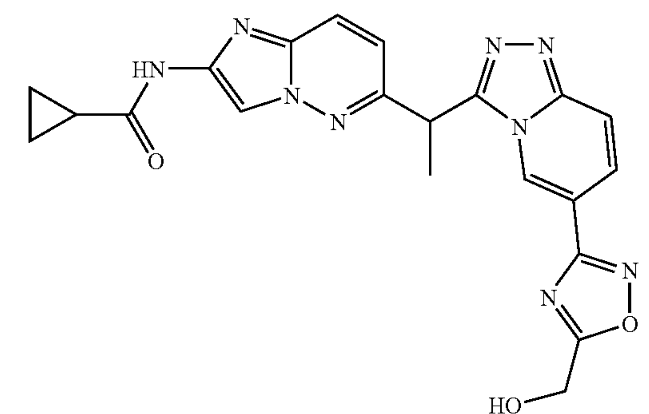
N-(6-(1-(6-(5-(hydroxymethyl)-1,2,4-oxadiazol-3-yl)-[1,2,4]triazolo[4,3-a]pyridin-3-yl)ethyl)imidazo[1,2-b]pyridazin-2-yl)cyclopropanecarboxamide
