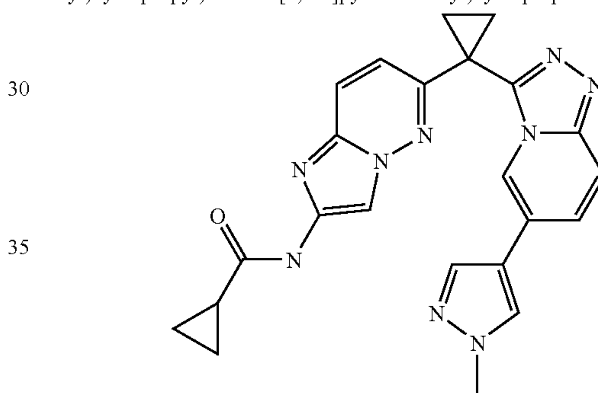
N-(6-(1-(6-(1-methyl-1H-pyrazol-4-yl)-[1,2,4]triazolo[4,3-a]pyridin-3-yl)cyclopropyl)imidazo[1,2-b]pyridazin-2-yl)cyclopropanecarboxamide
