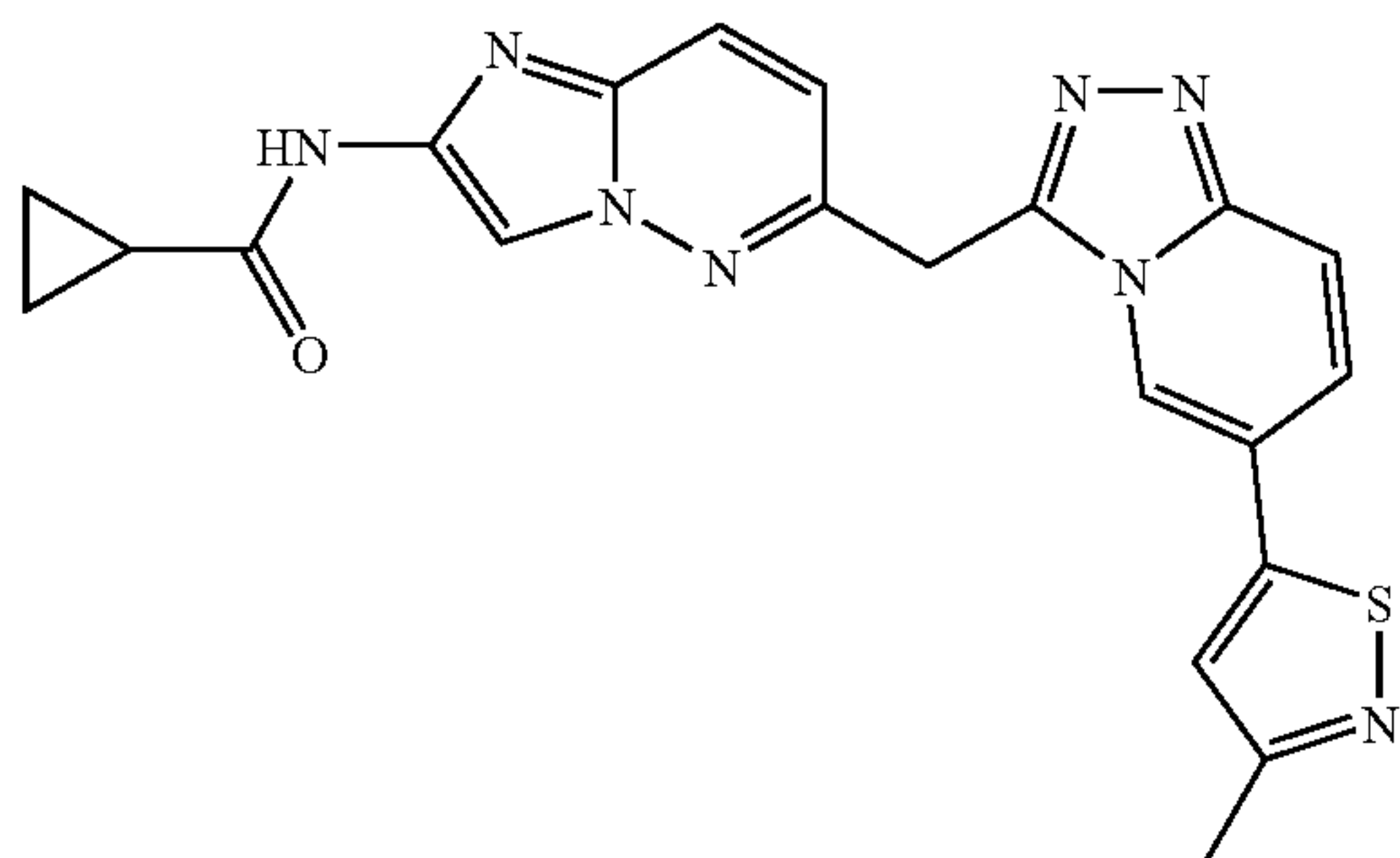
N-(6-((6-(3-methylisothiazol-5-yl)-[1,2,4]triazolo[4,3-a]pyridin-3-yl)methyl)imidazo[1,2-b]pyridazin-2-yl)cyclopropanecarboxamide
