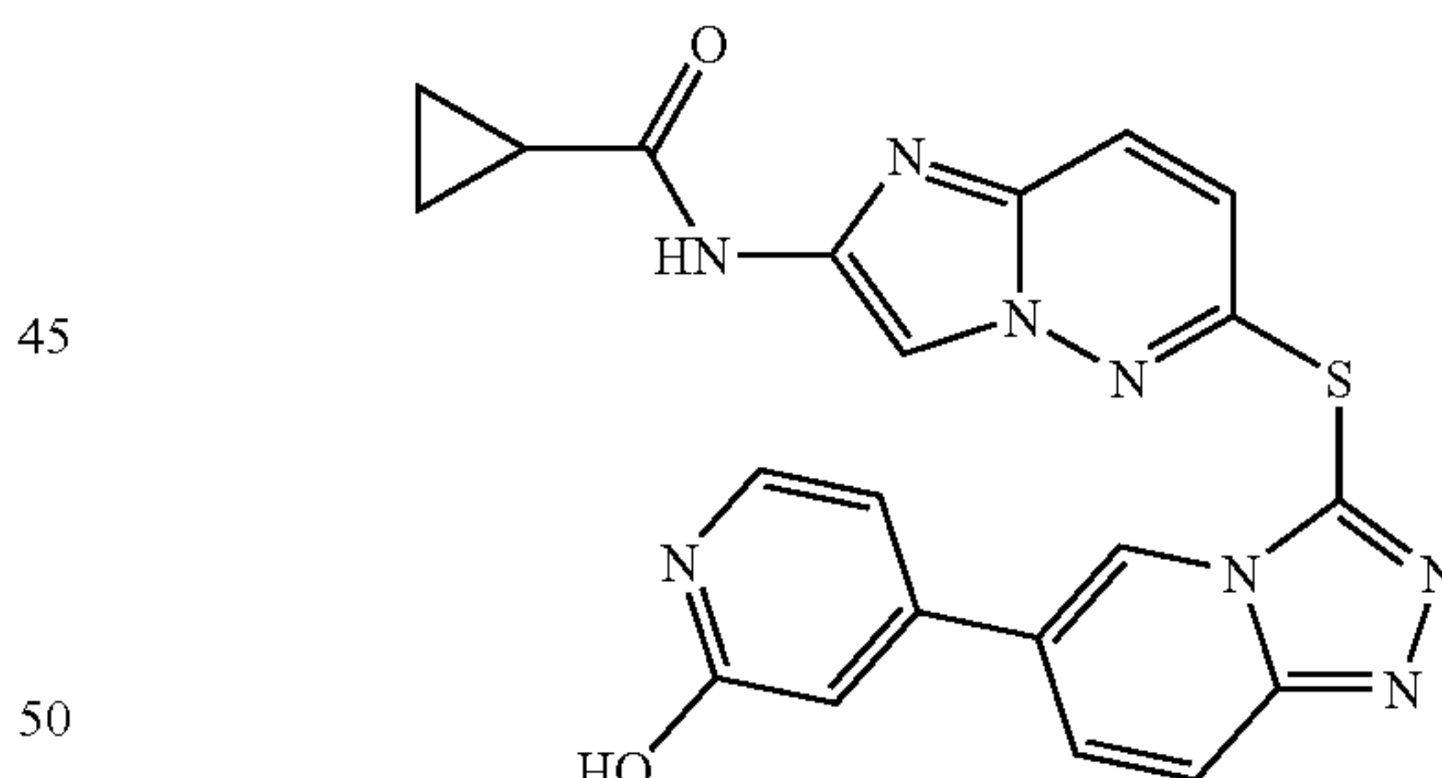
N-(6-(6-(2-hydroxypyridin-4-yl)-[1,2,4]triazolo[4,3-a]pyridin-3-ylthio)imidazo[1,2-b]pyridazin-2-yl)cyclopropanecarboxamide
