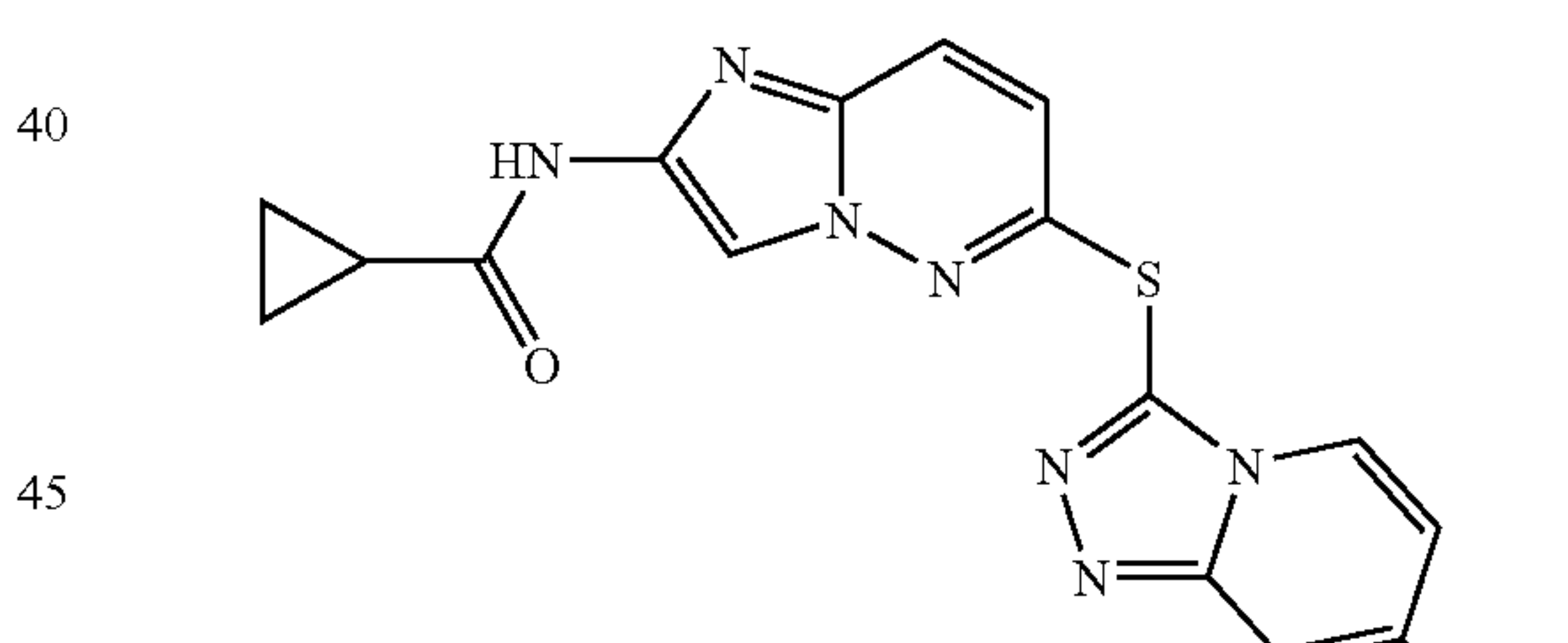
N-(6-(7-(methylamino)-[1,2,4]triazolo[4,3-a]pyridin-3-ylthio)imidazo[1,2-b]pyridazin-2-yl)cyclopropanecarboxamide
