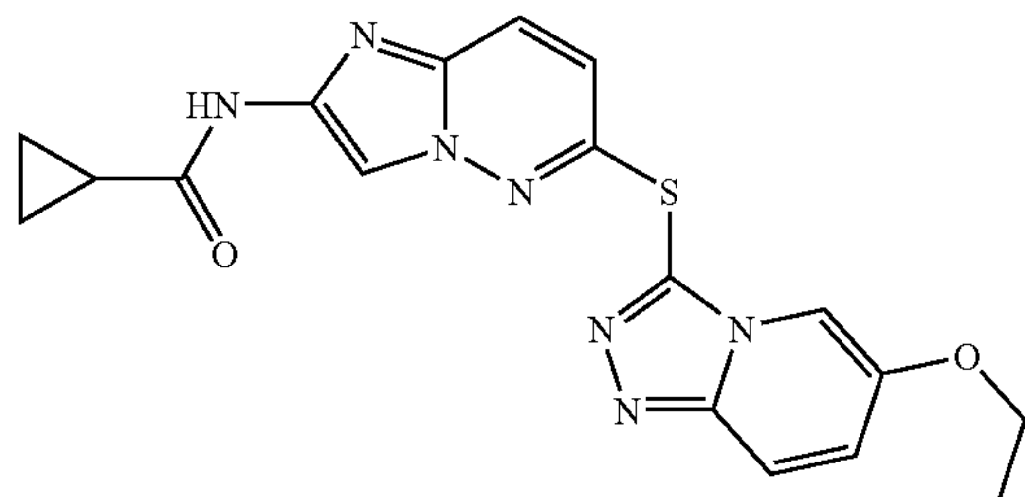
N-(6-(6-ethoxy-[1,2,4]triazolo[4,3-a]pyridin-3-ylthio)imidazo[1,2-b]pyridazin-2-yl)cyclopropanecarboxamide
