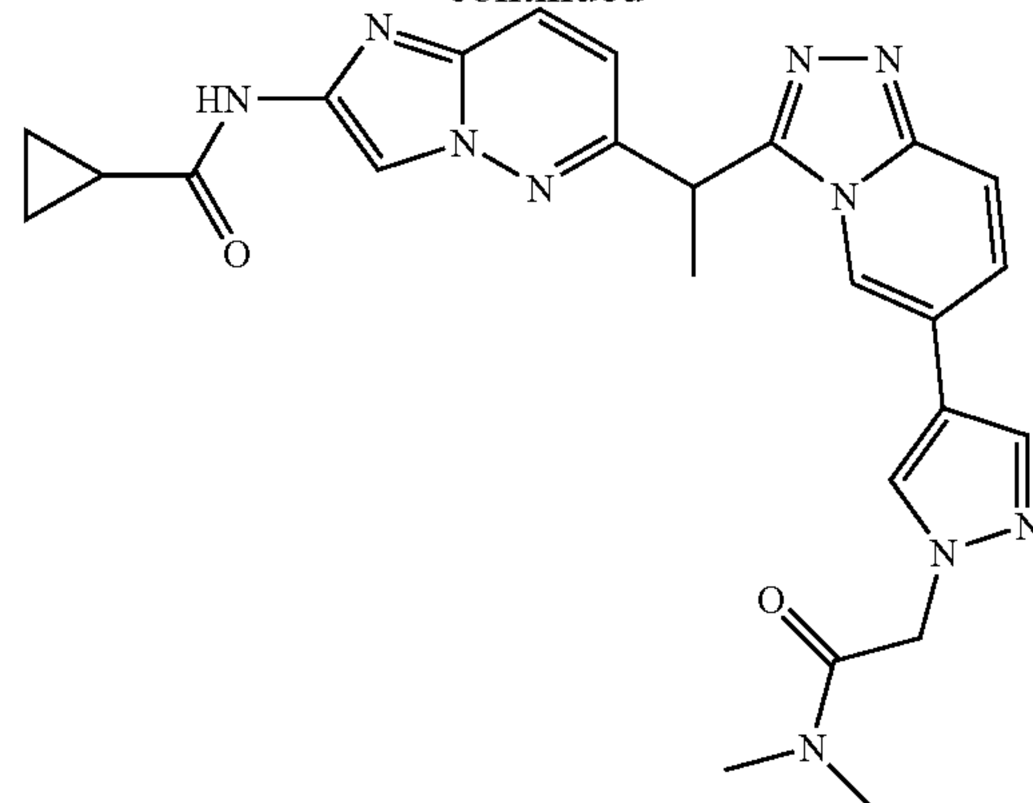
N-(6-(1-(6-(1-(2-(dimethylamino)-2-oxoethyl)-1H-pyrazol-4-yl)-[1,2,4]triazolo[4,3-a]pyridin-3-yl)ethyl)imidazo[1,2-b]pyridazin-2-yl)cyclopropanecarboxamide
