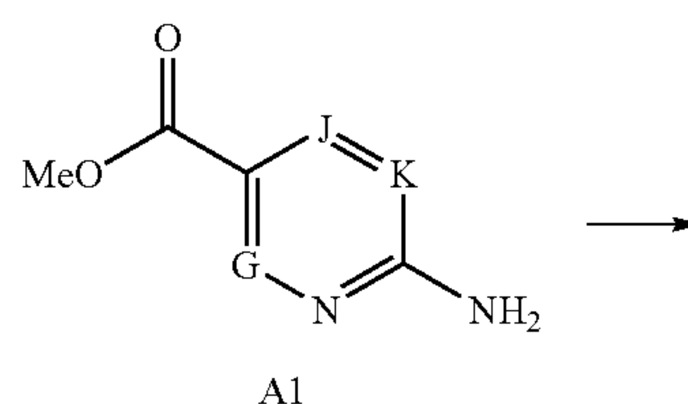
Scheme A
