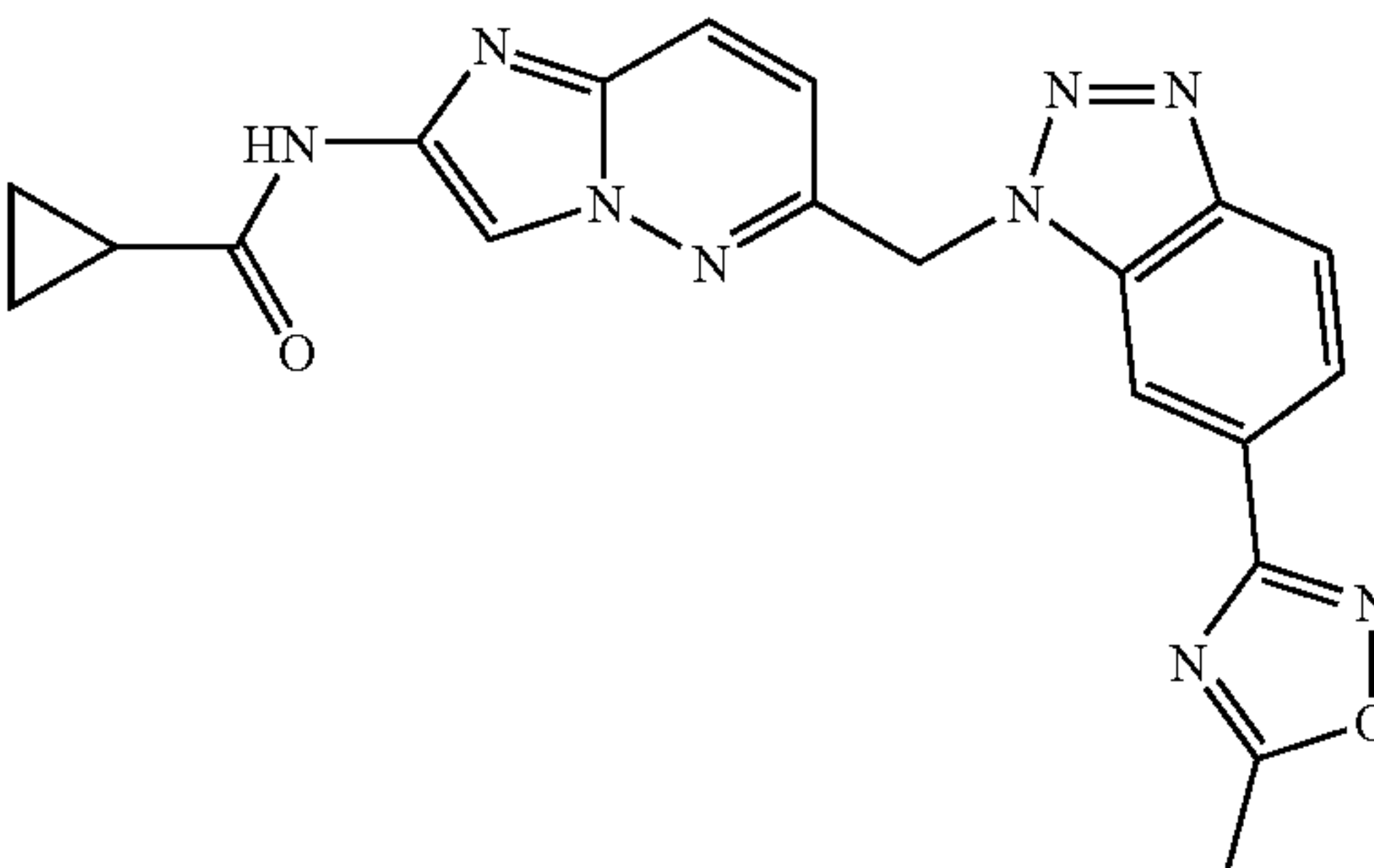
N-(6-((6-(5-methyl-1,2,4-oxadiazol-3-yl)-1H-benzo[d][1,2,3]triazol-1-yl)methyl)imidazo[1,2-b]pyridazin-2-yl)cyclopropanecarboxamide
