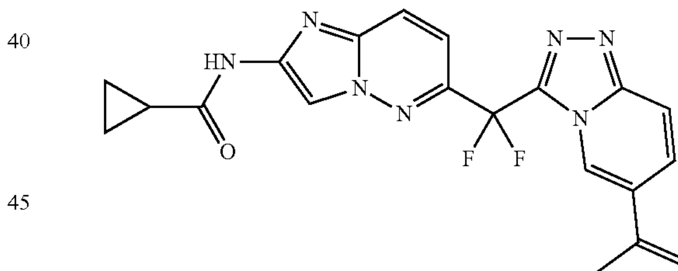
N-(6-(difluoro(6-(prop-1-en-2-yl)-[1,2,4]triazolo[4,3-a]pyridin-3-yl)methyl)imidazo[1,2-b]pyridazin-2-yl)cyclopropanecarboxamide
