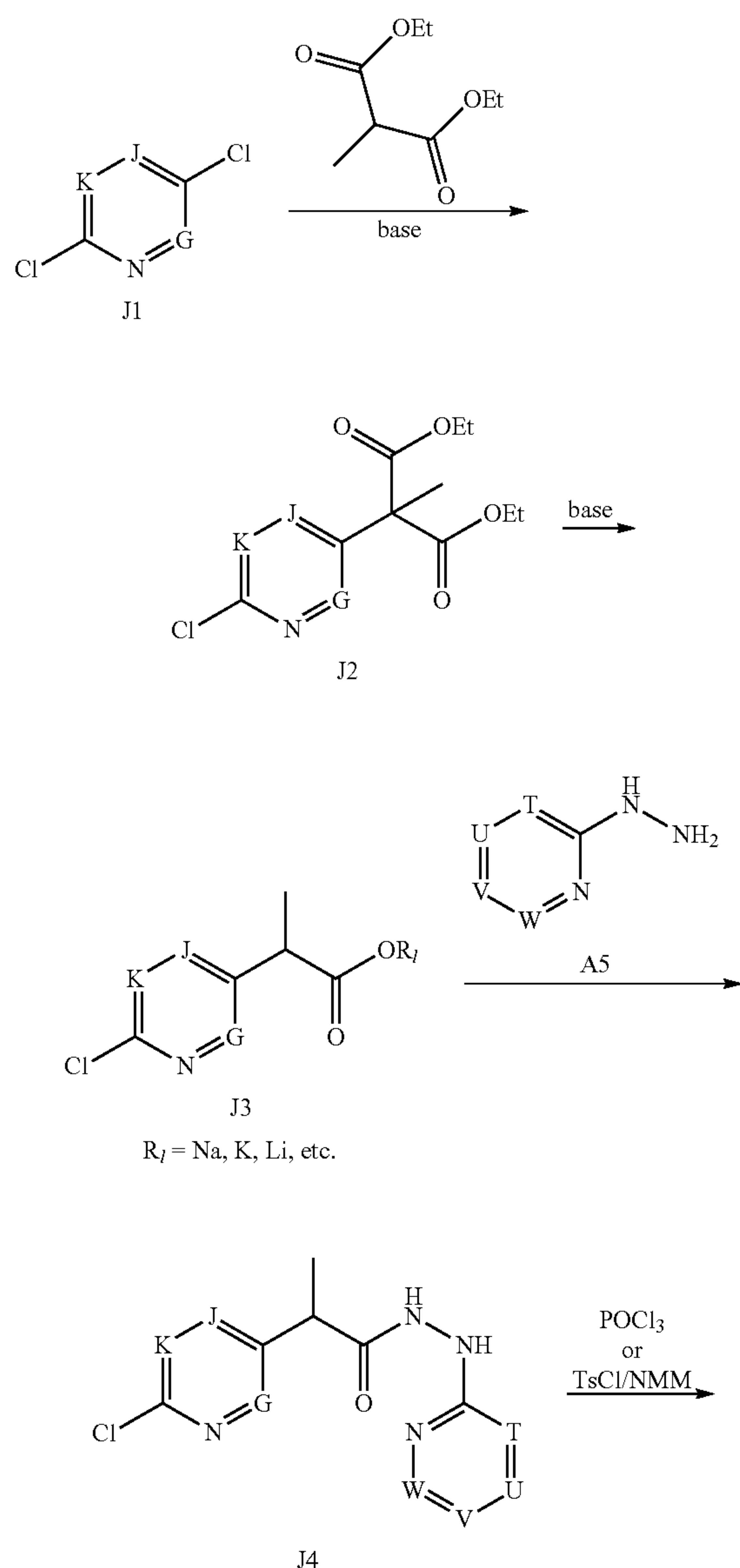
Scheme J
