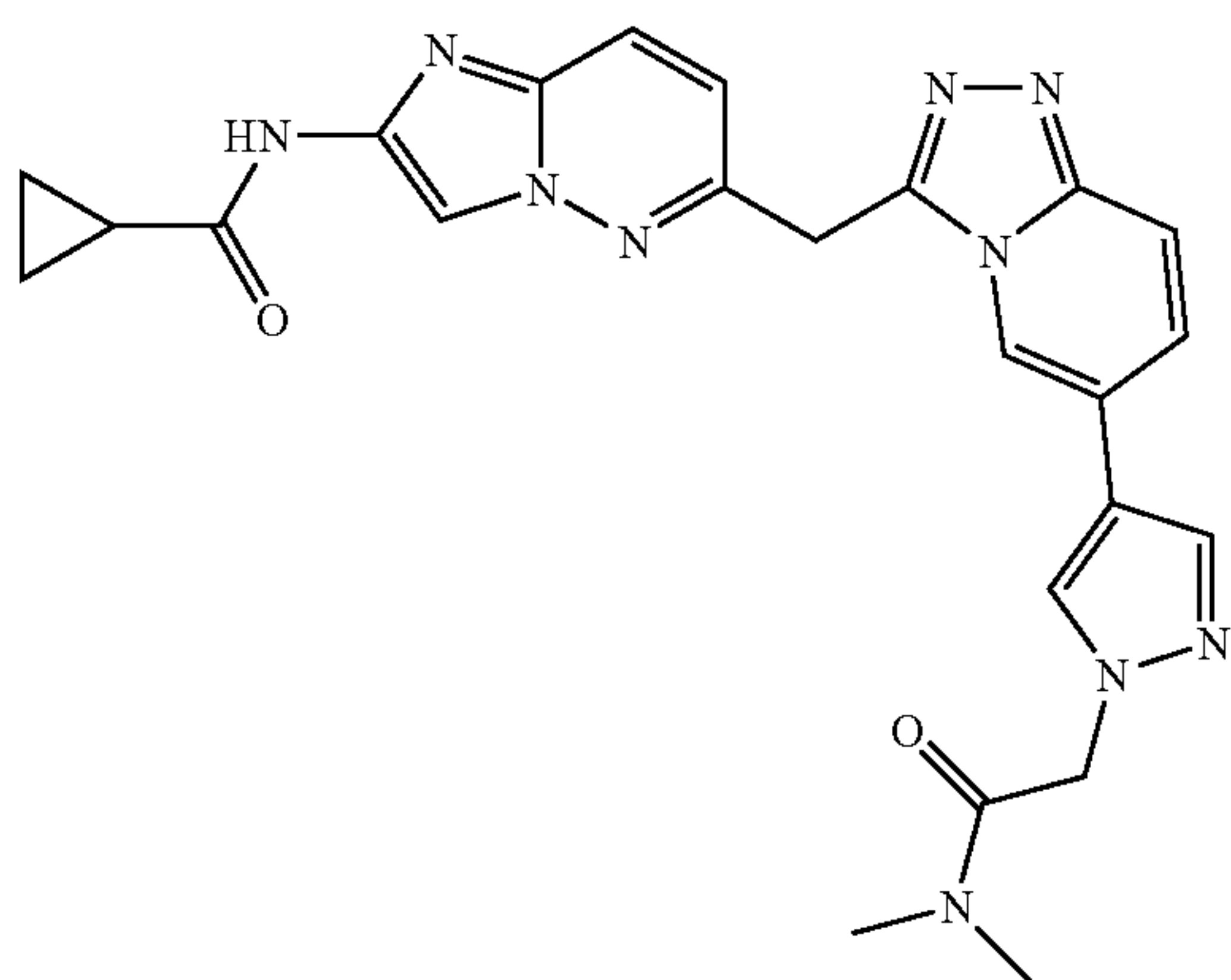
N-(6-((6-(1-(2-(dimethylamino)-2-oxoethyl)-1H-pyrazol-4-yl)-[1,2,4]triazolo[4,3-a]pyridin-3-yl)methyl)imidazo[1,2-b]pyridazin-2-yl)cyclopropanecarboxamide
