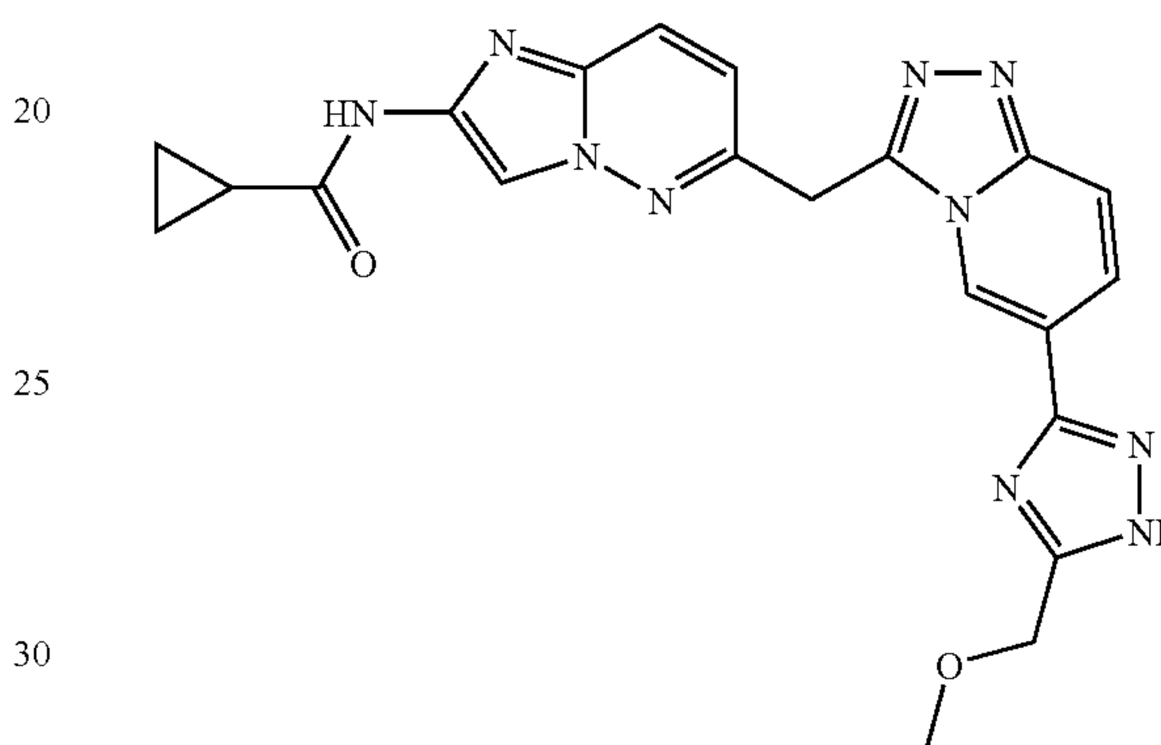
N-((6-((6-(5-(methoxymethyl)-1H-1,2,4-triazol-3-yl)-[1,2,4]triazolo[4,3-a]pyridin-3-yl)methyl)imidazo[1,2-b]pyridazin-2-yl)cyclopropanecarboxamide
