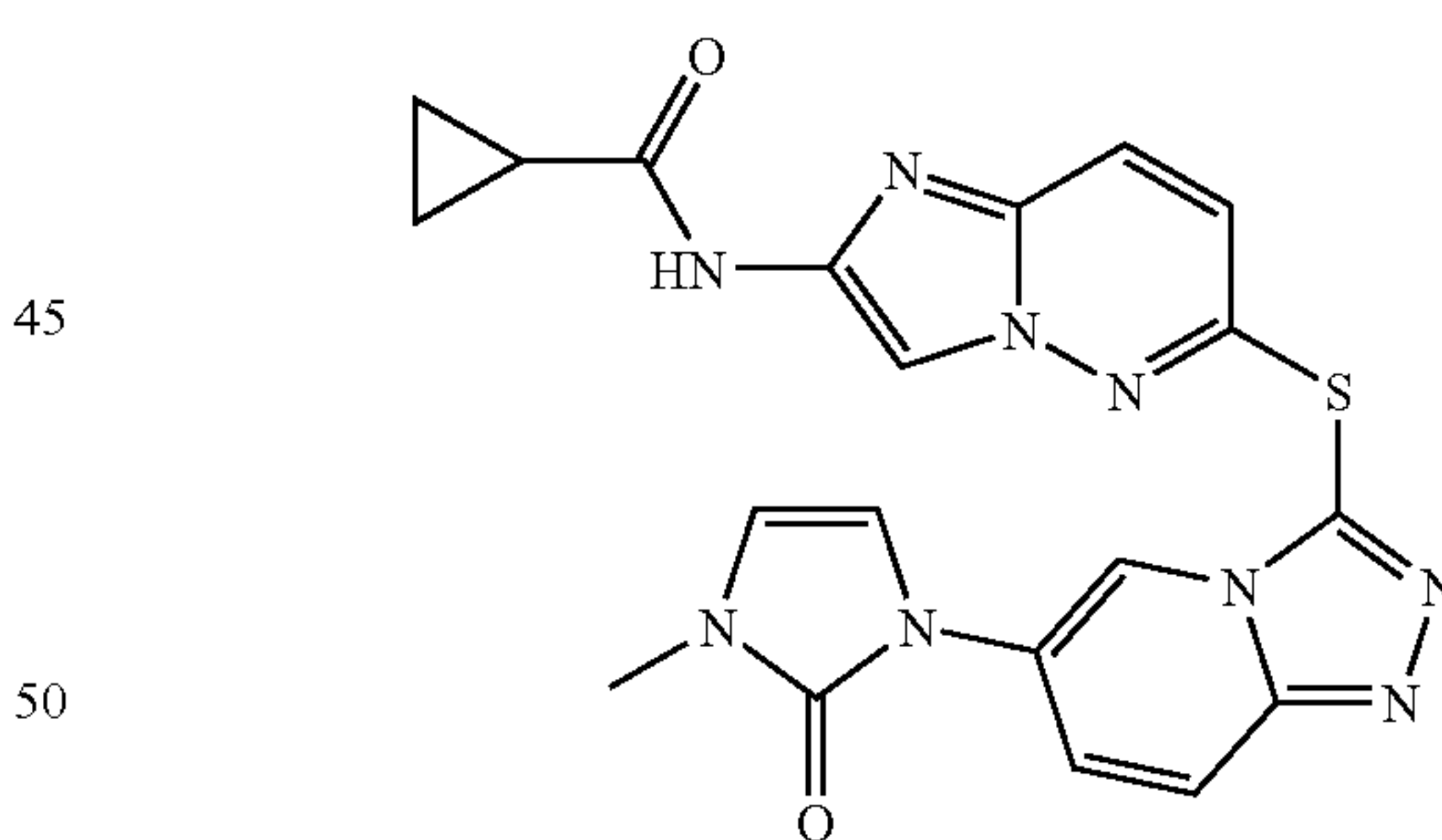
N-(6-(6-(3-methyl-2-oxo-2,3-dihydro-1H-imidazol-1-yl)-[1,2,4]triazolo[4,3-a]pyridin-3-ylthio)imidazo[1,2-b]pyridazin-2-yl)cyclopropanecarboxamide
