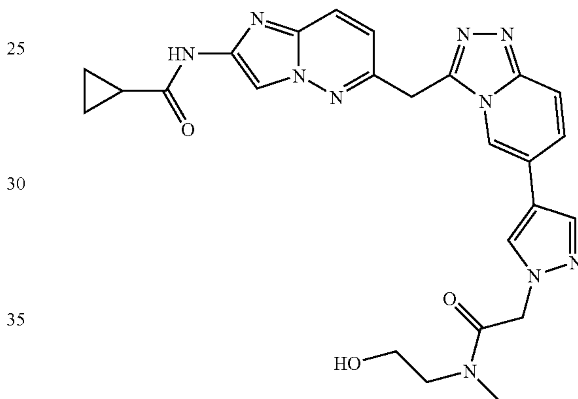
N-(6-((6-(1-(2-((2-hydroxyethyl)(methyl)amino)-2-oxoethyl)-1H-pyrazol-4-yl)-[1,2,4]triazolo[4,3-a]pyridin-3-yl)methyl)imidazo[1,2-b]pyridazin-2-yl)cyclopropanecarboxamide
