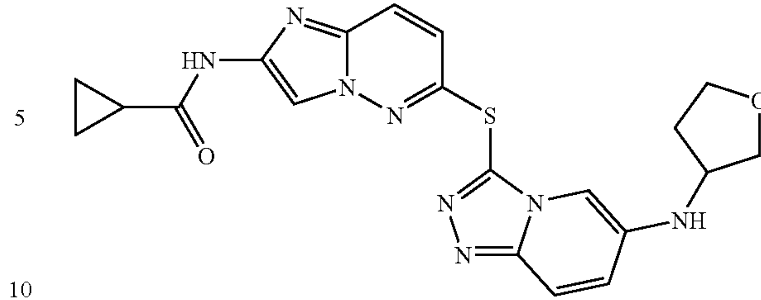
N-(6-(6-(tetrahydrofuran-3-ylamino)-[1,2,4]triazolo[4,3-a]pyridin-3-ylthio)imidazo[1,2-b]pyridazin-2-yl)cyclopropanecarboxamide
