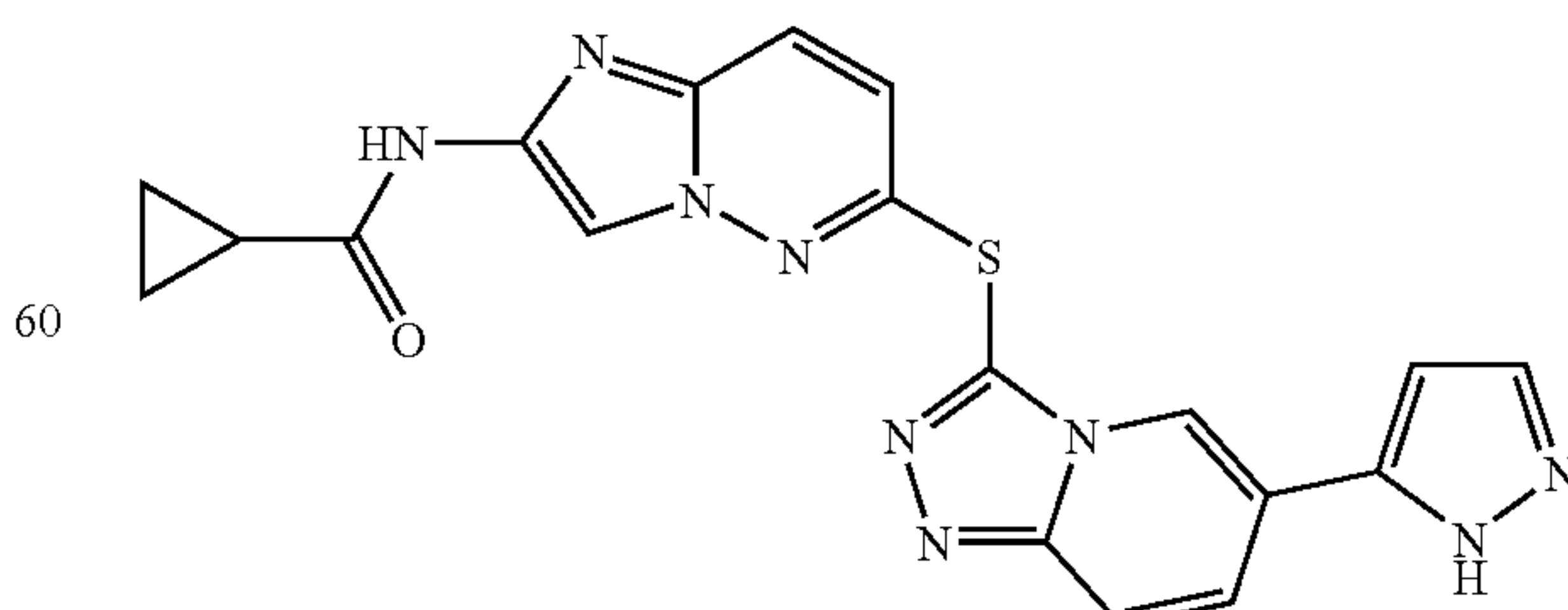
N-(6-(6-(1H-pyrazol-5-yl)-[1,2,4]triazolo[4,3-a]pyridin-3-ylthio)imidazo[1,2-b]pyridazin-2-yl)cyclopropanecarboxamide
