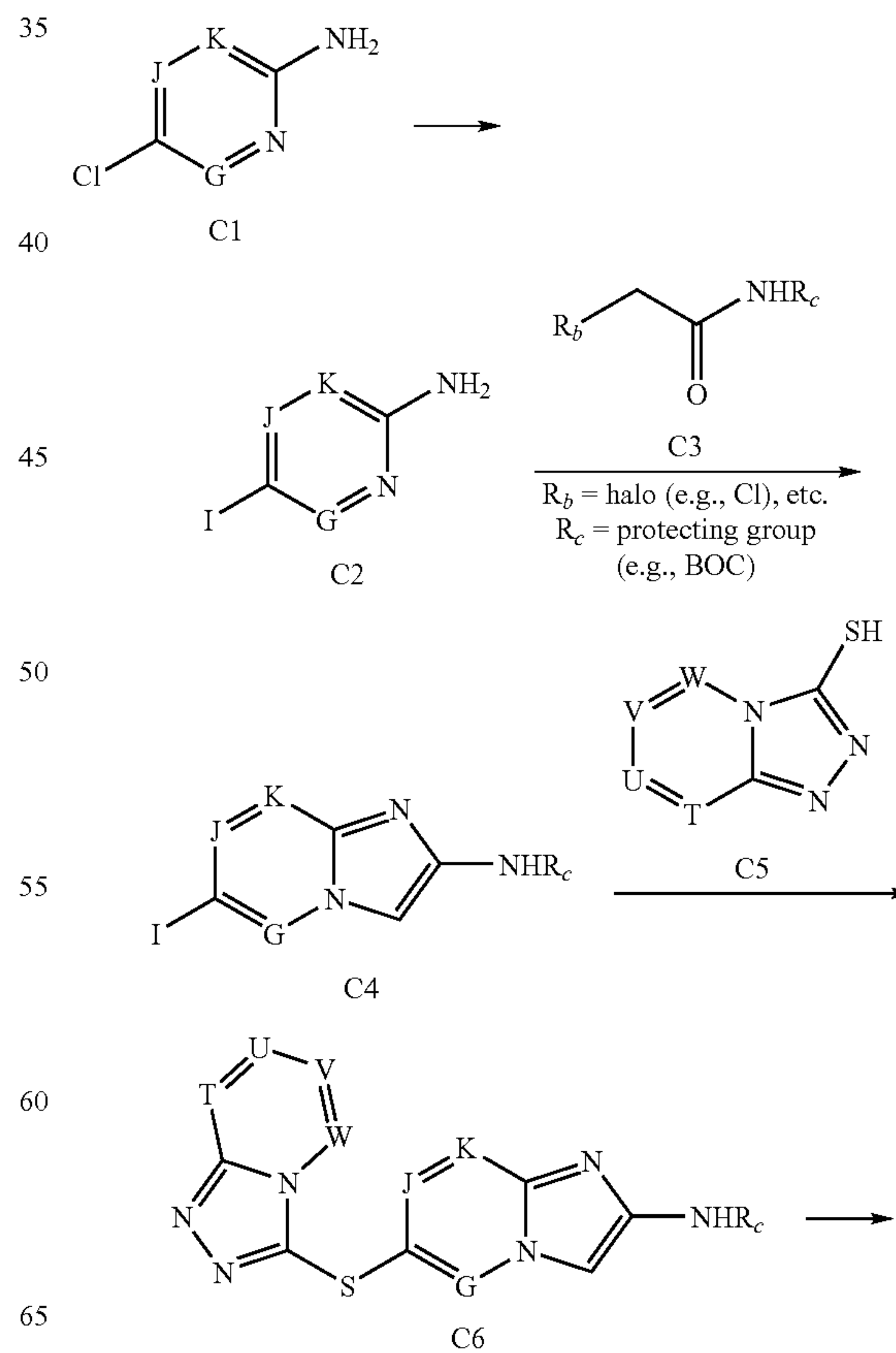
Scheme C
