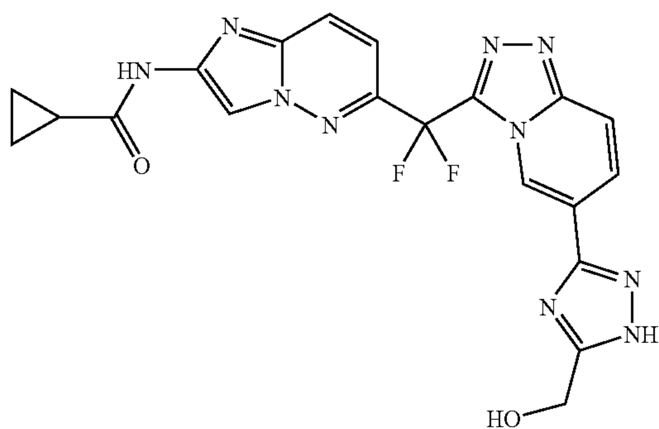
N-(6-(difluoro(6-(5-(hydroxymethyl)-1H-1,2,4-triazol-3-yl)-[1,2,4]triazolo[4,3-a]pyridin-3-yl)methyl)imidazo[1,2-b]pyridazin-2-yl)cyclopropanecarboxamide
