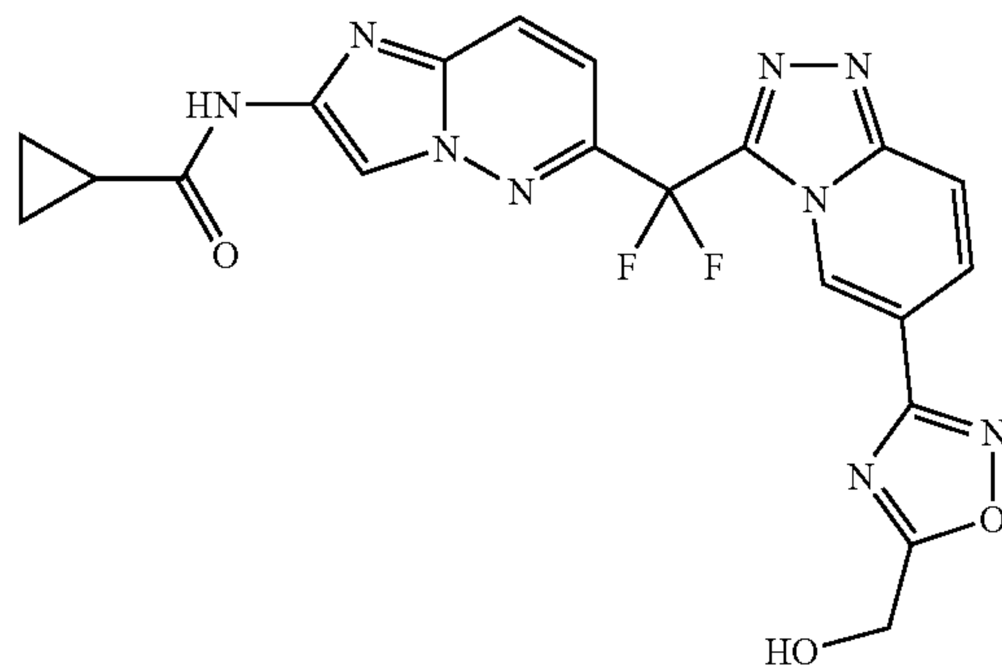
N-(6-(difluoro(6-(5-(hydroxymethyl)-1,2,4-oxadiazol-3-yl)-[1,2,4]triazolo[4,3-a]pyridin-3-yl)methyl)imidazo[1,2-b]pyridazin-2-yl)cyclopropanecarboxamide
