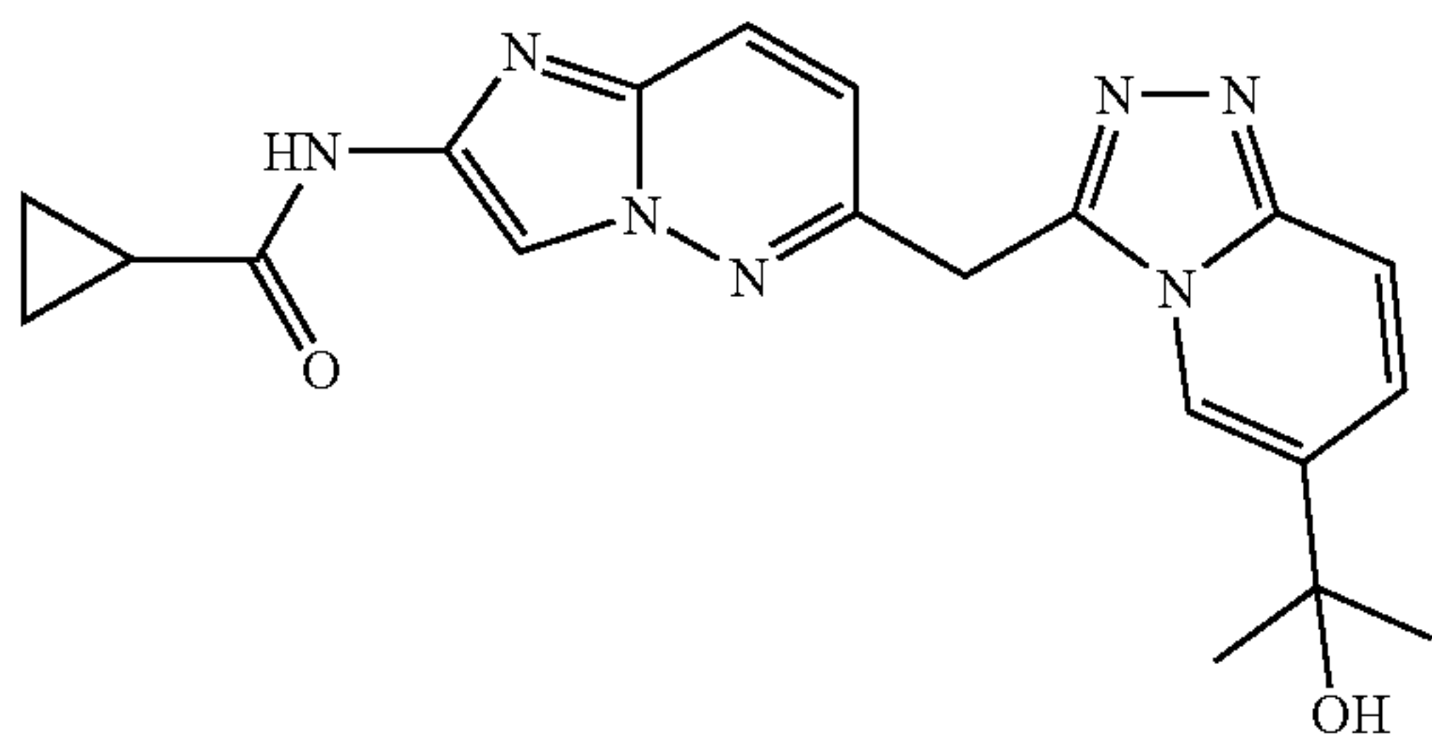
N-((6-((6-(2-hydroxypropan-2-yl)-[1,2,4]triazolo[4,3-a]pyridin-3-yl)methyl)imidazo[1,2-b]pyridazin-2-yl)cyclopropanecarboxamide
