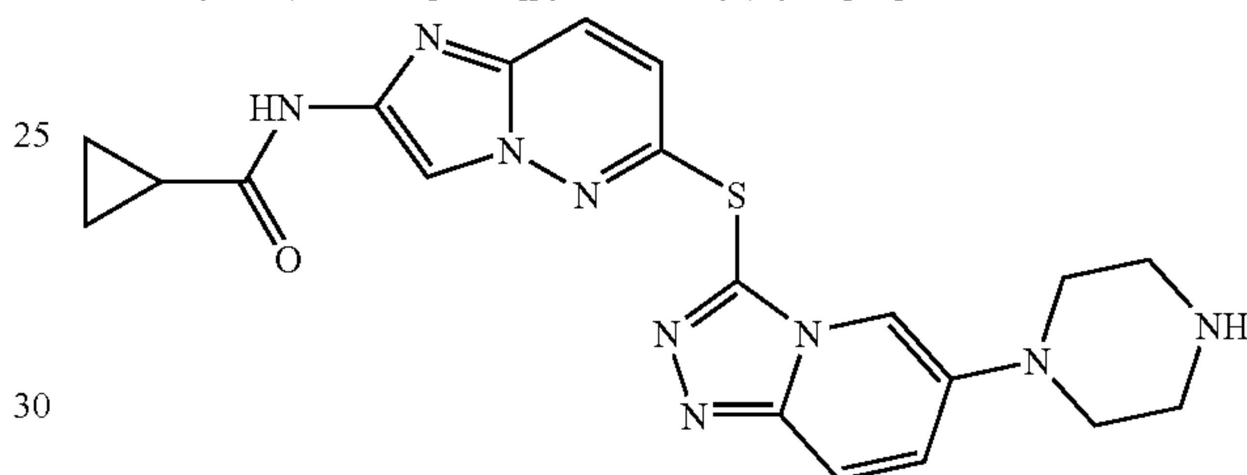
N-(6-(6-(piperazin-1-yl)-[1,2,4]triazolo[4,3-a]pyridin-3-ylthio)imidazo[1,2-b]pyridazin-2-yl)cyclopropanecarboxamide
