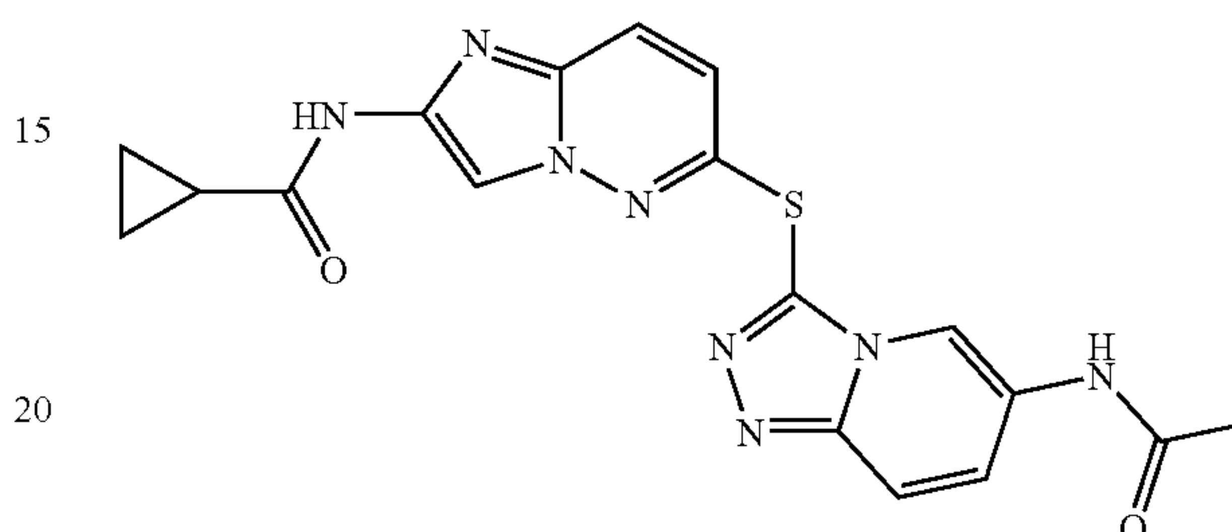
N-(6-(6-(acetamido)-[1,2,4]triazolo[4,3-a]pyridin-3-ylthio)imidazo[1,2-b]pyridazin-2-yl)cyclopropanecarboxamide
