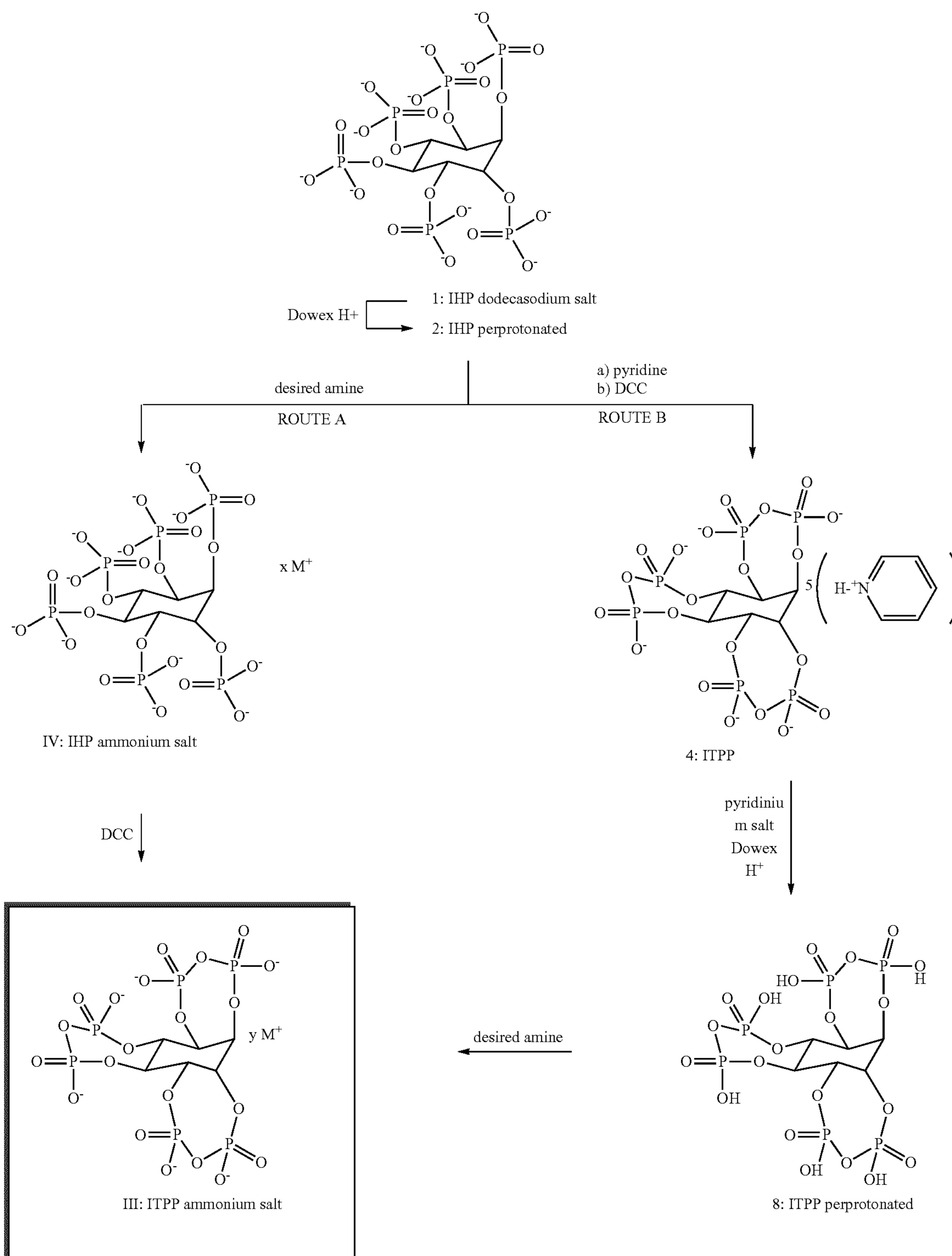
Scheme 6. General routes for the synthesis of ITTP ammonium salts.
