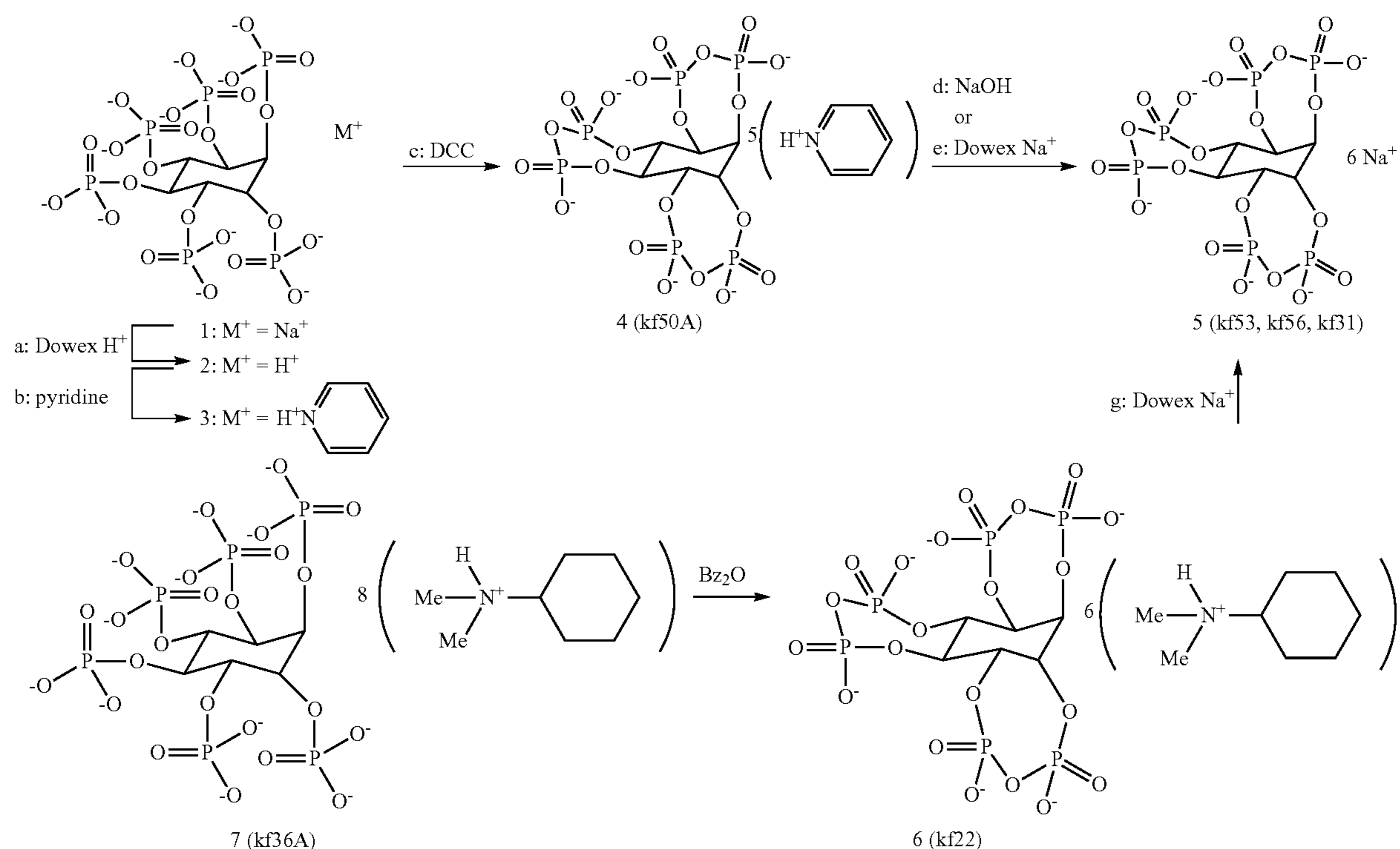
Scheme 3. The ITPP Na salts formation
