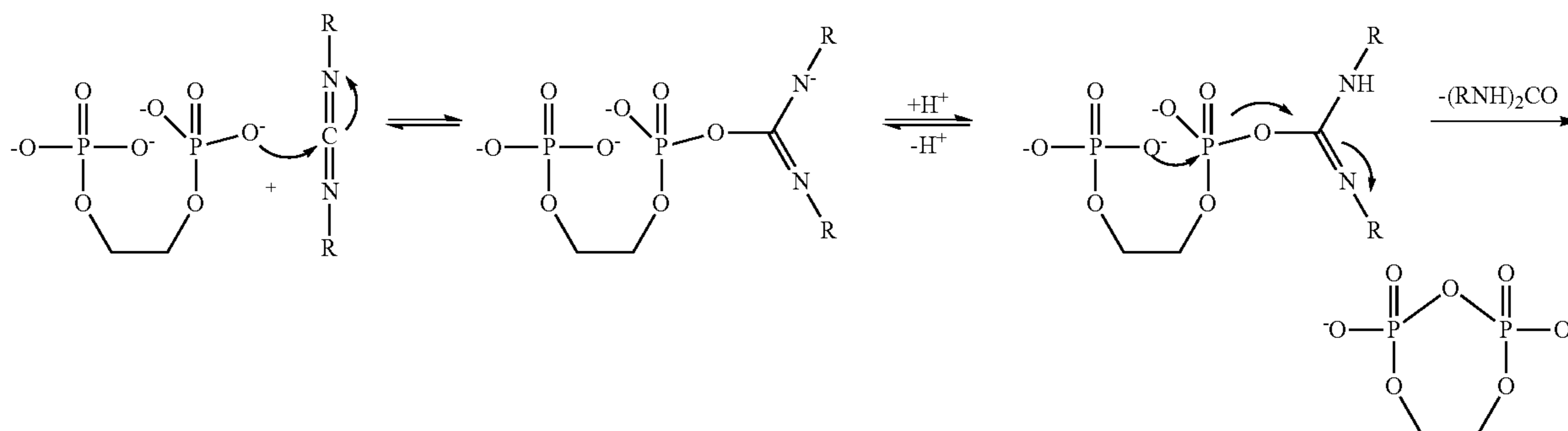
Scheme 4. Mechanistic pathways of the formation of pyrophosphates through a reaction with DCC.
