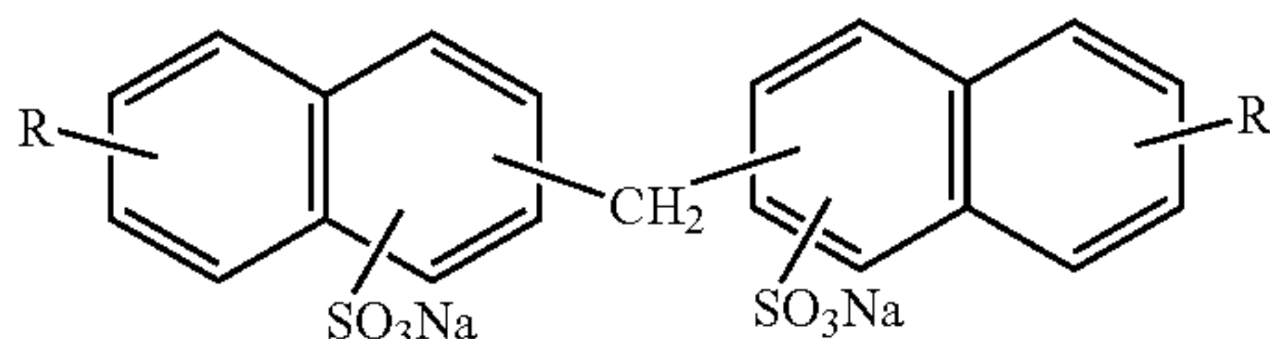
Chemical formula 5
