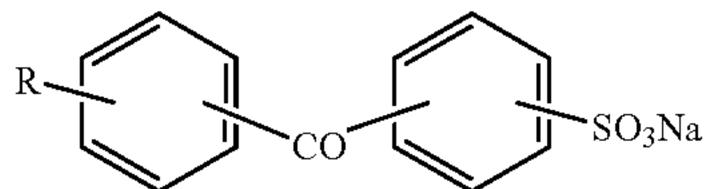
Chemical formula 5
