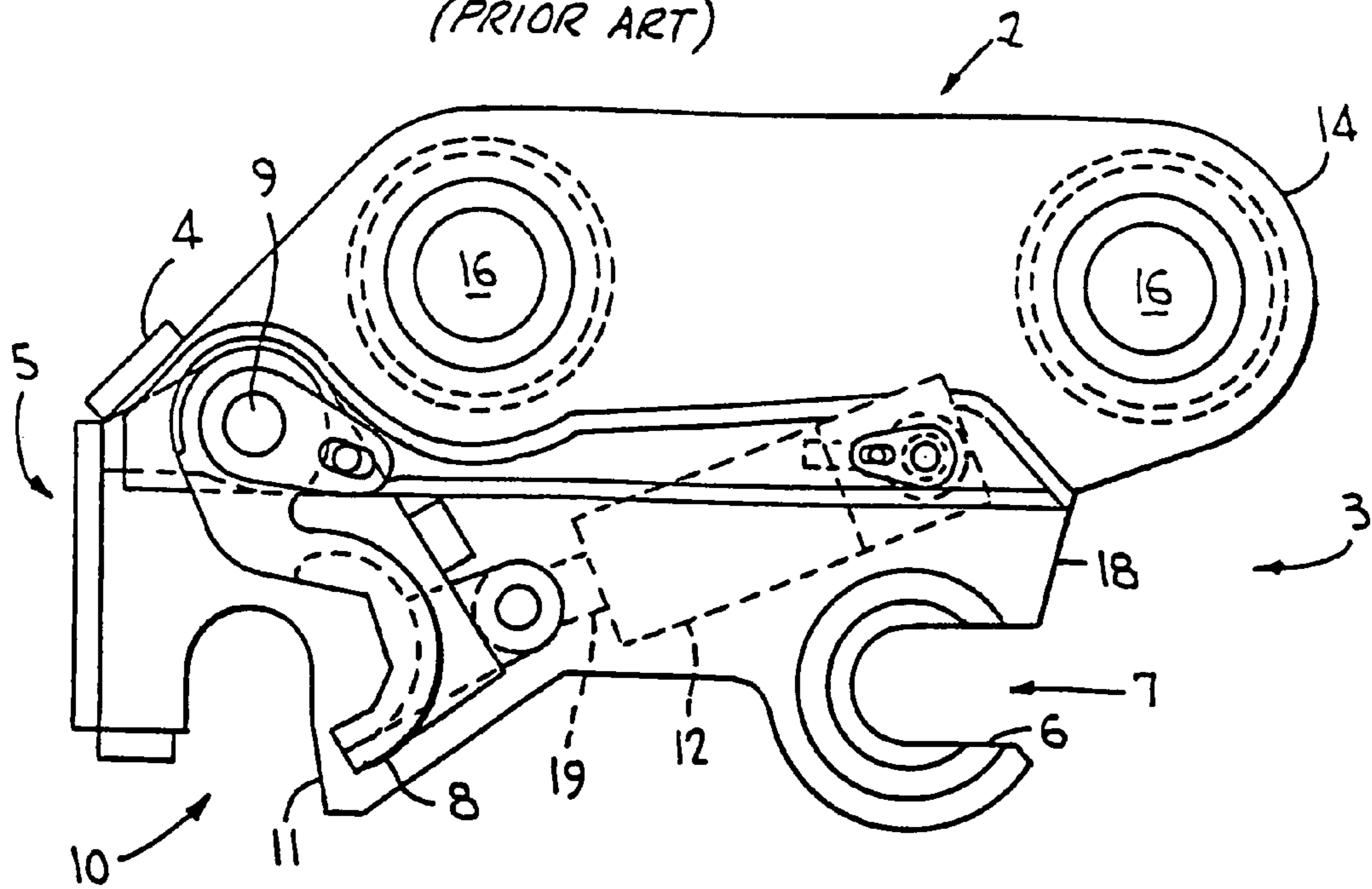
FIG. 2 (PRIOR ART)
