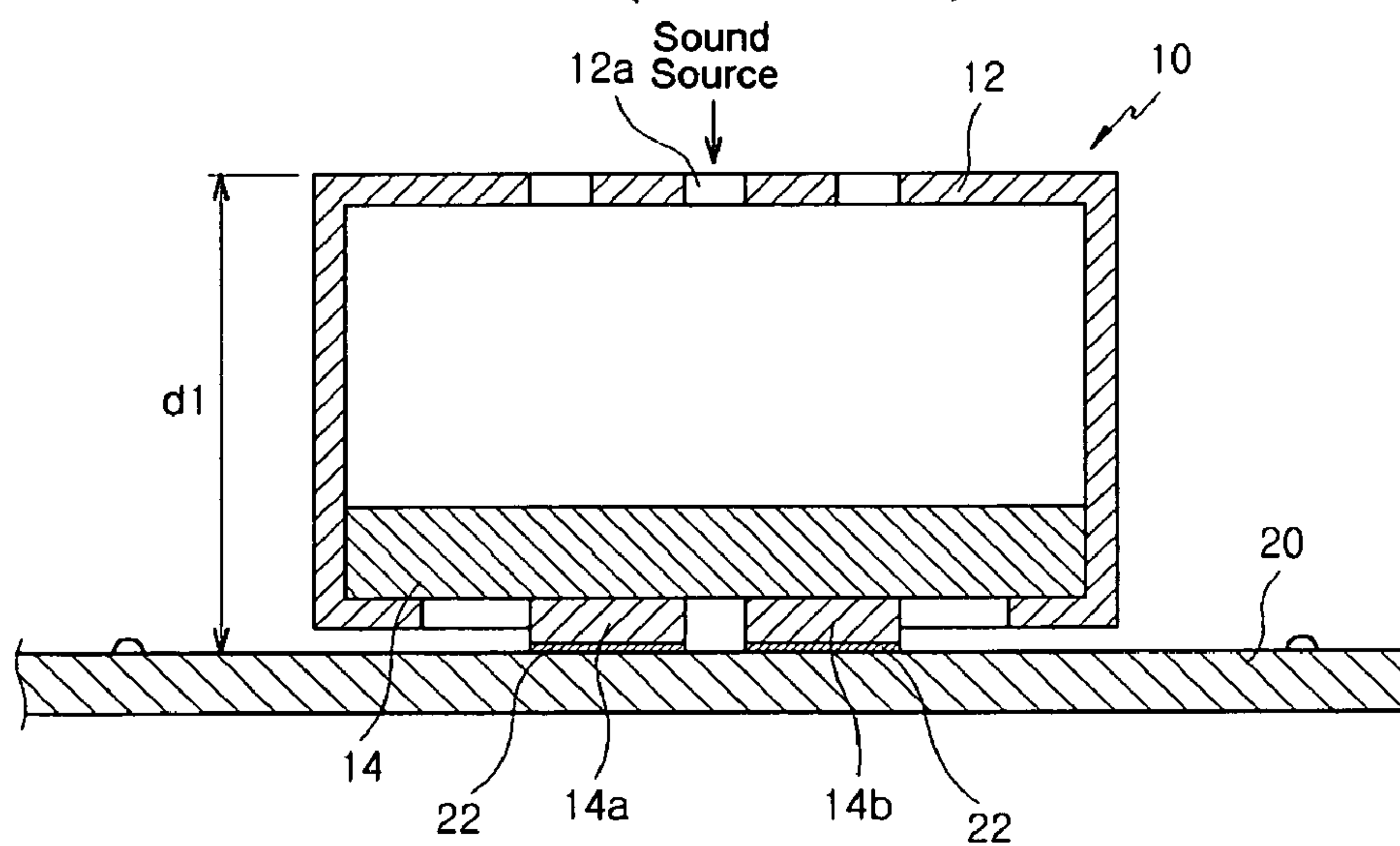
FIG 2 (PRIOR ART)
