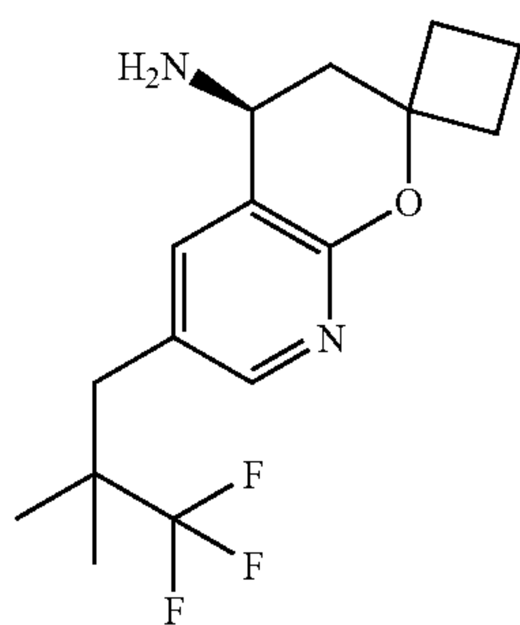
(4S)-6-(2',2'-Dimethyl-3',3',3'-trifluoro-propyl)-2,2-spirocyclobutyl-3,4-dihydro-2H-pyrano[2,3-b]pyridin-4-amine
