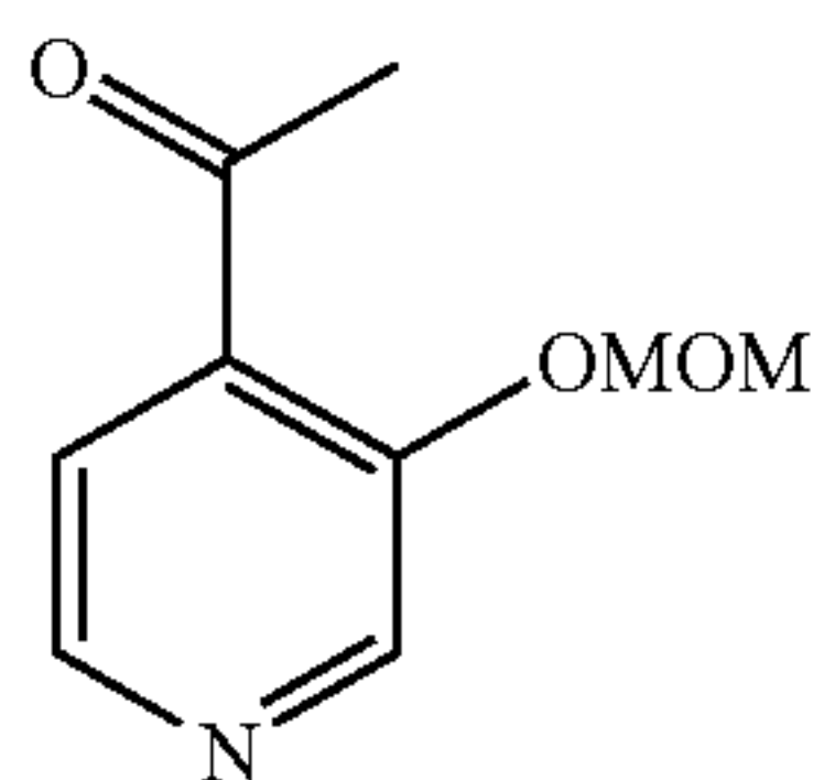
1-(3-(Methoxymethoxy)pyridin-4-yl)ethanone
