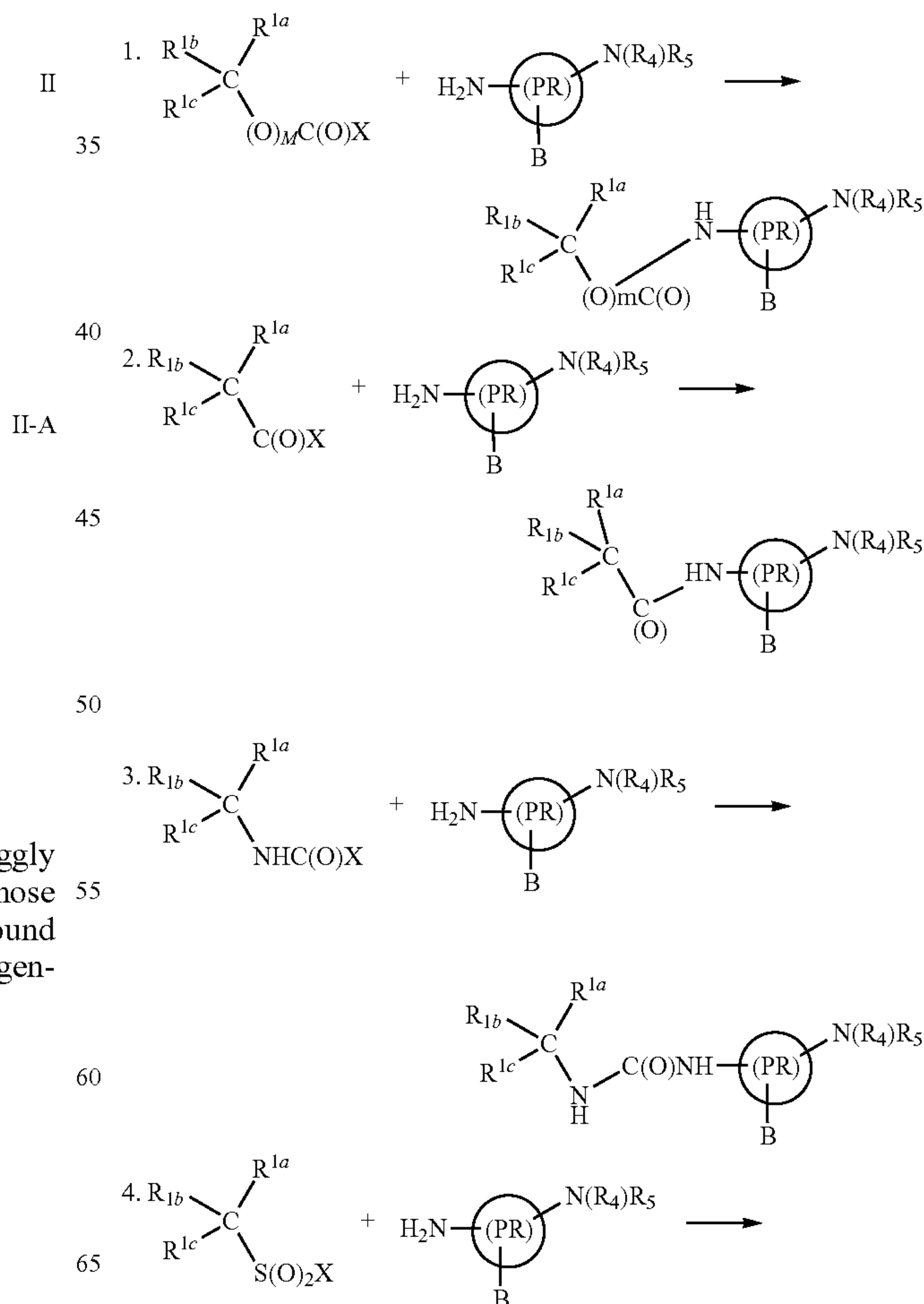
Scheme 2
