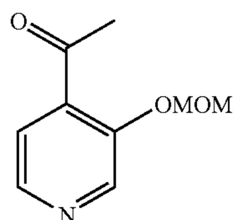
1-(3-(Methoxymethoxy)pyridin-4-yl)ethanone
