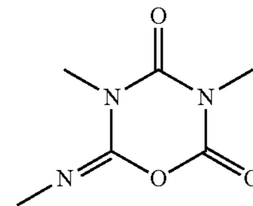
iminooxadiazinedione ring
