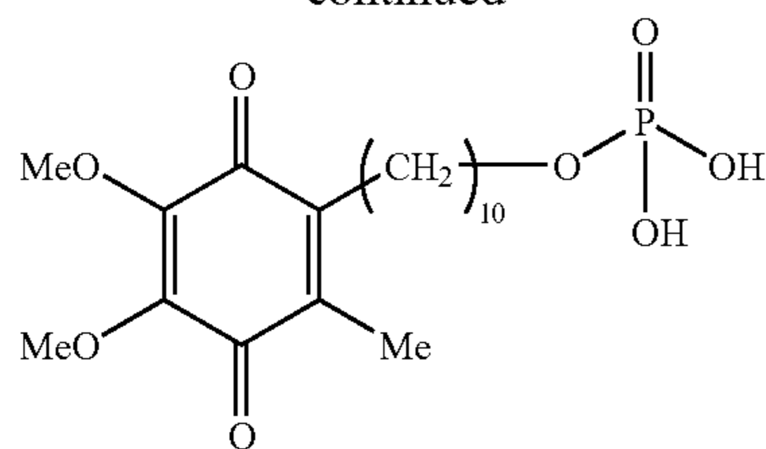
(idebenone phosphate ester)
