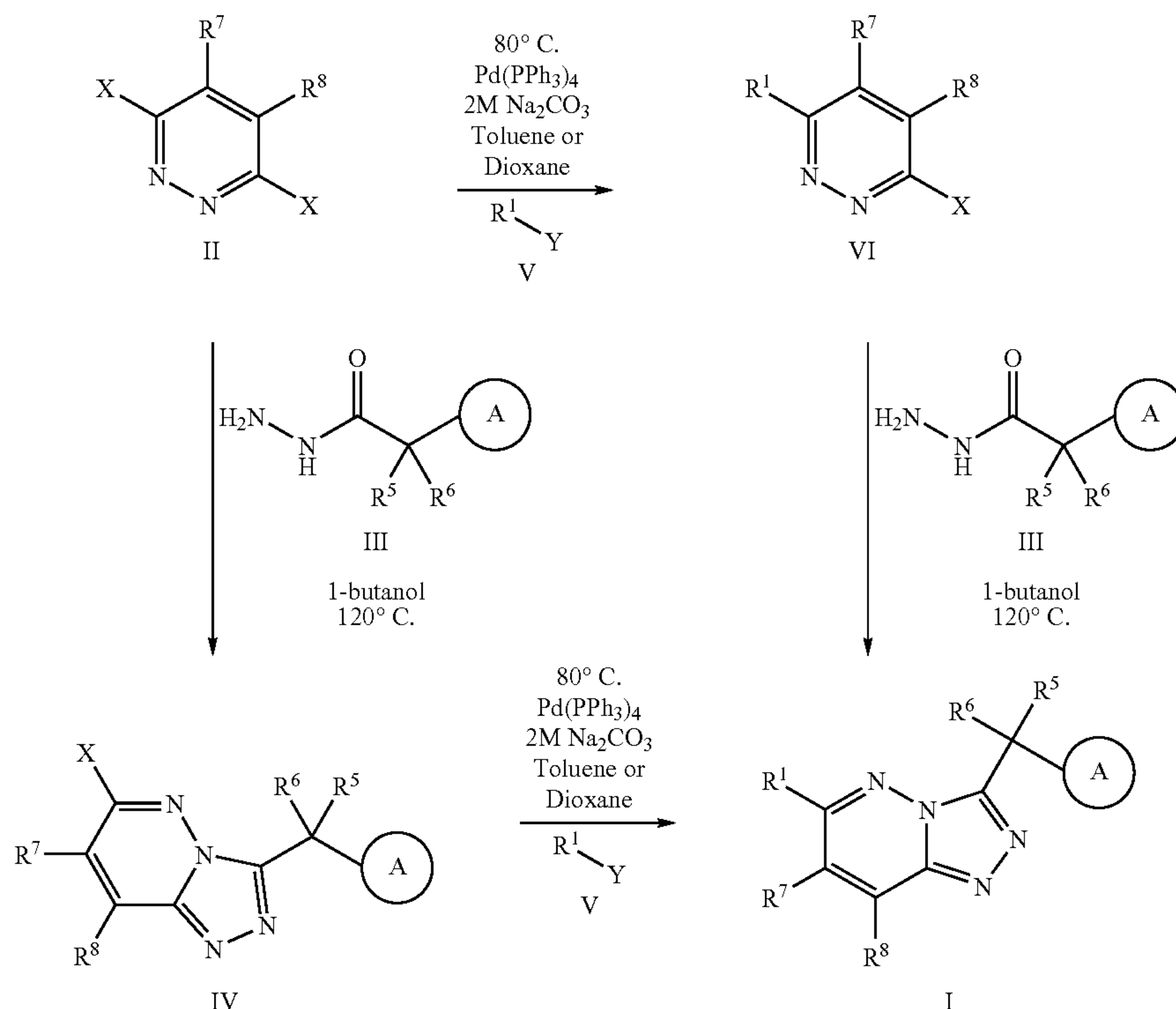
Scheme 1
