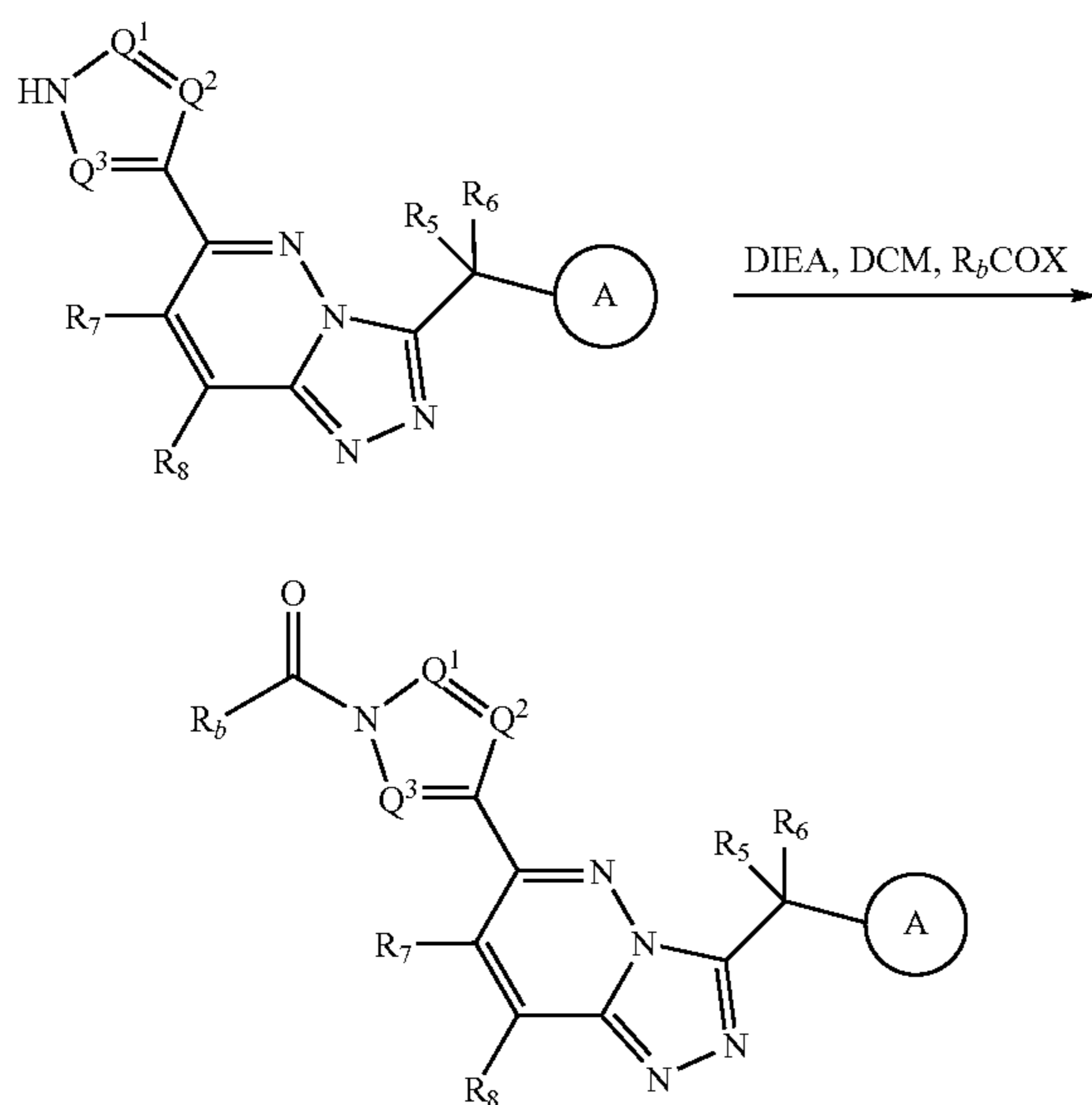
Scheme 5c
