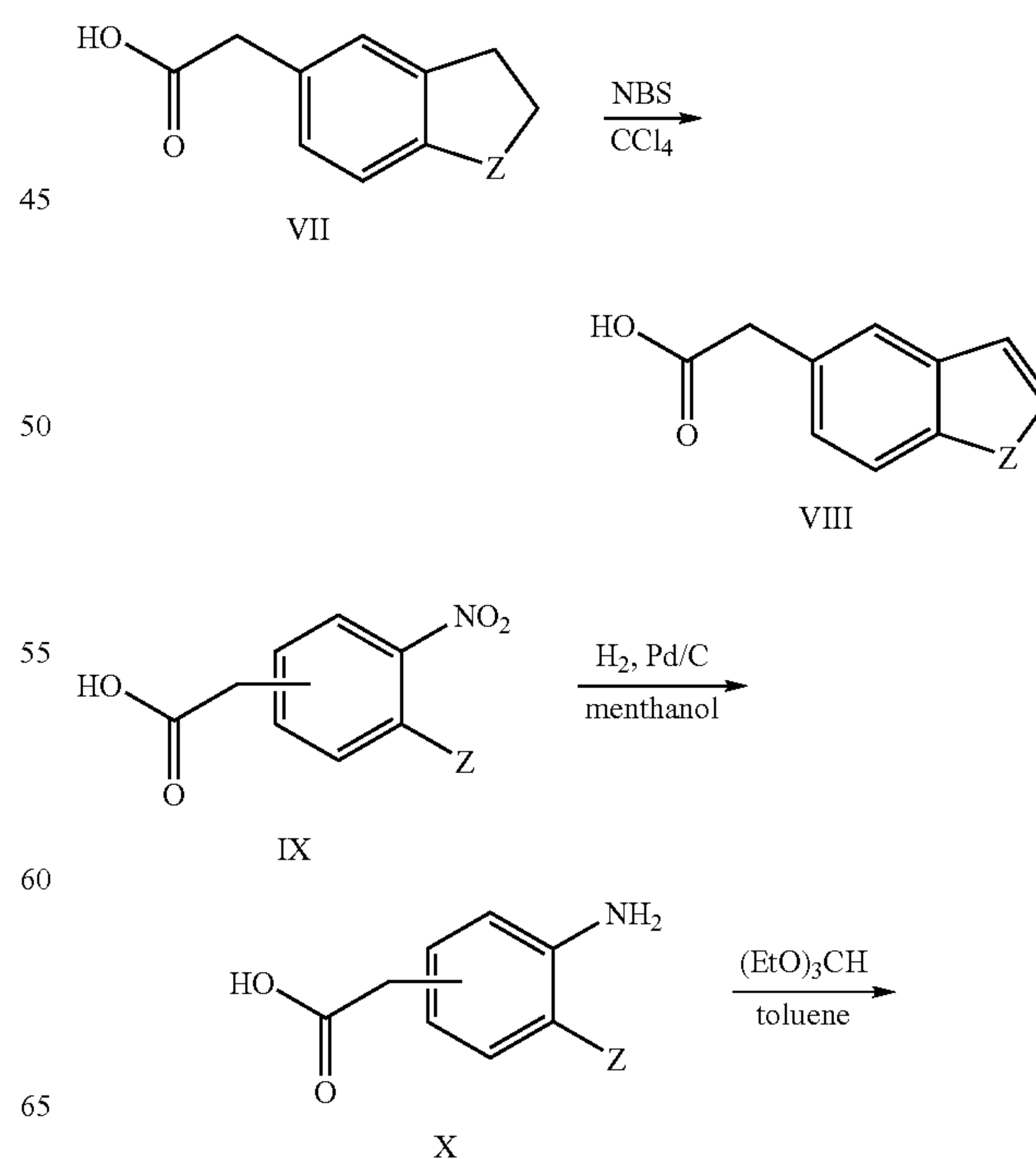
Scheme 2
