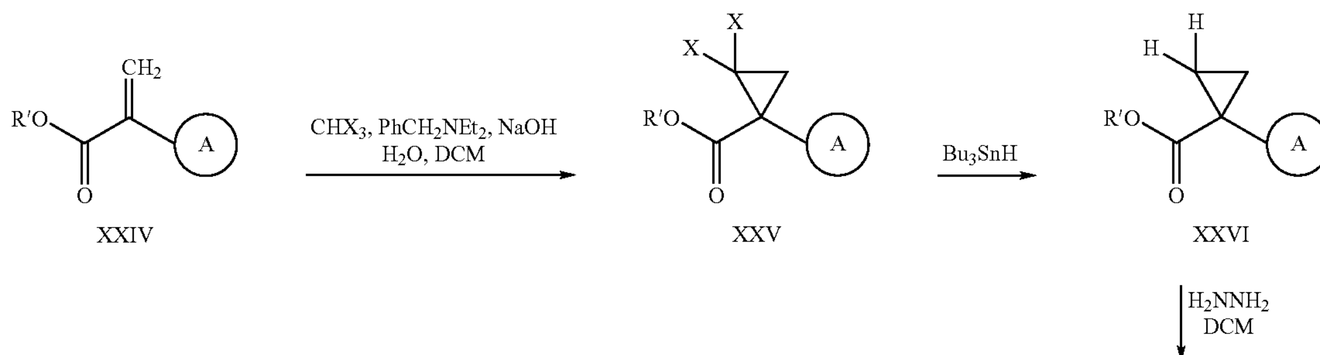
Scheme 4c
