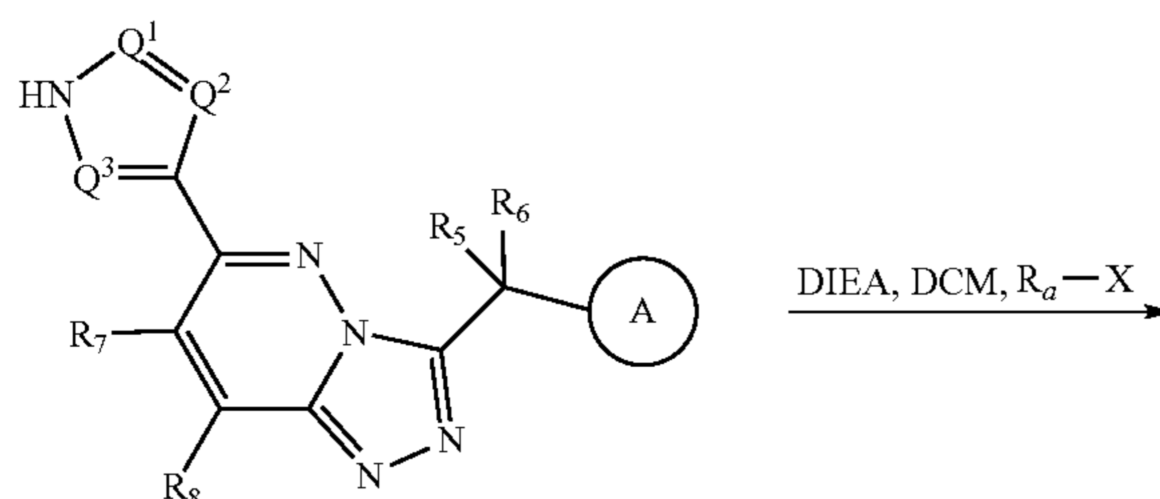
Scheme 5d
