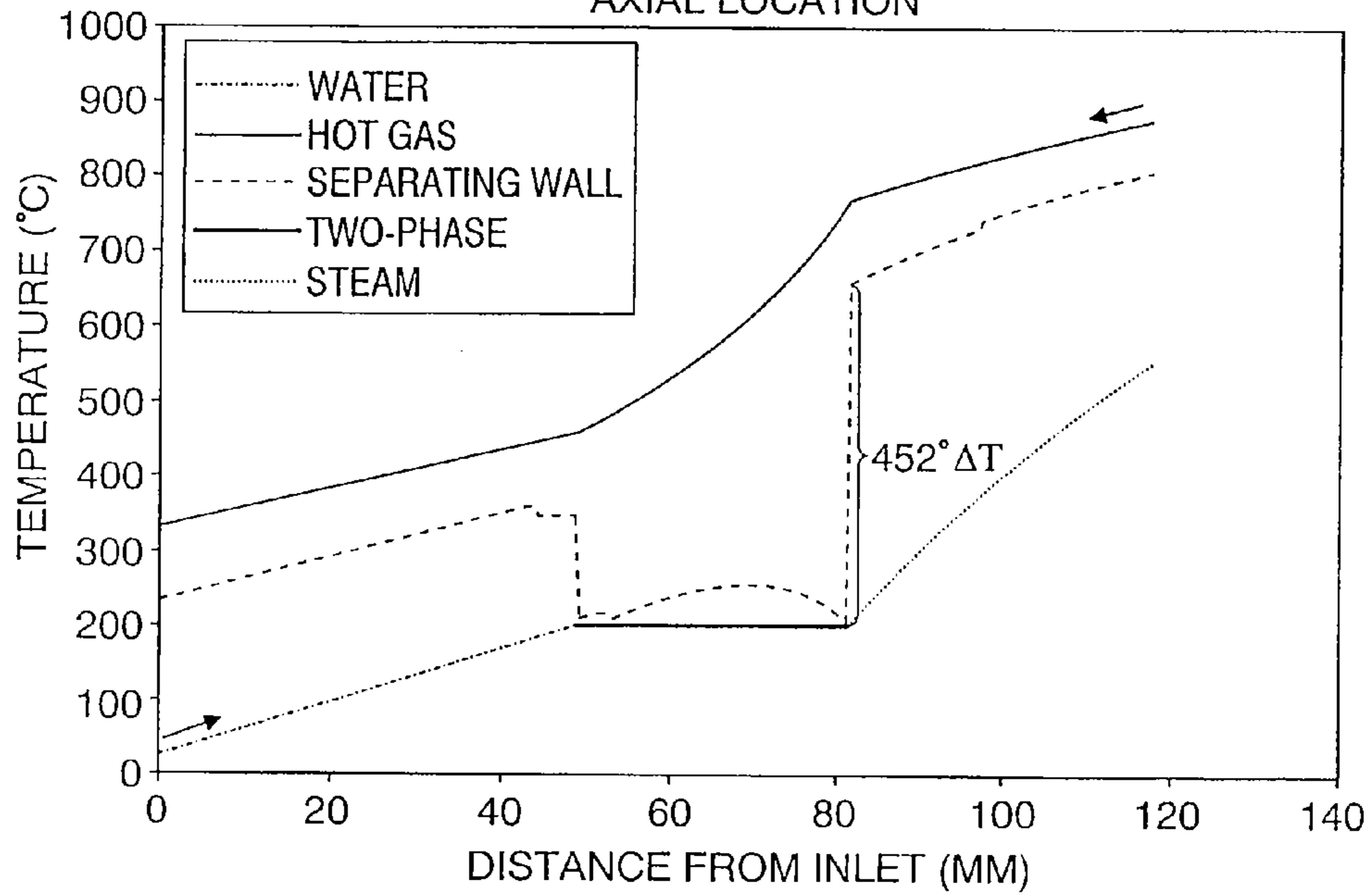
COUNTERFLOW VAPORIZER - TEMPERATURE VS. AXIAL LOCATION
