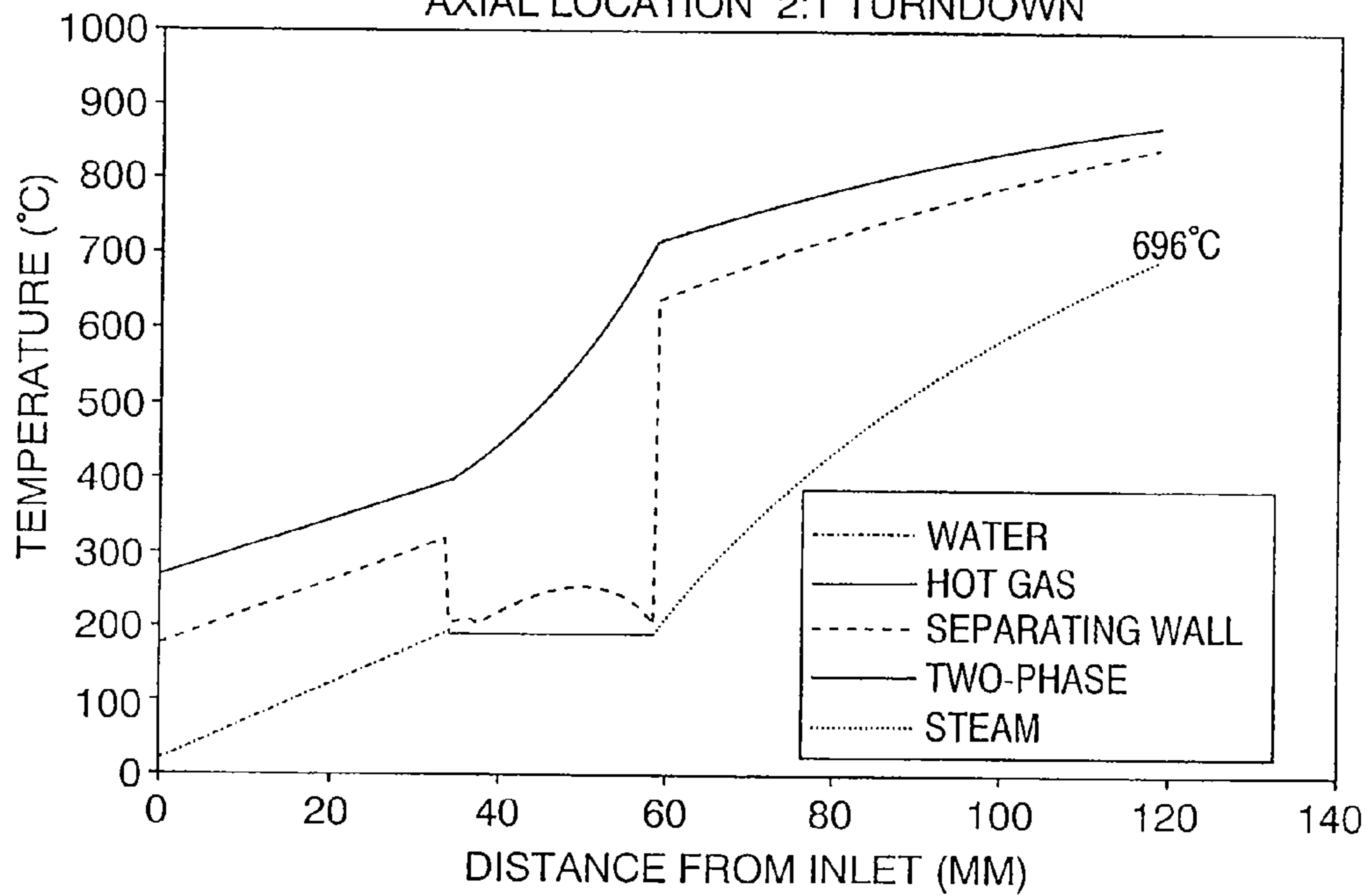
COUNTERFLOW VAPORIZER - TEMPERATURE VS. AXIAL LOCATION 2:1 TURNDOWN
