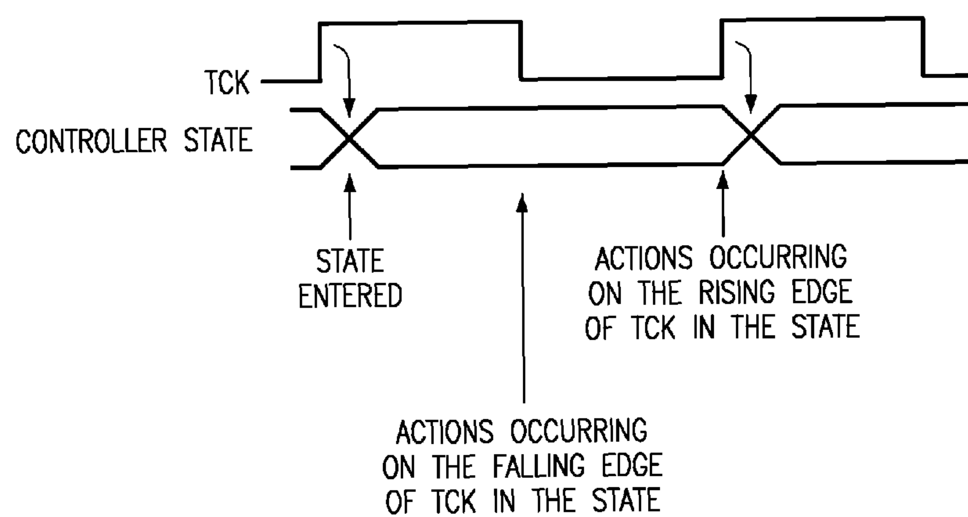
FIG. 15 (PRIOR ART)
