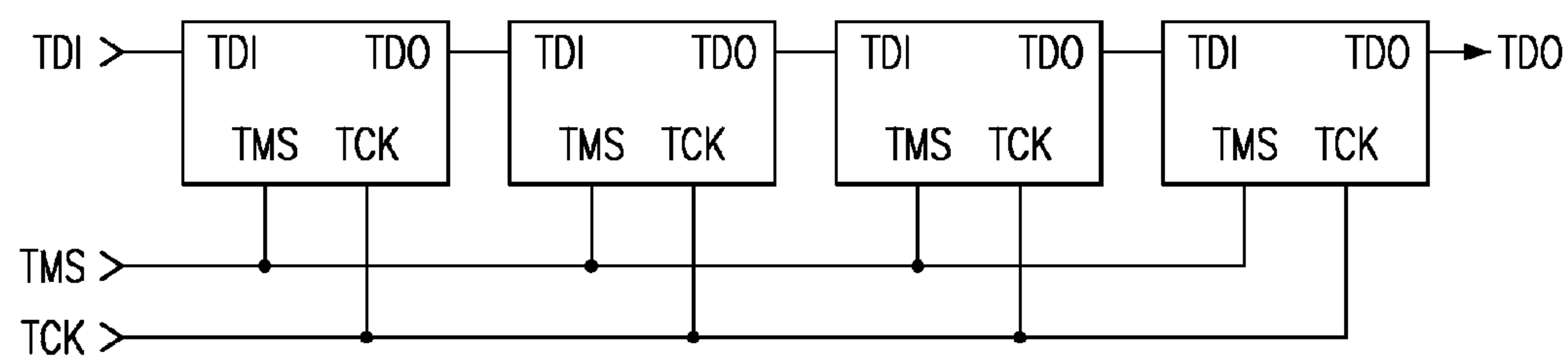
FIG. 13 (PRIOR ART)
