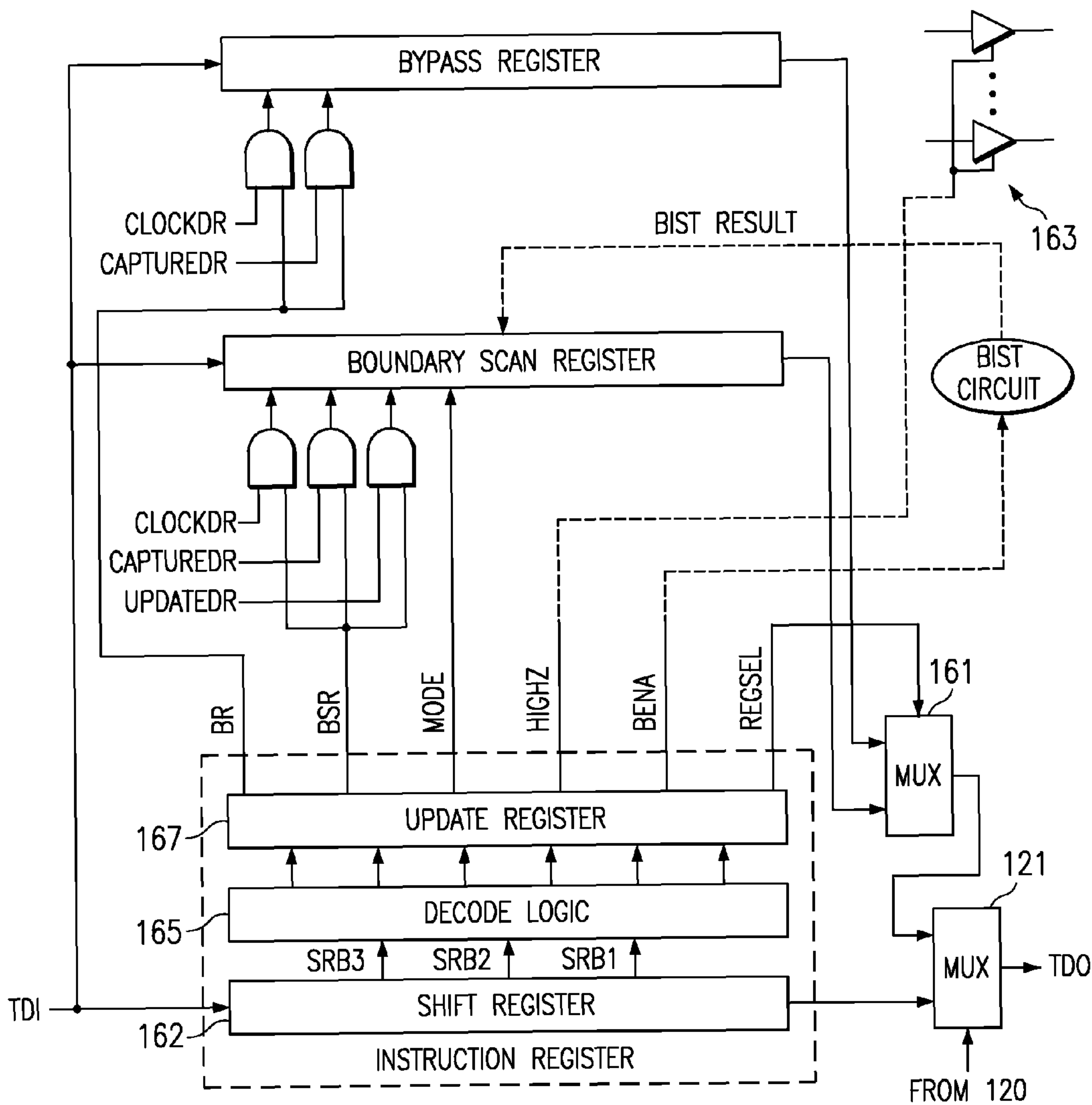
FIG. 16 (PRIOR ART)
