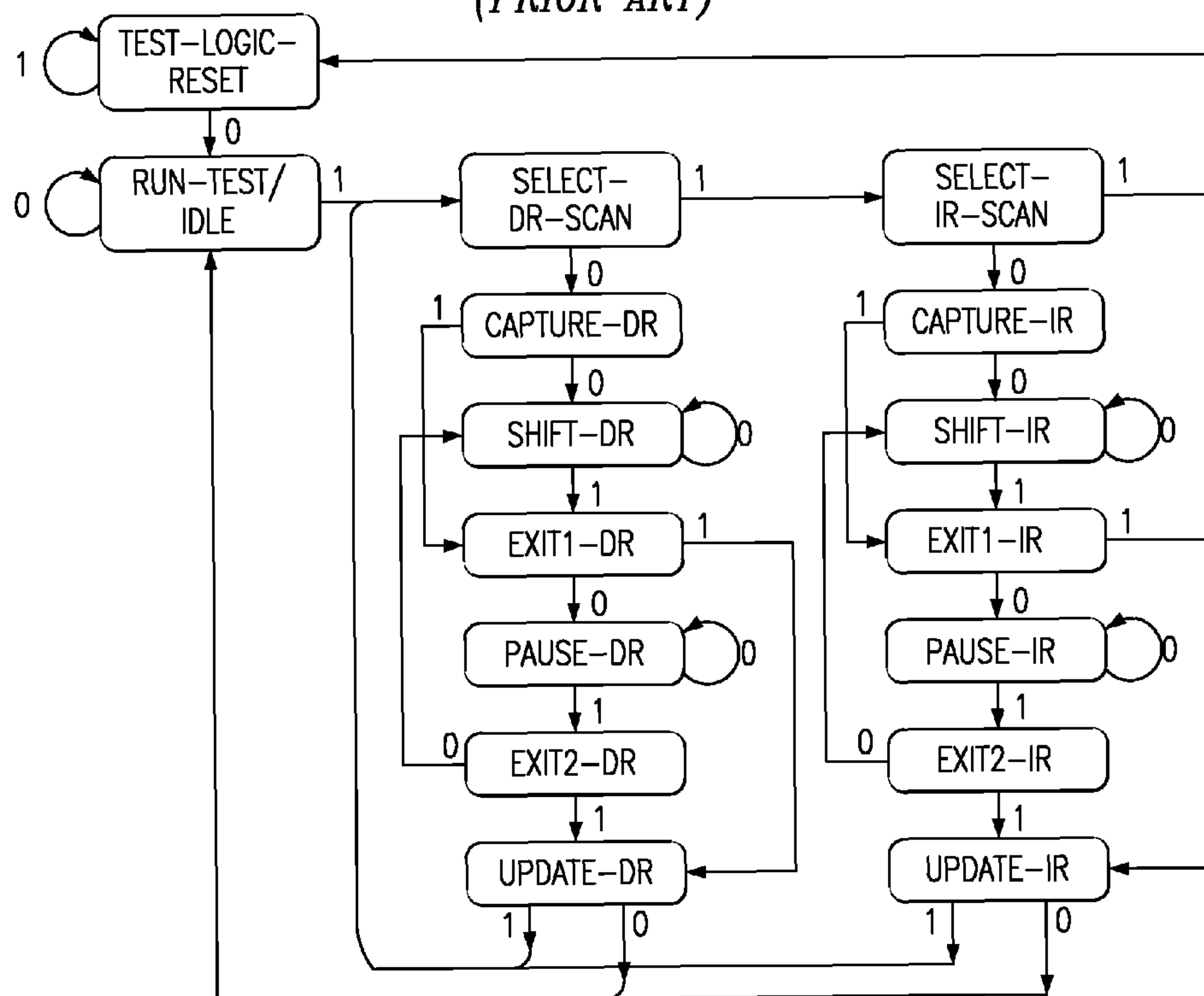
FIG. 14 (PRIOR ART)
