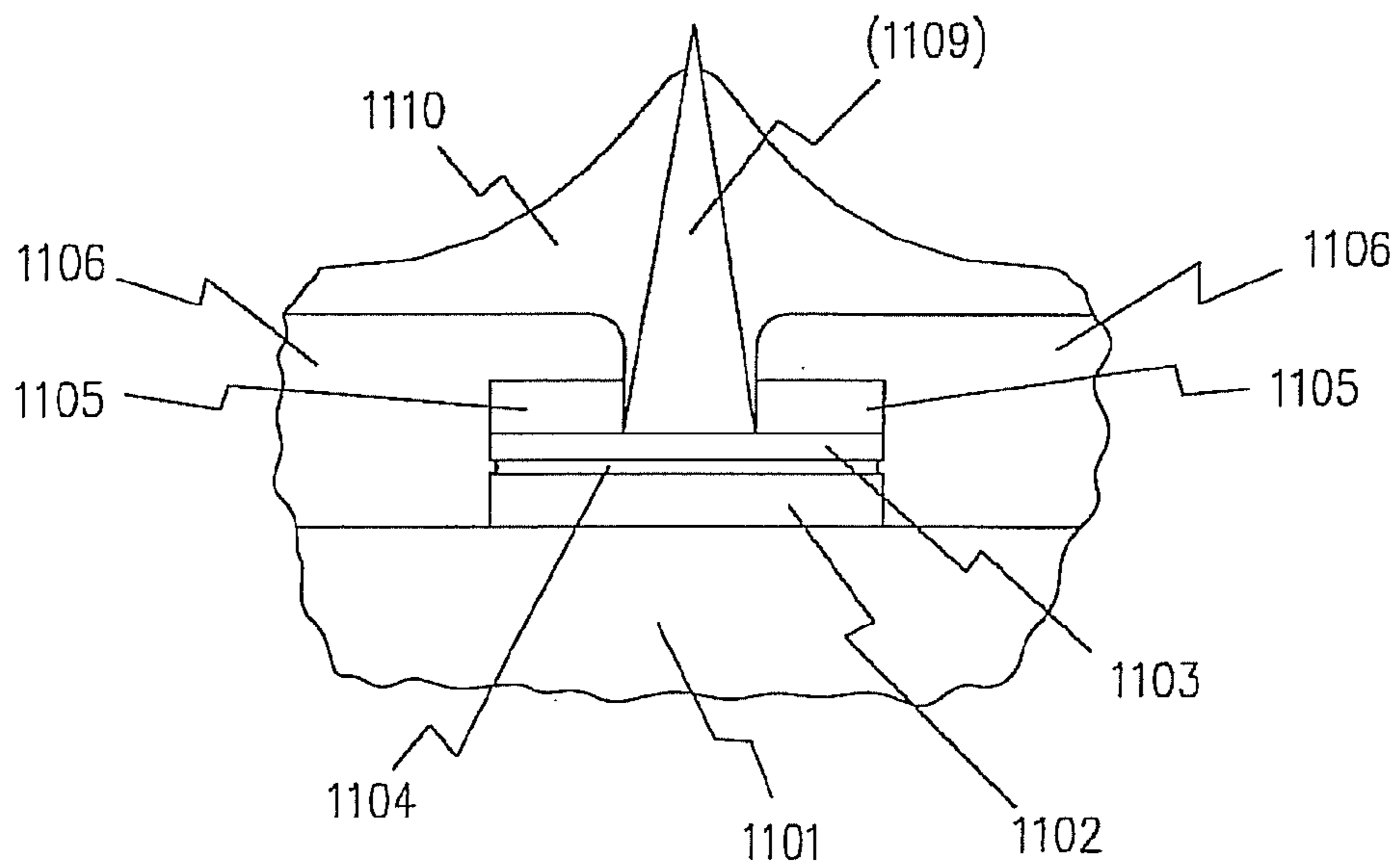
FIGURE 11b ELECTRODES
