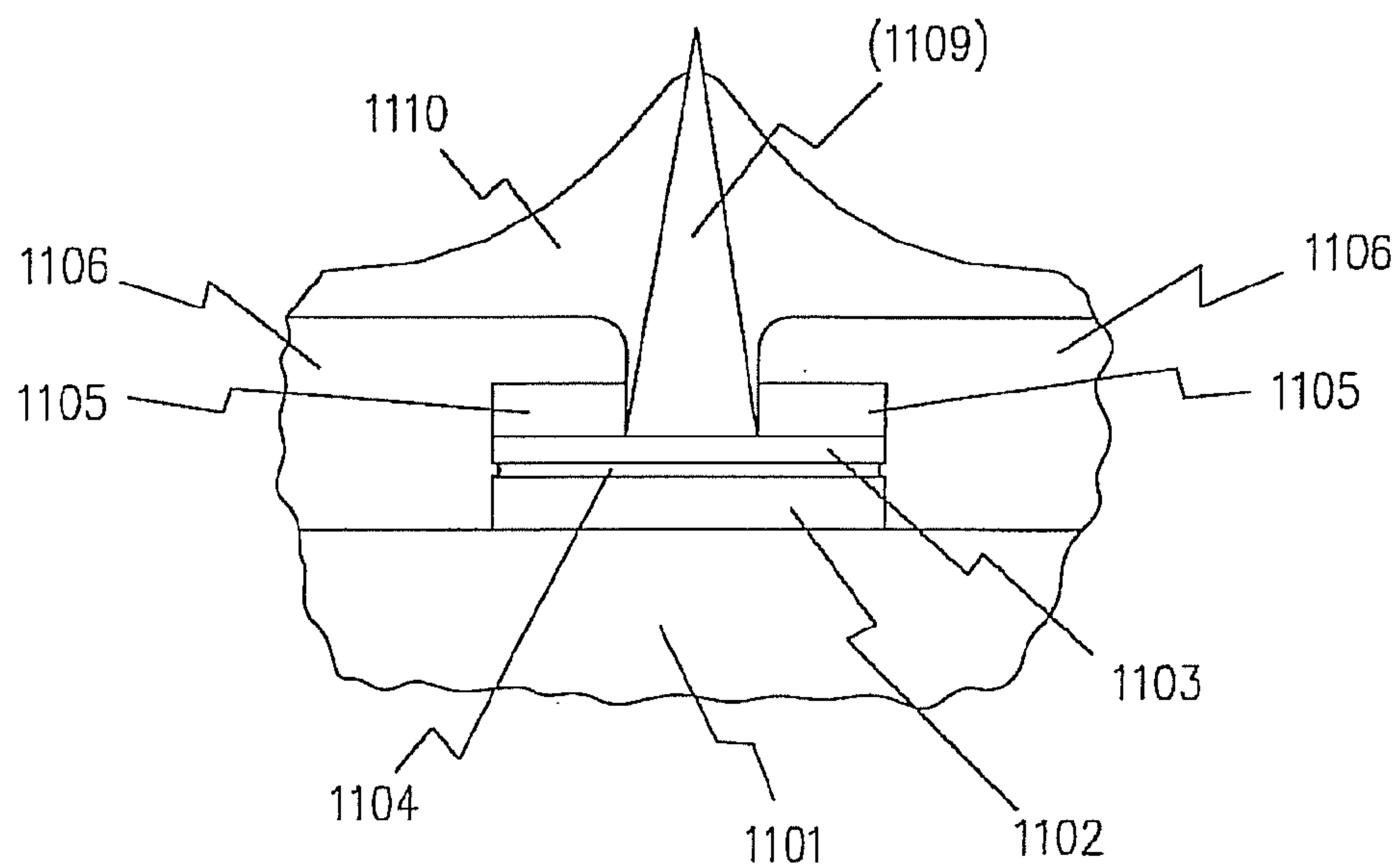
FIGURE 11b ELECTRODES
