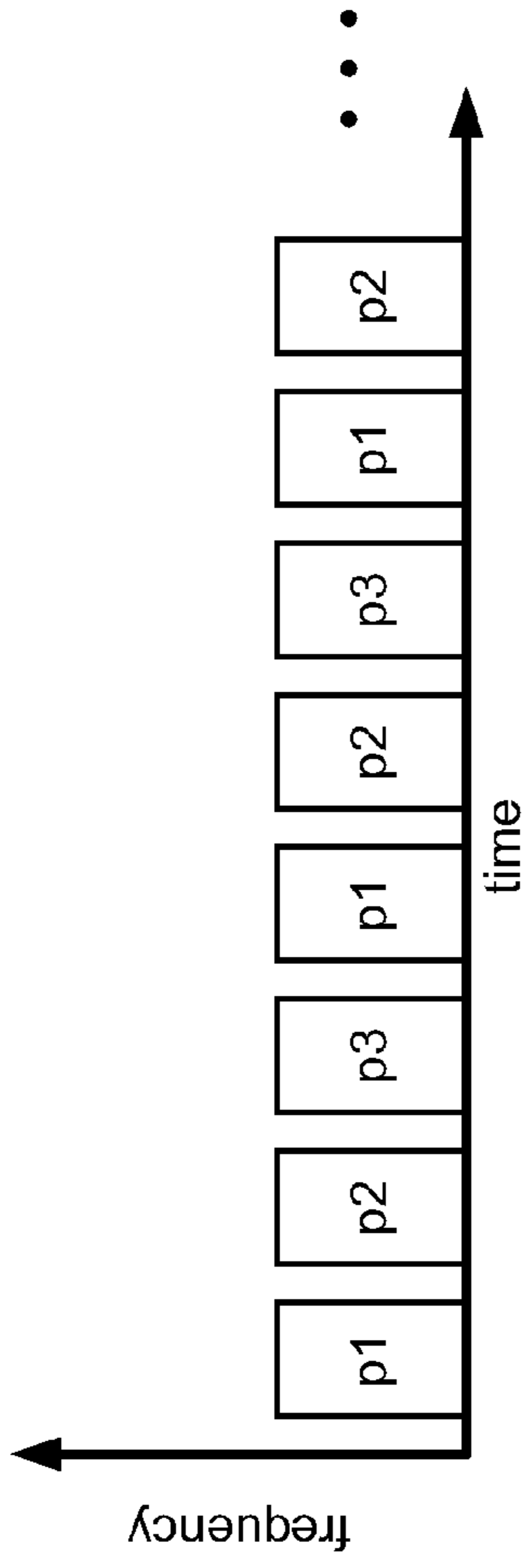
3 SOPs (Simultaneously Operating Piconets) using TDMA only
