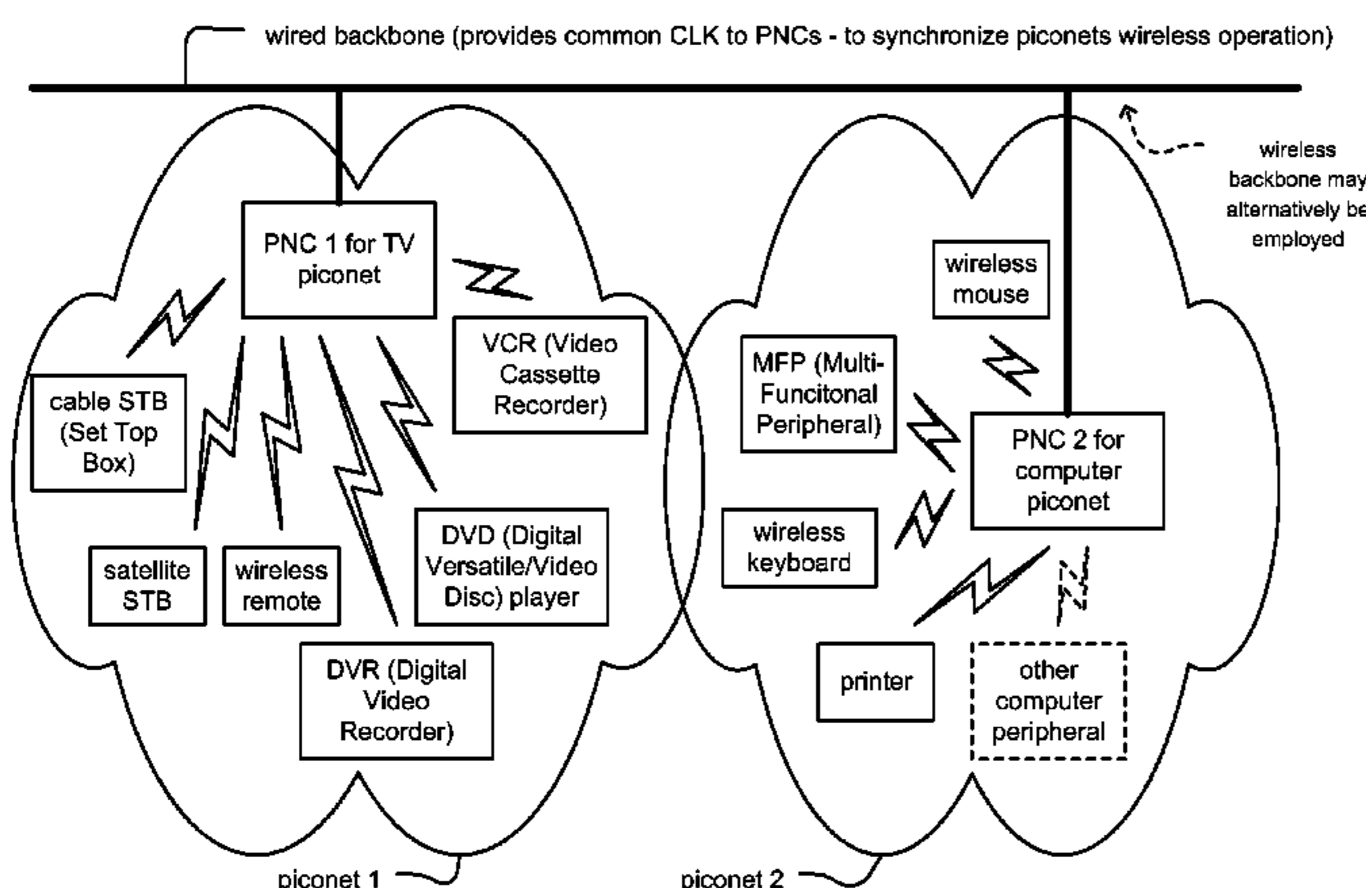
2 SOPs (Simultaneously Operating Piconets) with PNCs (piconet coordinators) coupled to common backbone
