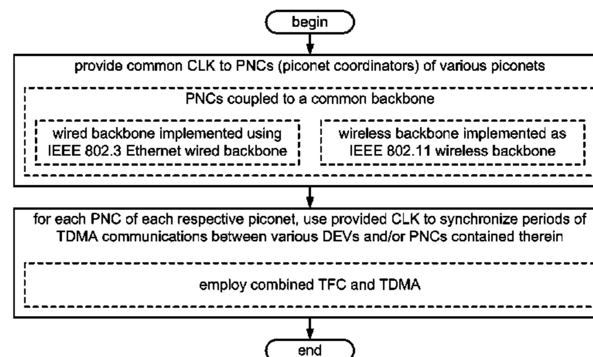
method for operating synchronized SOPs (Simultaneously Operating Piconets)
