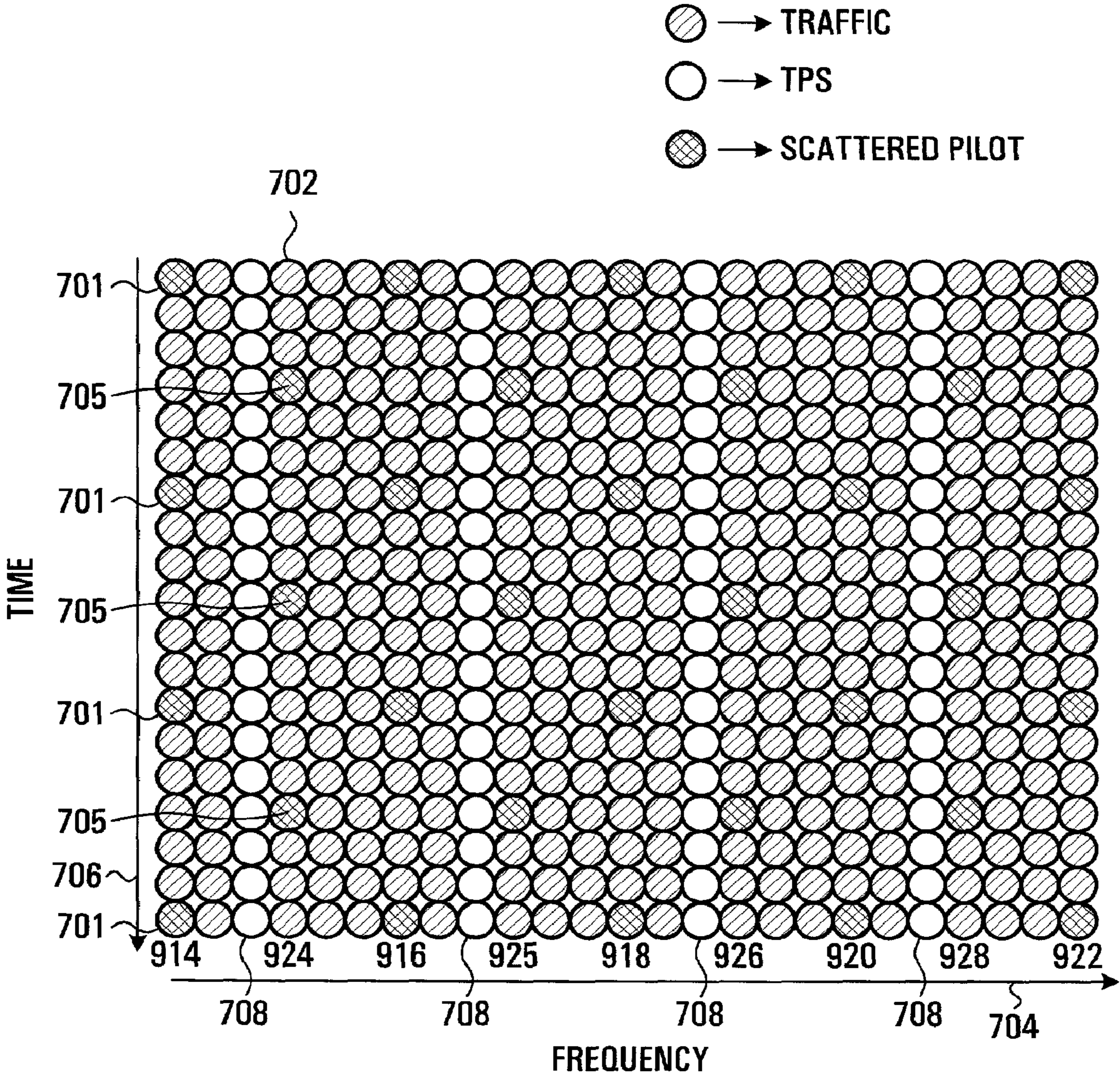
FIG. 7 (PRIOR ART)
