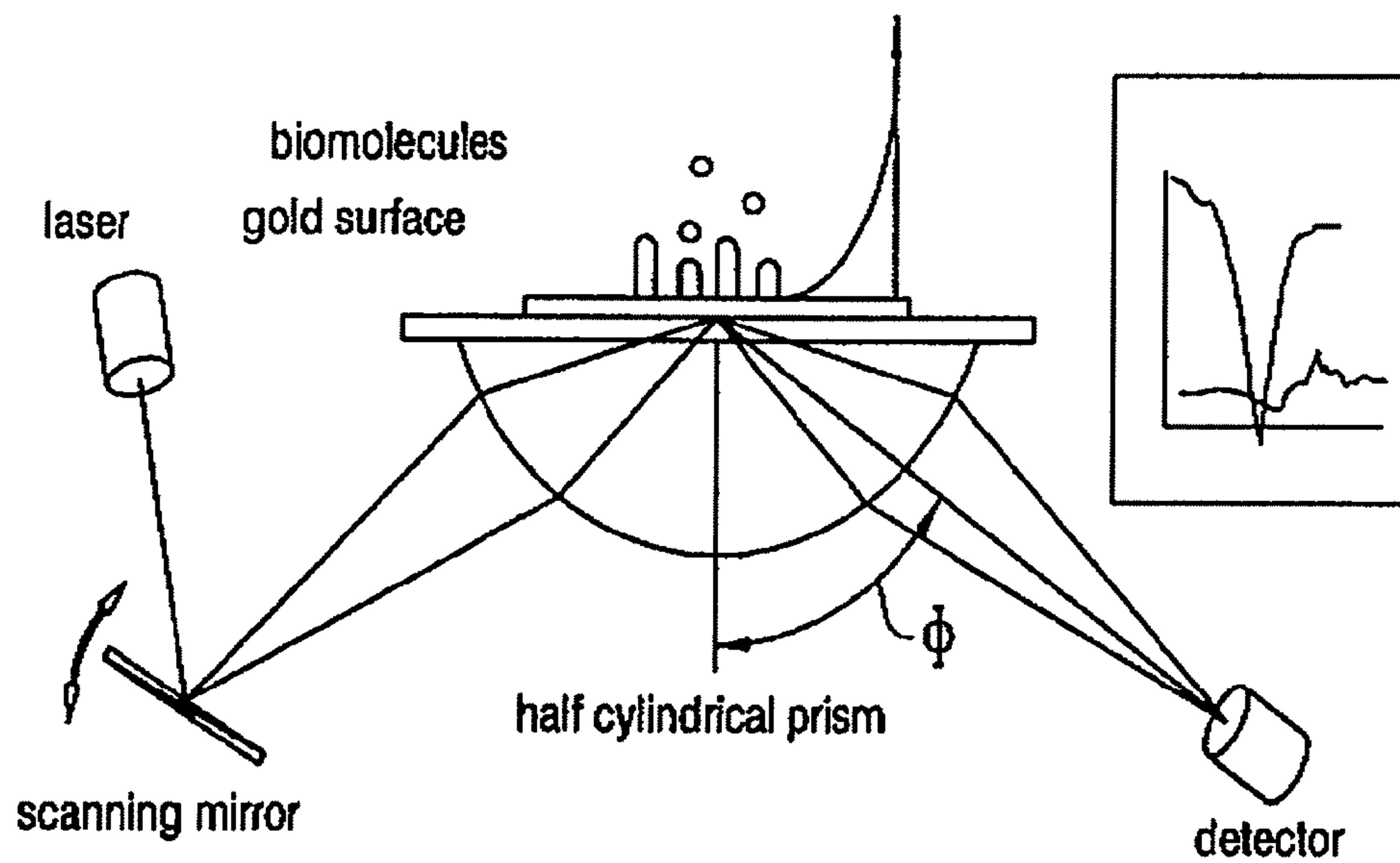
Fig. 1 (PRIOR ART)
