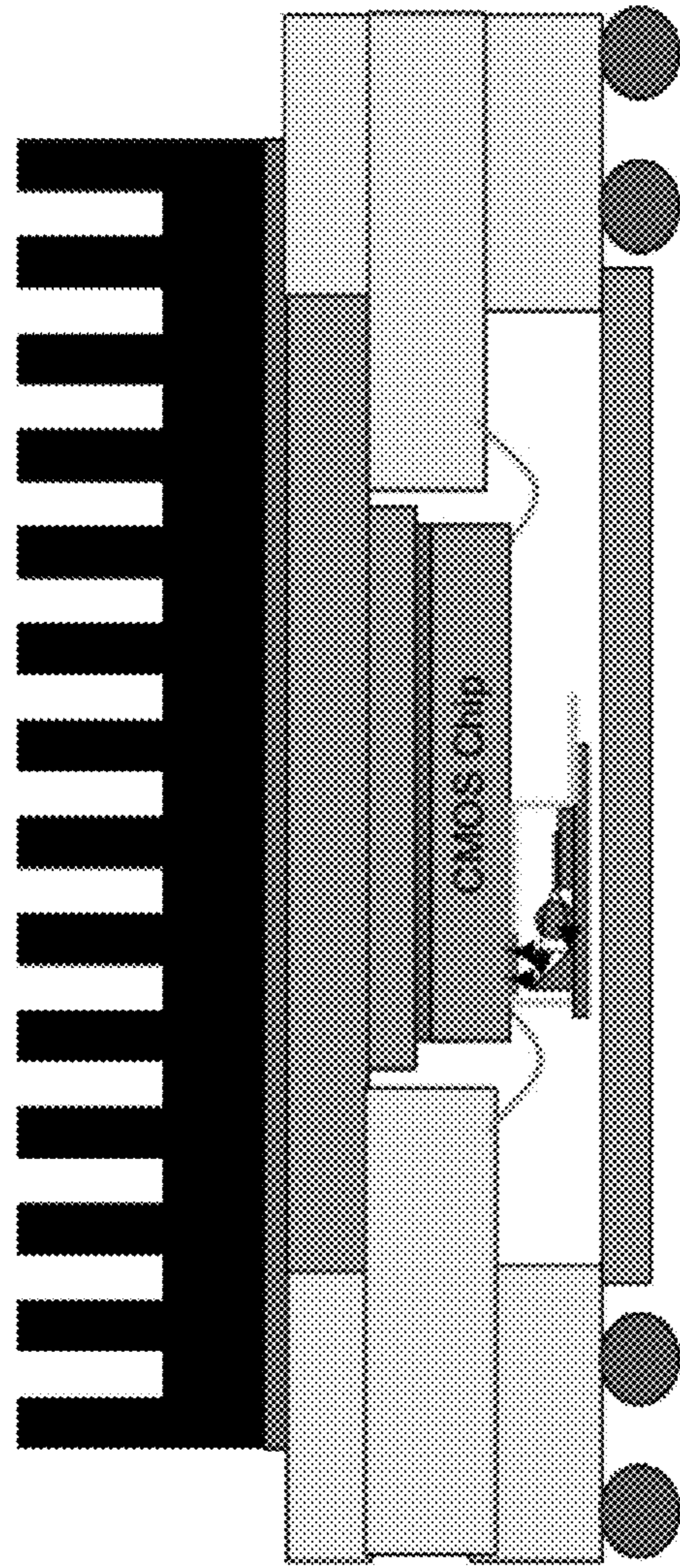
Cavity Down Wire Bond w/Heatspreader (External Heatsink)
