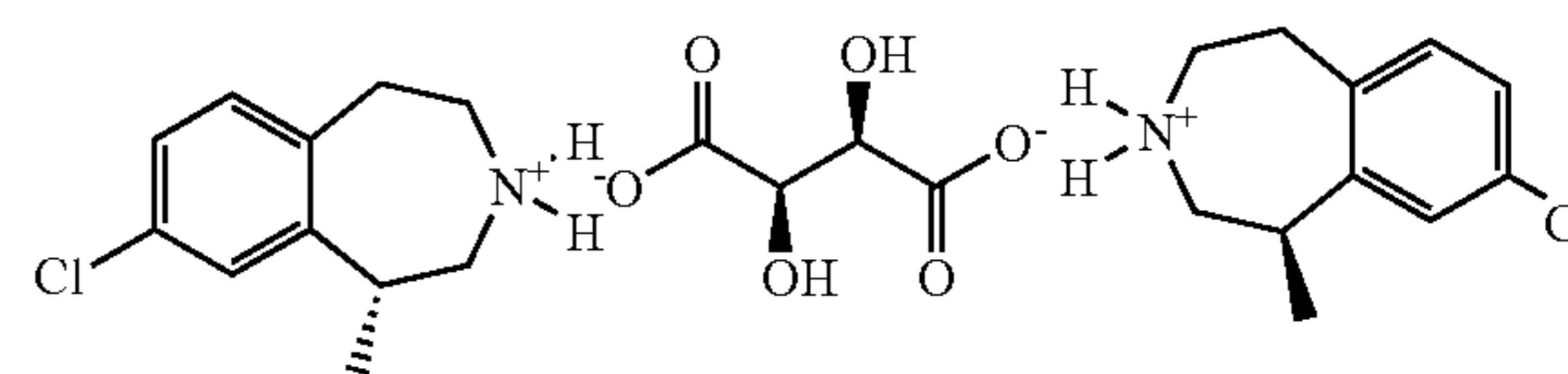
Synthetic Scheme 1.5
