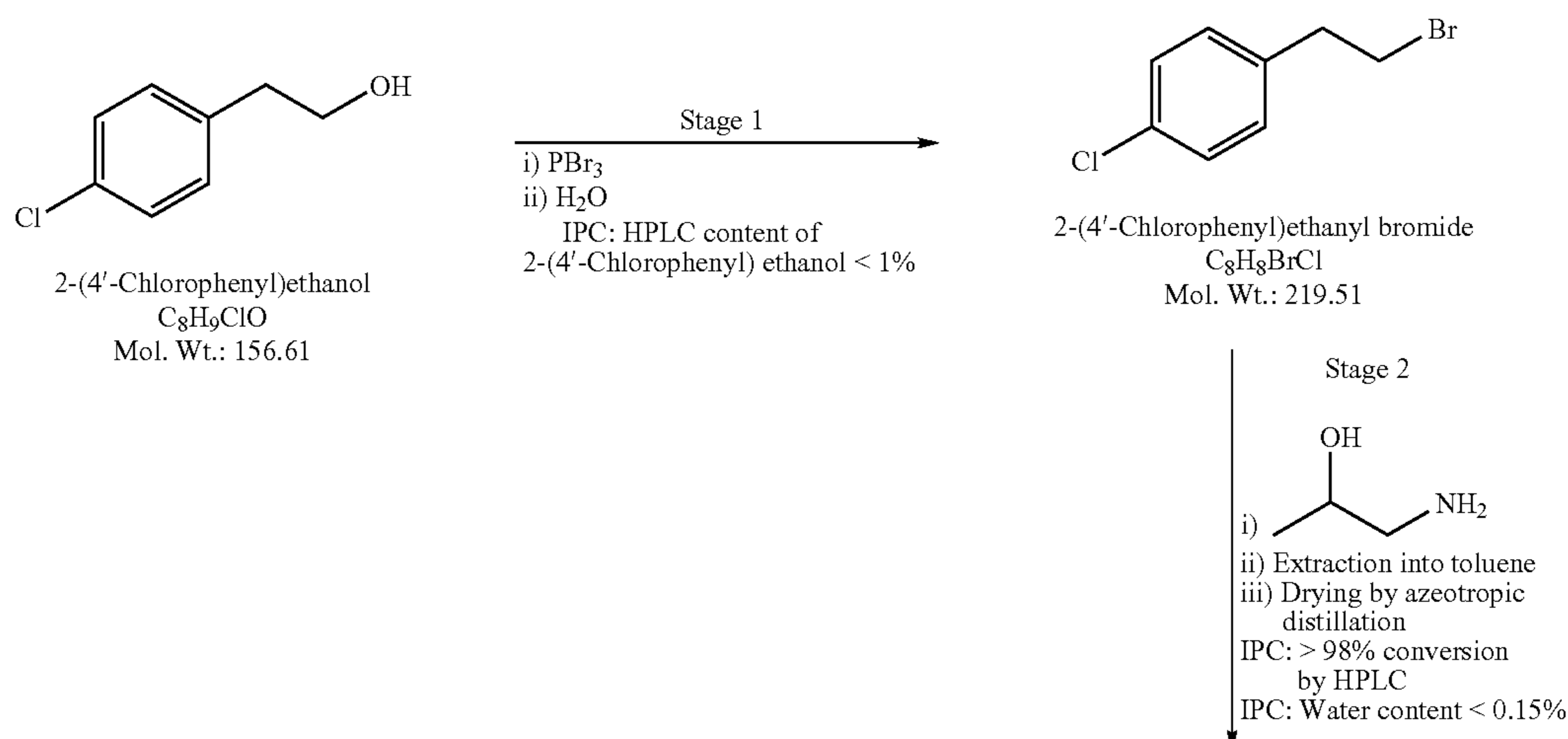
Synthetic Scheme 1.1
