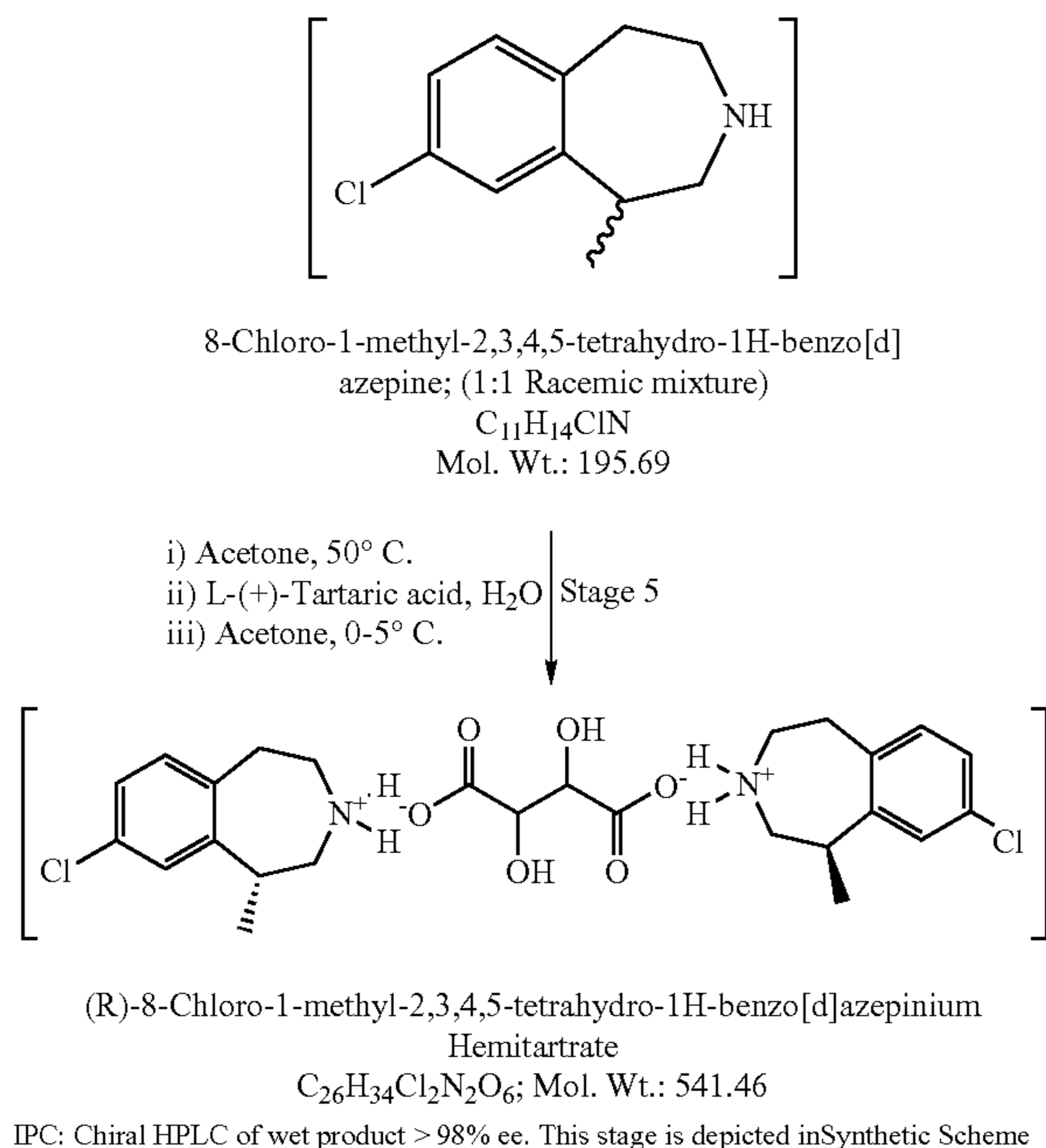
Synthetic Scheme 1.3
