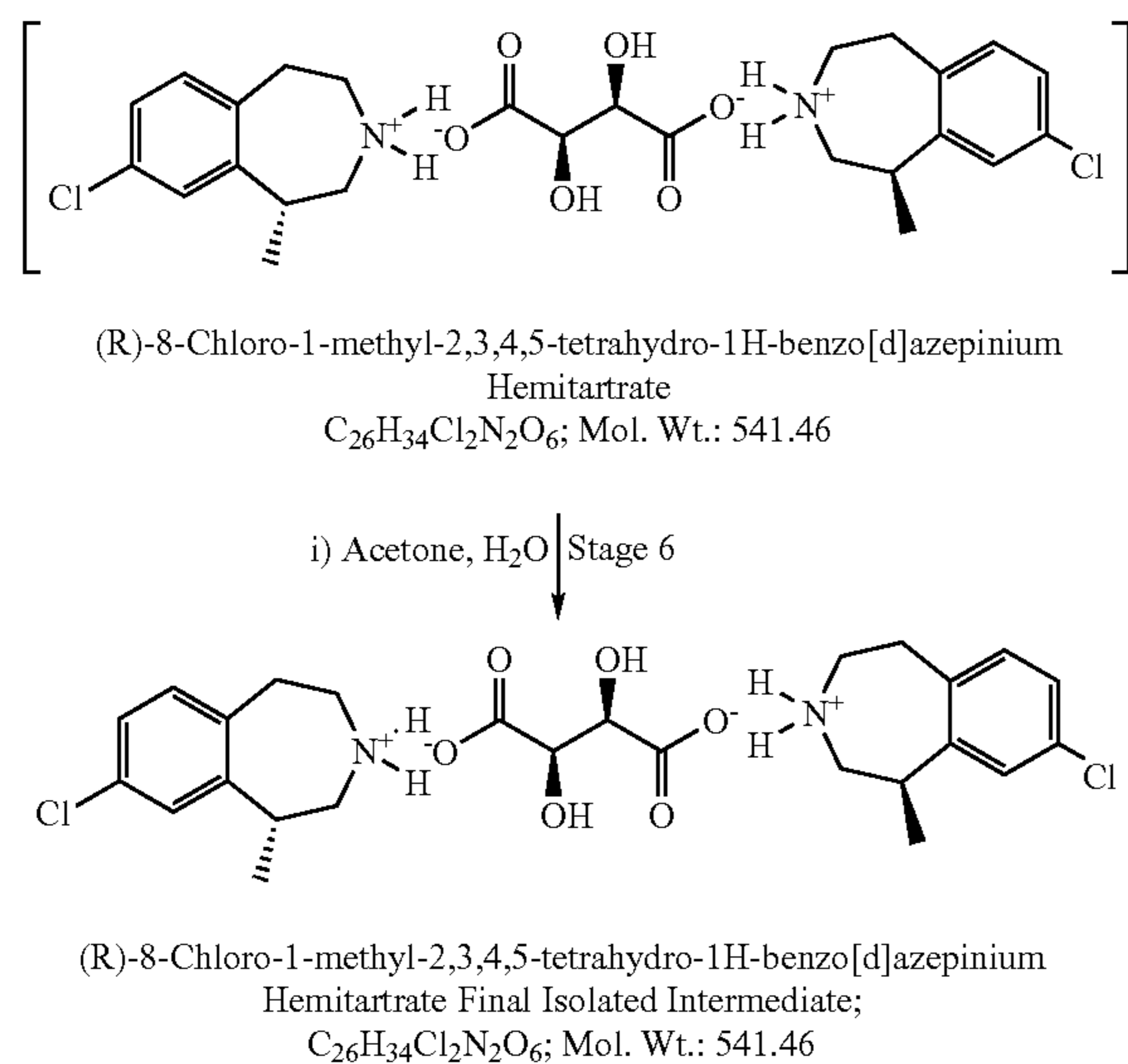
Synthetic Scheme 1.4
