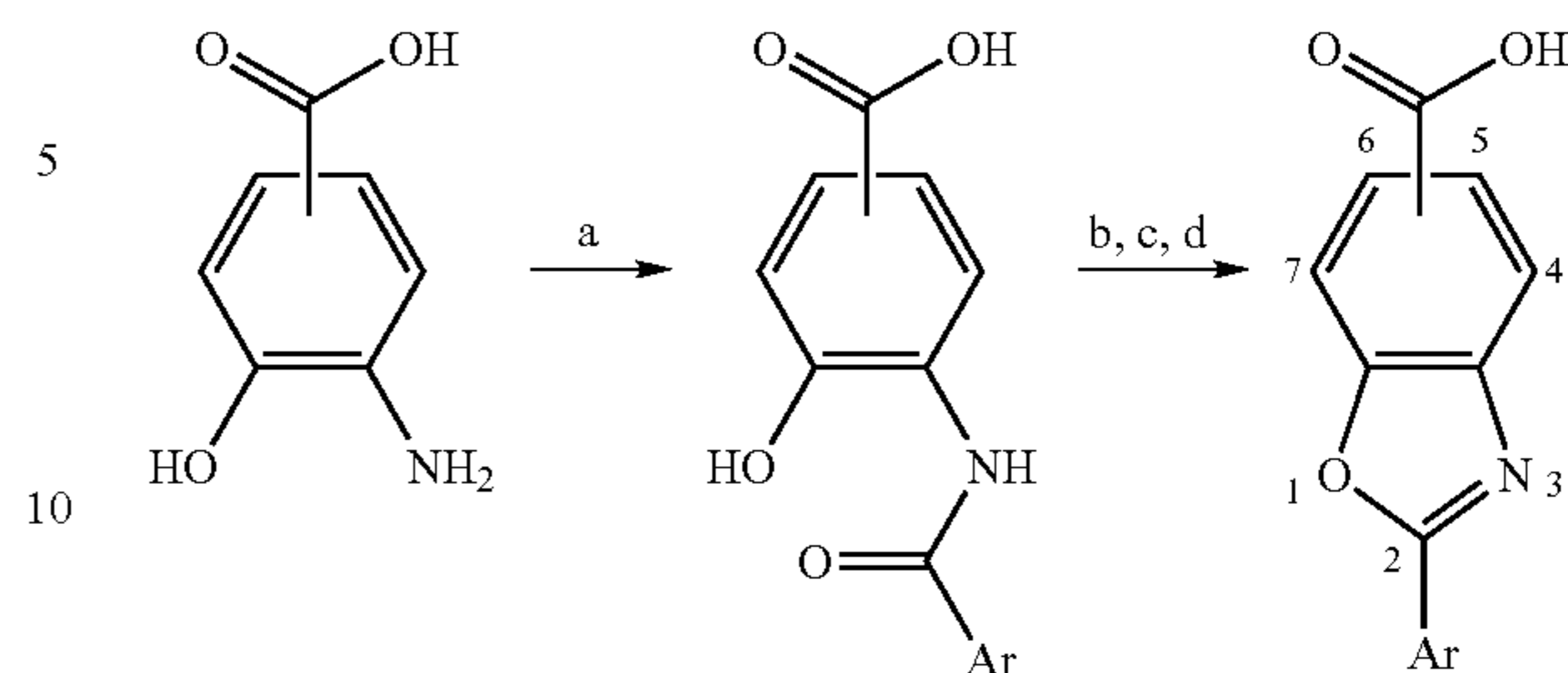
Scheme 1: General Synthesis of Benzoxazoles
