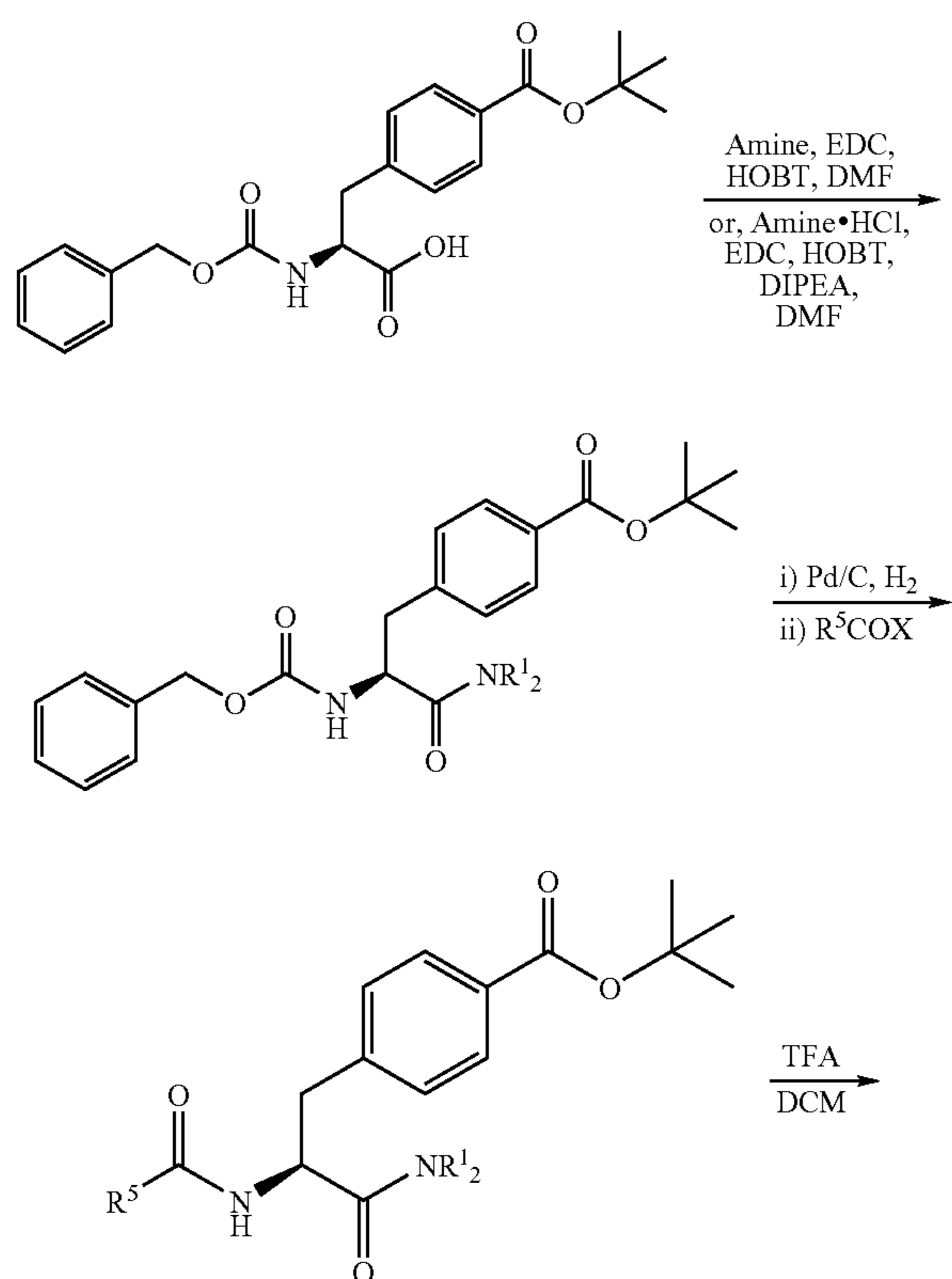
SCHEME 4
