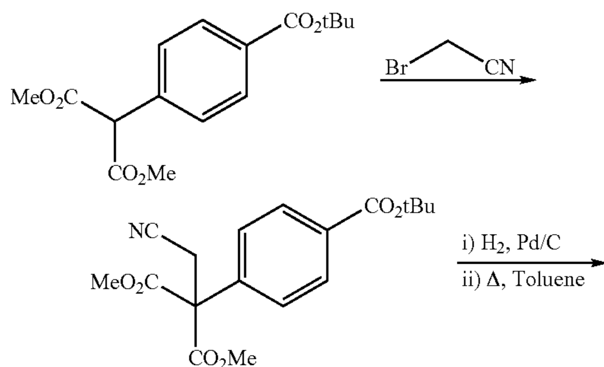
SCHEME 13
