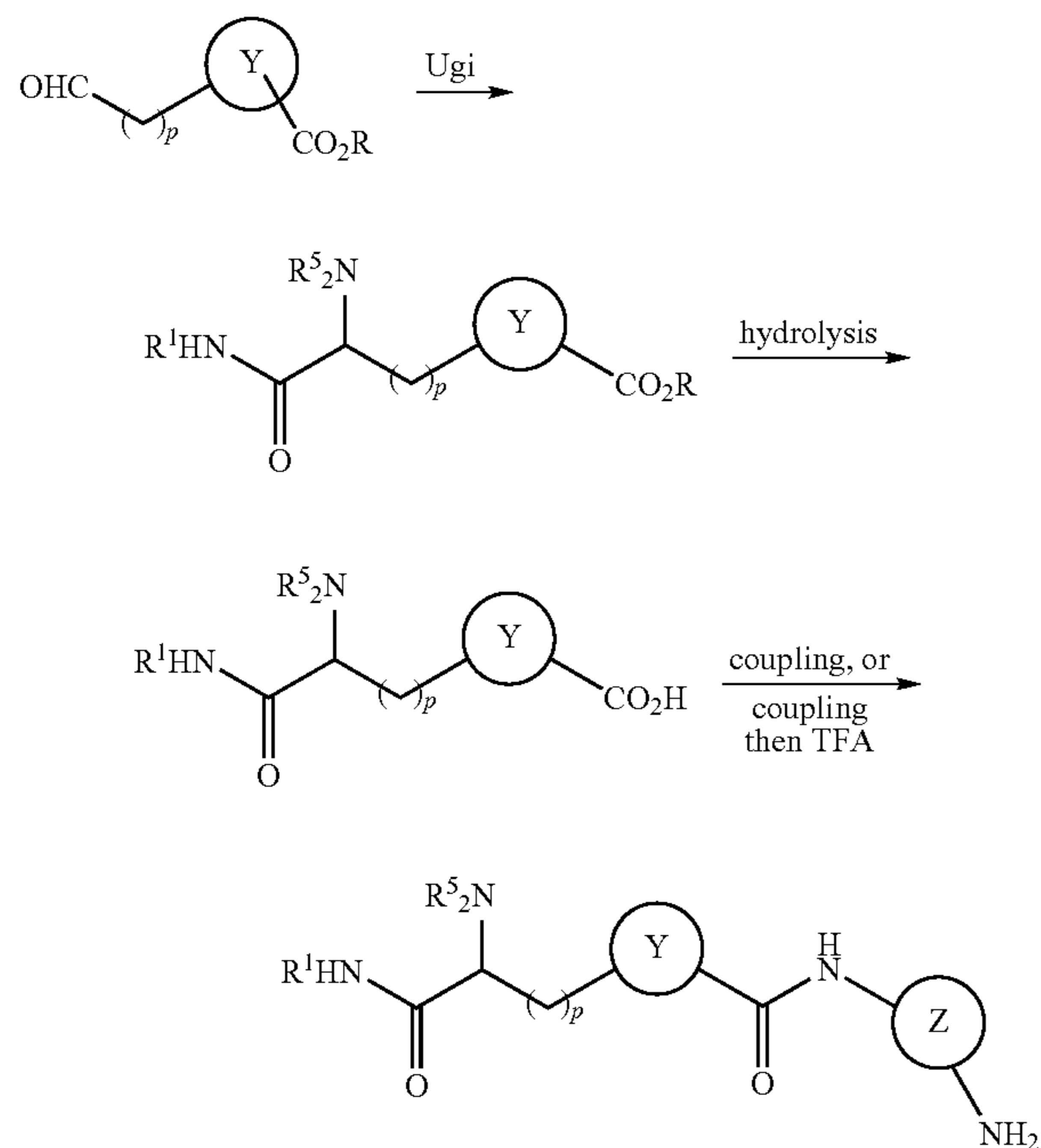
SCHEME 3
