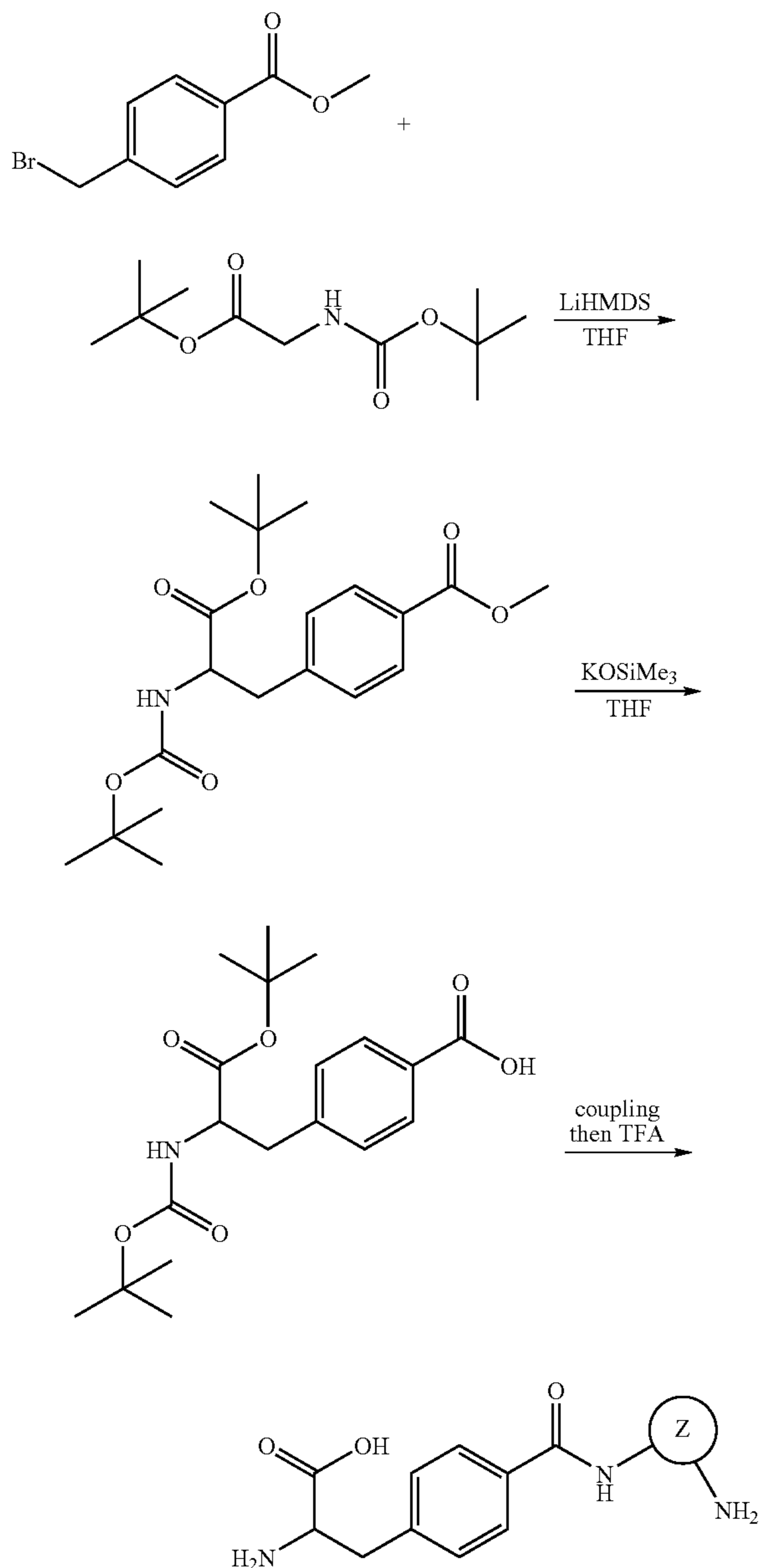
SCHEME 5A
