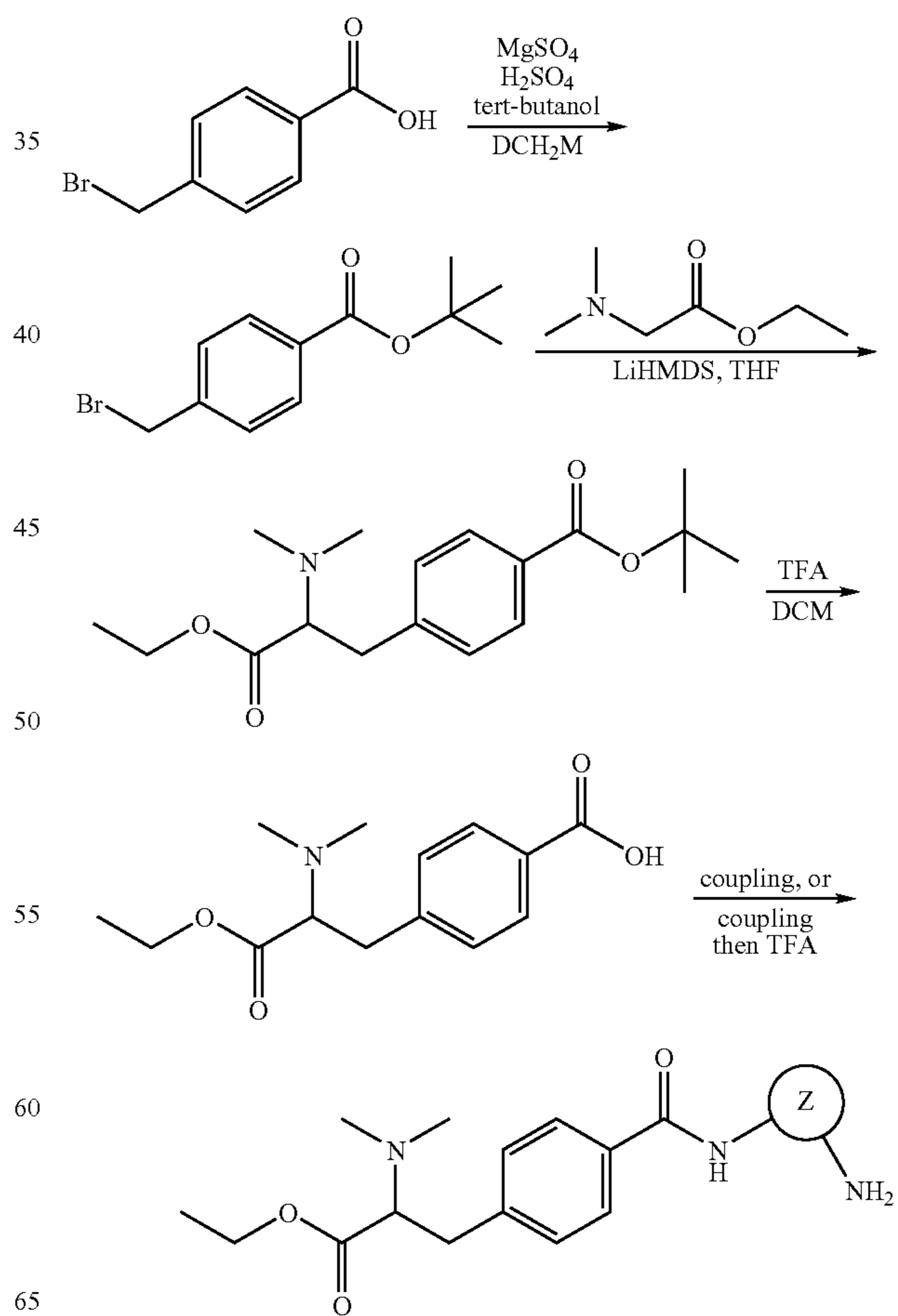
SCHEME 5
