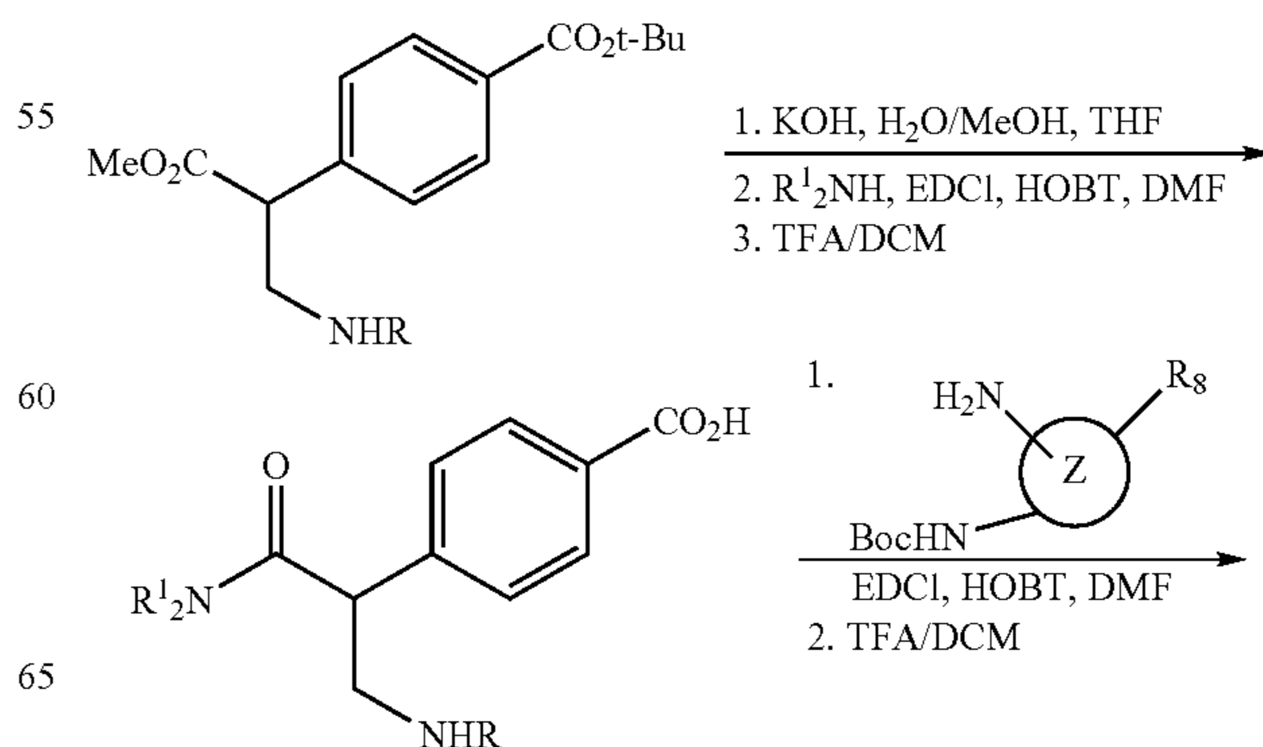
SCHEME 8
