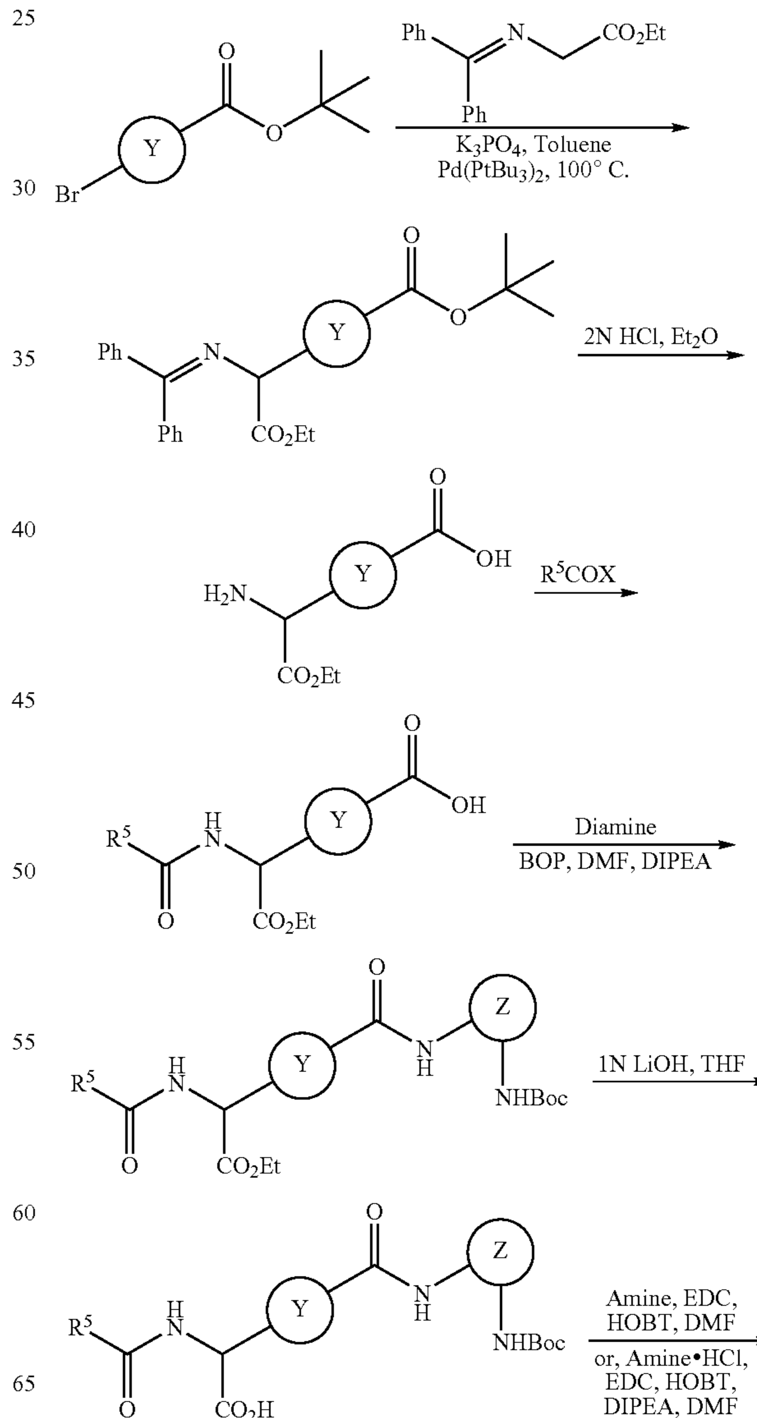
SCHEME 1
