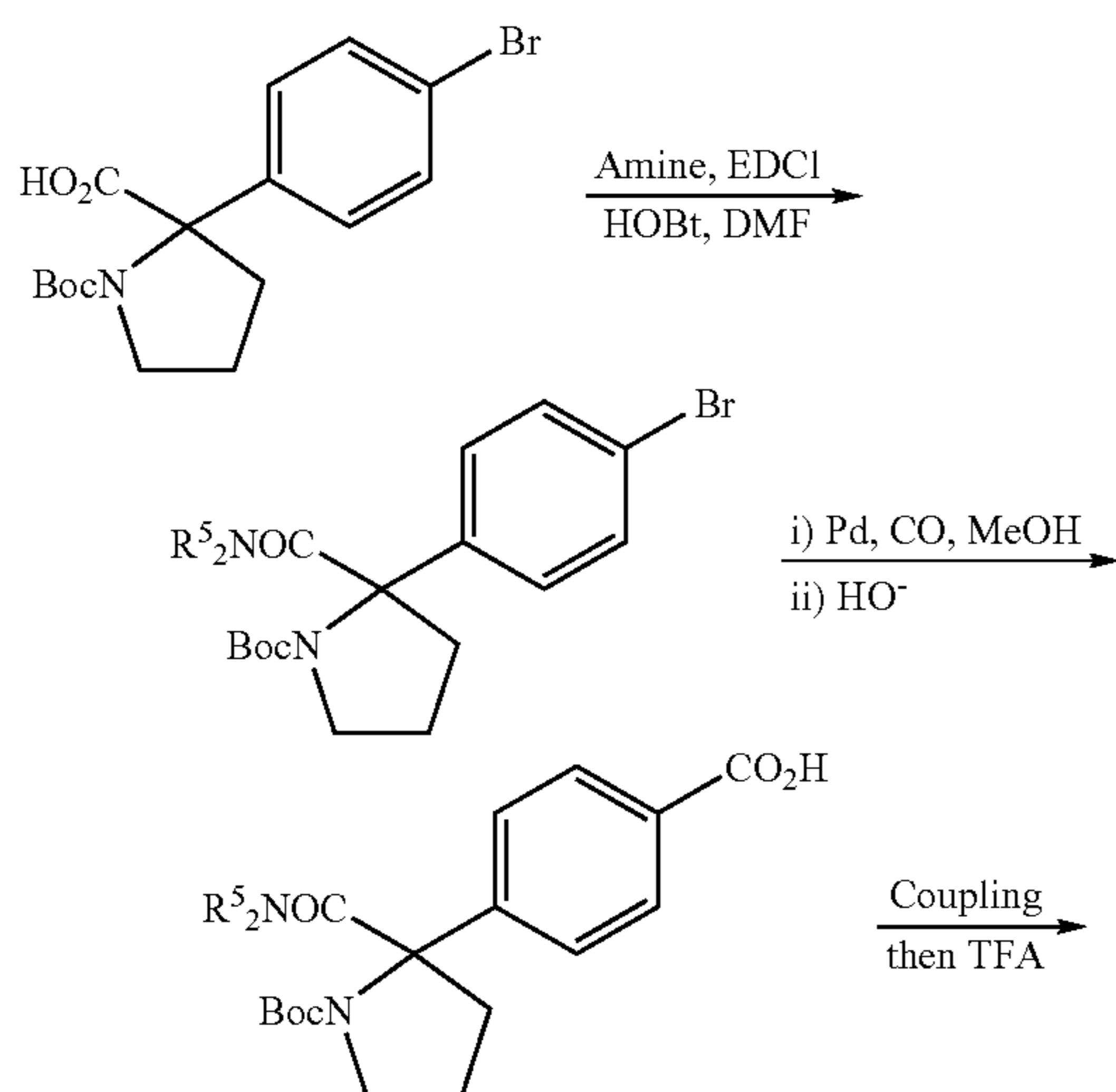
SCHEME 12
