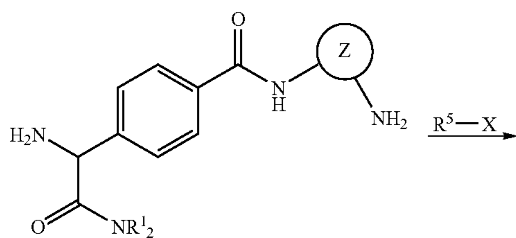
SCHEME 6
