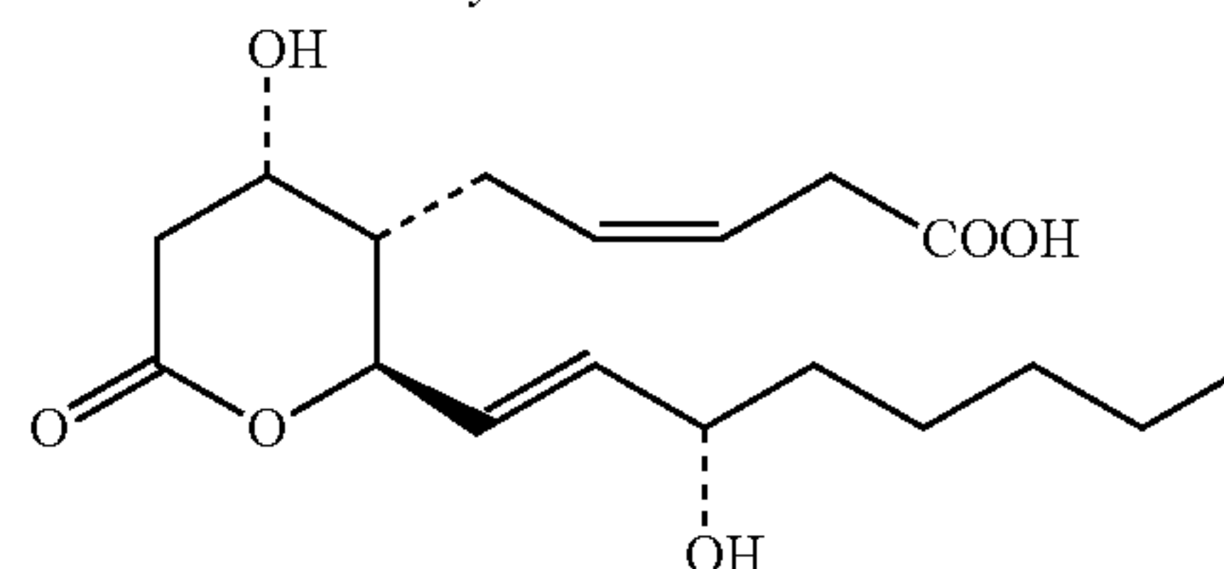
11-dehydro Thromboxane B2
