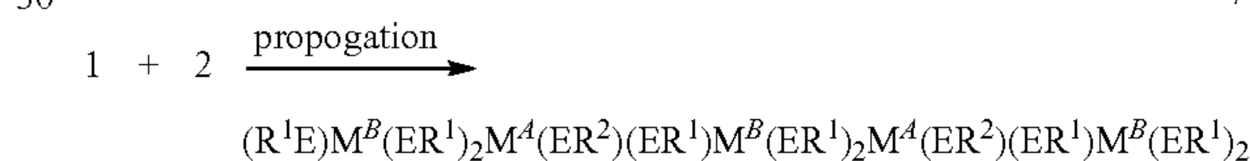
REACTION SCHEME 4:
