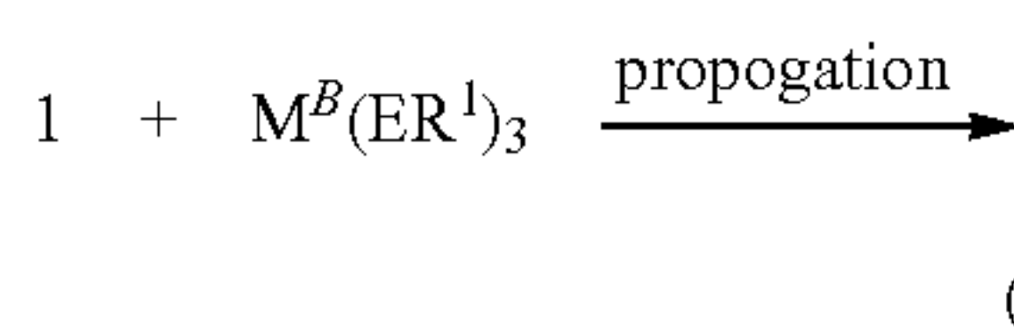
REACTION SCHEME 2:
