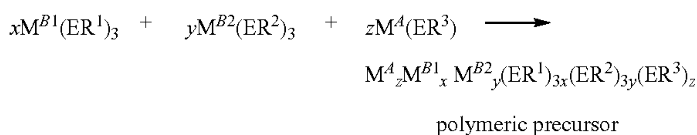
REACTION SCHEME 12:
