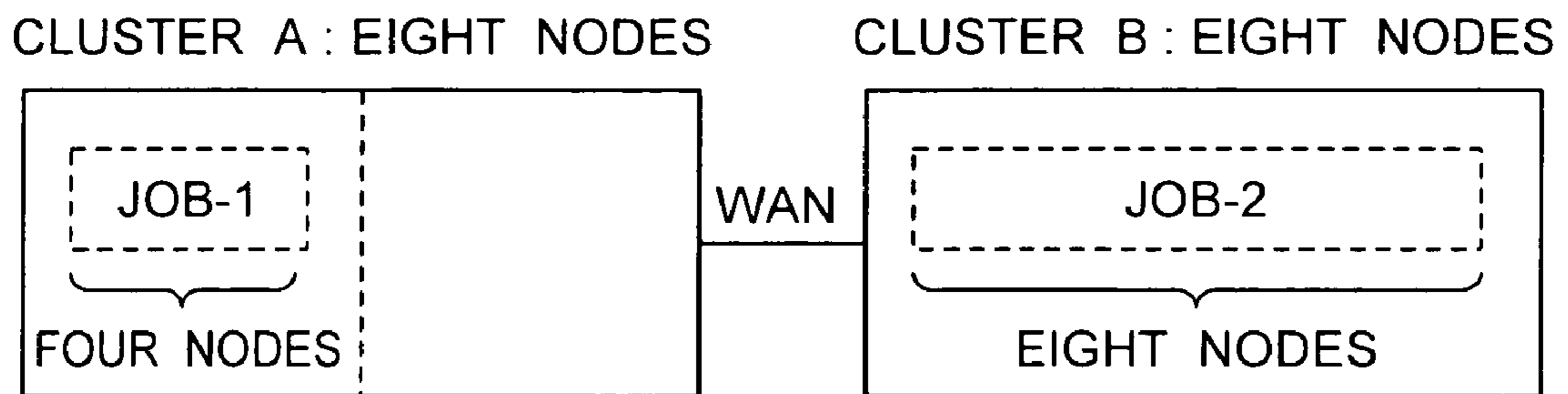
ASSIGNMENT OF JOB BEFORE ISSUING RESERVATION REQUEST
