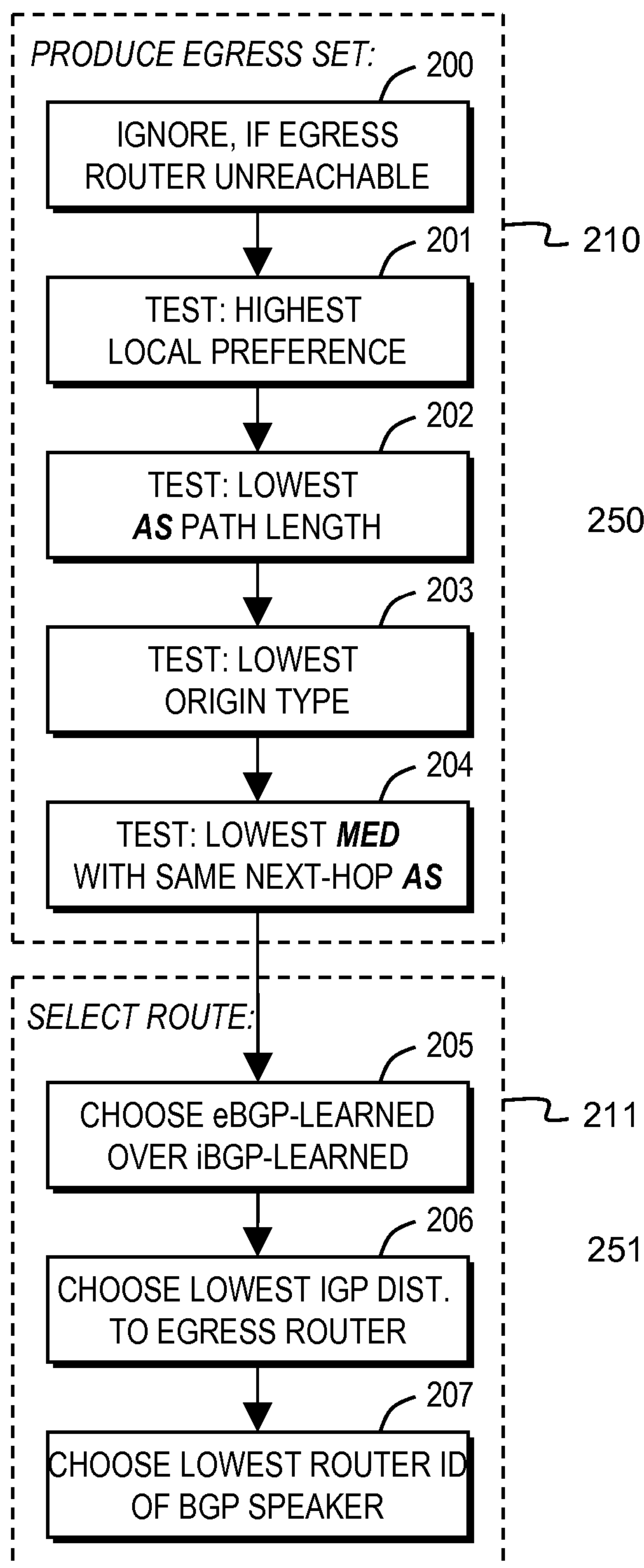
PRIOR ART FIG. 2A
