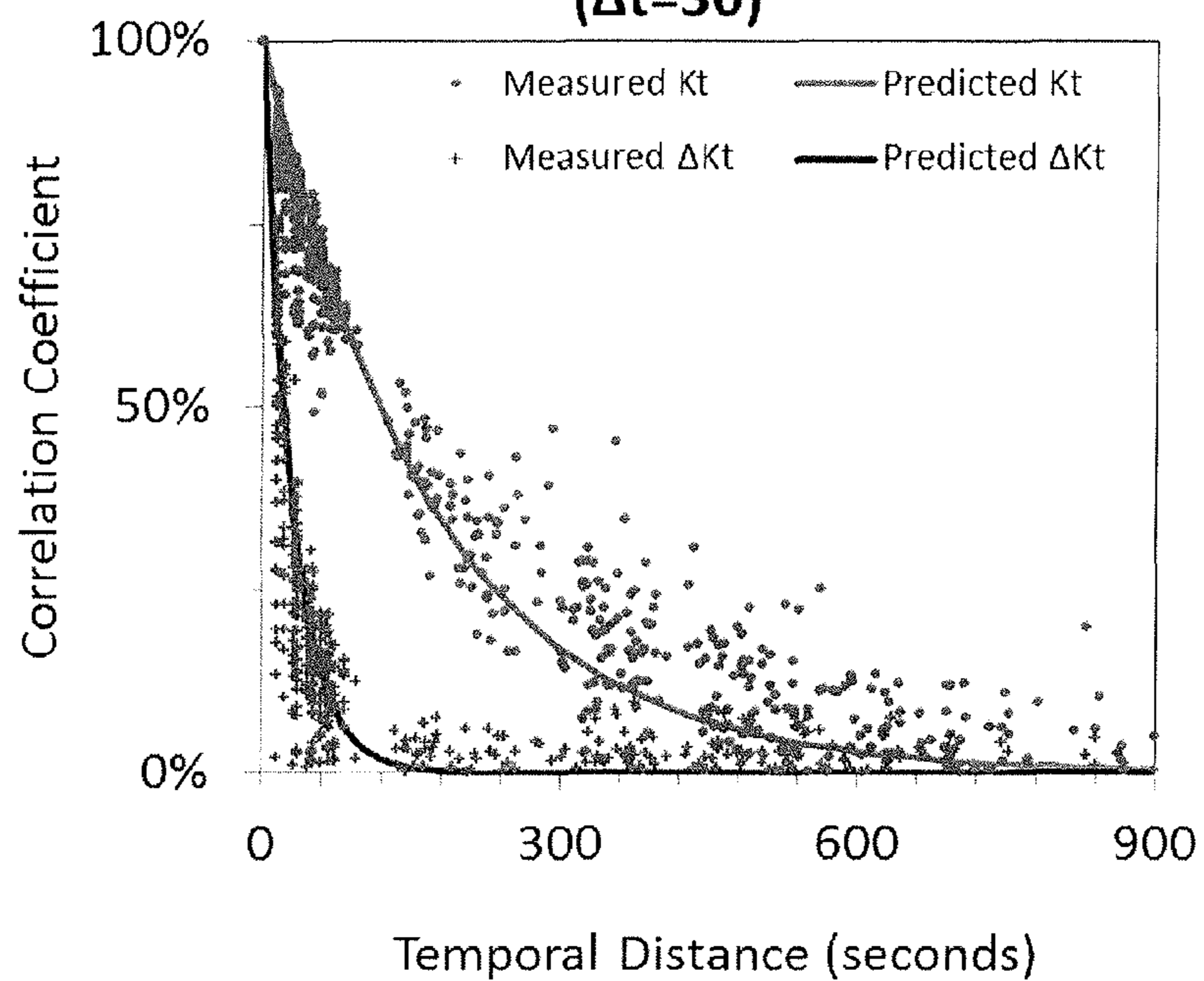
Correlation vs. Temporal Distance ( \Delta t=30 )
