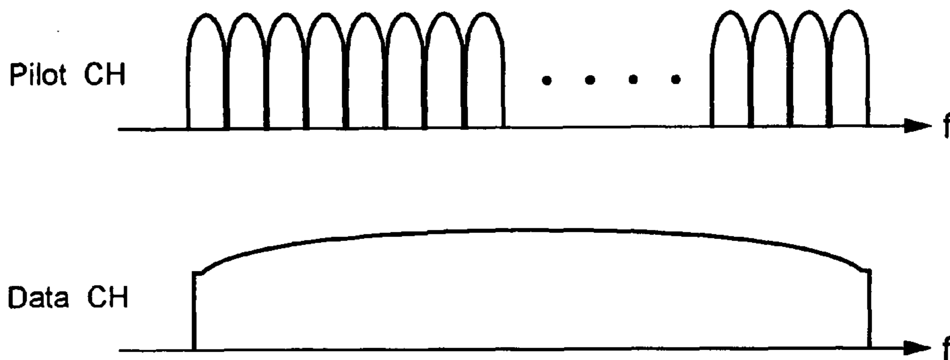
MULTIPLEXING OF Pilot CH AND Data CH ( WHERE FDM pilot AND SRF ( Symbol Repetition Factor = 4 ) )
