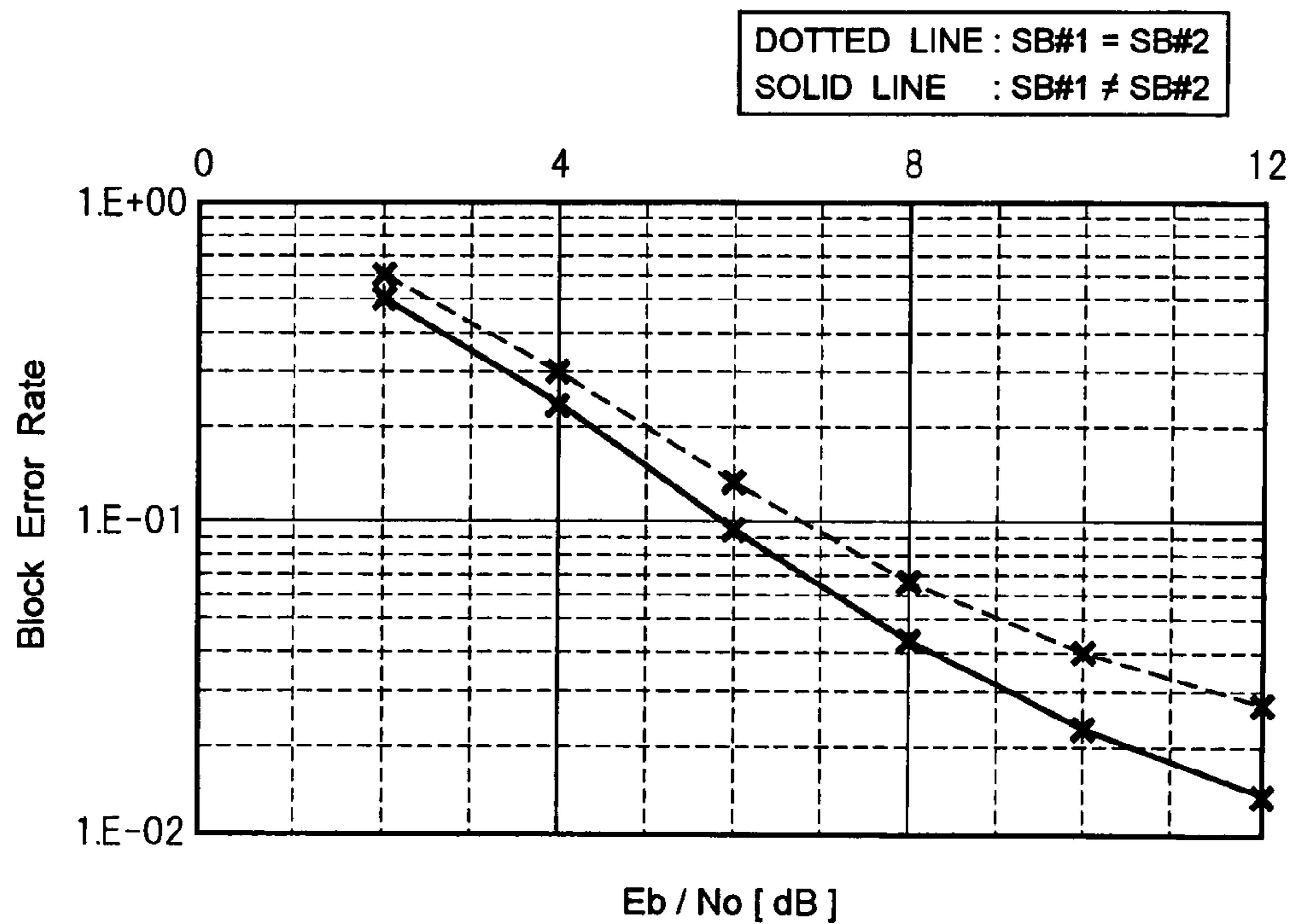
BLOCK ERROR RATE FOR E_b/N_0 (SIGNAL ENERGY FOR ONE BIT AND NOISE - TO - POWER DENSITY RATIO)
