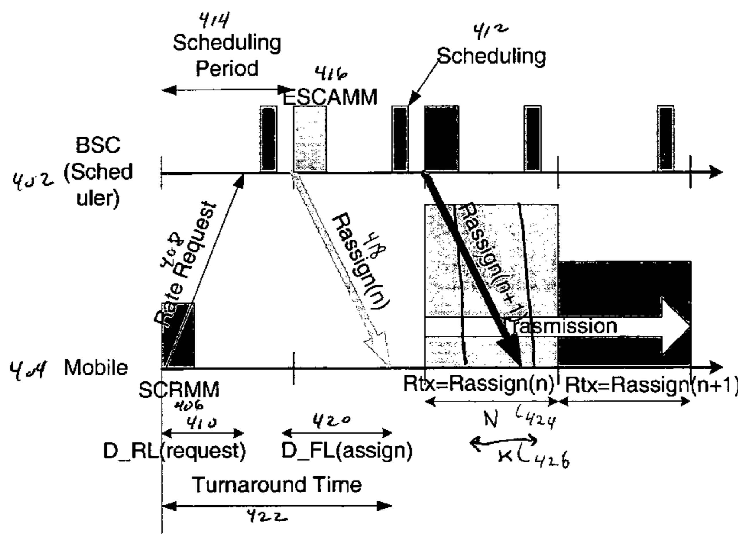
Parameters associated in mobile station scheduling on RL
