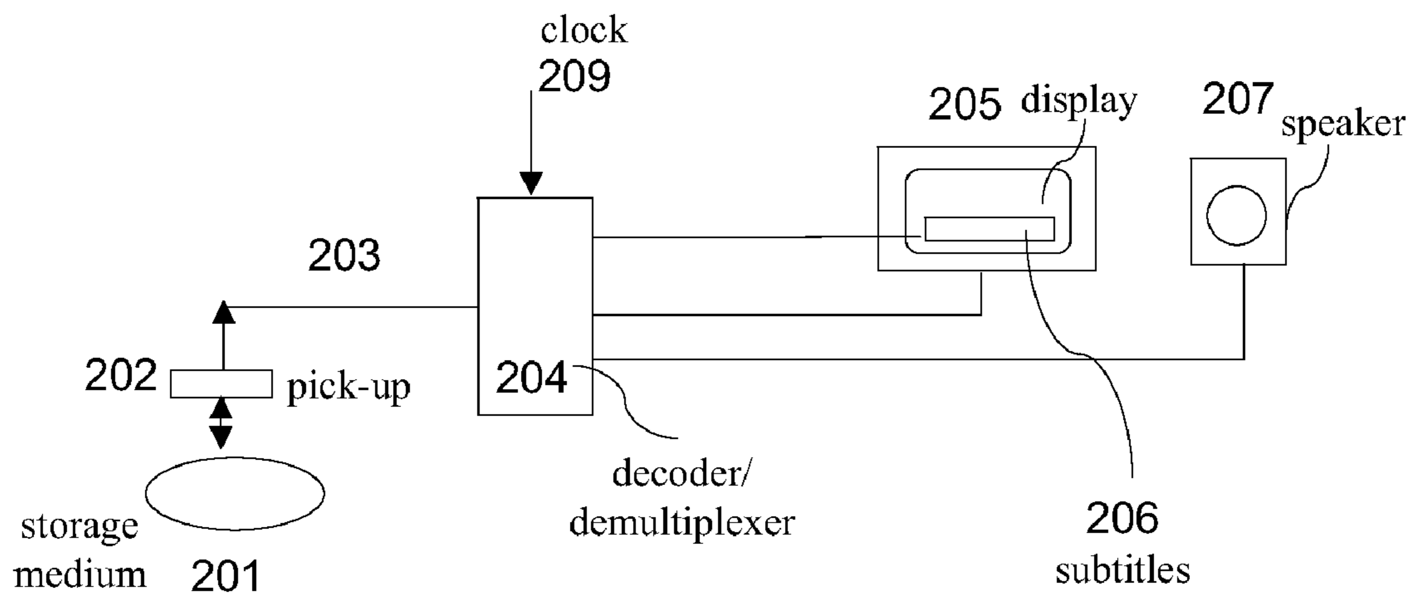
FIG. 2 PRIOR ART
