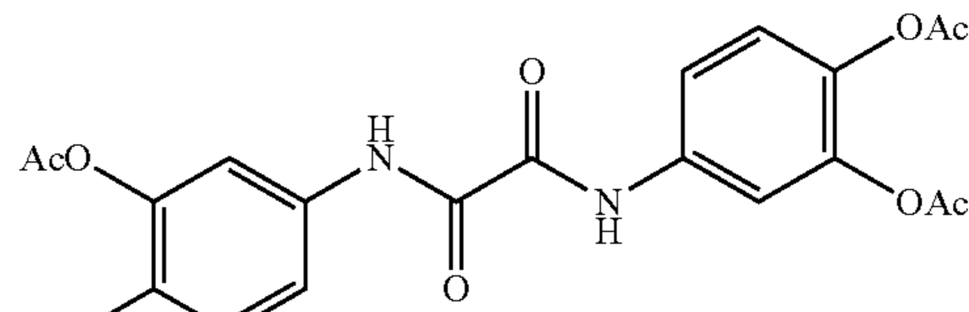
Oxalic acid bis(3,4-diacetoxyanilide)
