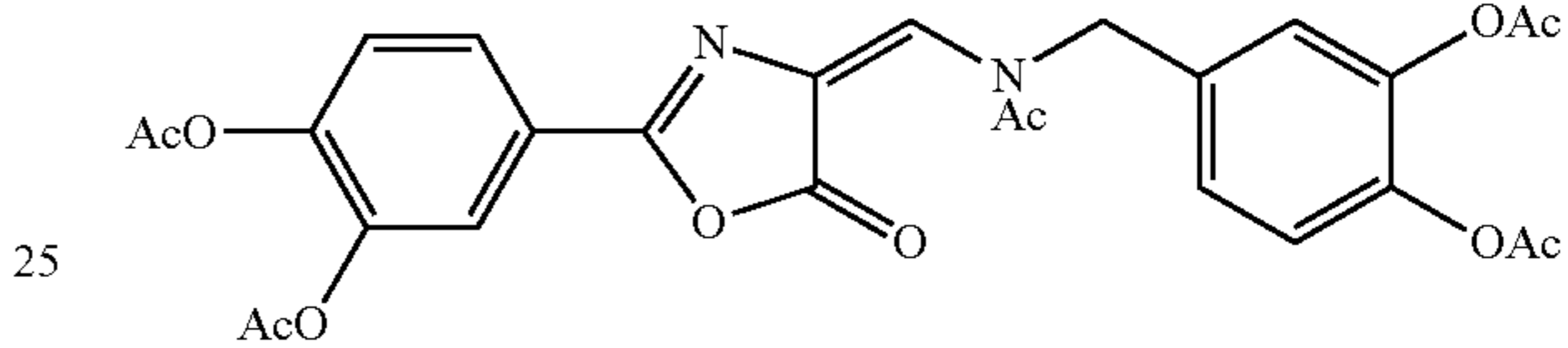
N-acetyl-4-(3,4-diacetoxybenzylamino)methylene)-2-(3,4-diacetoxyphenyl)-oxazolin-5-one
