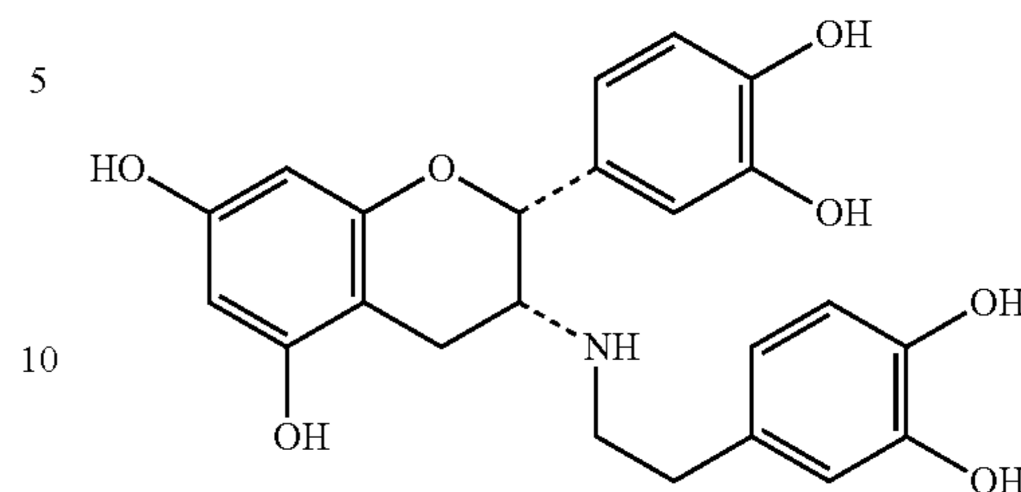
3-deoxy-3-(3,4-dihydroxyphenethyl)(-)-amino-epicatechin
