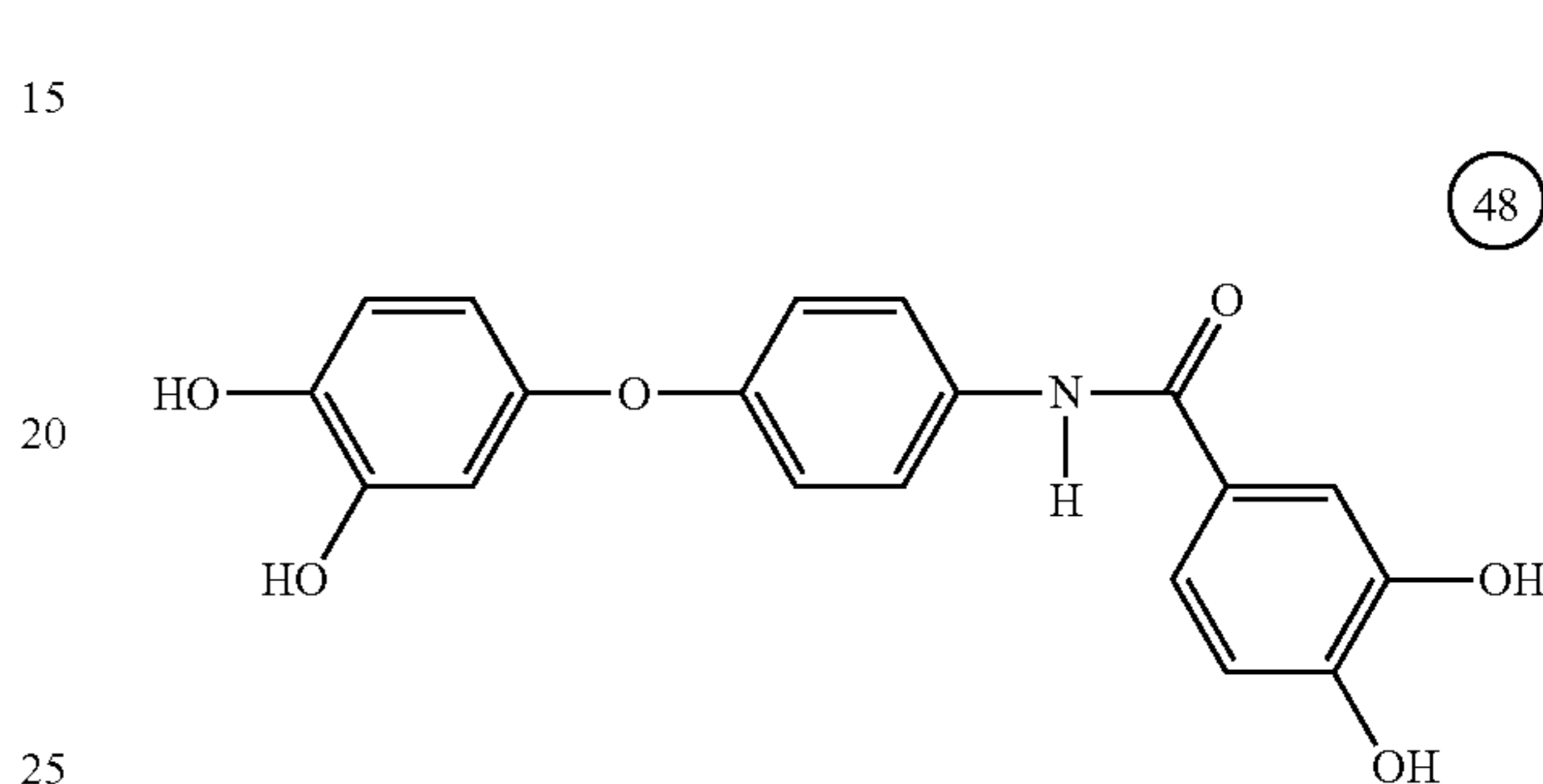
3,4-dihydroxybenzoic acid p-(3,4-di- hydroxyphenoxy) anilide
