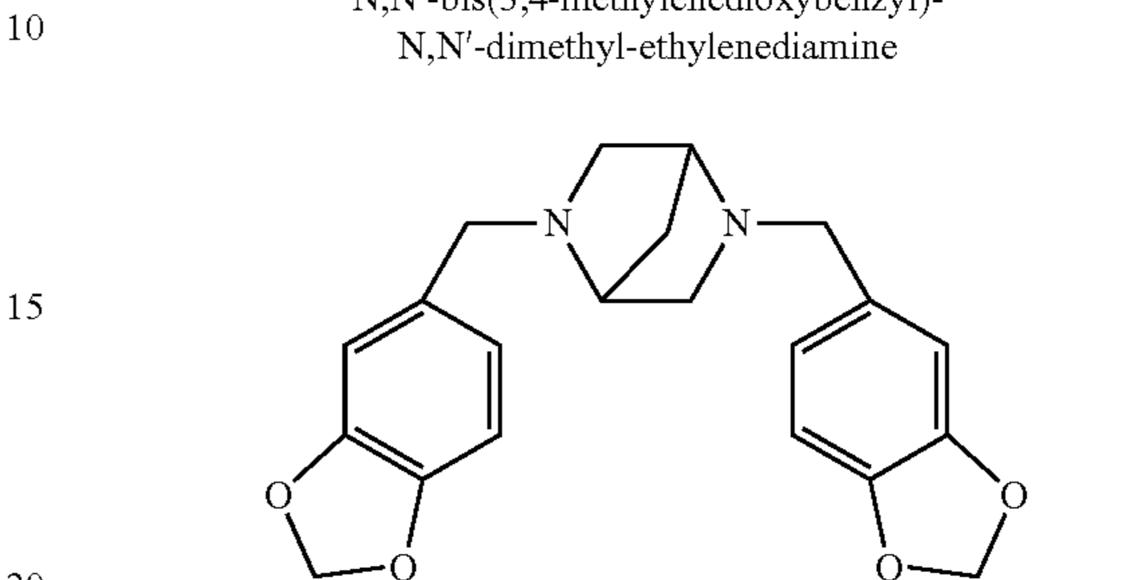
2,5-bis(3,4-methylenedioxybenzyl)-2,5-diaza[2,2,1]-bicycloheptane
