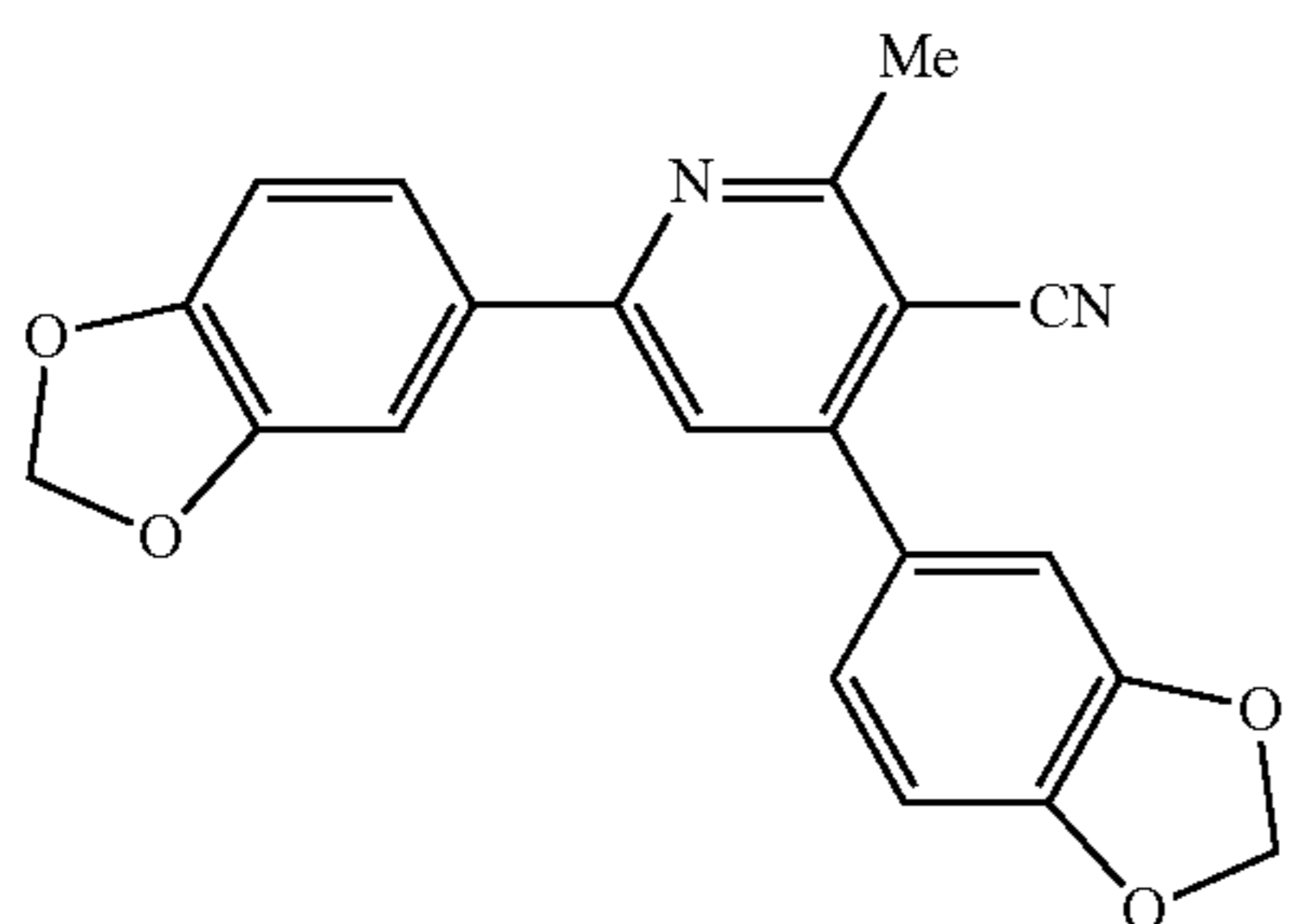
4,6-bis(3,4-methylenedioxyphenyl)- 3-cyano-2-methylpyridine
