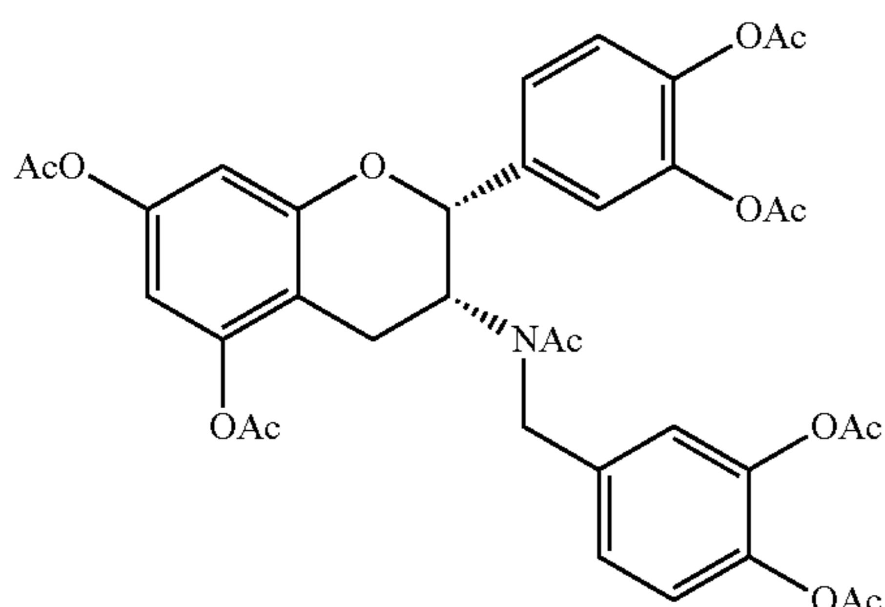
N-acetyl-3-deoxy-3-(3,4-diacetoxybenzyl)-amino-5,7,3',4'-tetraacetyl-epicatechin
