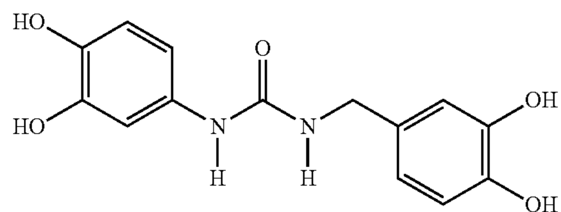
1-(3,4-dihydroxyphenyl)-3-(3,4-dihydroxybenzyl)urea
