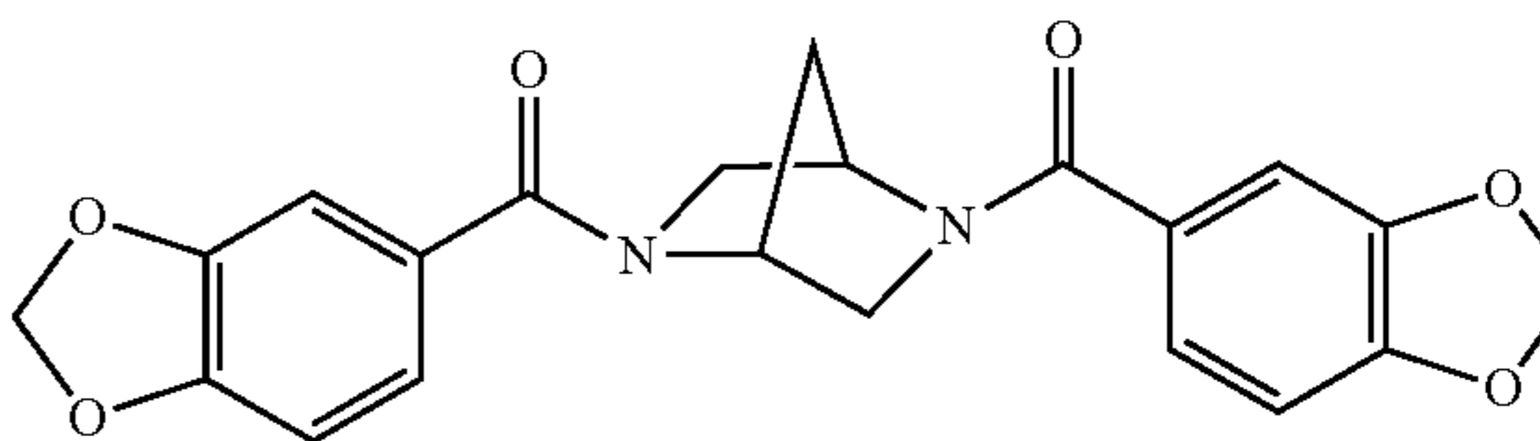
2,5-bis(3,4-methylenedioxybenzoyl)-2,5-diaza[2,2,1]-bicycloheptane
