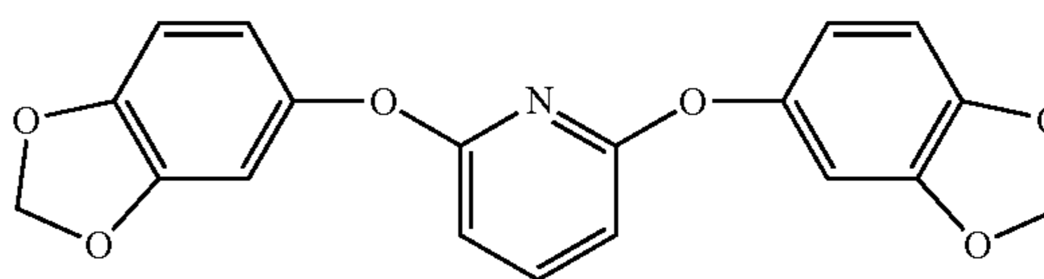
2,6-bis(3,4-methylenedioxyphenoxy) pyridine
