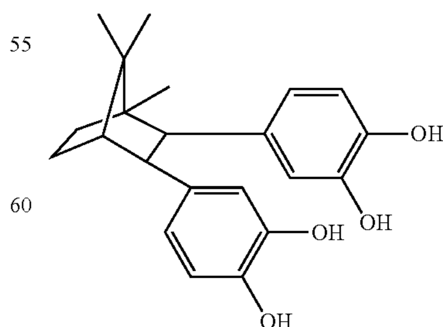
2,3-bis(3,4-dihydroxyphenyl)-1,7,7-trimethyl-bicyclo[2.2.1]heptane
