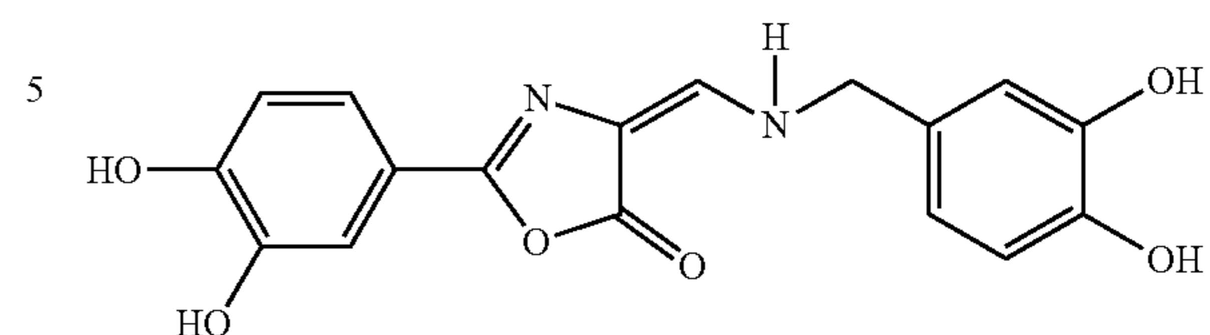
4-(3,4-dihydroxybenzylaminomethylene)-2-(3,4-dihydroxyphenyl)oxazolin-5-one
