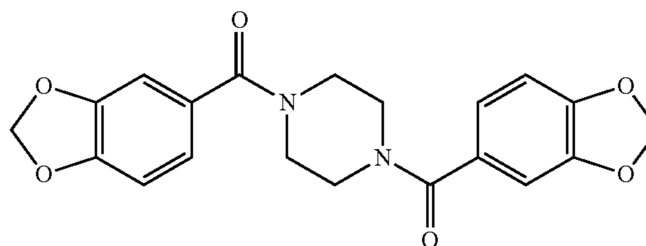
1,4-bis(3,4-methylenedioxybenzoyl)piperazine
