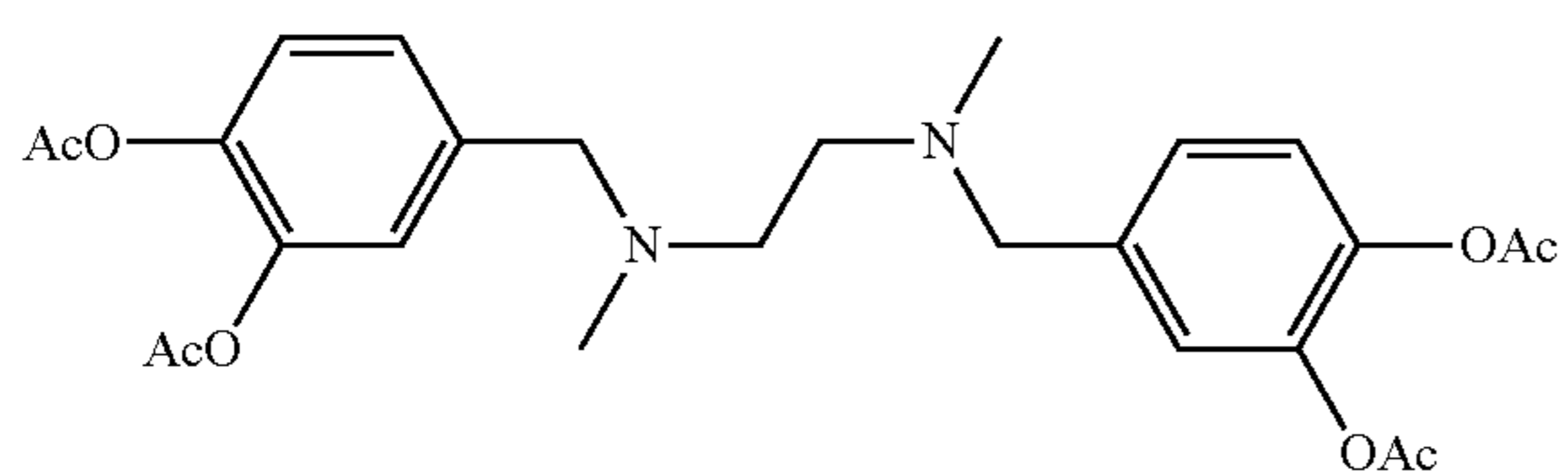
N,N'-bis(3,4-diacetoxybenzyl)- N,N'-dimethyl-ethylenediamine
