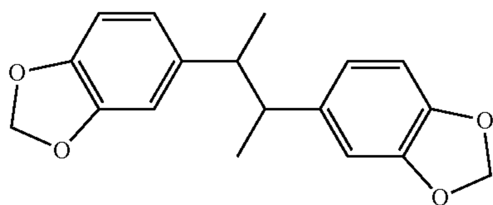
2,3-bis(3,4-methylenedioxyphenyl)butane
