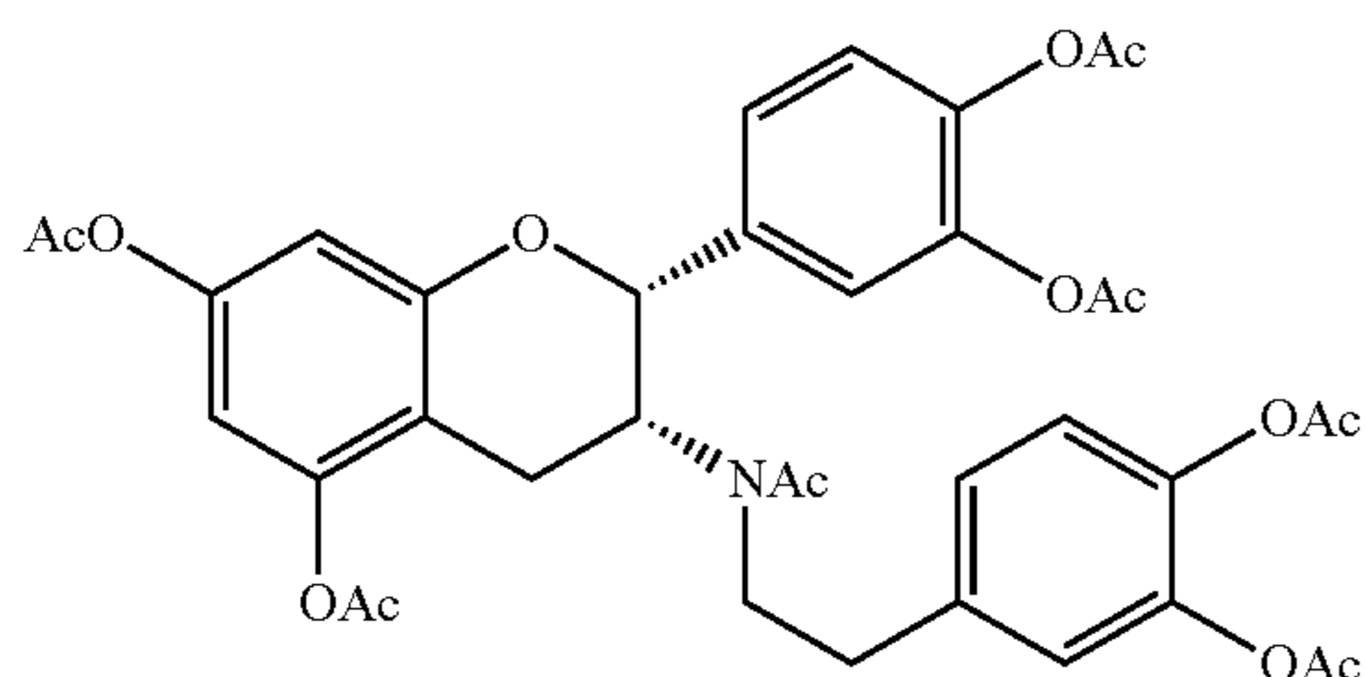
N-acetyl-3-deoxy-3-(3,4-diacetoxypheethyl)-amino-5,7,3',4'-tetraacetyl-epicatechin
