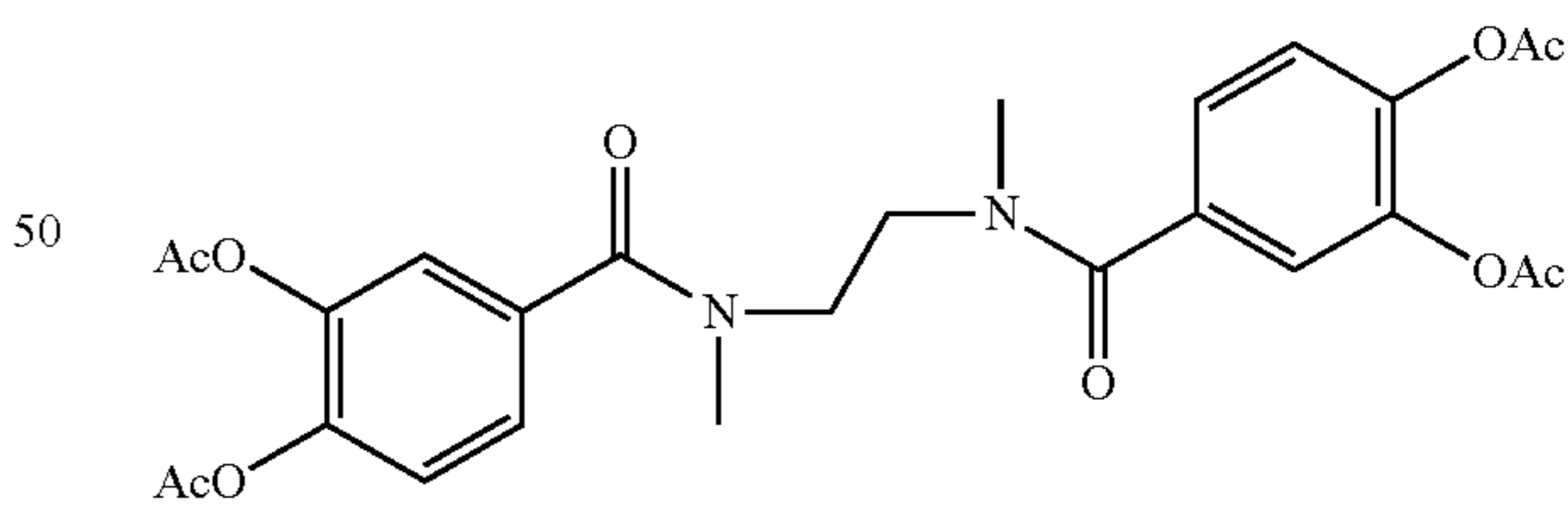
N,N'-bis(3,4-diacetoxybenzoyl)-N,N'-dimethyl(-)ethylenediamine
