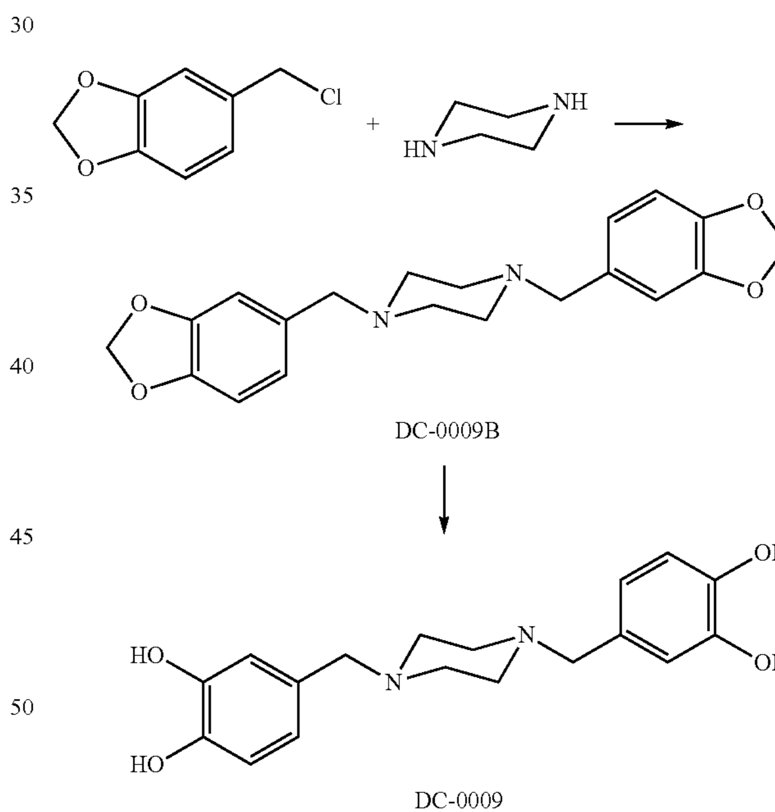
1,4-bis-(3,4-methylenedioxybenzyl)piperazine (DC-0009B)
