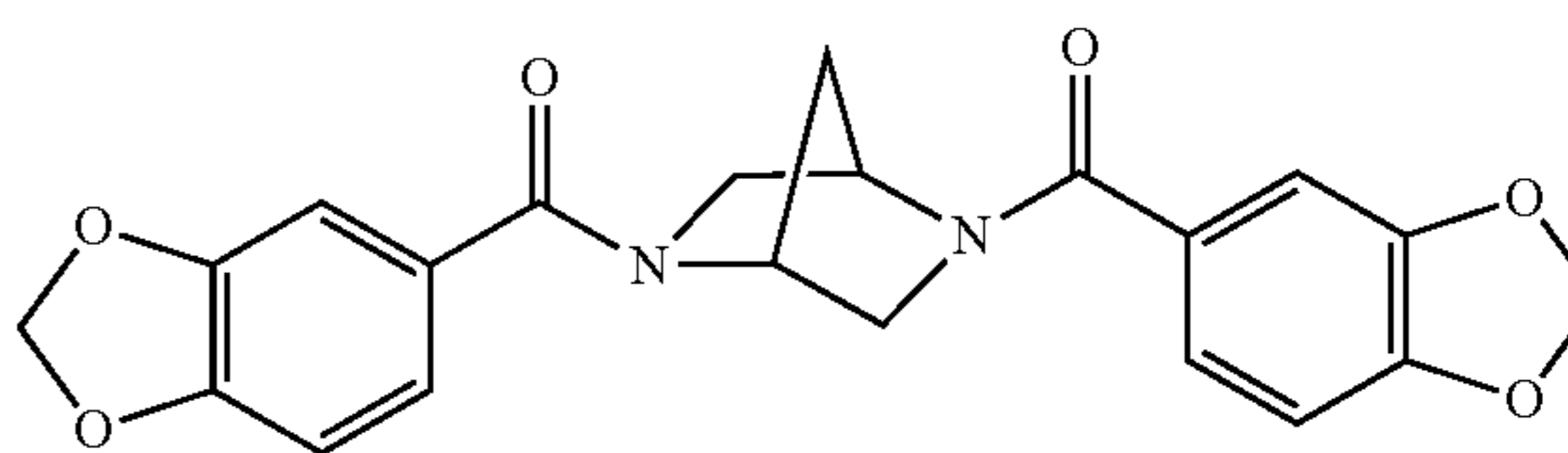
2,5-bis(3,4-methylenedioxybenzoyl)-2,5-diaza[2,2,1]-bicycloheptane
