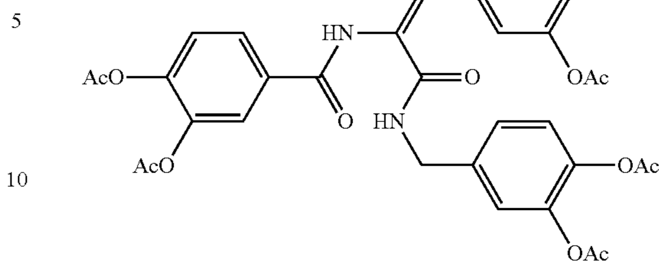
\alpha -(3,4-diacetoxybenzamido)-3,4-diacetoxy(-)cinnamic acid 3,4-diacetoxybenzyl amide
