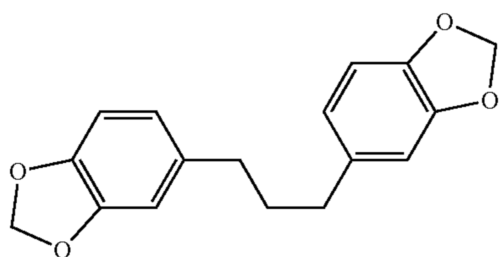
1,3-bis(3,4-methylenedioxyphenyl)propane
