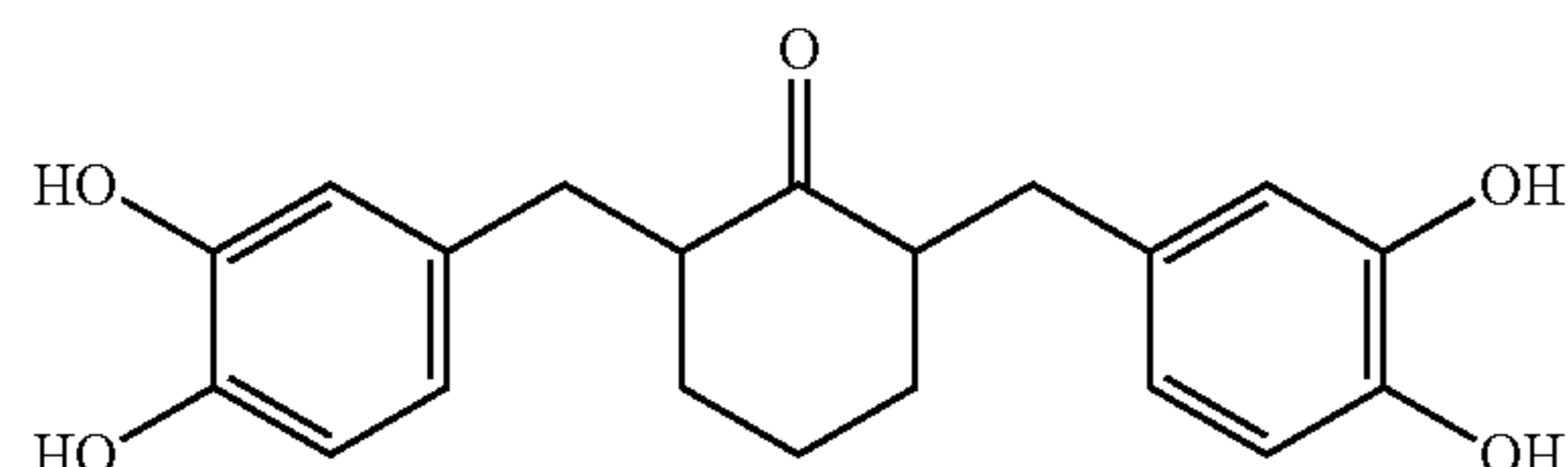
2,6-bis(3,4-dihydroxybenzyl)cyclohexanone
