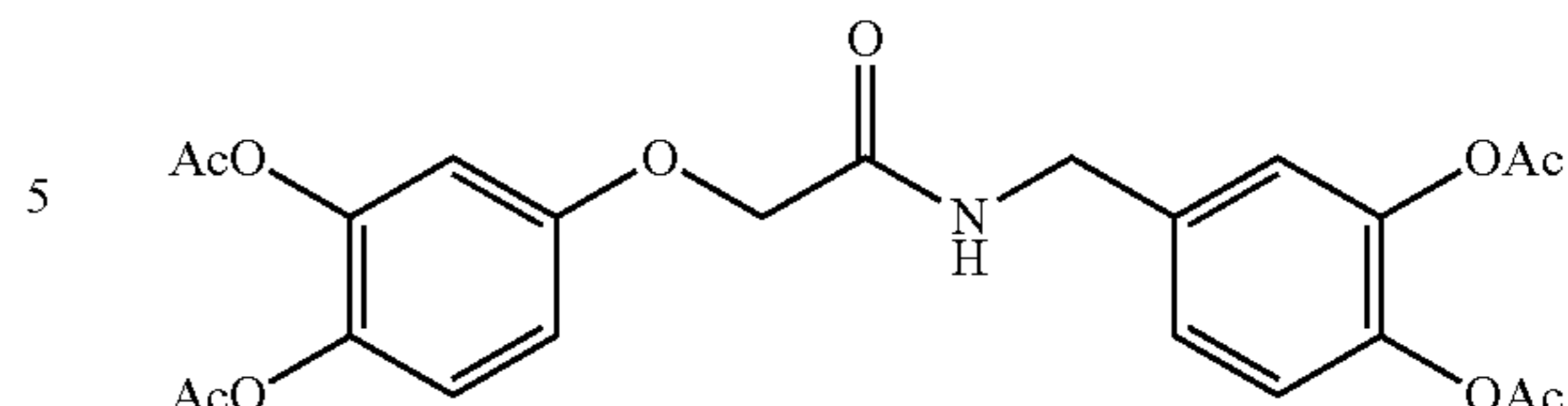
3,4-diacetoxyphenoxyacetic acid 3,4-diacetoxybenzylamide
