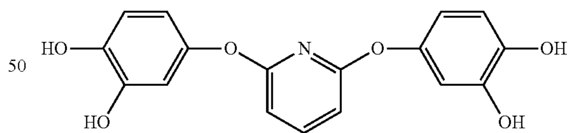
2,6-bis(3,4-dihydroxyphenoxy)pyridine
