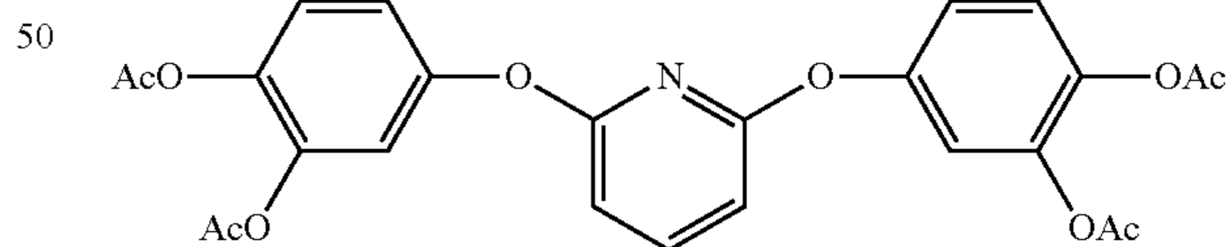
2,6-bis(3,4-diacetoxyphenoxy) pyridine
