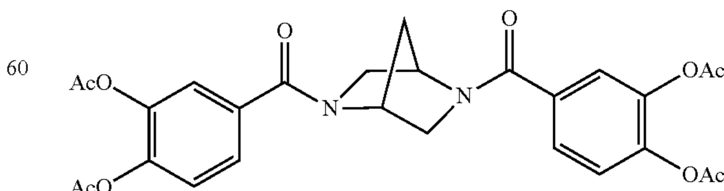
2,5-bis(3,4-diacetoxybenzoyl)-2,5-diaza[2,2,1]-bicycloheptane
