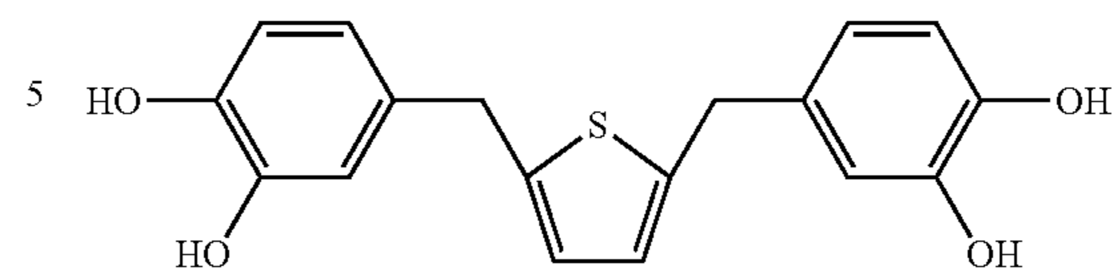
2,5-bis(3,4-dihydroxybenzyl)thiophene
