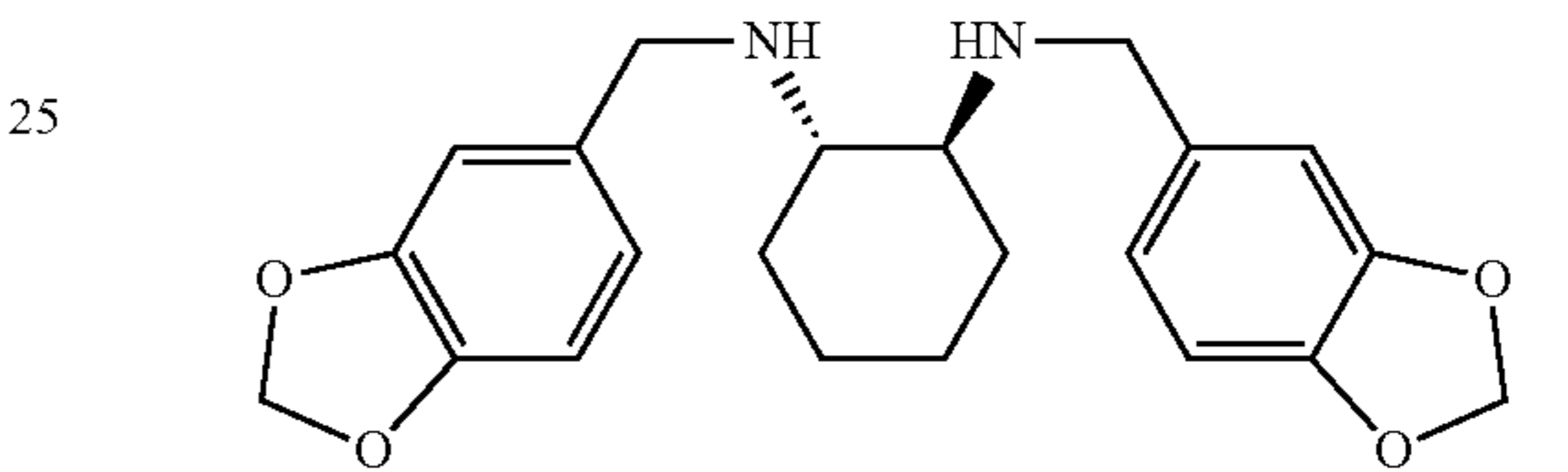
N,N'-bis(3,4-methylenedioxybenzyl)-trans-1,2-diaminocyclohexane
