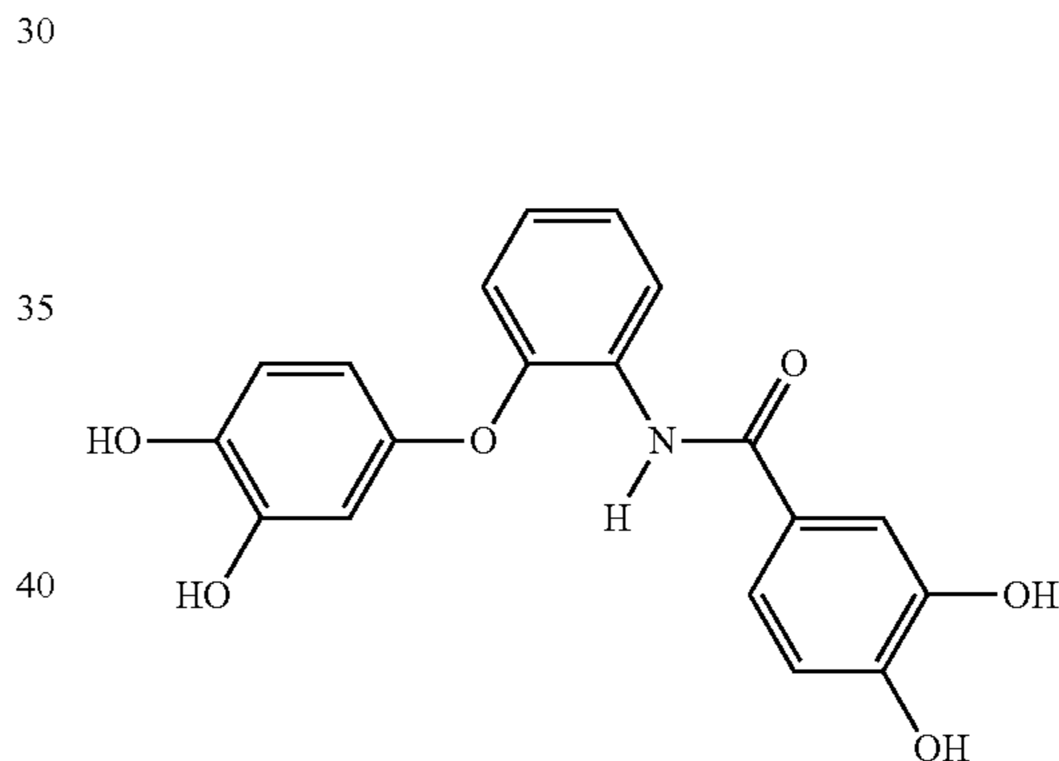
3,4-dihydroxybenzoic acid o-(3,4-dihydrox- phenoxy)anilide
