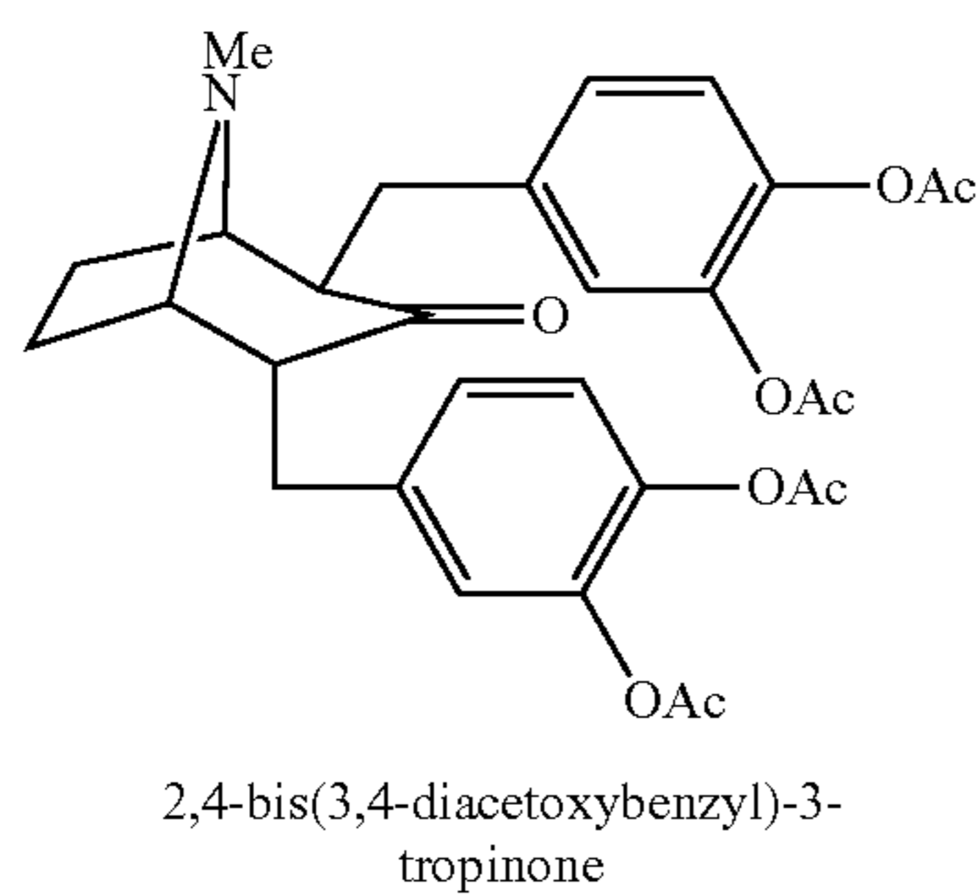
3,5-bis(3,4-diacetoxybenzyl)-1-methyl-4-piperidinone
