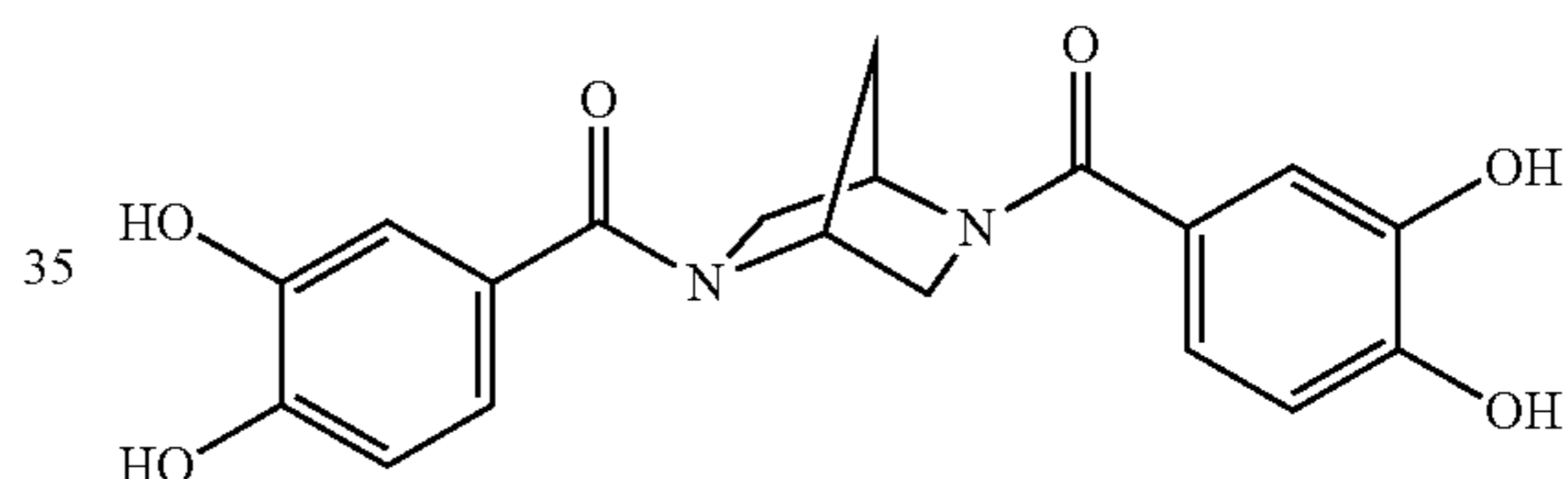
2,5-bis(3,4-dihydroxybenzoyl)-2,5-diaza-[2.2.1]-bicycloheptane
