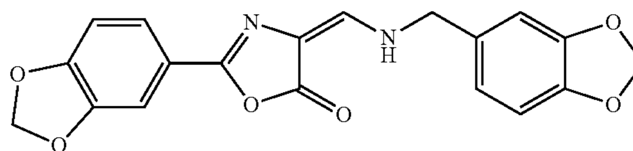
4-(3,4-methylenedioxybenzylaminomethylene)-2-(3,4-methylenedioxyphenyl)oxazolin-5-one
