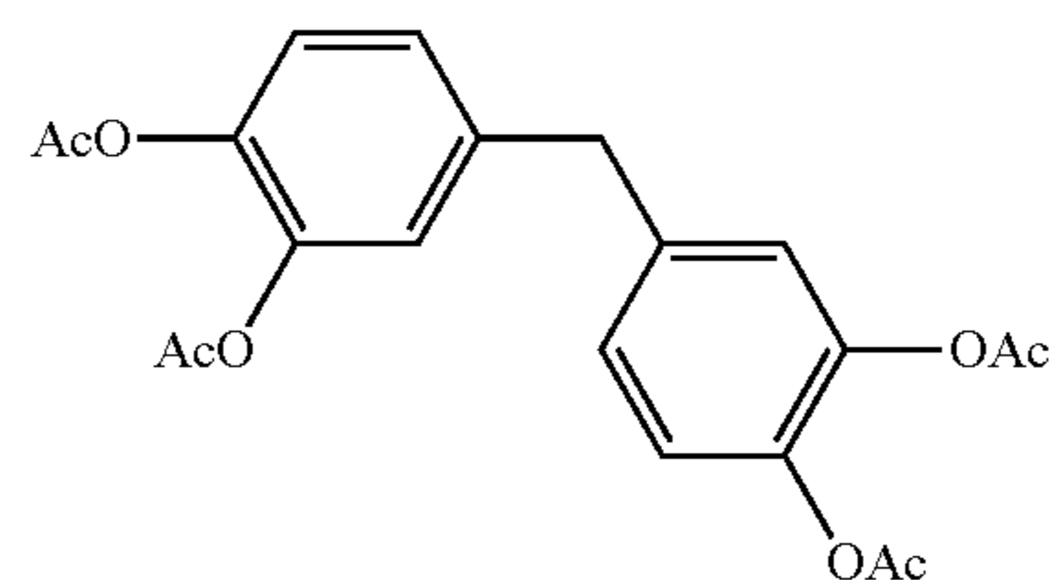
1,1-bis(3,4-diacetoxyphenyl)methane
