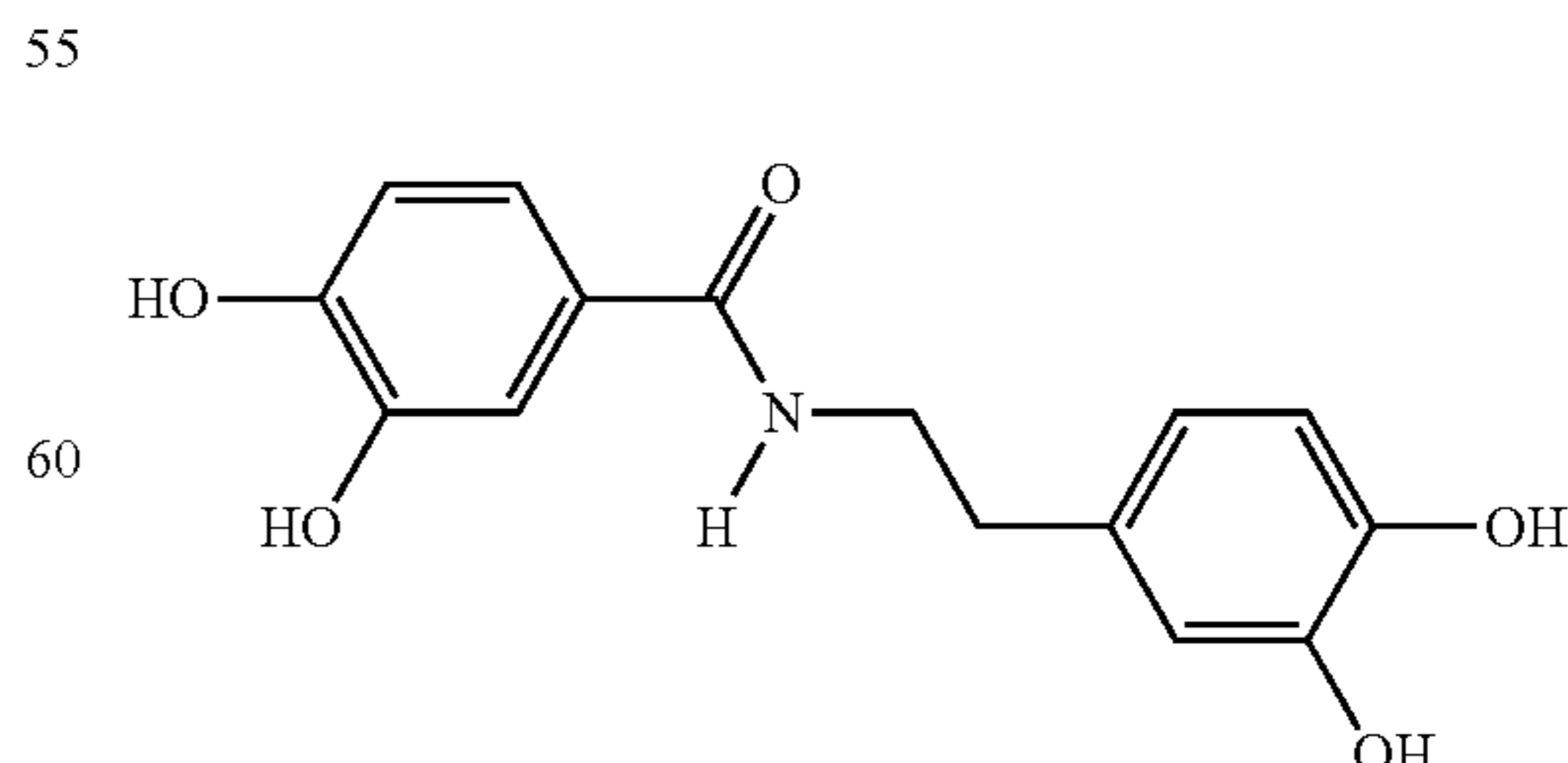
3,4-dihydroxybenzoic acid 3,4-dihydroxy- phenethyl amide
