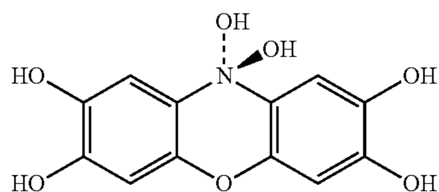
Phenoxazine-2,3,7,8,10-pentaol
