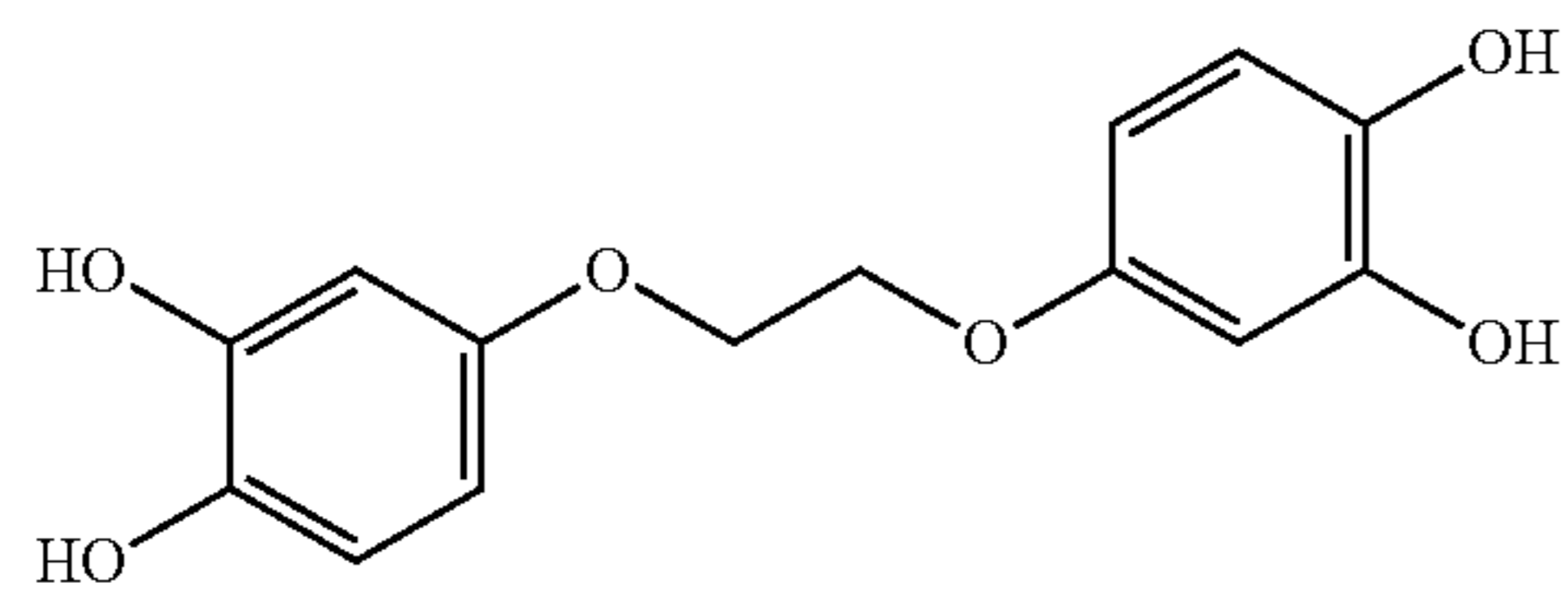
1,2-bis(3,4-dihydroxyphenoxy)ethane
