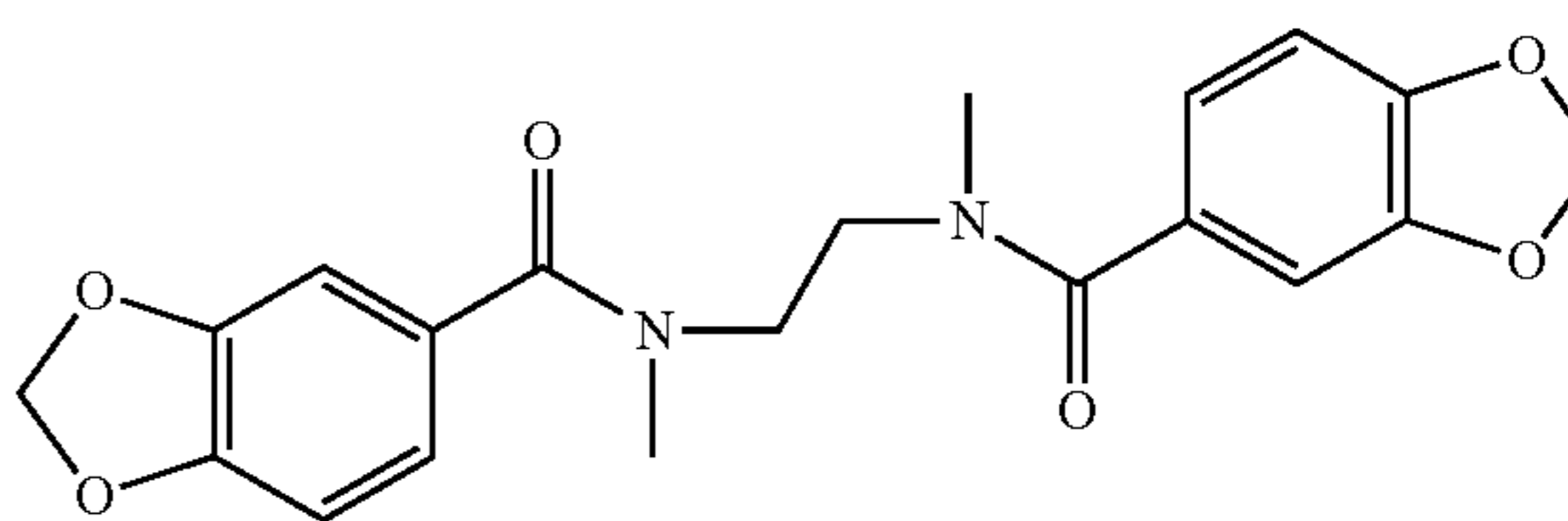
N,N'-bis(3,4-methylenedioxybenzoyl)-N,N'-dimethyl(-)ethylenediamine
