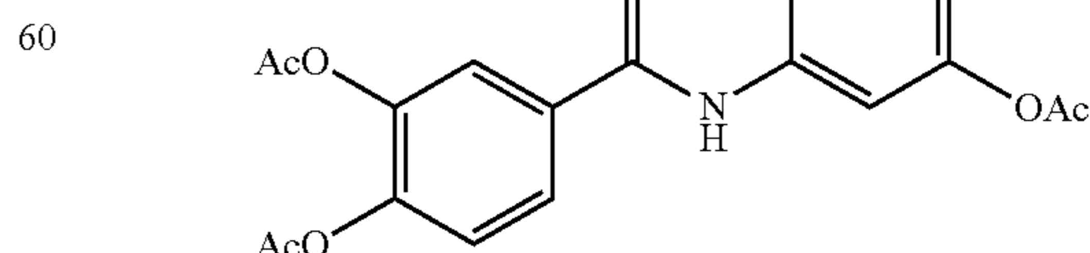
3,4-diacetoxybenzoic acid 3,4-diacetoxyanilide
