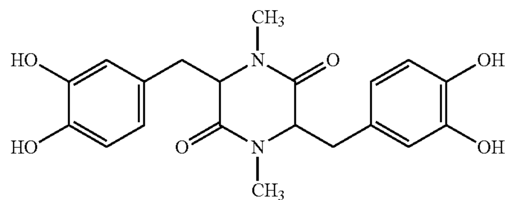
3,6-bis(3,4-dihydroxybenzylidene)-1,4-dimethyl-2,5-diketopiperazine
