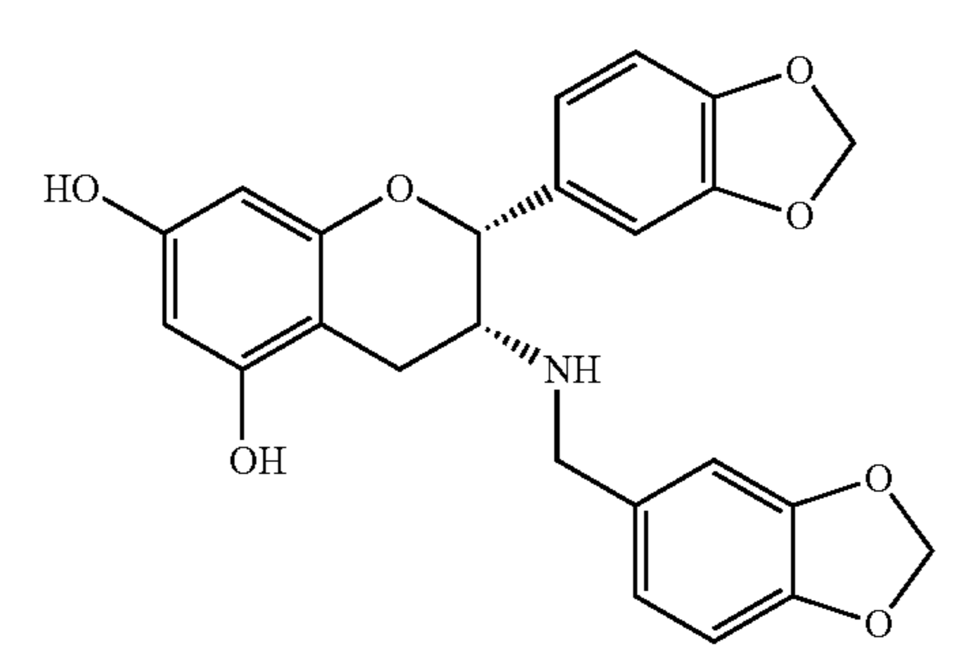
3-deoxy-3-(3,4-methylenedioxybenzyl)-aminoepicatechin
