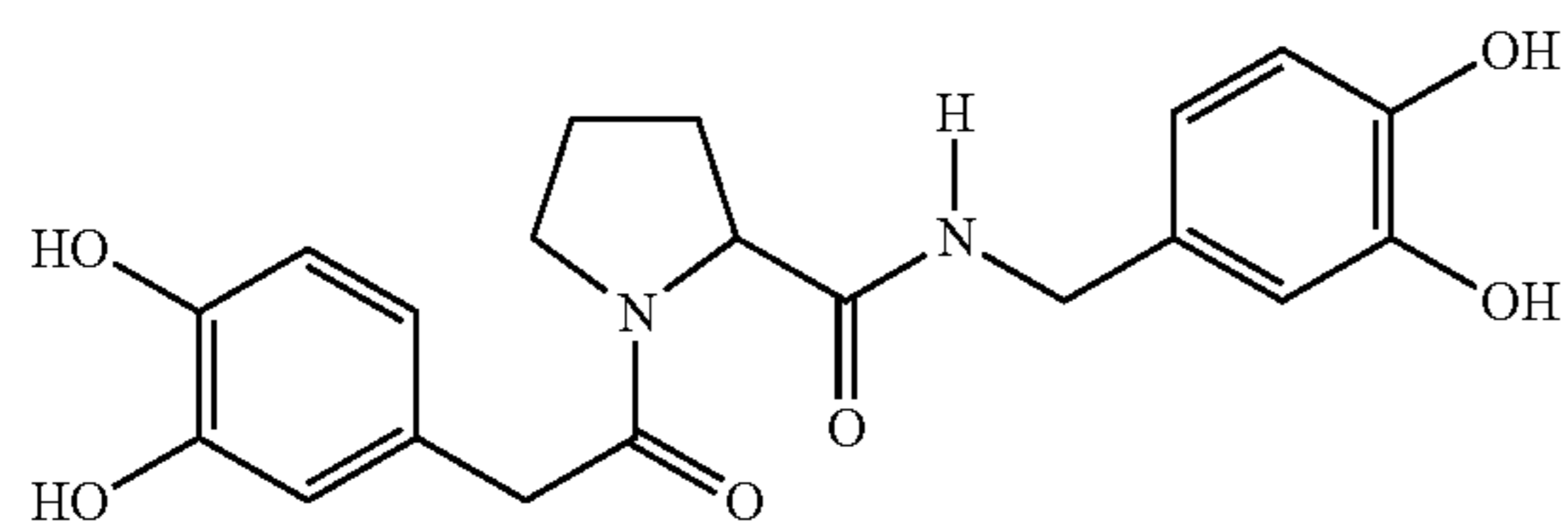
N-(3,4-hydroxyphenylacetyl)proline-3,4-dihydroxyanilide
