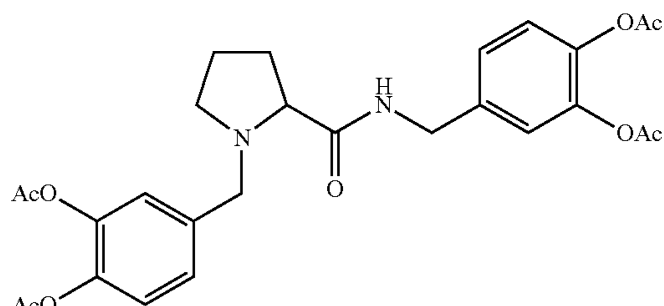
N-(3,4-diacetoxybenzyl)proline 3,4- diacetoxybenzylamide
