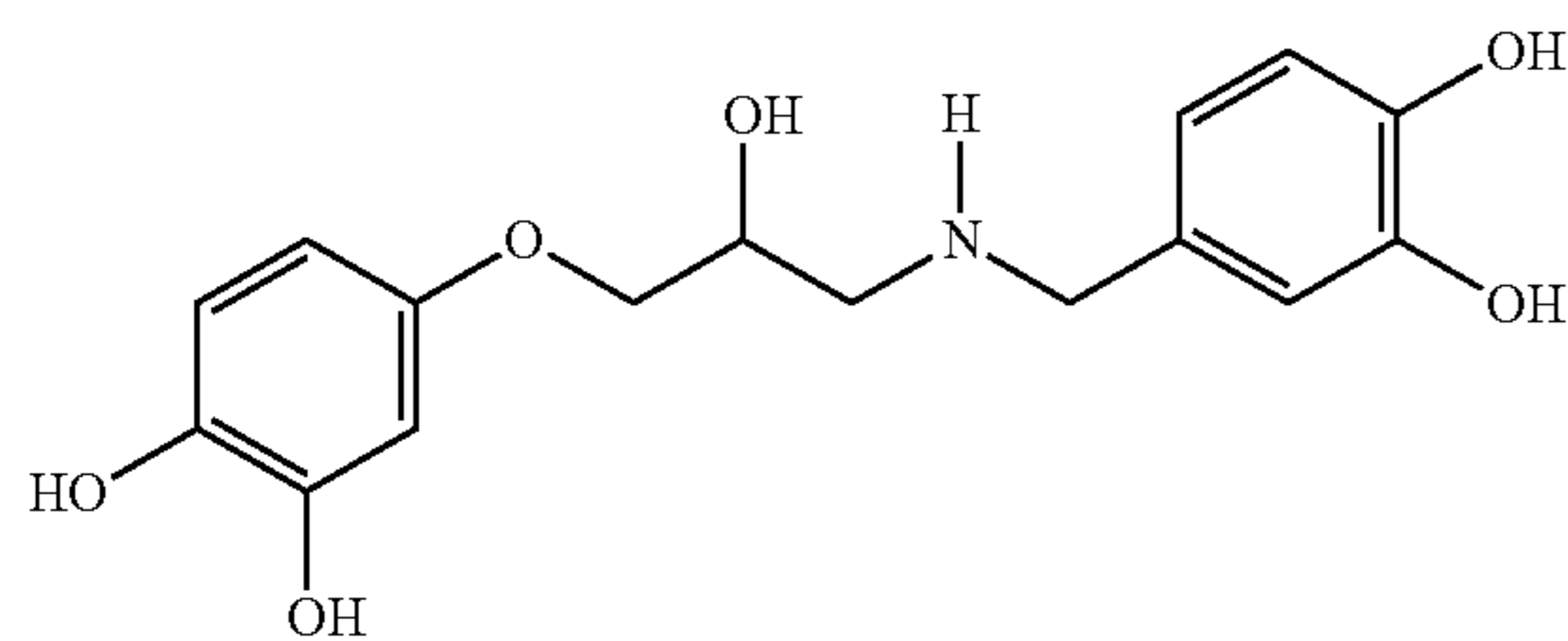
N-(3,4-dihydroxybenzyl)-3-(3,4-dihydrox- propyl)amine
