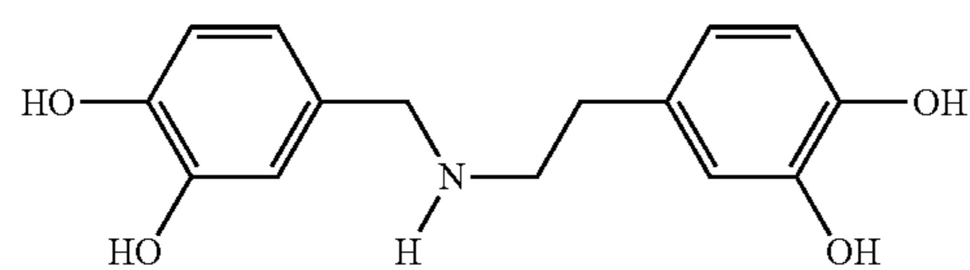
N-(3,4-dihydroxybenzyl)-3,4-dihydroxy(-)-phenethylamine
