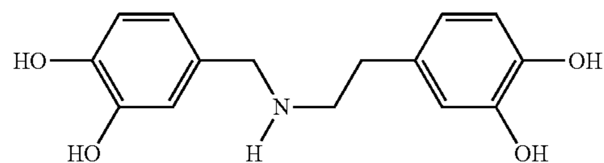
N-(3,4-dihydroxybenzyl)-3,4-dihydroxy(-)-phenethylamine
