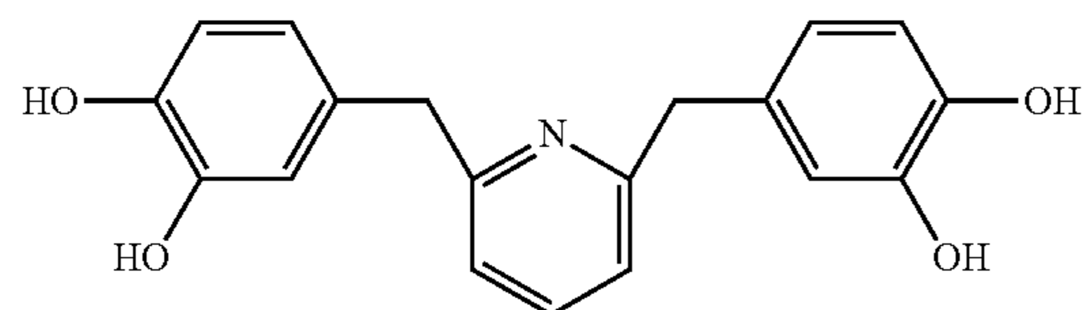
2,6-bis(3,4-dihydroxybenzyl)pyridine
