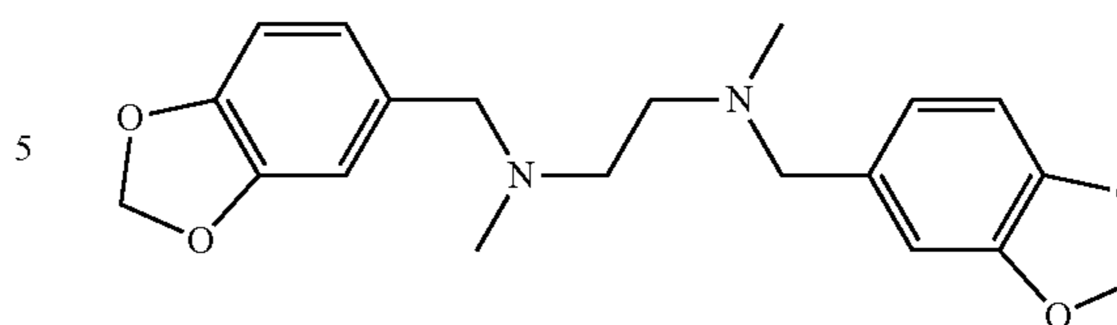
N,N'-bis(3,4-methylenedioxybenzyl)-N,N'-dimethyl-ethylenediamine
