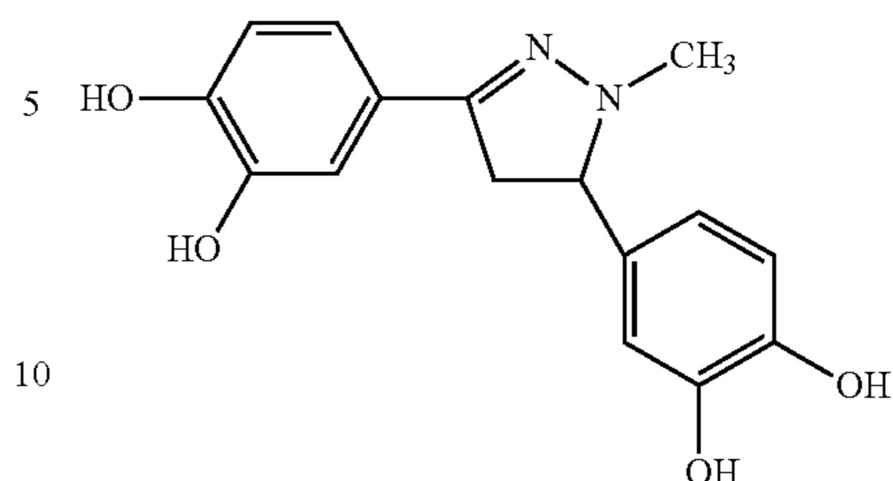
3,5-bis(3,4-dihydroxyphenyl)-1-methyl-1H-pyrazoline
