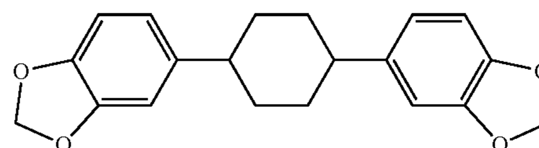
1,4-bis(3,4-methylenedioxyphenyl)cyclohexane
