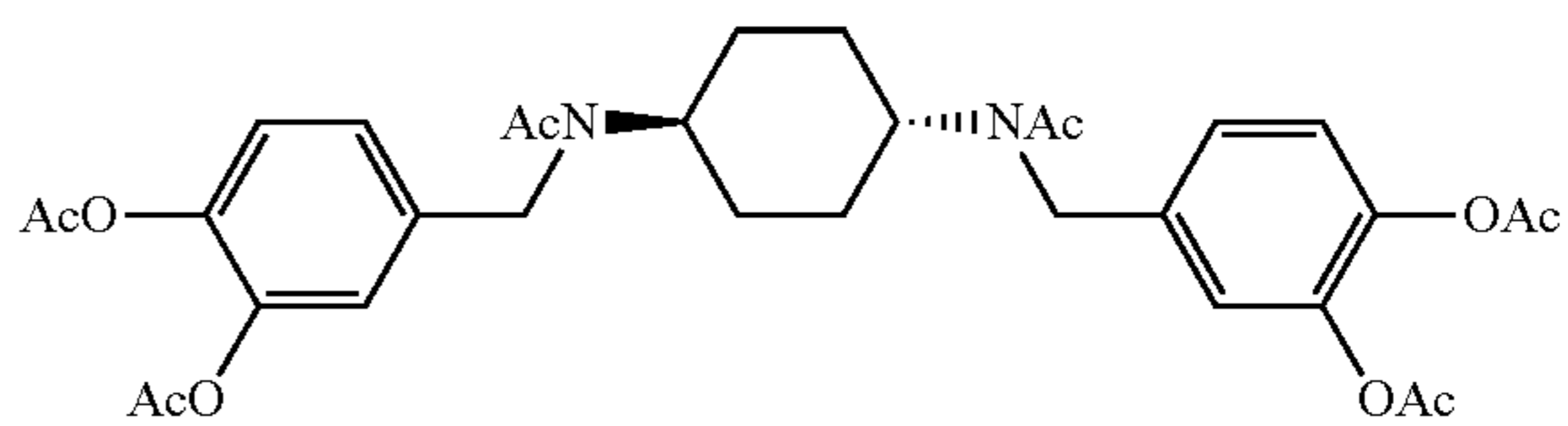
N,N'-bis(acetyl)-bis(3,4-diacetoxybenzyl)- trans-1,4-diaminocyclohexane
