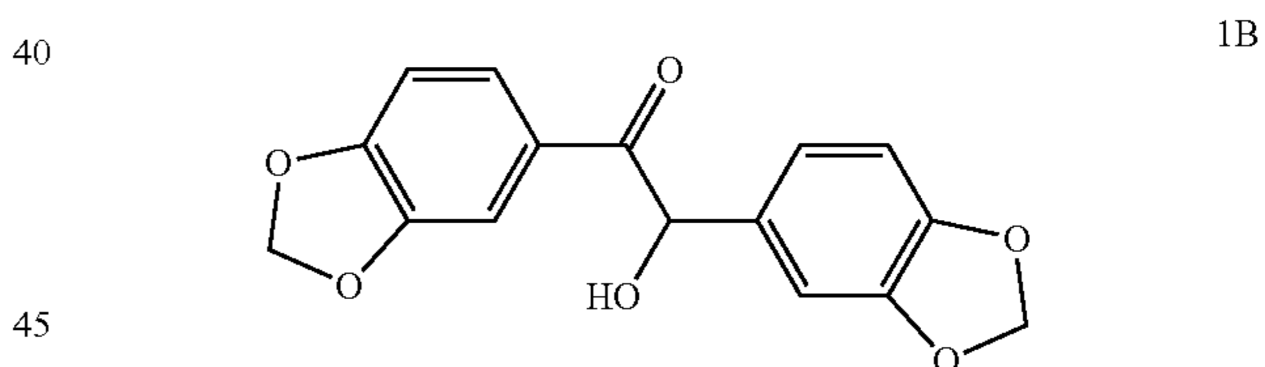
bis(3,4-methylenedioxy)benzoic acid
