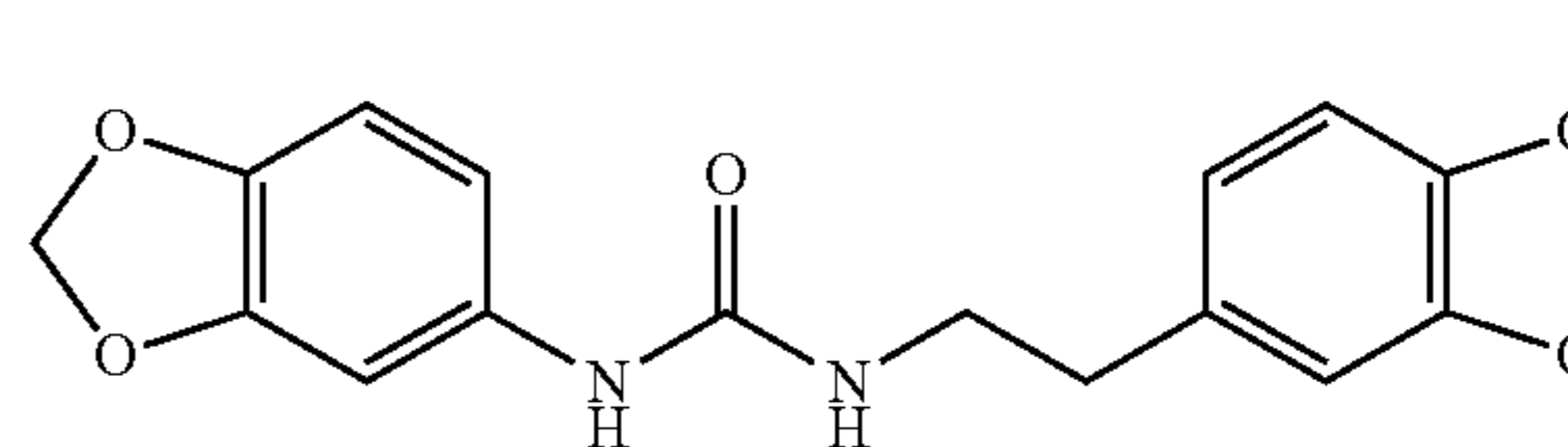
1-(3,4-methylenedioxyphenyl)-3-(3,4-methylenedioxyphenethyl) urea
