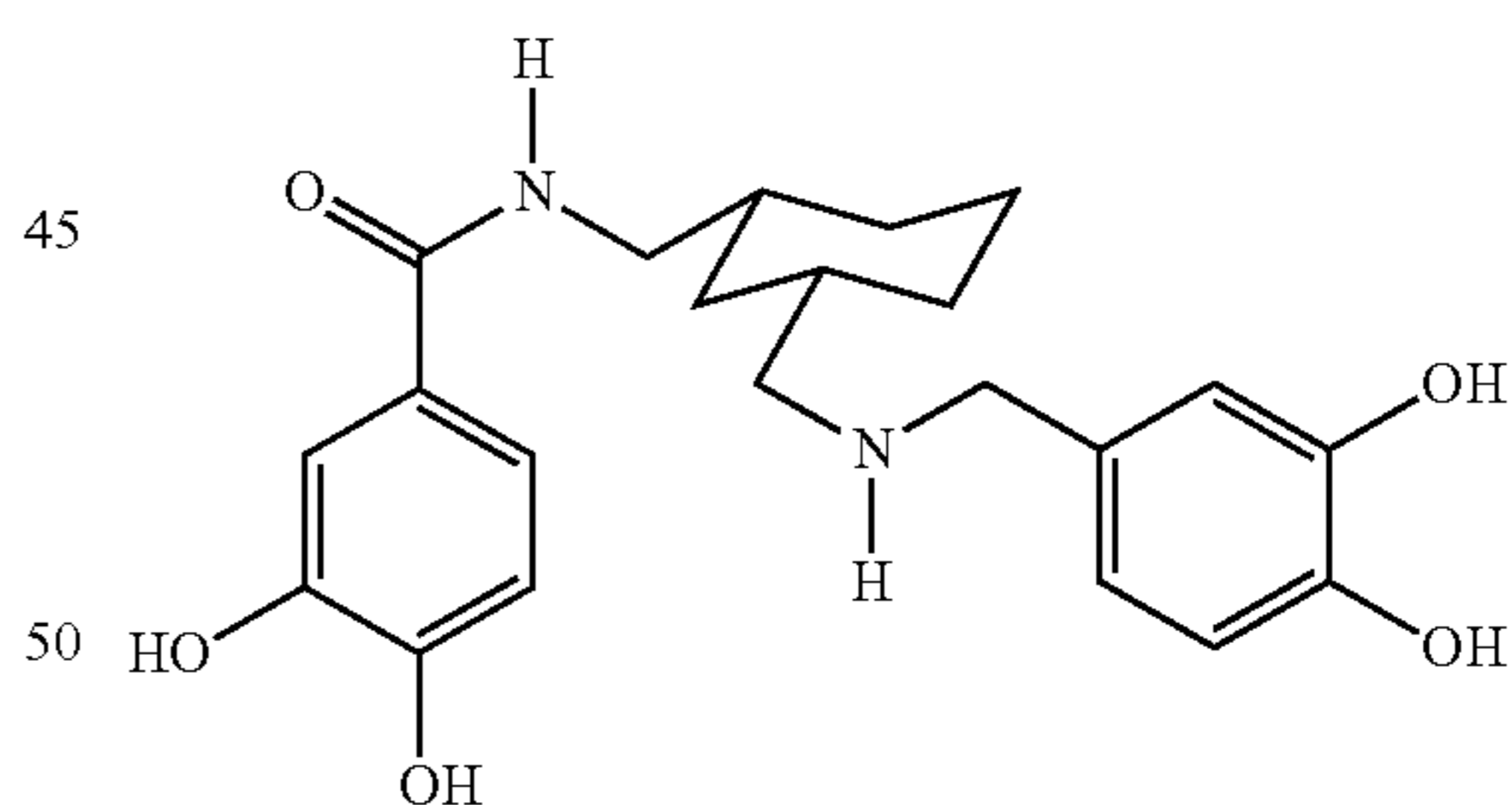
N,N'-bis(3,4-dihydroxybenzoyl)-cis-1,3-bis-aminomethylcyclohexane
