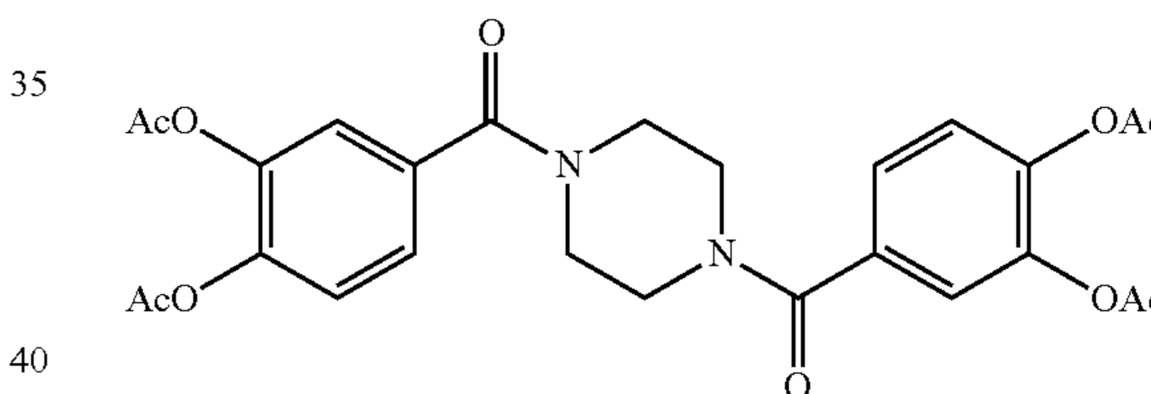
1,4-bis(3,4-diacetoxybenzoyl)piperazine
