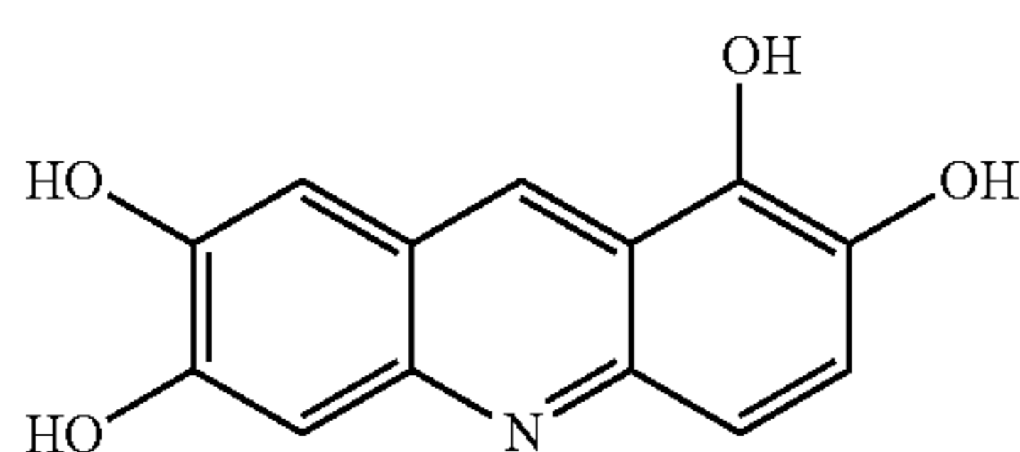
Acridine-1,2,6,7-tetraol
