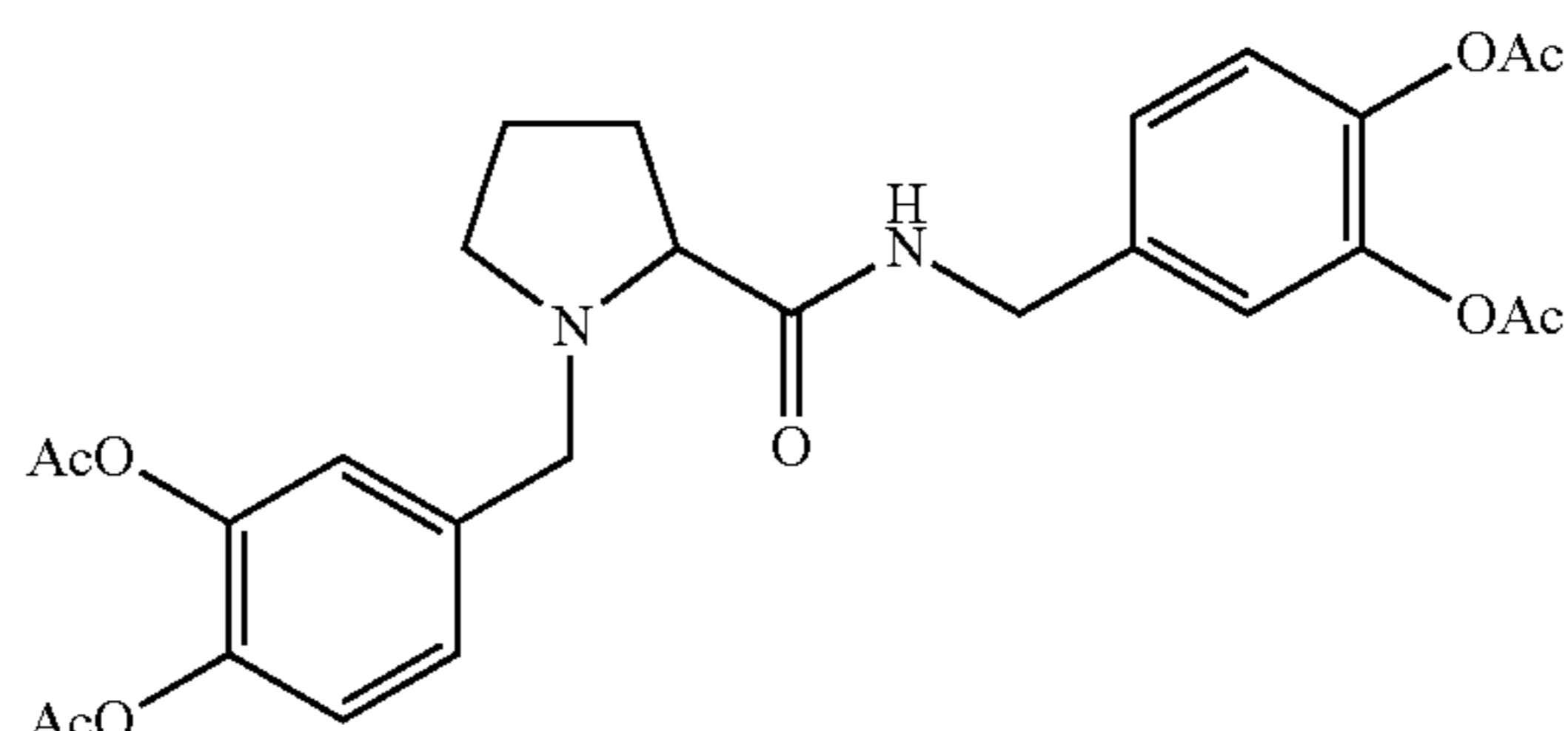
N-(3,4-diacetoxybenzyl)proline 3,4- diacetoxybenzylamide
