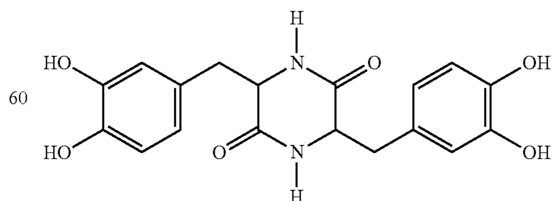
3,6-bis(3,4-dihydroxybenzyl)-1-methyl-2,5-diketopiperazine
