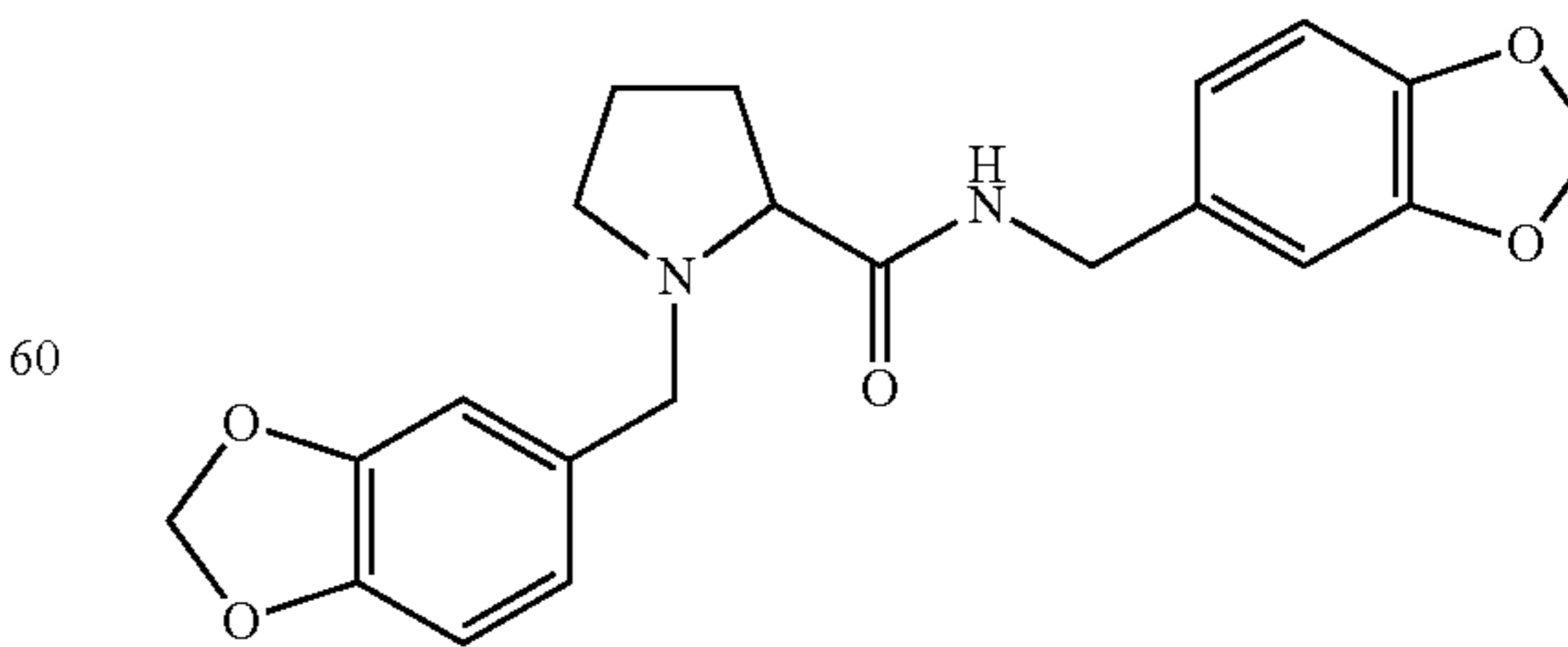
N-(3,4-methylenedioxybenzyl)proline 3,4-methylenedioxybenzylamide
