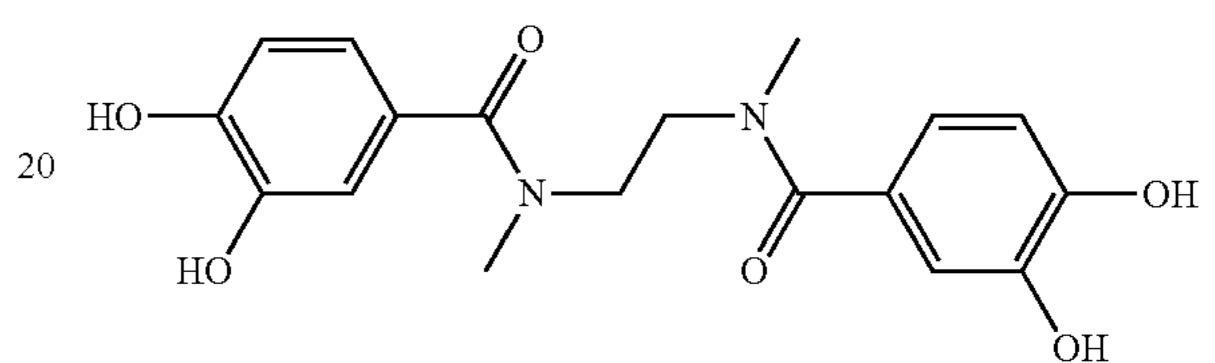
N,N'-bis(3,4-dihydroxybenzoyl)-N,N'-dimethyl(-)ethylenediamine
