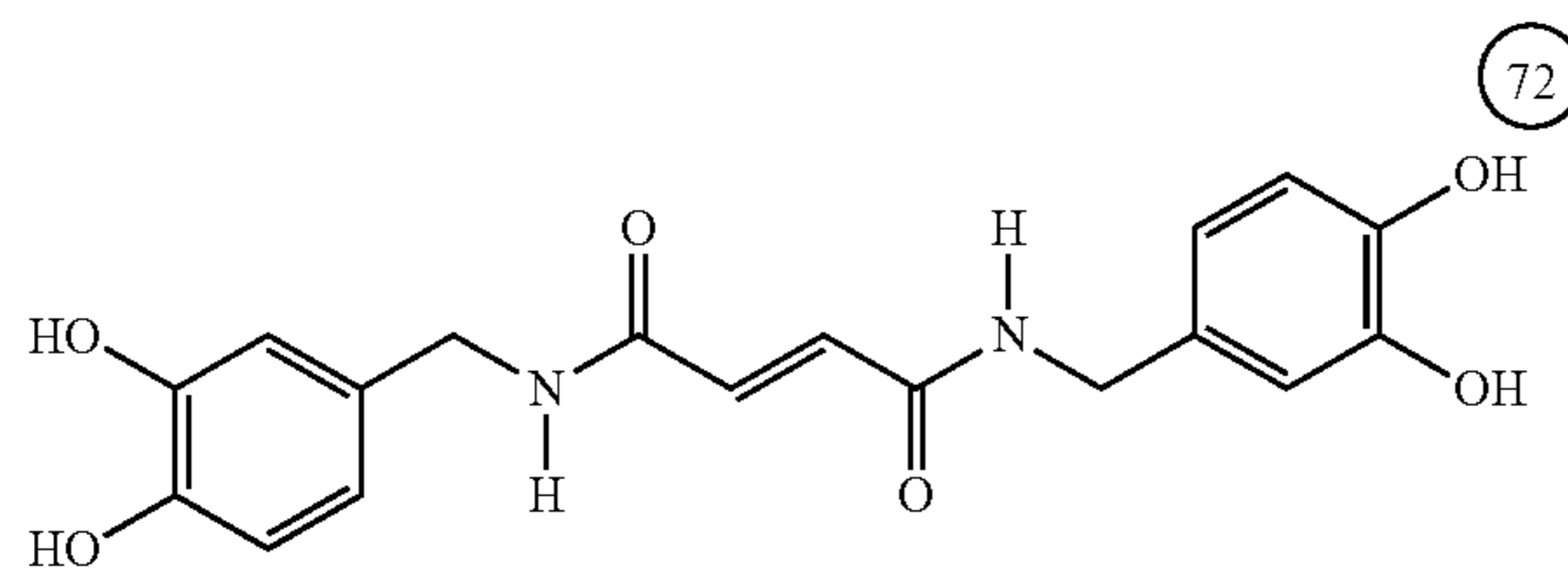
Fumaric acid bis-(3,4-dihydroxybenzylamide)
