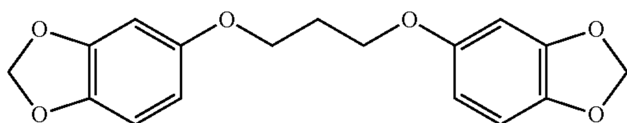
1,3-bis(3,4-methylenedioxyphenoxy) propane
