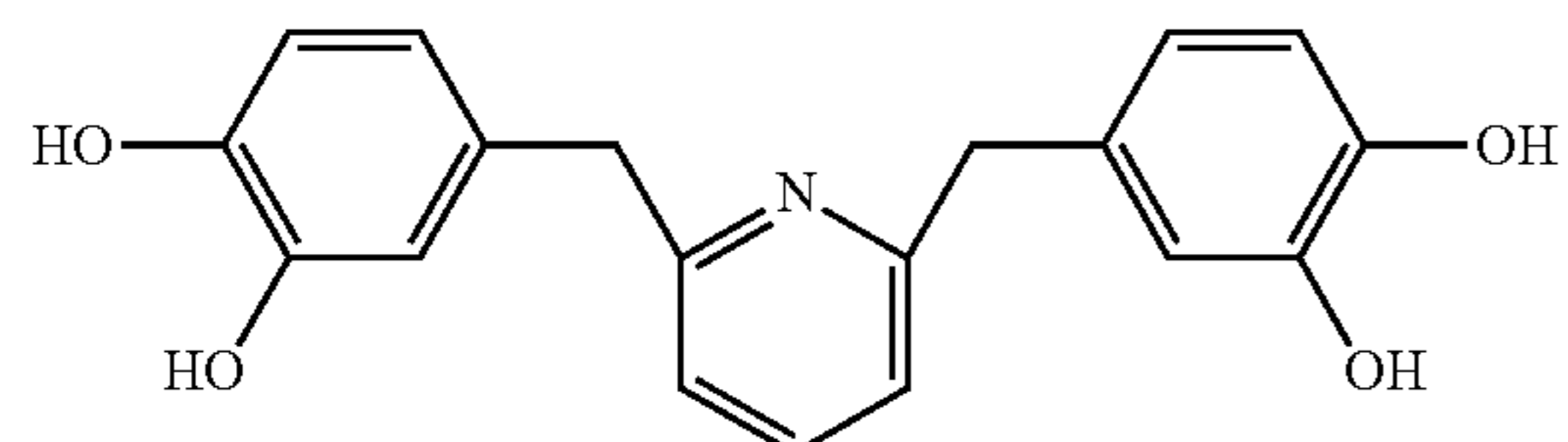
2,6-bis(3,4-dihydroxybenzyl)pyridine
