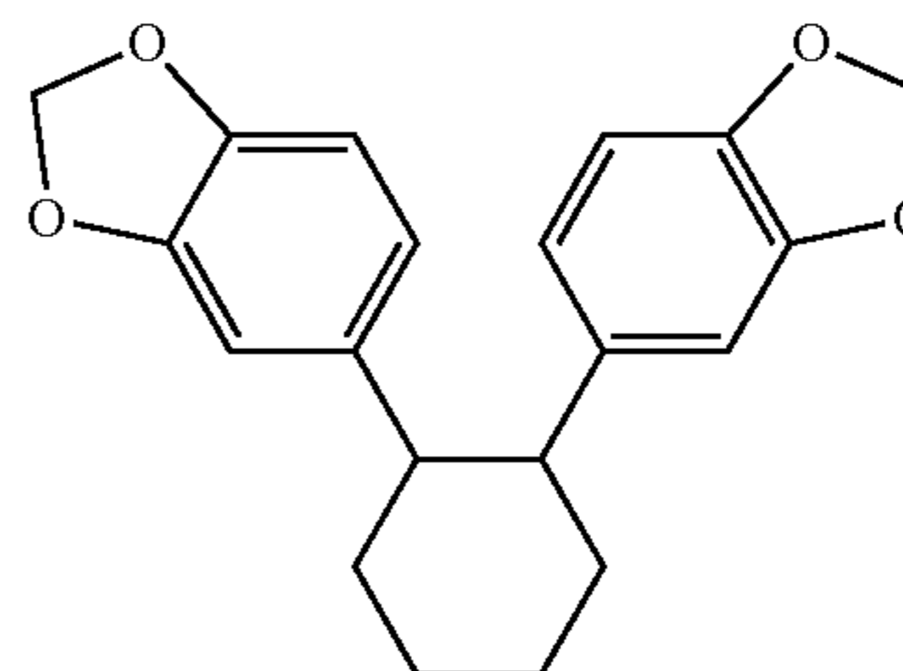
1,2-bis(3,4-methylenedioxyphenyl)cyclohexane
