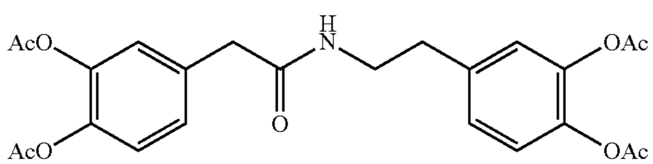
3,4-diacetoxyphenylacetic acid 3,4-diacetoxyphenethylamide
