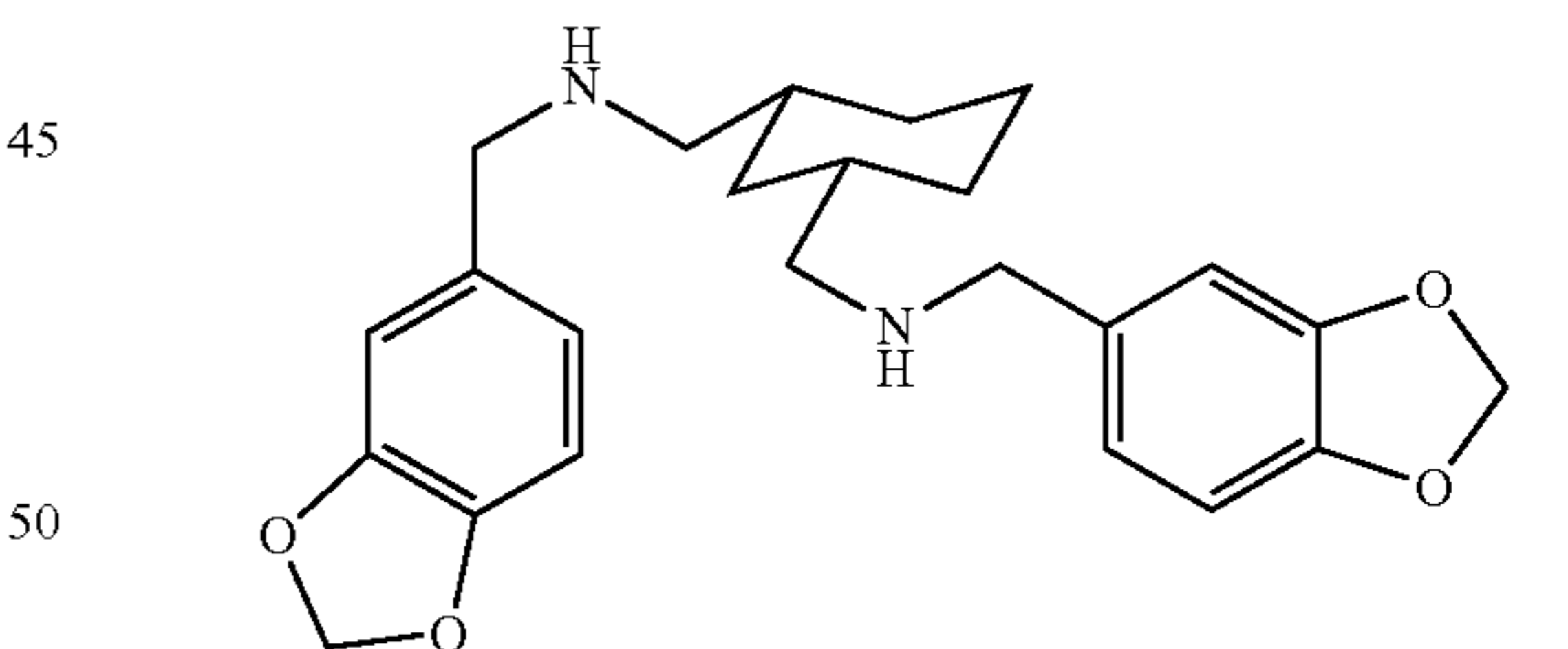
N,N'-bis(3,4-methylenedioxybenzyl)-cis-1,3-bis-aminomethylcyclohexane
