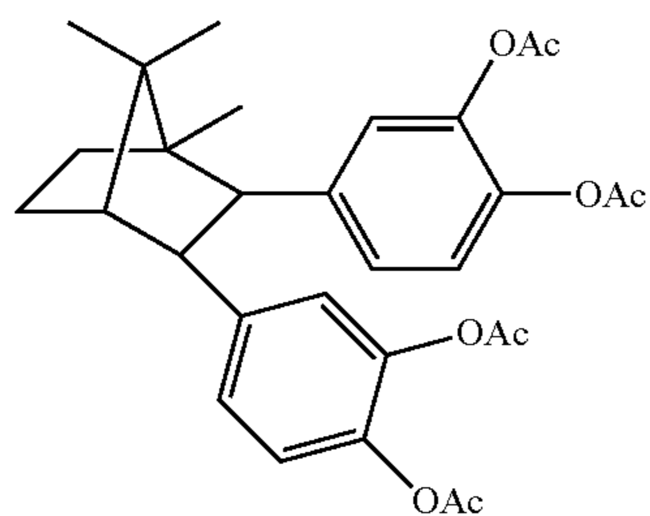
2,3-bis(3,4-diacetoxyphenyl)- 1,7,7-trimethyl-bicyclo[2,2,1]heptane
