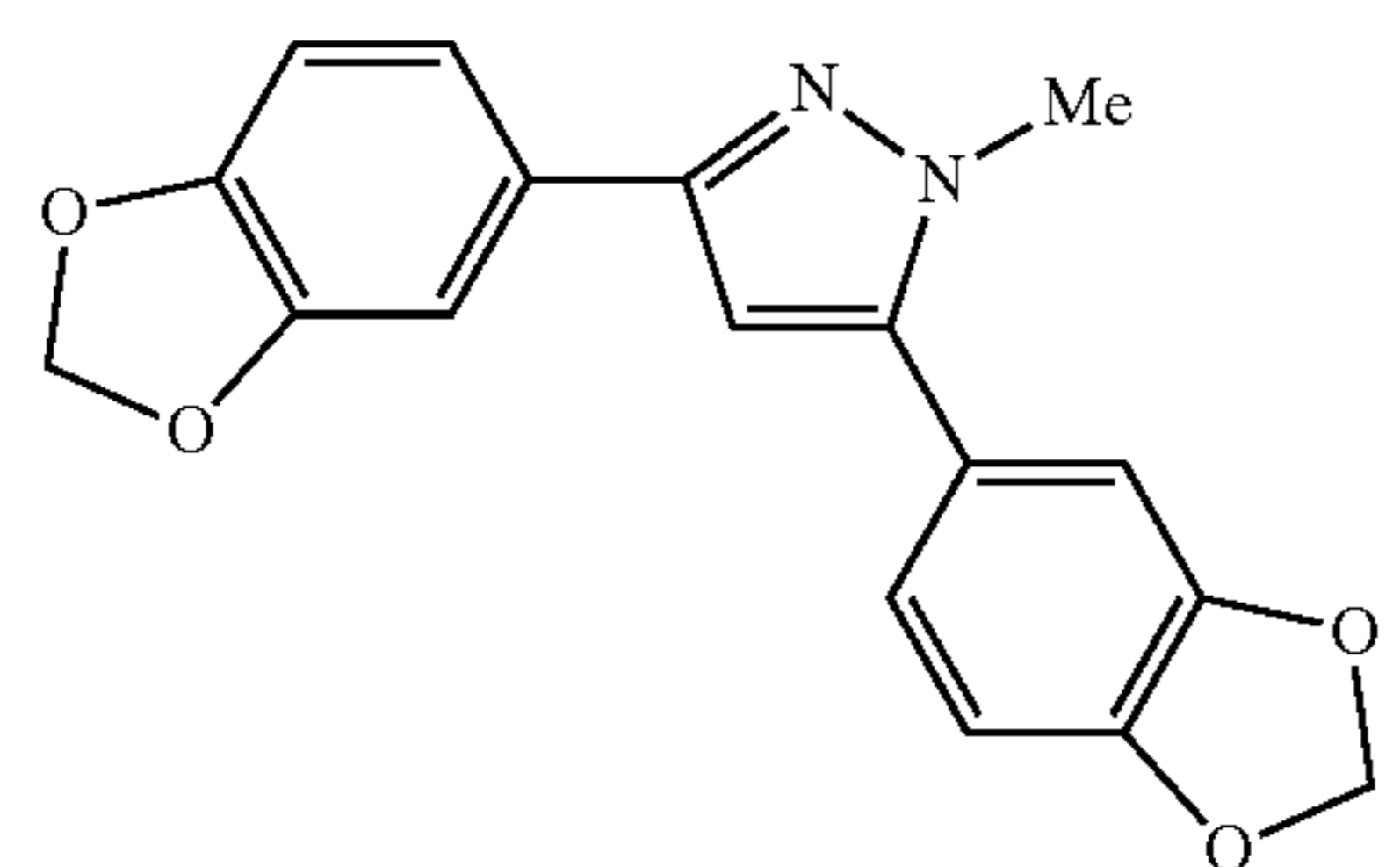
3,5-bis(3,4-methylenedioxyphenyl)- 1-methyl-1H-pyrazoline
