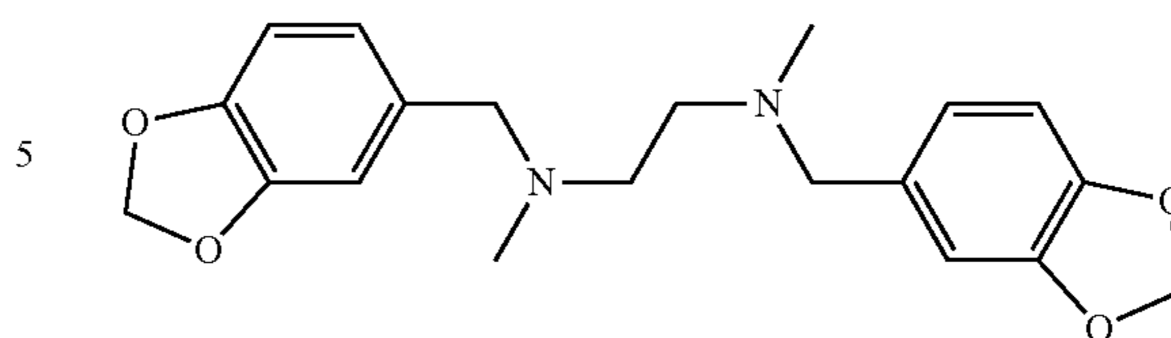
N,N'-bis(3,4-methylenedioxybenzyl)- N,N'-dimethyl-ethylenediamine
