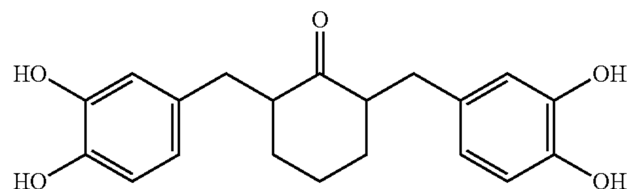
2,6-bis(3,4-dihydroxybenzyl)cyclohexanone
