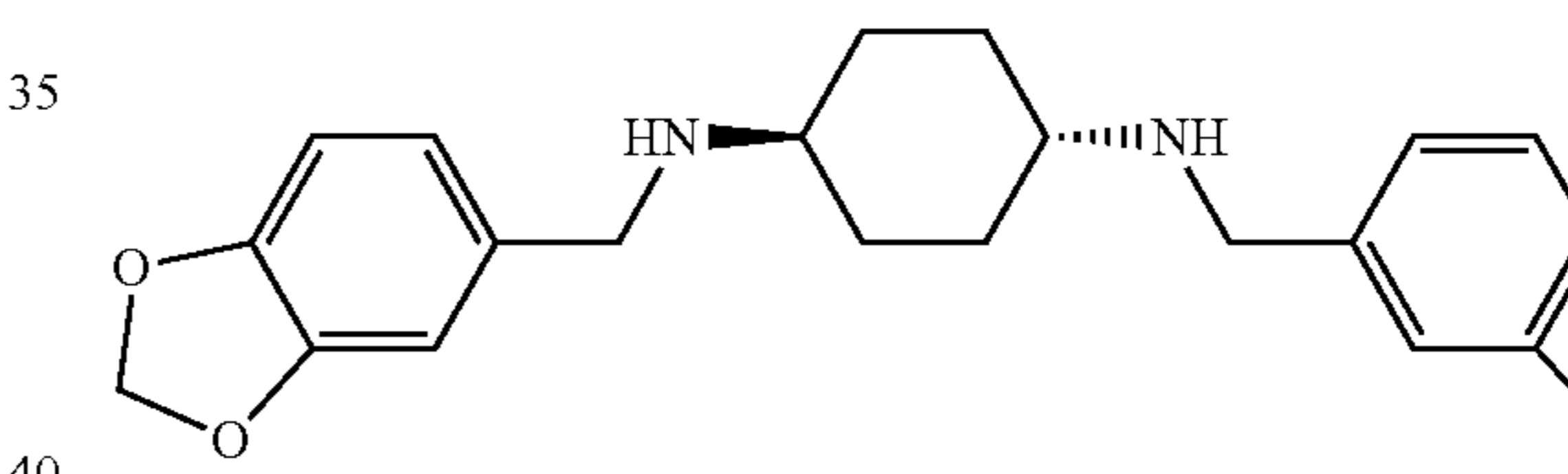
N,N'-bis(3,4-methylenedioxybenzyl)-trans-1,4-diaminocyclohexane
