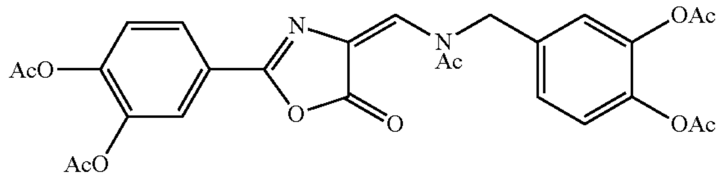
N-acetyl-4-(3,4-diacetoxybenzylamino)methylene)-2-(3,4-diacetoxyphenyl)-oxazolin-5-one
