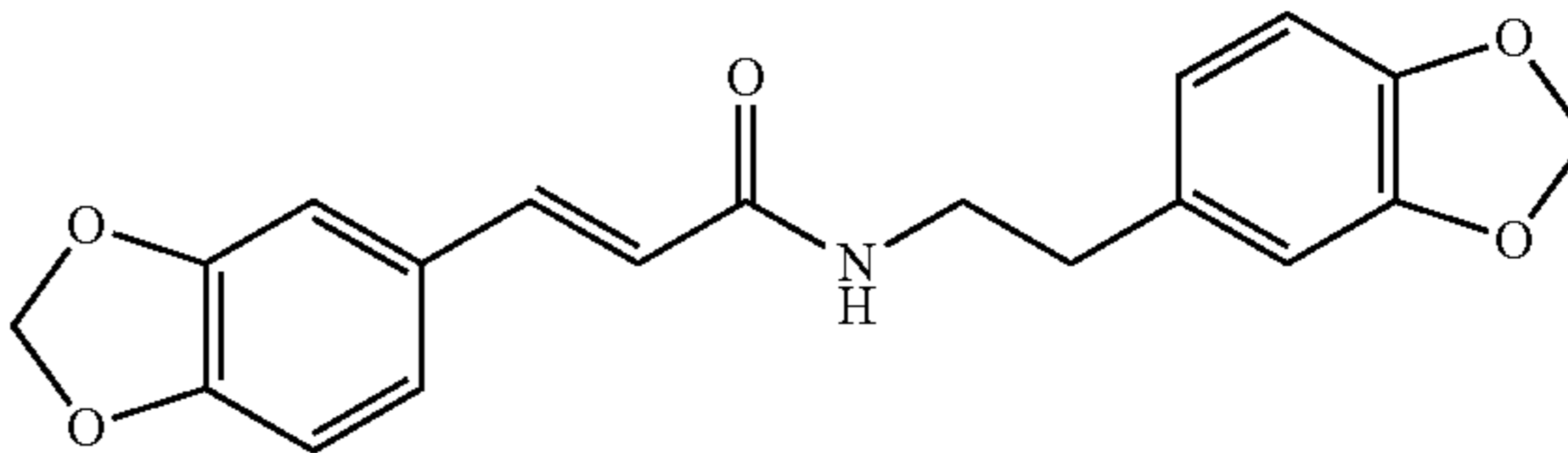
3,4-methylenedioxycinnamic acid 3,4-methylenedioxyphenethylamide
