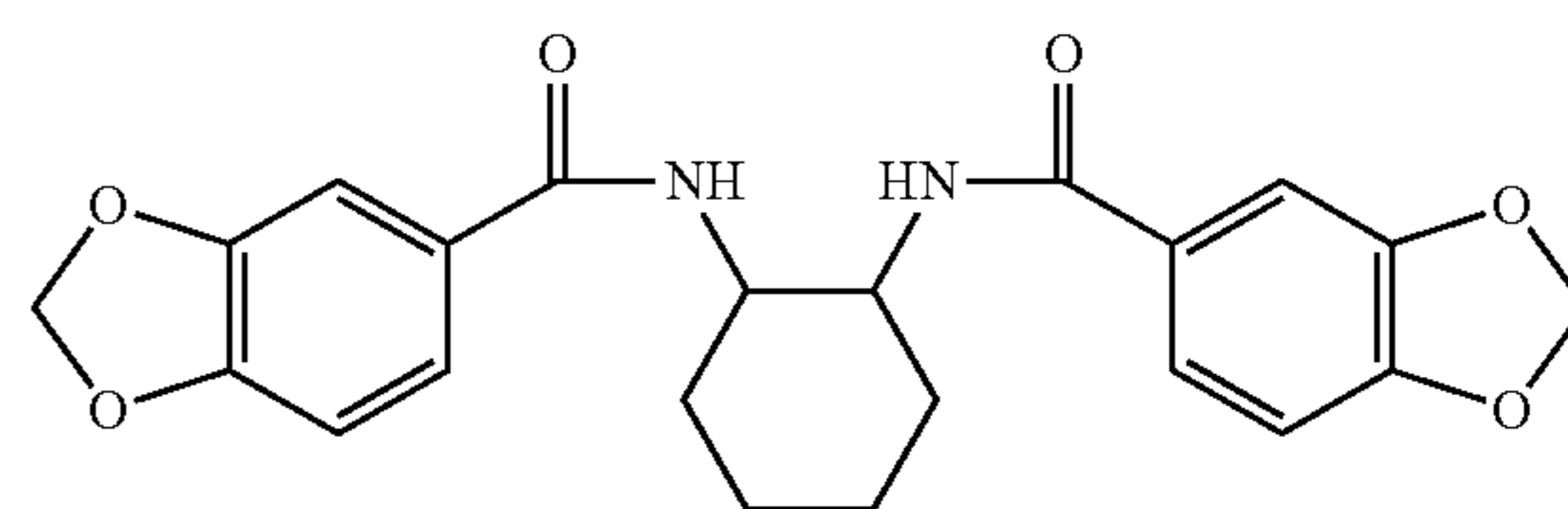
N,N'-bis(3,4-methylenedioxybenzoyl)-trans-diaminocyclohexane
