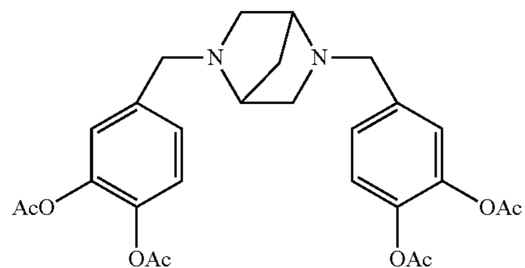
2,5-bis(3,4-diacetoxybenzyl)-2,5- diaza[2,2,1]-bicycloheptane
